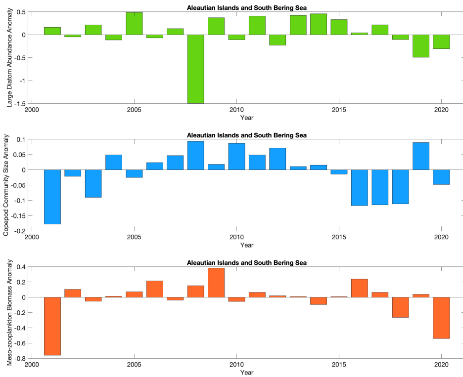
Figure 22: Annual anomalies of three indices of lower trophic levels from CPR data (from top to bottom): Large diatom abundance, copepod community size and meso-zooplankton biomass (see text for description and derivation) for region shown in Figure 21.
