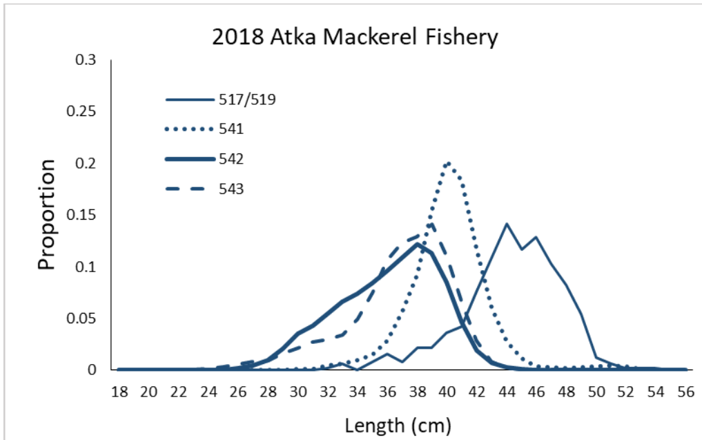
Figure 17.2. 2018 Atka mackerel fishery length-frequency data by area fished (see Figure 17.1). Numbers refer to management areas.
