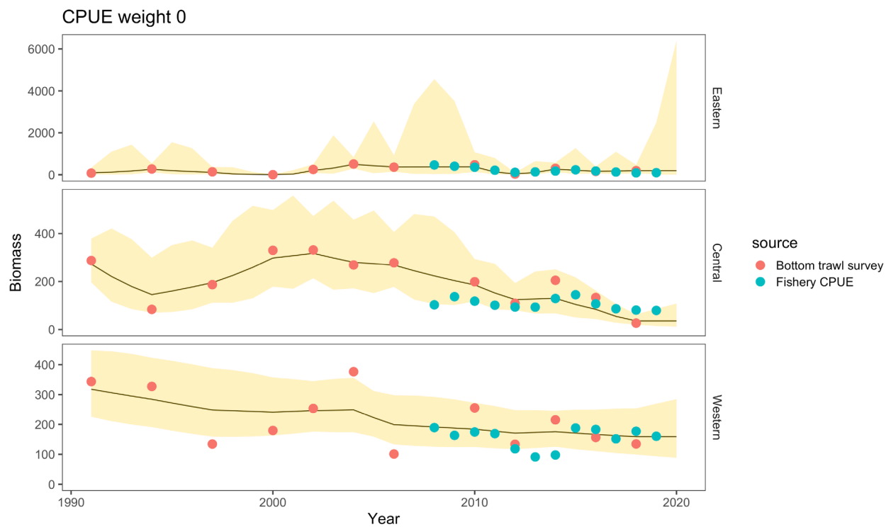
Figure 17C-4. Atka mackerel area-apportionment results fit with the random-effects model with proportions by region over time (top) and fit to both survey and nominal fishery CPUE data (with the western data from 2011-2014 downweighted). In this case, the weight is given to only the bottom trawl survey data for illustration purposes.
