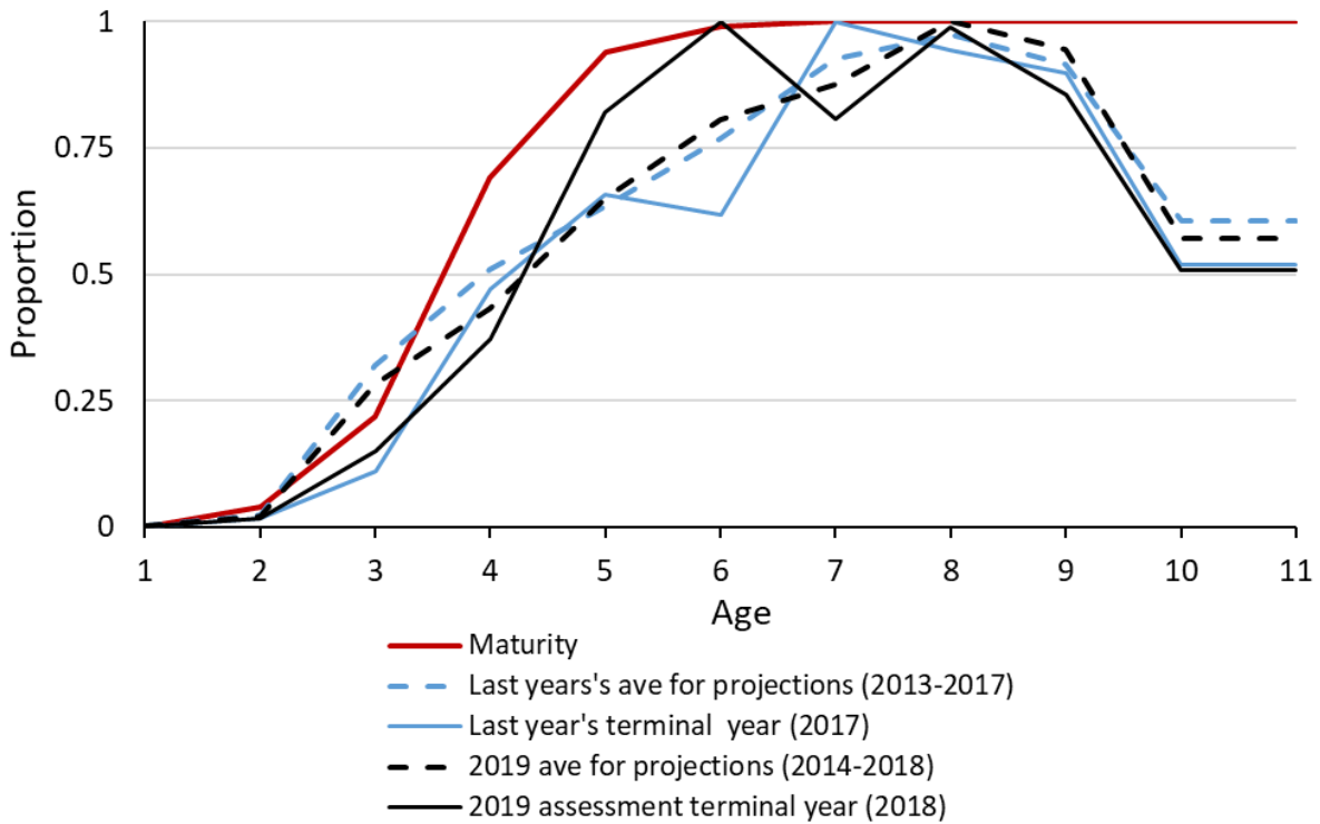
Figure 17.14. Estimated fishery selectivity patterns in the current assessment with a) last year's average for projections (2013-2017), b) the 2019 assessment average selectivity used for projections (2014-2018), c) last year's assessment terminal year (2017), and d) the 2019 assessment terminal year (2018) compared with the maturity-at-age estimates for BSAI Atka mackerel.
