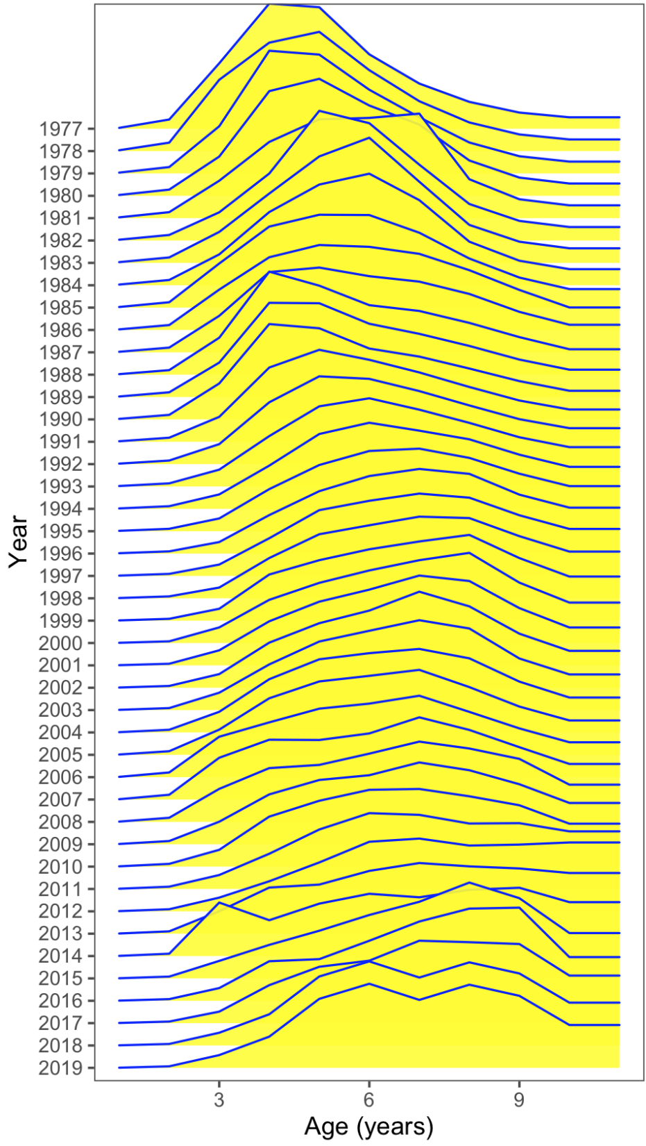
Figure 17.13. Fishery selectivity estimates over time for BSAI Atka mackerel.
