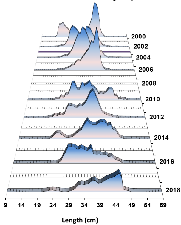
Figure 17.7. Atka mackerel bottom trawl survey length frequency data by subarea in 2018 (top) and for all areas, 2000-2018 (bottom). Vertical scales are proportional for a given area or year.
