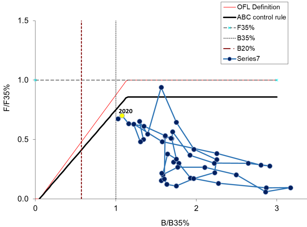
Figure 17.20. Aleutian Islands Atka mackerel spawning biomass relative to B_{35\%} and fishing mortality relative to F_{OFL} (1977-2021). The ratio of fishing mortality to F_{OFL} is calculated using the estimated selectivity pattern in that year. Estimates of spawning biomass and B_{35\%} are based on current estimates of weight-at-age and mean recruitment. Because these estimates change as new data become available, this figure can only be used in a general way to evaluate management performance relative to biomass and fishing mortality reference levels.
