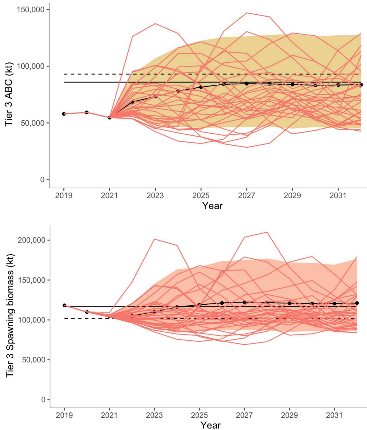
Figure 17.19. Projected Atka mackerel catch (assuming TAC taken in 2019 and reduced catches in 2020 and 2021; top) and spawning biomass (bottom) in thousands of metric tons under maximum permissible harvest control rule specifications after 2021. The individual thin lines represent samples of simulated trajectories.
