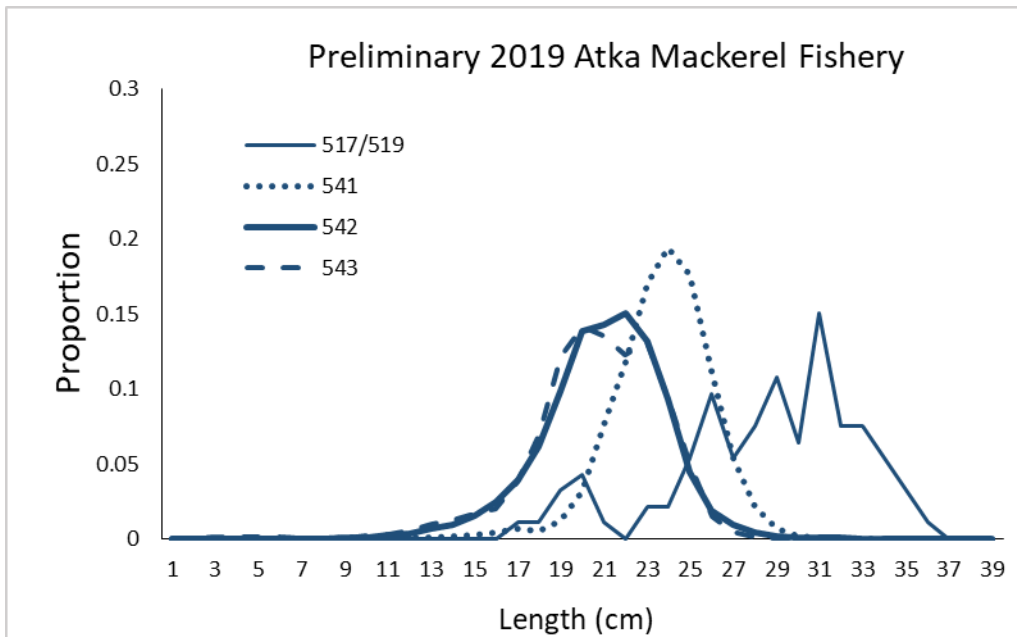
Figure 17.3. Preliminary 2019 Atka mackerel fishery length-frequency data by area fished (see Figure 17.1). Numbers refer to management areas.
