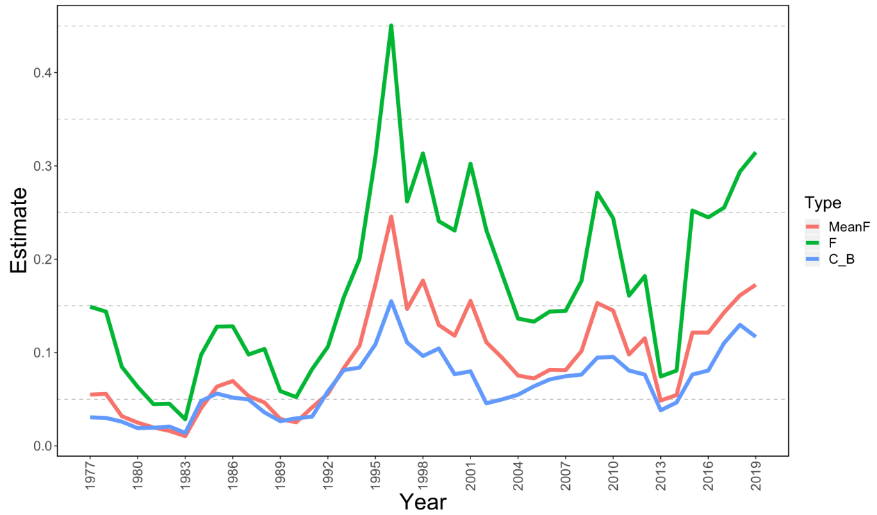
Figure 17.18 Estimated time series of Model 16.0 mean and full-selection fishing mortality and catch/biomass (C_B) exploitation rates of Atka mackerel, 1977-2019. Catch/biomass rates are the ratios of catch to beginning year age 3+ biomass.
