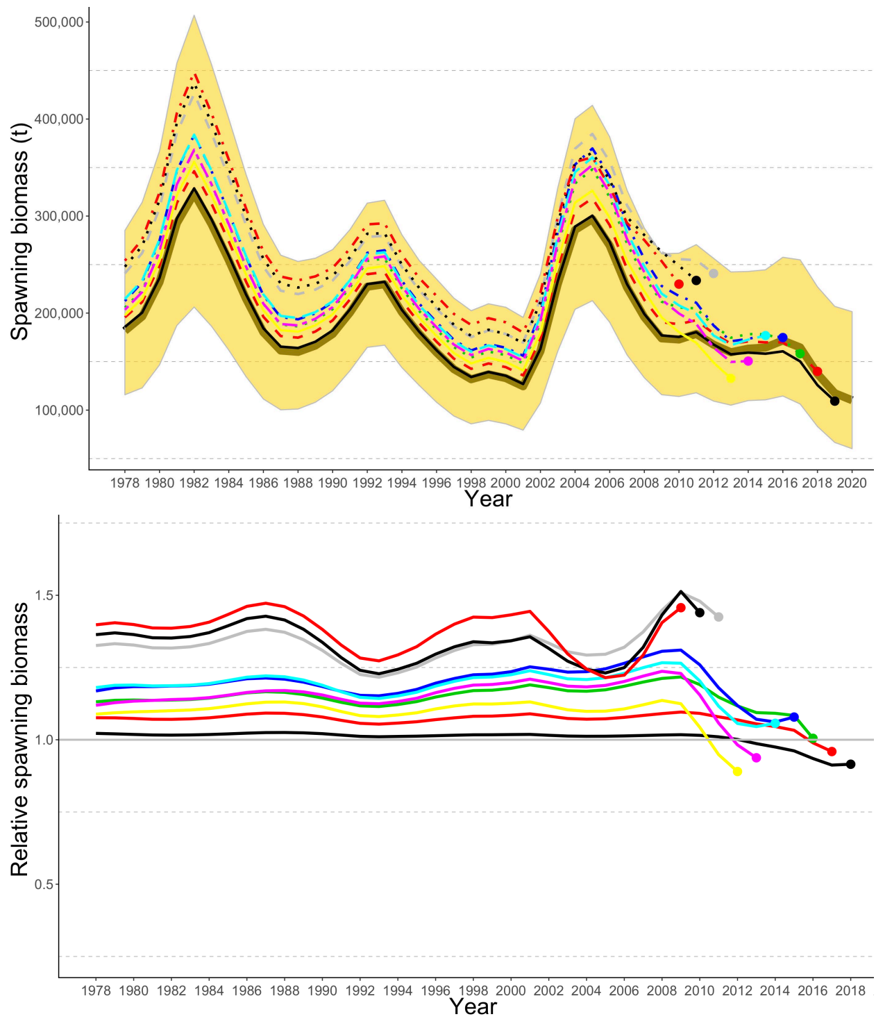
Figure 17.9. Retrospective plots showing the BSAI Atka mackerel spawning biomass over time (top) and the relative difference (bottom) over 10 different “peels”. Mohn’s rho was 0.08.
