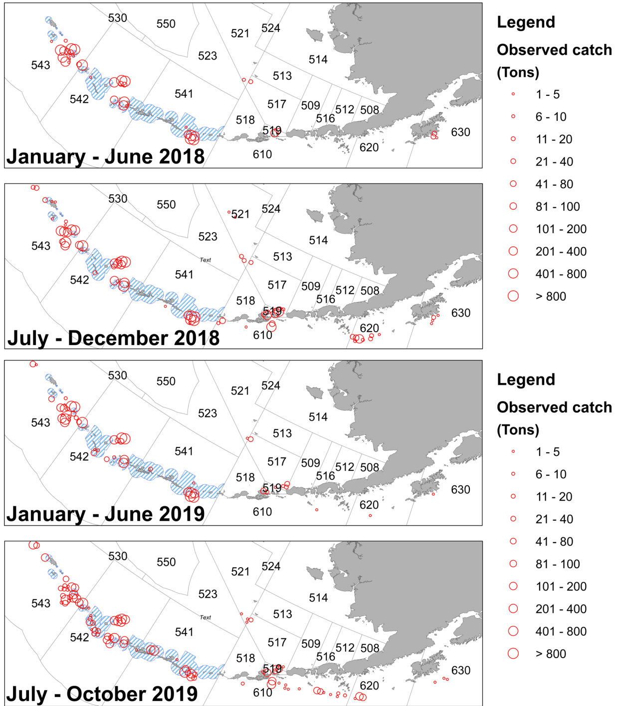
Figure 17.1. Observed catches of Atka mackerel summed for 20 km 2 cells for 2018 and 2019 where observed catch per haul was greater than 1 t. Shaded areas represent areas closed to directed Atka mackerel fishing.
