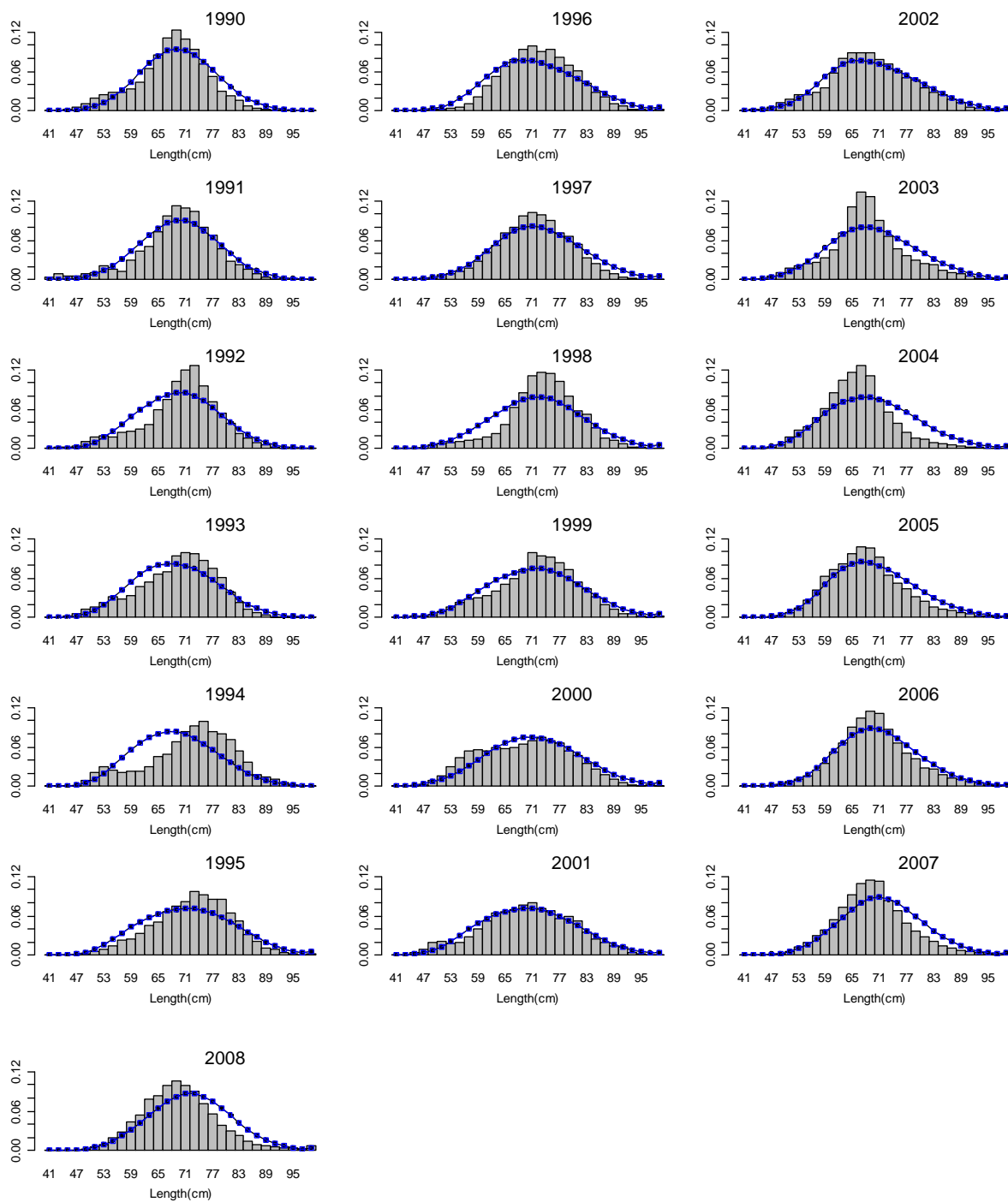
Figure 3.14. Domestic fixed gear fishery lengths compositions for females. Bars are observed frequencies and line is predicted frequencies.
