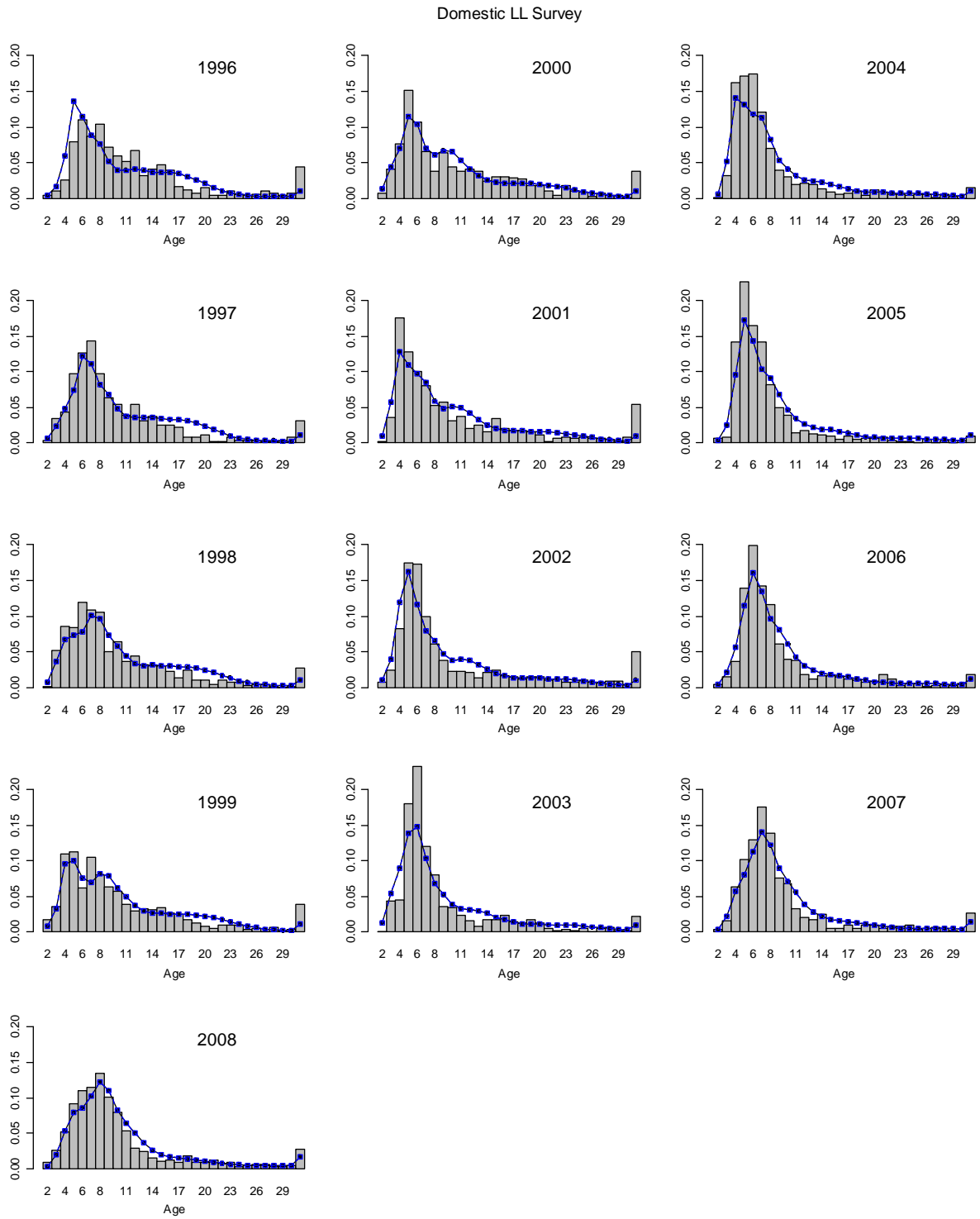
Figure 3.16. Domestic longline survey age compositions. Bars are observed frequencies and line is predicted frequencies.
