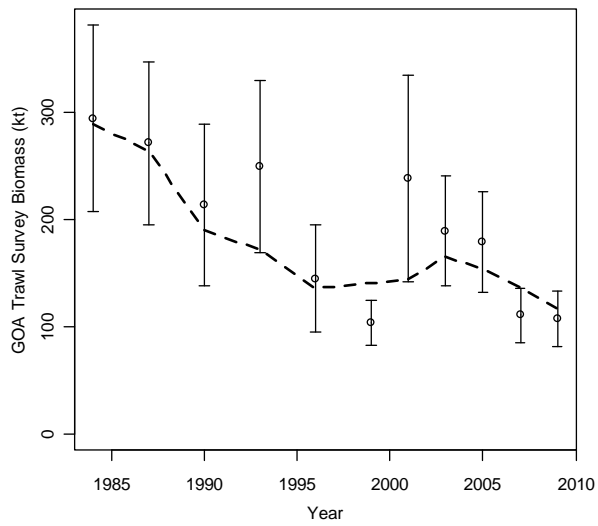
Figure 3.3. Observed and predicted sablefish abundance indices. Fishery indices are on top two panels, GOA trawl survey is on the bottom left panel. Points are observed estimates with approximate 95% confidence intervals while dashed lines are model predictions.
