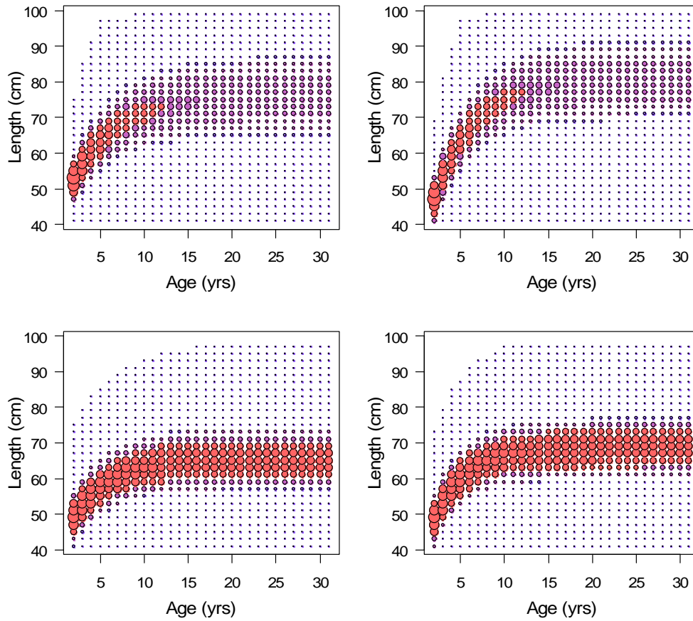
Figure 3.8. Age-length conversion matrices for sablefish. Top panels are female, bottom panels are males, left is 1981-1993, right is 1996-2004.
