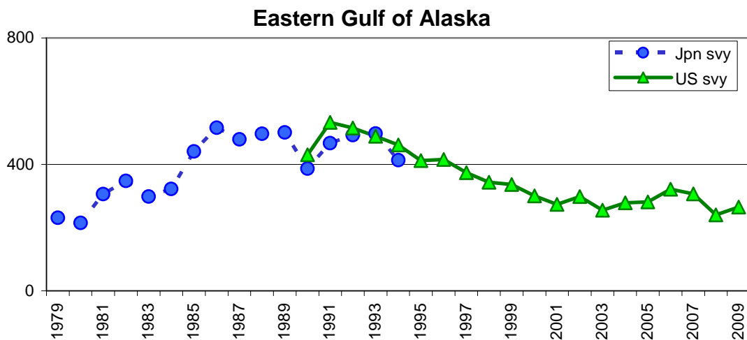
Figure 3.6. Relative abundance (weight) by region and survey. The regions Bering Sea, Aleutians Islands, and western Gulf of Alaska are combined in the first plot. The two surveys are the Japan-U.S. cooperative longline survey and the domestic (U.S.) longline survey. In this plot, the values for the U.S. survey were adjusted to account for the higher efficiency of the U.S. survey gear.
