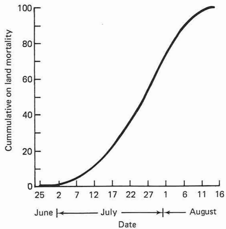
Figure 11.--Cumulative percentage of dead fur seal pups found on study areas on St. Paul Island, Alaska, 25 June-15 August 1954 (Kenyon et al. 1954).
