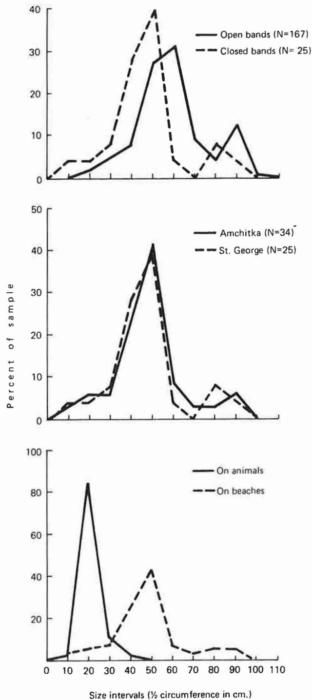
Figure 10.--Frequency distributions of plastic banding materials found on two islands in the vicinity of the Bering Sea and those found on entangled animals taken in the harvest in 1982 on St. Paul Island. Top panel: comparison of open and closed pieces on St. George Island. Middle panel: comparison of closed loops for two islands. Bottom panel: comparison of closed loop material (both islands) with those found on entangled animals.
