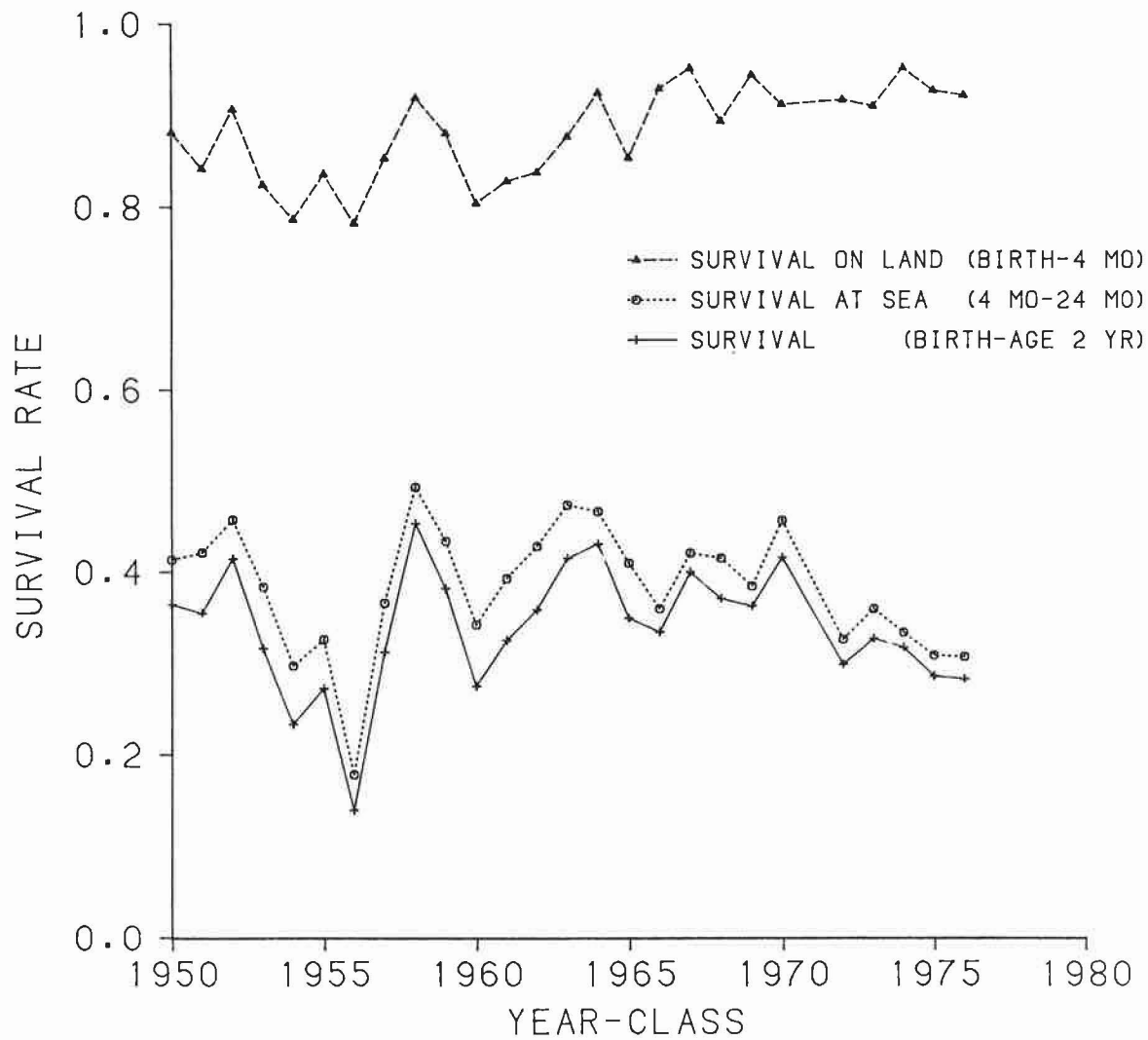
Figure 15.--Survival on land (birth - age 4 mo), survival at sea (age 4 mo-2 yr), and total survival (birth-2 yr) for male northern fur seals of the 1950-76 year classes of St. Paul Island, Alaska.
