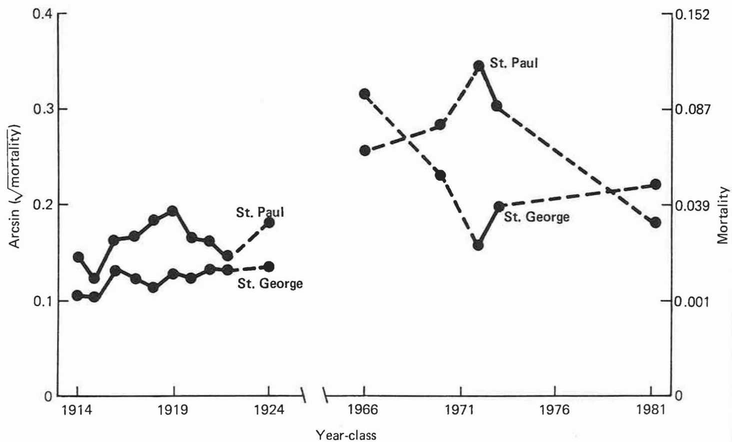
Figure 14.--Comparison of fur seal pup mortality on land for St. Paul and St. George Islands.
