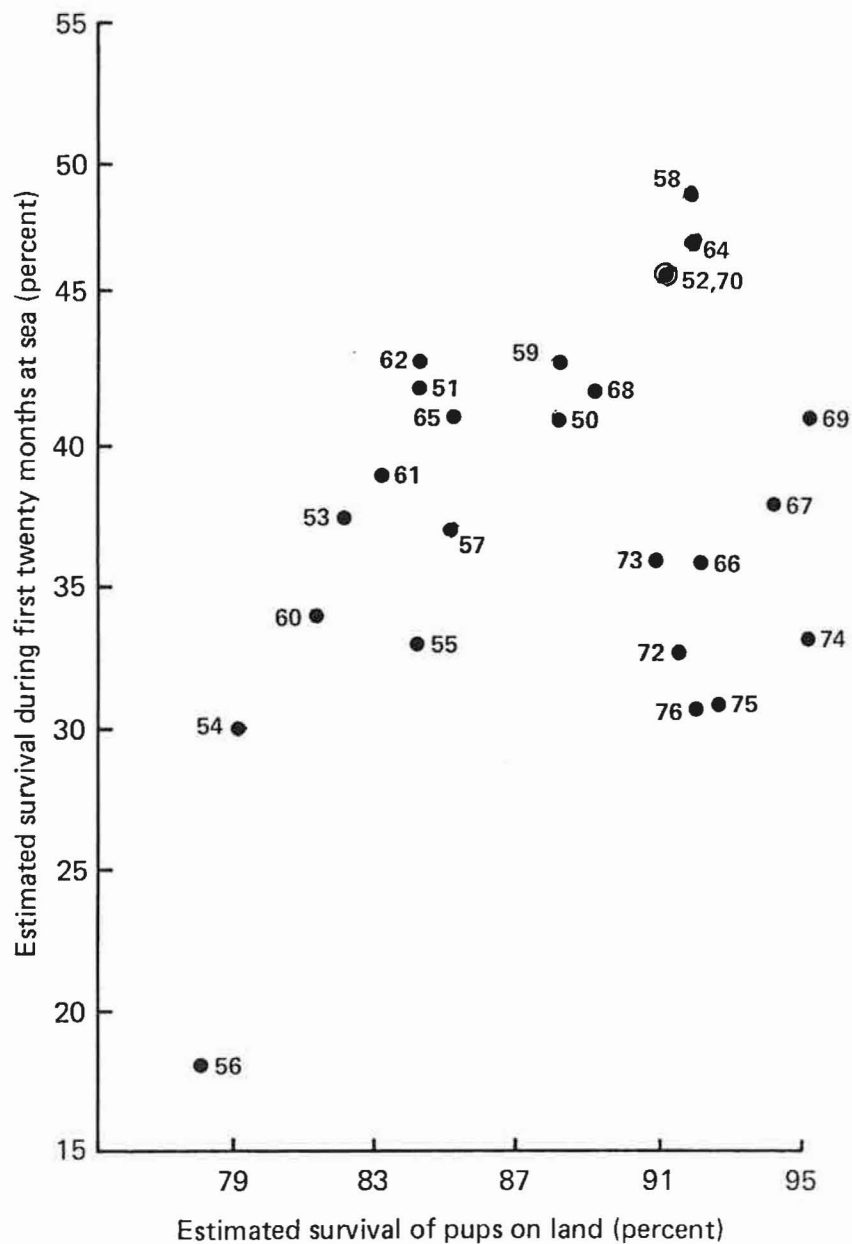
Figure 16.--Survival at sea (age 4 mo-age 24 mo) versus survival on land (birth-age 4 mo) for male northern fur seals of the 1950-76 year classes of St. Paul Island, Alaska.
