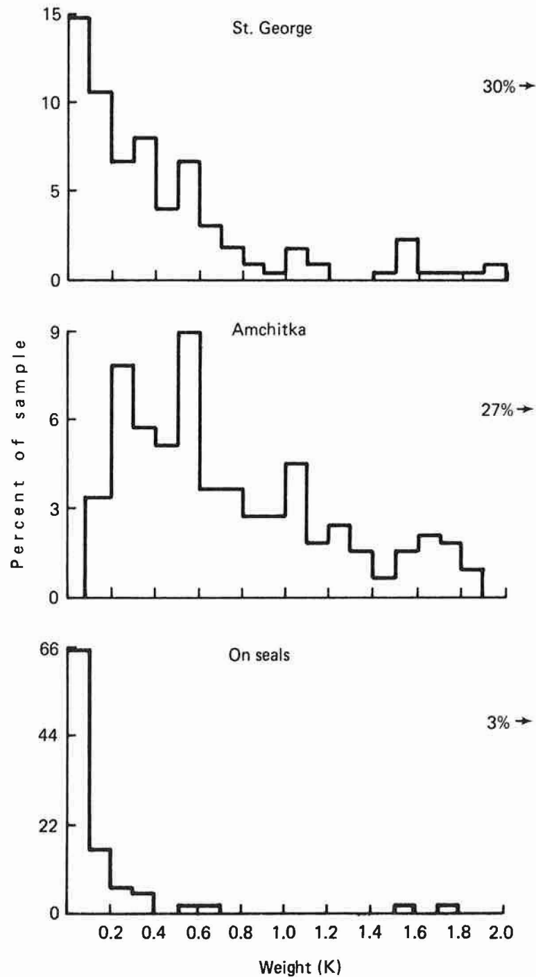
Figure 8.-- A comparison of the size frequency distribution of net fragments (based on weight) found in 1982 on two islands (St. George and Amchitka) in the vicinity of the Bering Sea with that on fur seals taken in the 1982 harvest on St. Paul Island (on seals).
