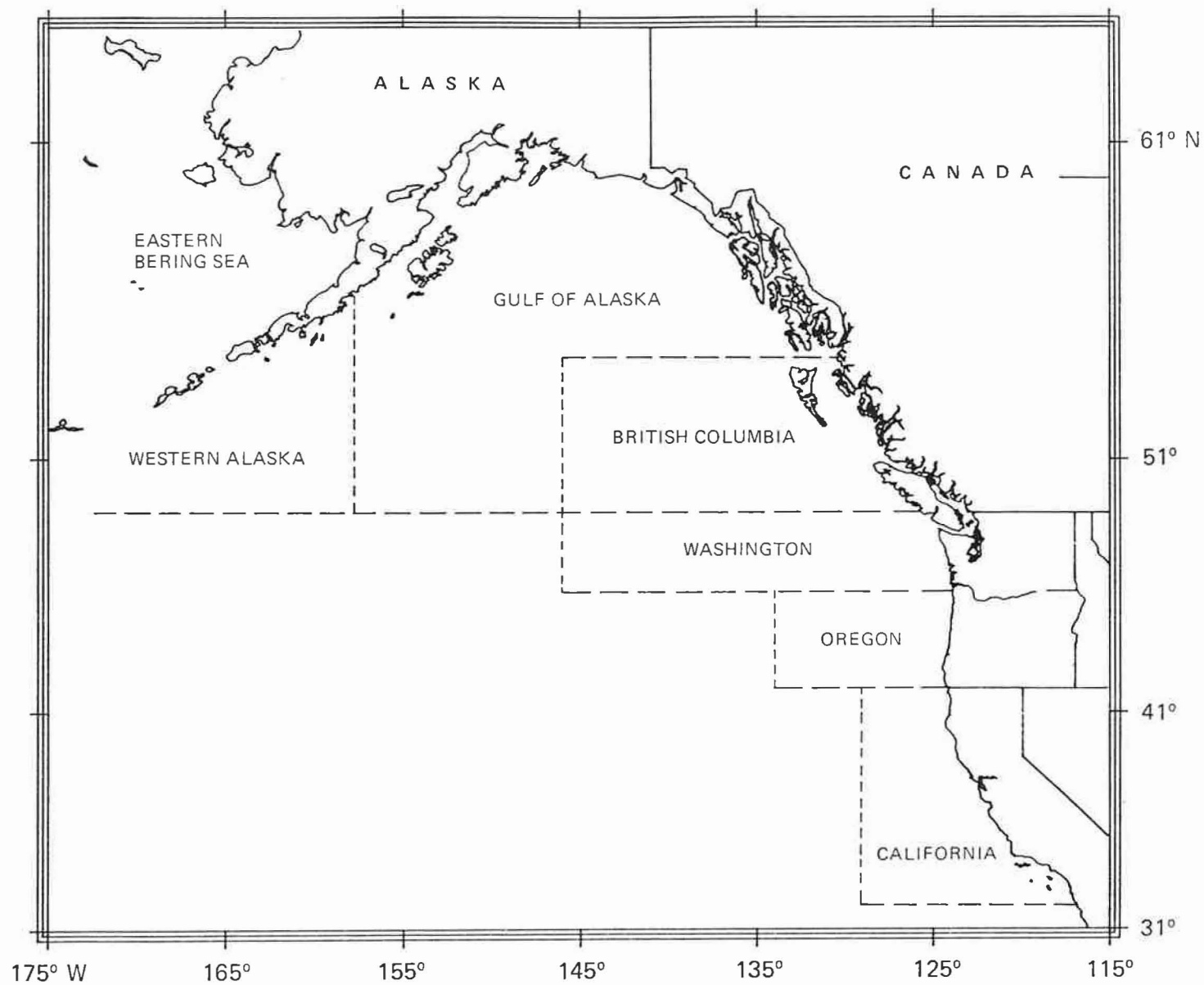
Figure 19.--The collection areas of northern fur seals, 1958-74.
