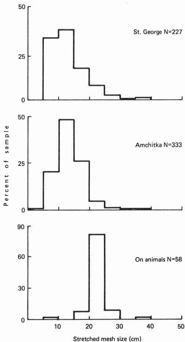
Figure 9.--A comparison of the frequency distribution of mesh sizes for net fragments found in 1982 on two islands (St. George and Amchitka) in the vicinity of the Bering Sea with that found on animals taken in the 1982 harvest on St. Paul Island.
