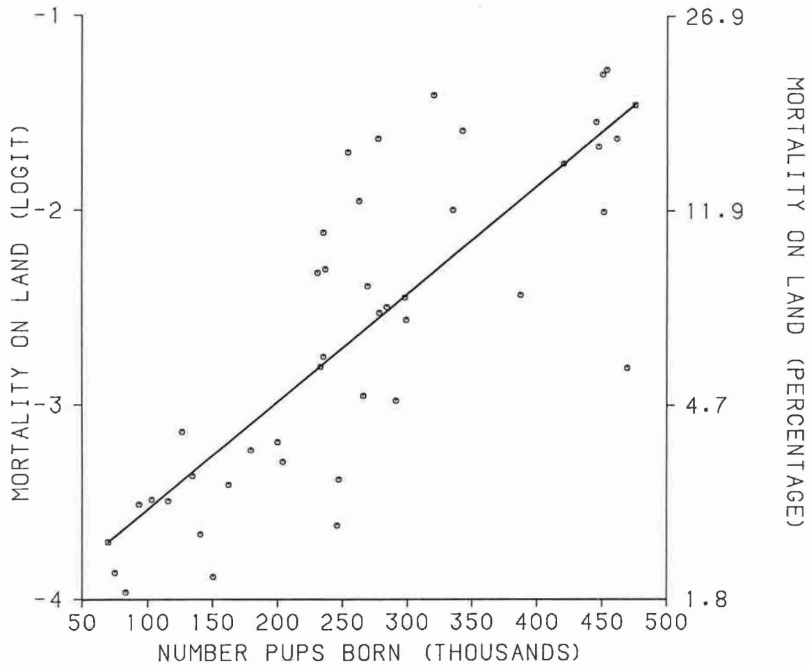
Figure 13.--Mortality on land versus numbers of pups born for all available year classes 1914-82, St. Paul Island, Alaska.
