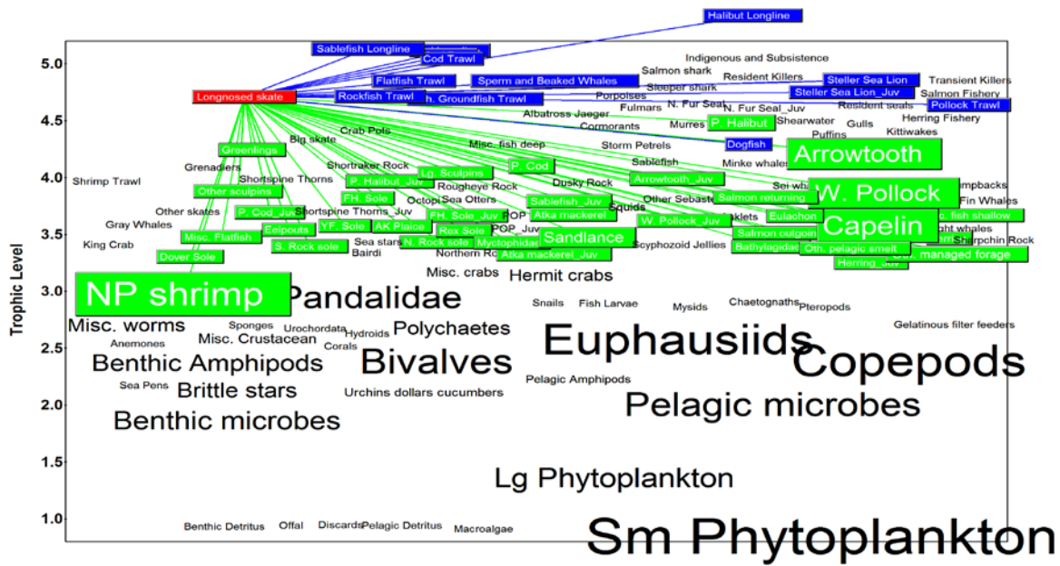
Figure 22. Food web for longnose skates in the GOA. (Source: K. Aydin, AFSC, code available upon request.)
