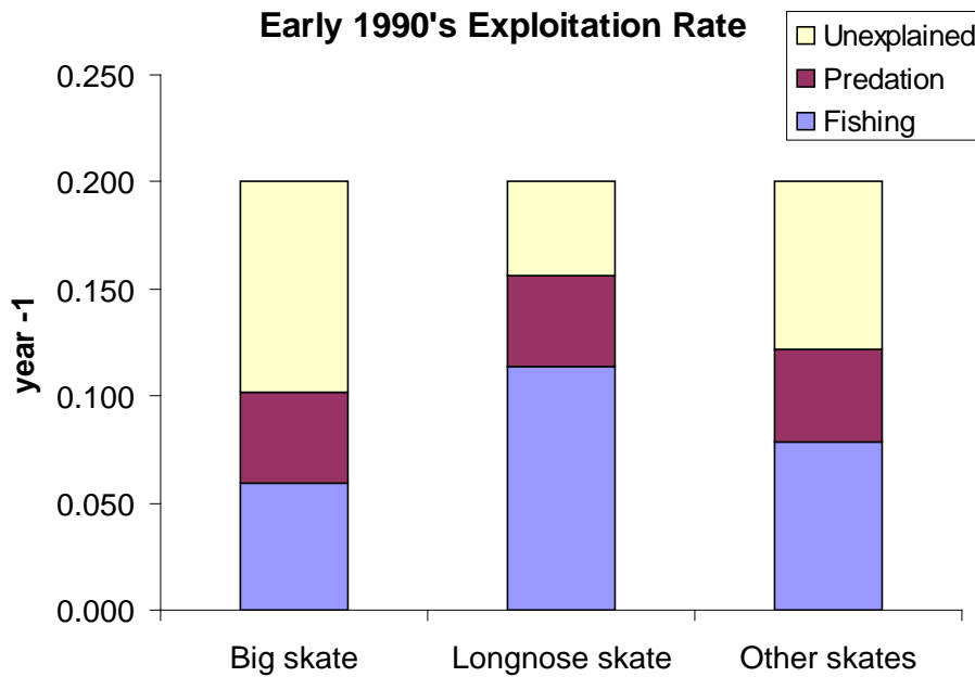
Figure 24. Mortality rates from predation and fishing for Other skates, longnose skates, and big skates in the GOA (early 1990s prior to target fishery developing for big skates). Total mortality (fishing + predation + unexplained) is assumed to equal the production rate for skate populations at equilibrium (here, 0.2 as approximated from Frisk et al. 2001). Total mortality is apportioned between estimates of predation mortality (from AFSC ecosystem modeling) and fishing mortality (exploitation rate: catch/biomass), and the remaining fraction of mortality is attributed to unknown sources.
