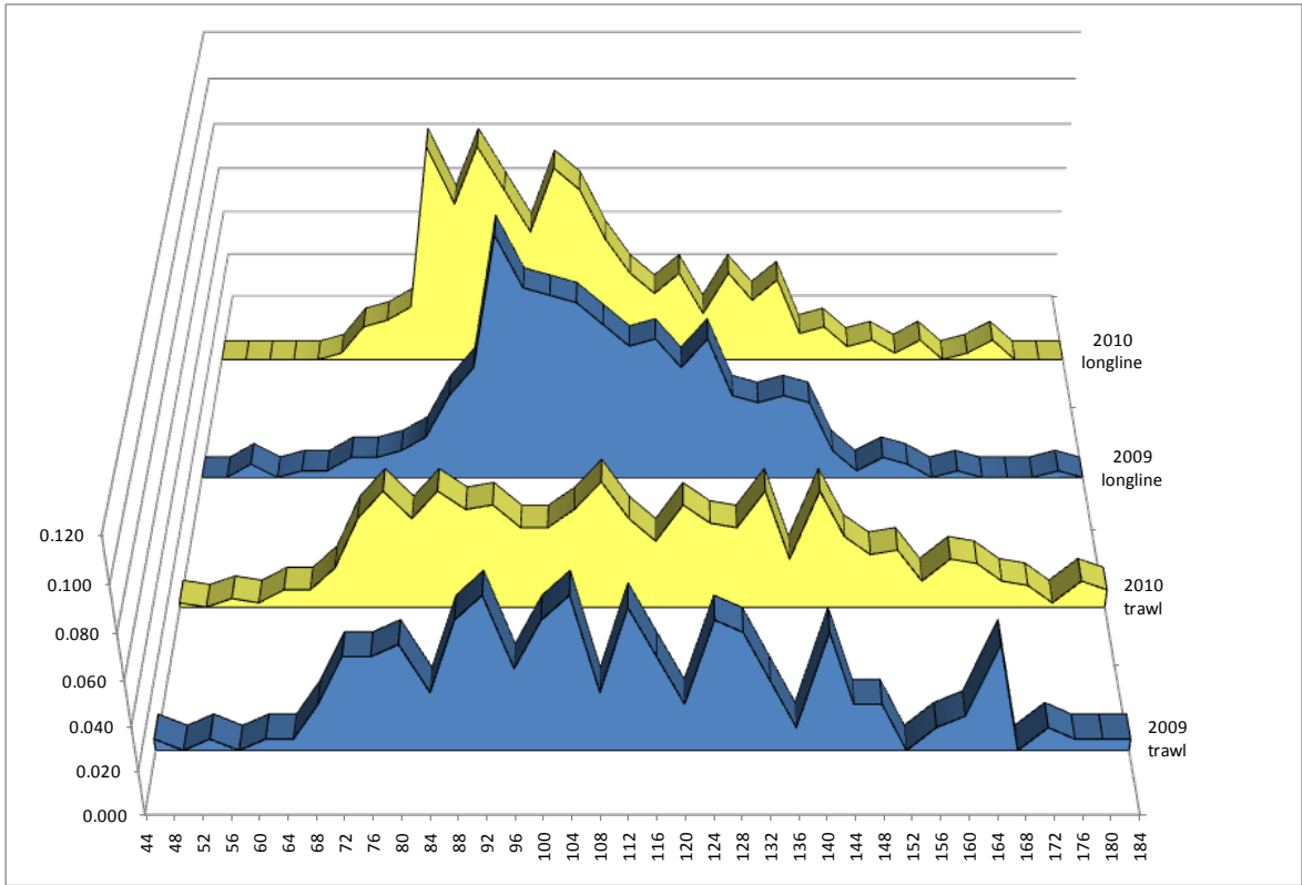
Figure 19a. Length compositions of fishery catches for big skates in 2009 and 2010.
