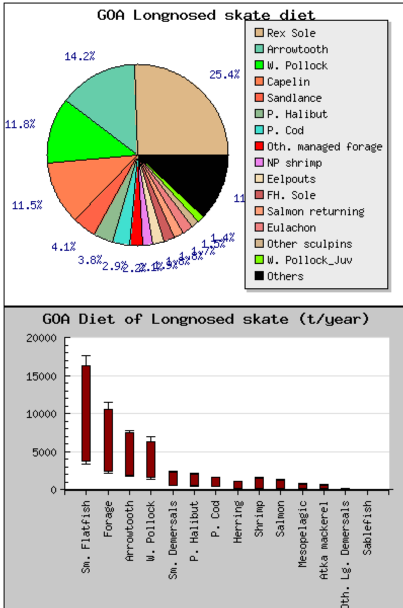
Figure 29. Diet composition and consumption of prey by longnose skates in the GOA. Results were generated from stomach content collections occurring during RACE trawl surveys.
