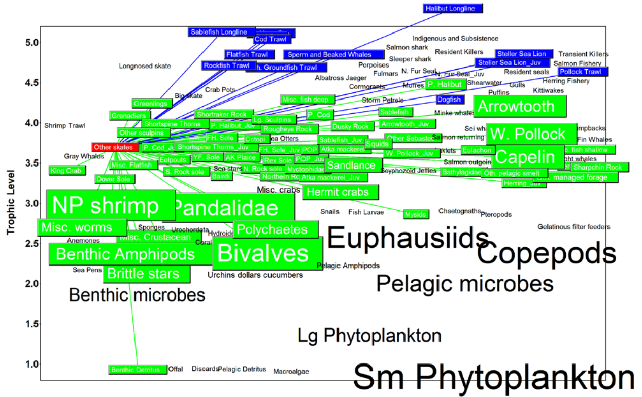
Figure 23. Food web for Other skates in the GOA. (Source: K. Aydin, AFSC, code available upon request.)
