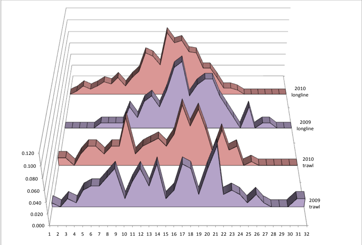
Figure 19b. Length compositions of fishery catches for longnose skates in 2009 and 2010.
