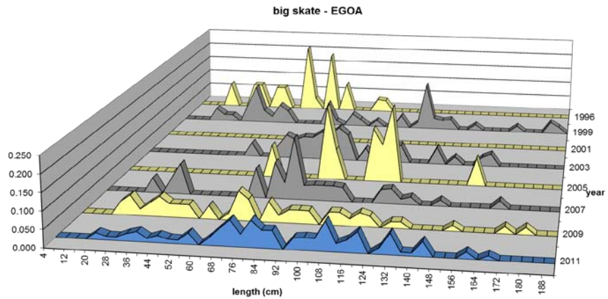
Figure 16. Big skate trawl survey length composition by regulatory area, 1996-2011. The most recent data (2011) are shown in blue.
