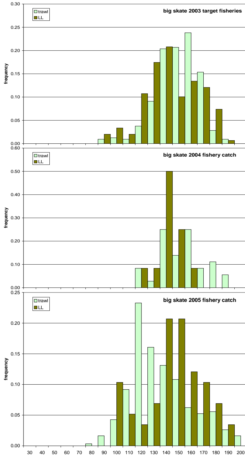
Figure 18. Big skate fishery length compositions, 2003-2005. LL = longline. 2003 N : trawl 319, LL 149; 2004 N : trawl 36, LL 12; 2005 N : trawl 305, LL 58.
