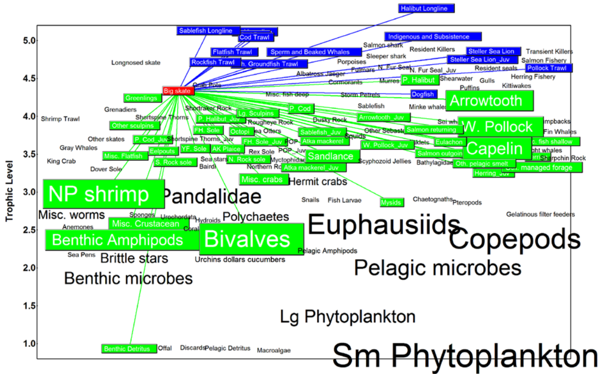
Figure 21. Food web for big skates in the GOA. (Source: K. Aydin, AFSC, code available upon request.)
