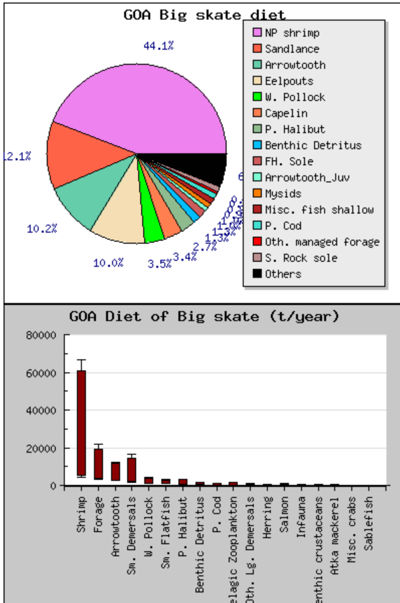
Figure 28. Diet composition and consumption of prey by big skates in the GOA. Results were generated from stomach content collections occurring during RACE trawl surveys.
