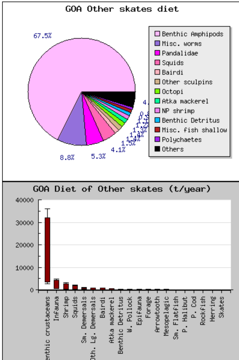
Figure 30. Diet composition and consumption of prey by Other skates in the GOA. Results were generated from stomach content collections occurring during RACE trawl surveys.
