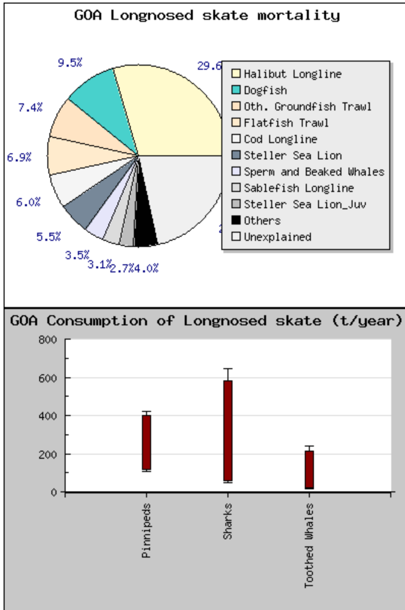
Figure 26. Mortality and consumption of longnose skates in the GOA. Model outputs were derived from diet compositions, production rates, and consumption rates of skate predators, and from skate catch data.
