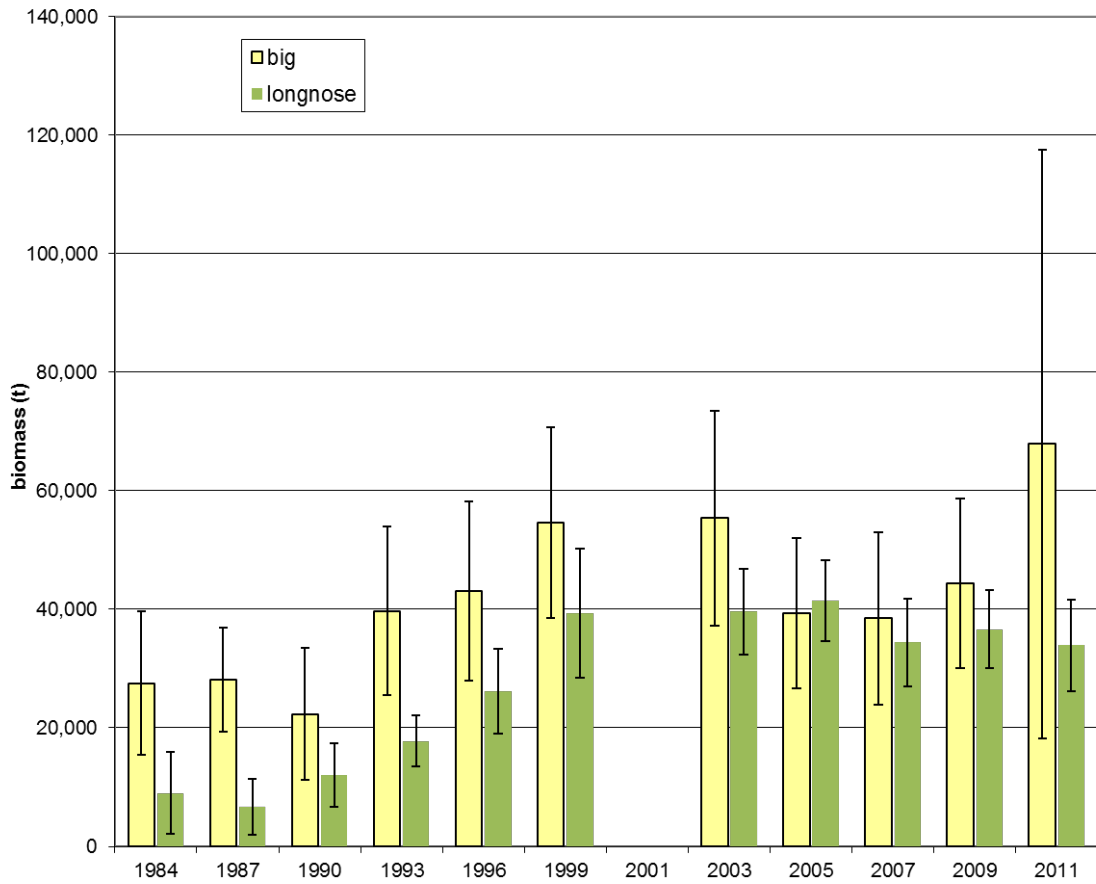
Figure 10. NMFS GOA bottom trawl survey biomass trends for big and longnose skates, 1984-2011. Error bars show plus/minus 2 standard deviations. The 2001 survey did not sample in the EGOA and is not included in the time series.
