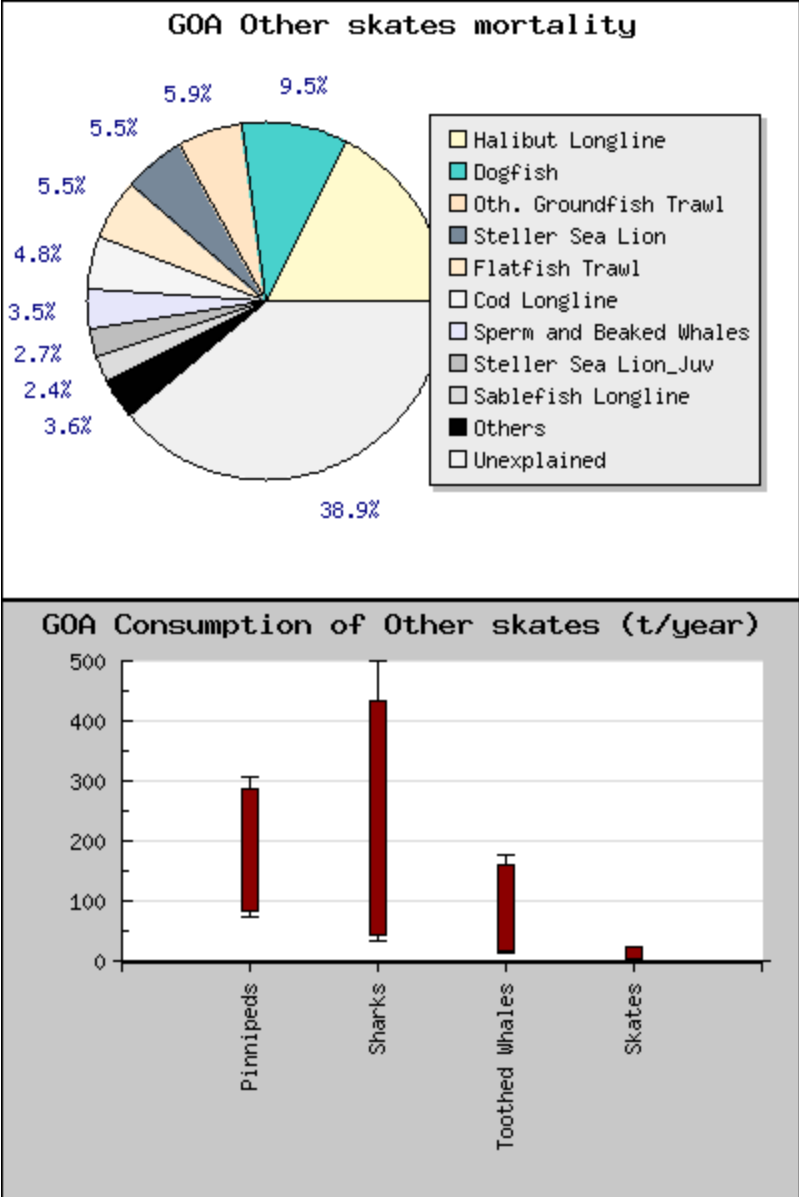
Figure 27. Mortality and consumption of Other skates in the GOA. Model outputs were derived from diet compositions, production rates, and consumption rates of skate predators, and from skate catch data.
