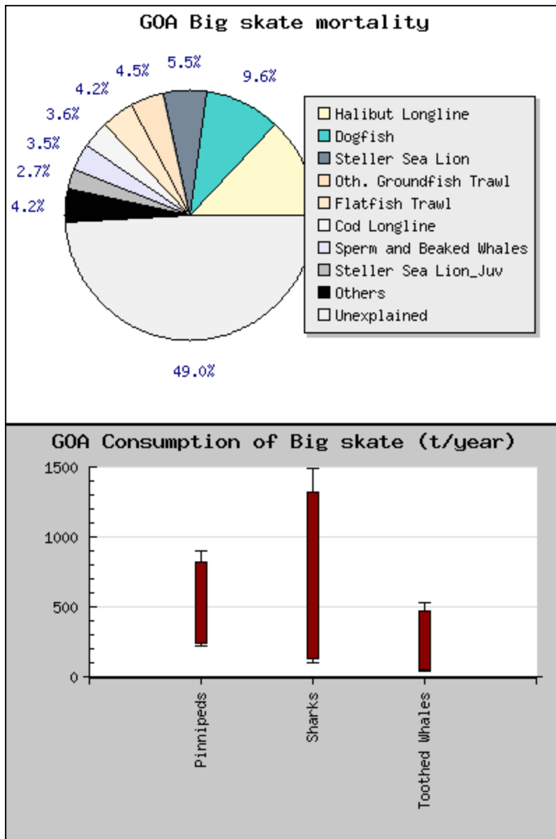
Figure 25. Mortality and consumption of big skates in the GOA. Model outputs were derived from diet compositions, production rates, and consumption rates of skate predators, and from skate catch data.
