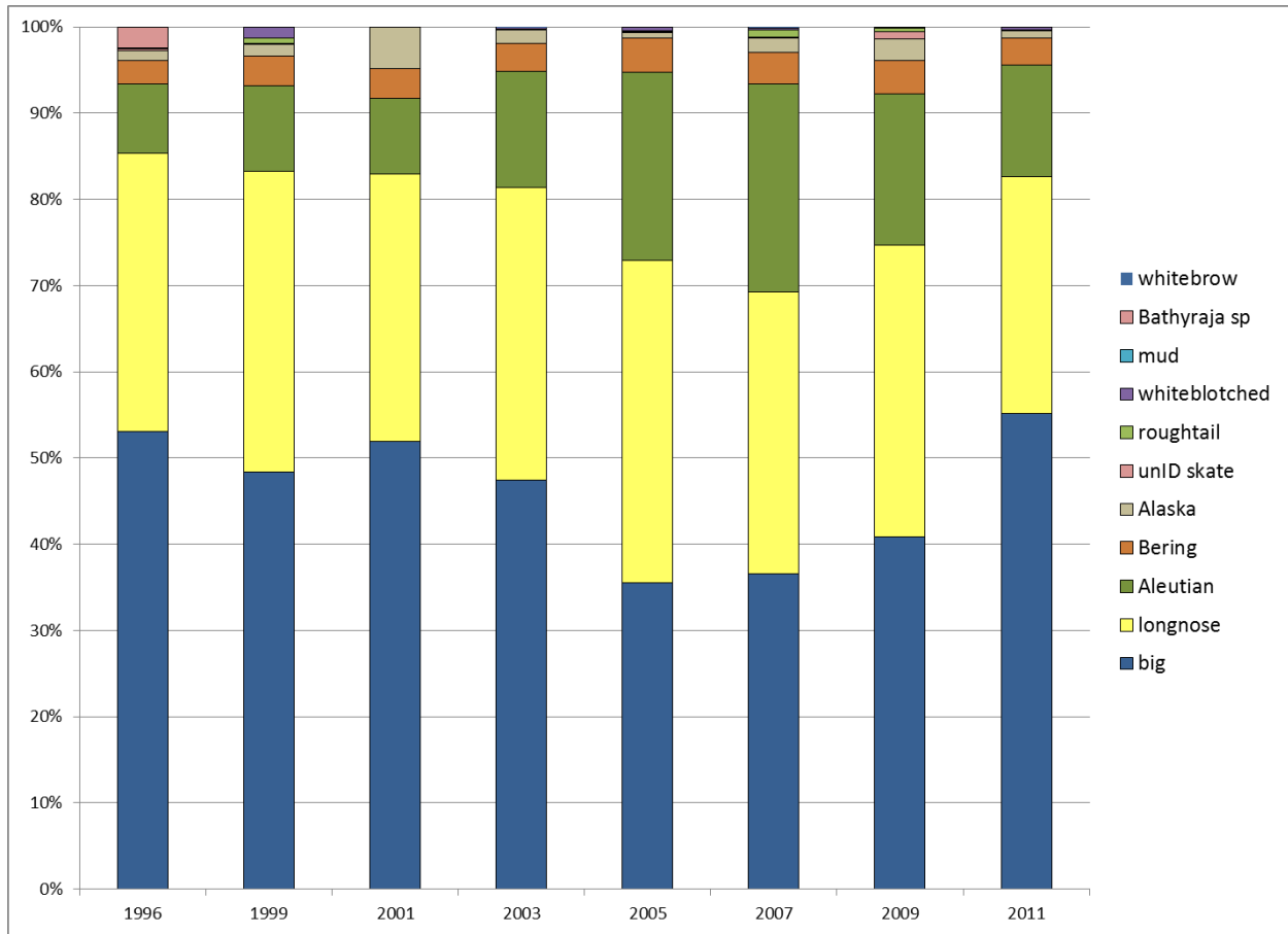
Figure 12. Gulfwide species composition of GOA skates, 1996-2011. The 2001 survey did not sample in the EGOA.
