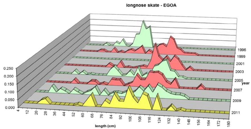
Figure 17. Longnose skate trawl survey length composition by regulatory area, 1996-2011. The most recent data (2011) are shown in yellow.
