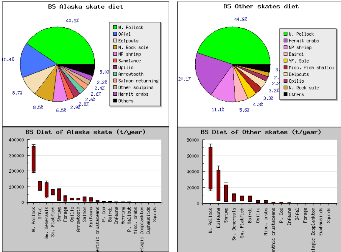
Figure 37. Diet composition (upper panels) and annual estimated prey consumption by skates (lower panels) for EBS Alaska skates (left panels) and Other Skates (right panels). Results were generated from stomach content collections occurring during RACE trawl surveys.
