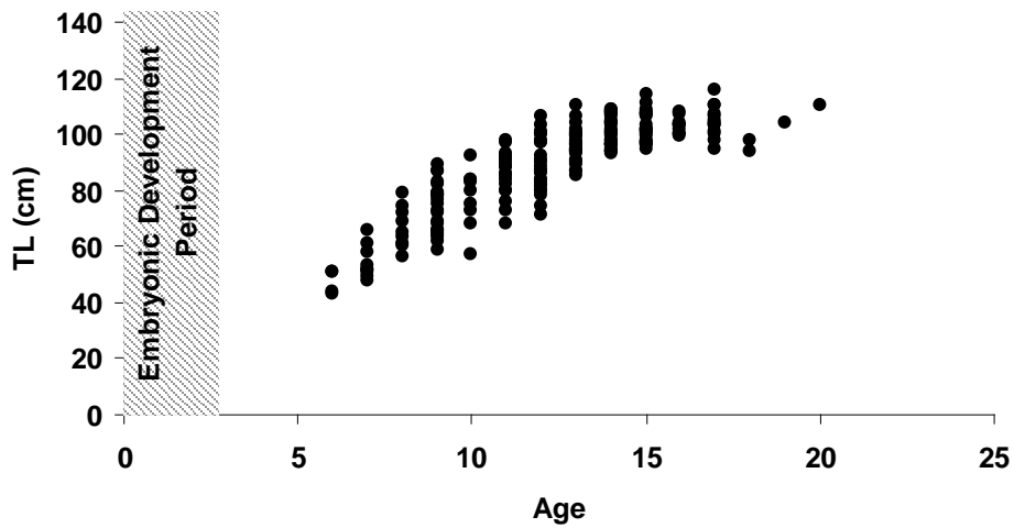
Figure 17. Observed size at age data from Alaska skates collected in the 2005 longline fishery, sexes combined (n=208). The three year embryonic development period included in the base model is represented by the shaded area.
