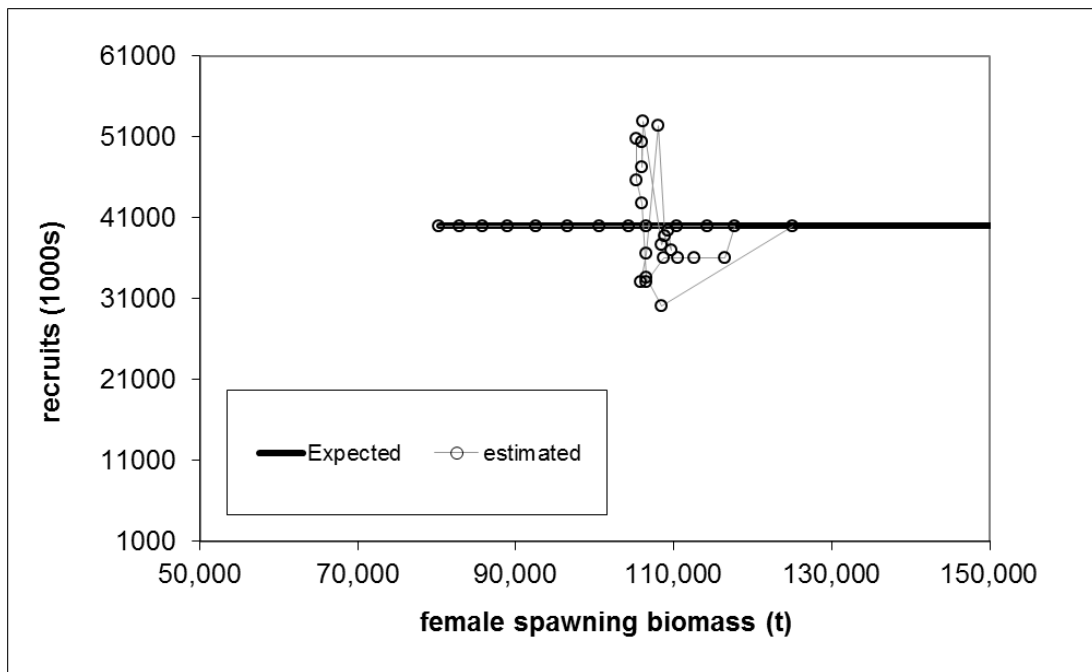
Figure 30. Relationship between female spawning biomass (t) and the number of age 0 recruits (in thousands of fish). Time series of individual year class estimates from SS2 is shown with a Beverton-Holt stock-recruit relationship with a steepness of 1.0.
