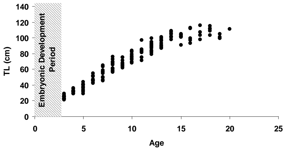
Figure 16. Observed size at age data from Alaska skates collected in the 2003 EBS shelf trawl survey, sexes combined (n=182). The three year embryonic development period included in the base model is represented by the shaded area.
