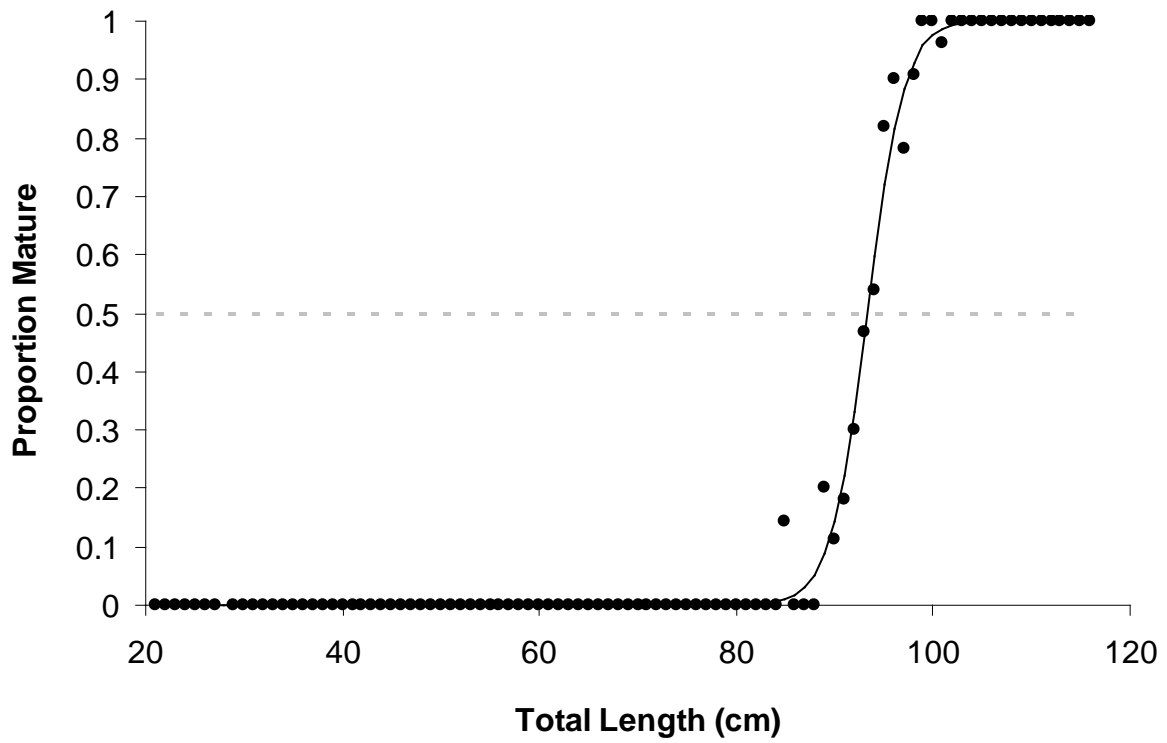
Figure 20. Female Alaska skate maturity-at-length data shown with fitted logistic curve from Matta (2006) (n=642).
