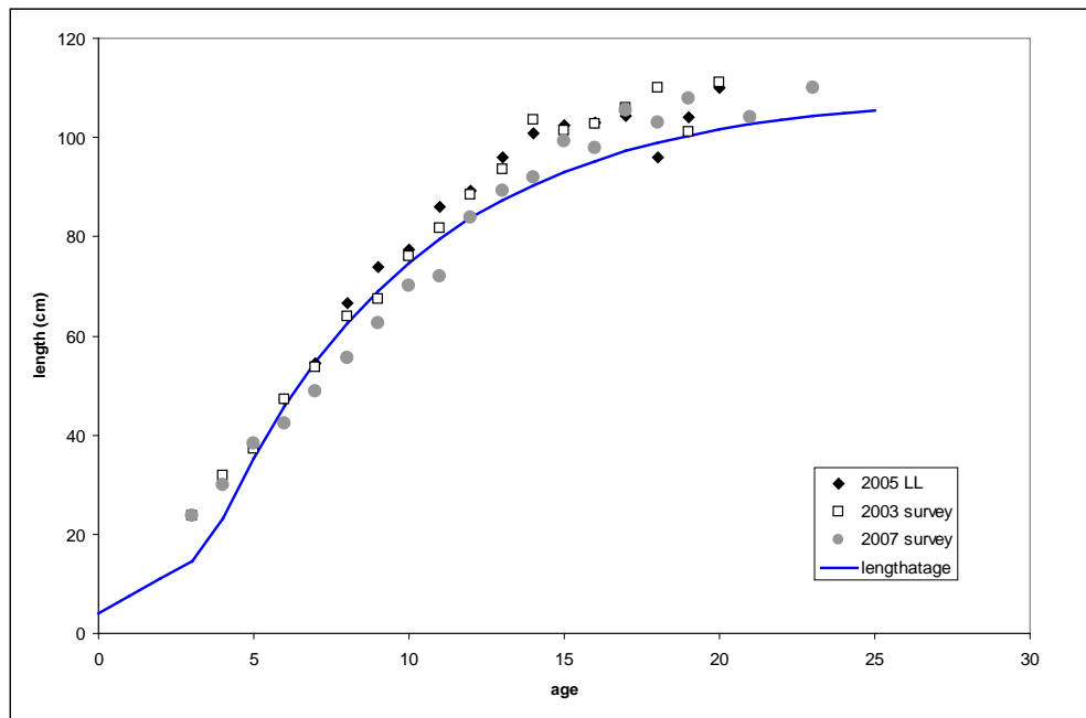
Figure 27. Observed length-at-age from the three datasets used in the model, with the population estimate of length-at-age (blue line) superimposed.
