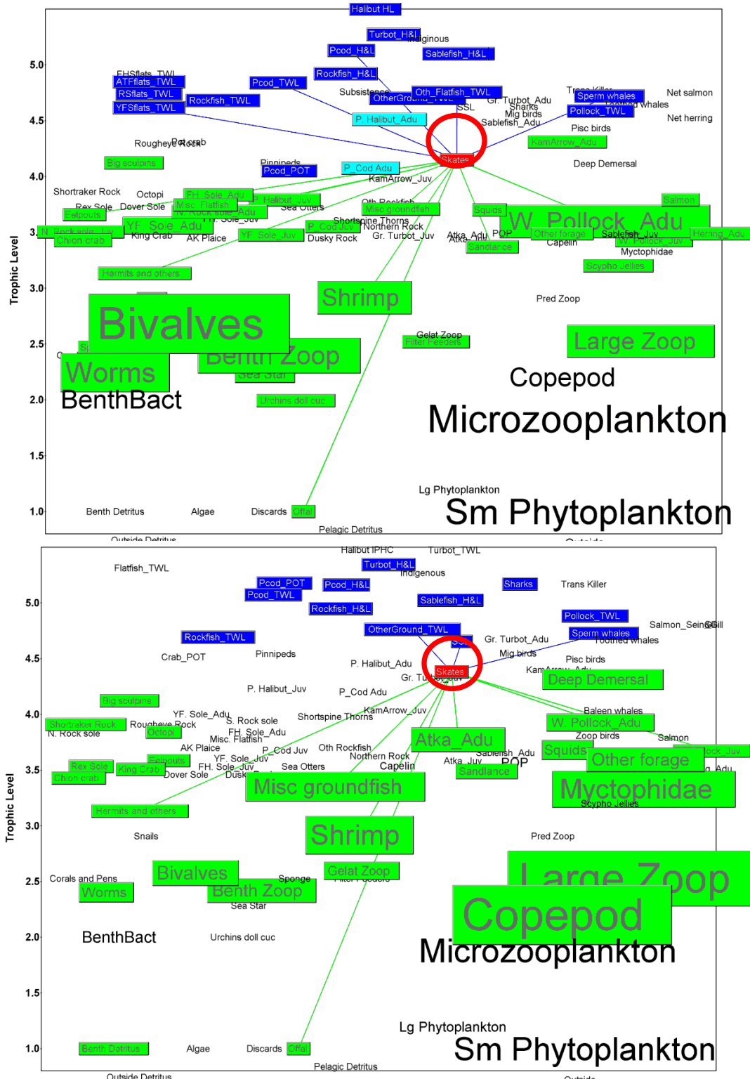
Figure 33. EBS (upper panel) and AI (lower panel) skate food webs derived from mass balance ecosystem models, with skate species aggregated in each area. (Source: K. Aydin, AFSC, code available upon request.)
