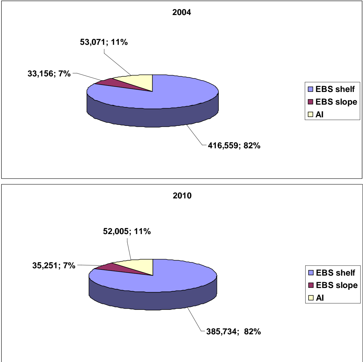
Figure 5. Distribution of skate biomass in the 3 subregions of the BSAI, 2004 and 2010. Data are biomass estimates from AFSC groundfish surveys.
