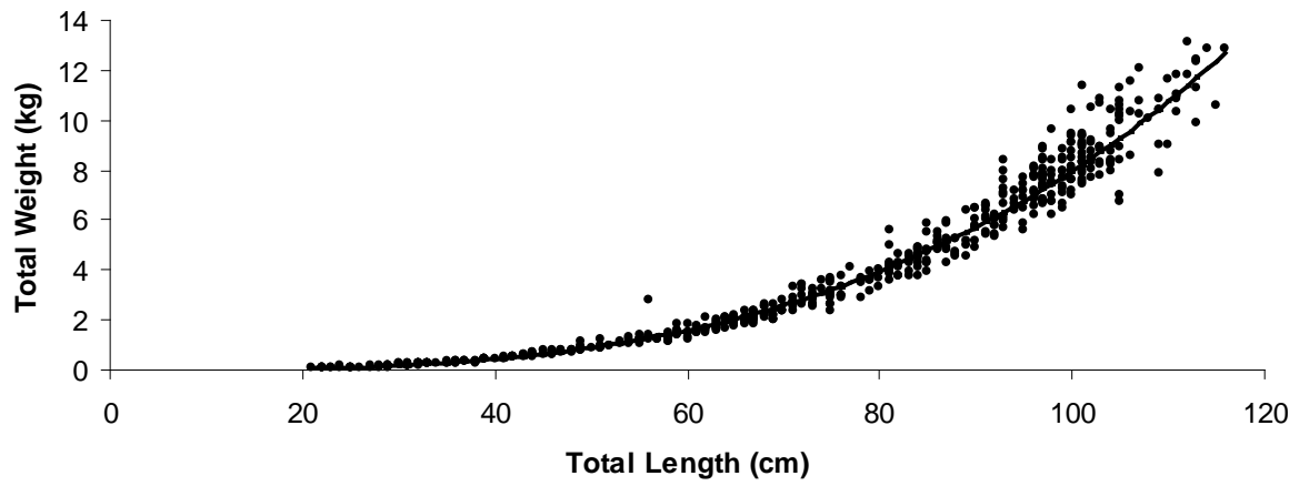
Figure 18. The relationship between total length (TL) and total body weight (W) for the Alaska skate, both sexes combined (n=526).
