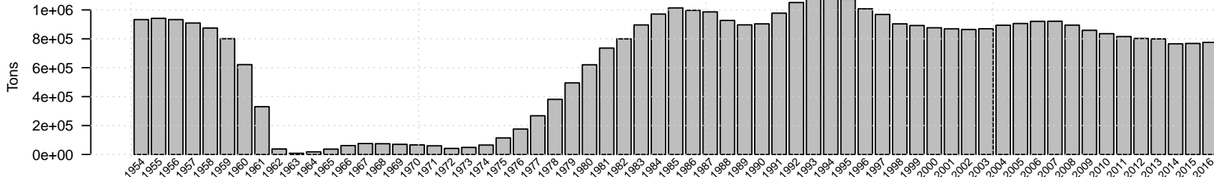
Bering Sea Aleutian Islands spawning biomass of Yellowfin sole
