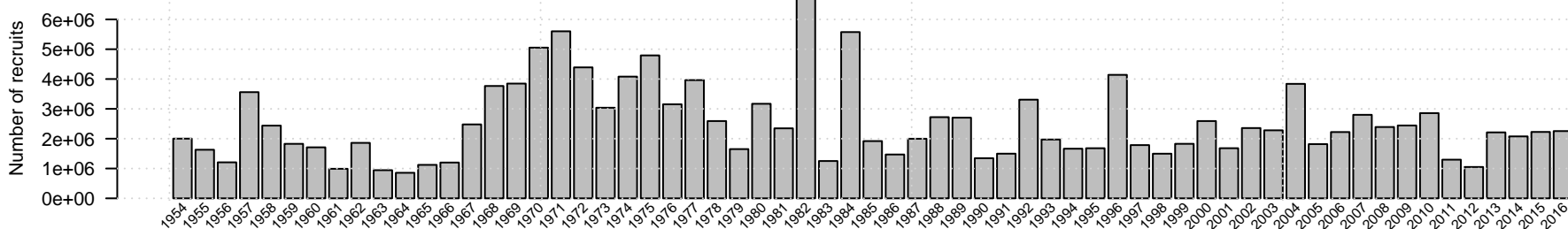
Bering Sea Aleutian Islands age 1 recruitment of Yellowfin sole
