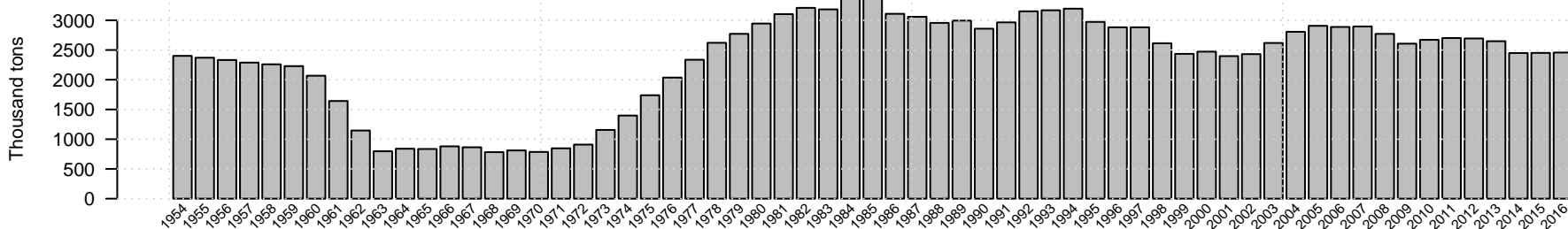
Bering Sea Aleutian Islands age 1 plus biomass of Yellowfin sole
