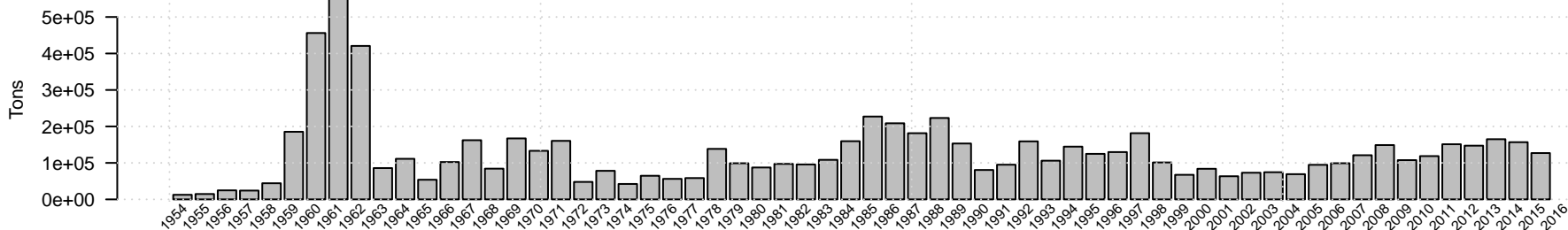
Bering Sea Aleutian Islands catch of Yellowfin sole
