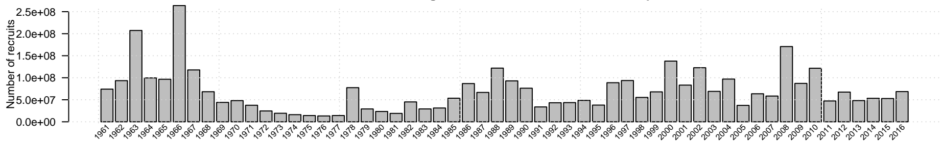
Gulf of Alaska age 2 recruitment of Pacific ocean perch
