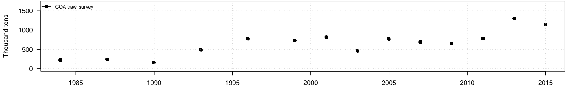
Gulf of Alaska survey biomass of Pacific ocean perch
