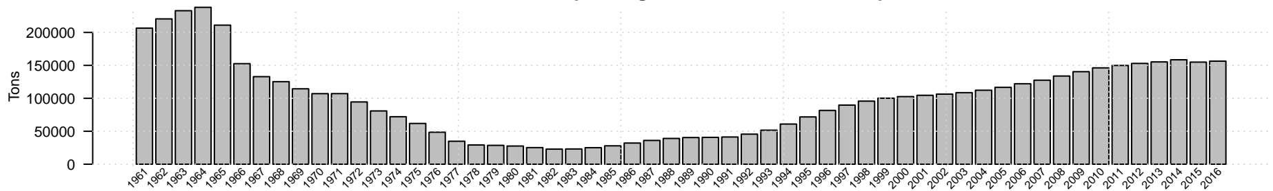
Gulf of Alaska spawning biomass of Pacific ocean perch
