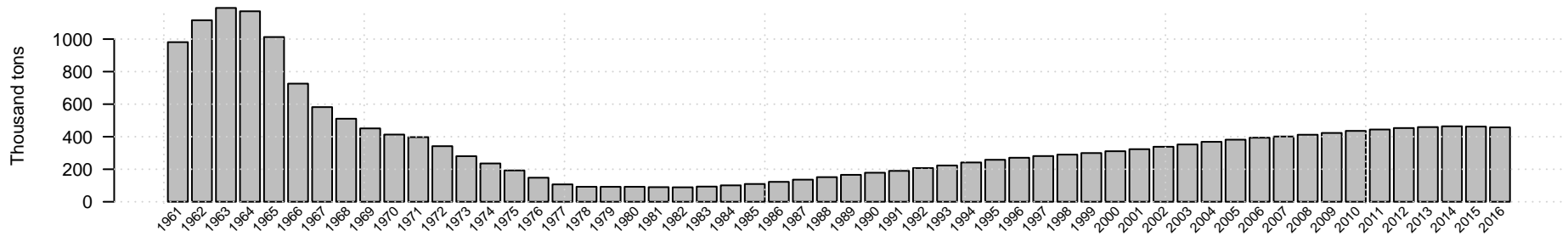
Gulf of Alaska age 2 plus biomass of Pacific ocean perch
