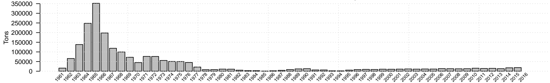
Gulf of Alaska catch of Pacific ocean perch
