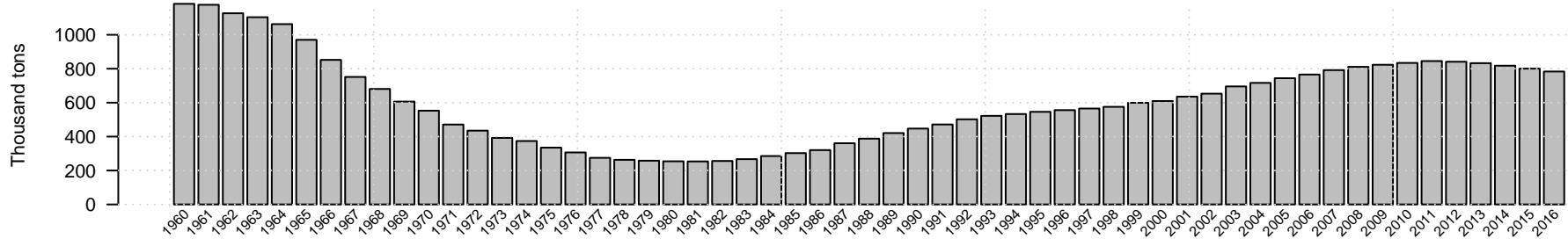
Bering Sea Aleutian Islands age 3 plus biomass of Pacific ocean perch
