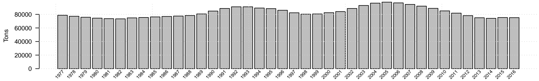
Gulf of Alaska age 3 plus biomass of Northern rock sole
