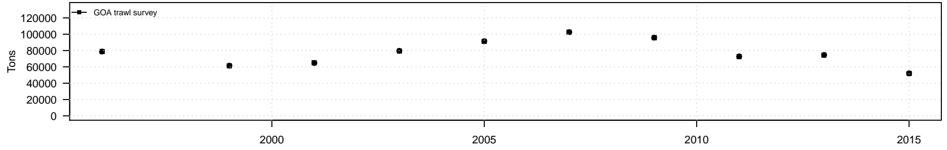
Gulf of Alaska survey biomass of Northern rock sole
