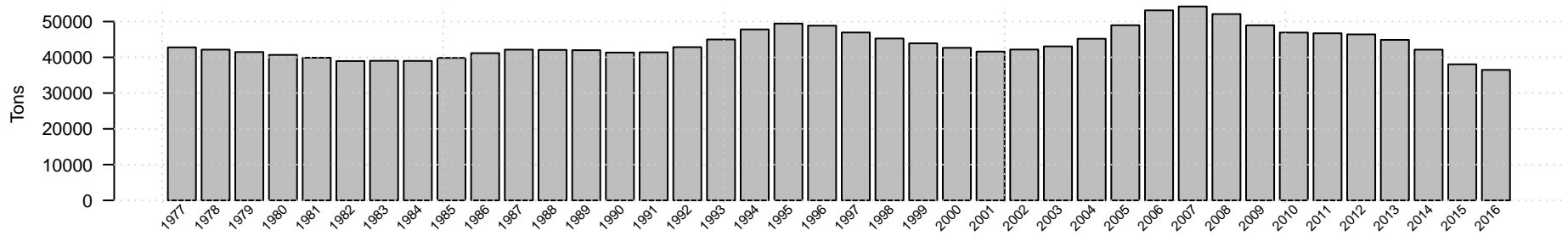
Gulf of Alaska spawning biomass of Northern rock sole
