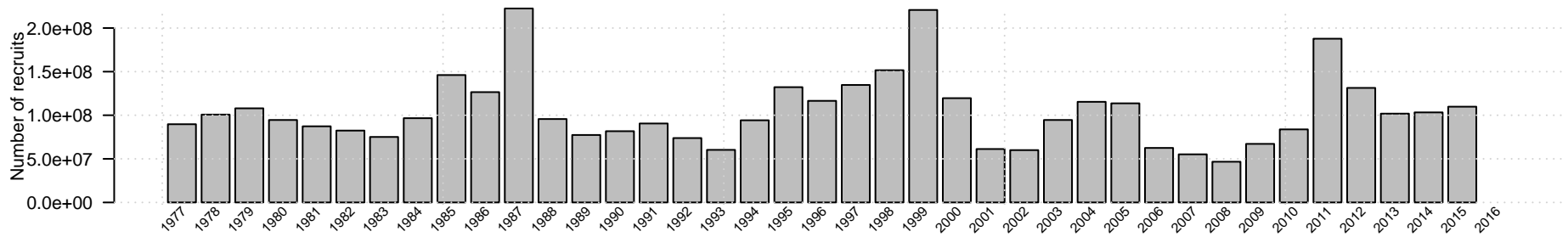
Gulf of Alaska age 0 recruitment of Northern rock sole
