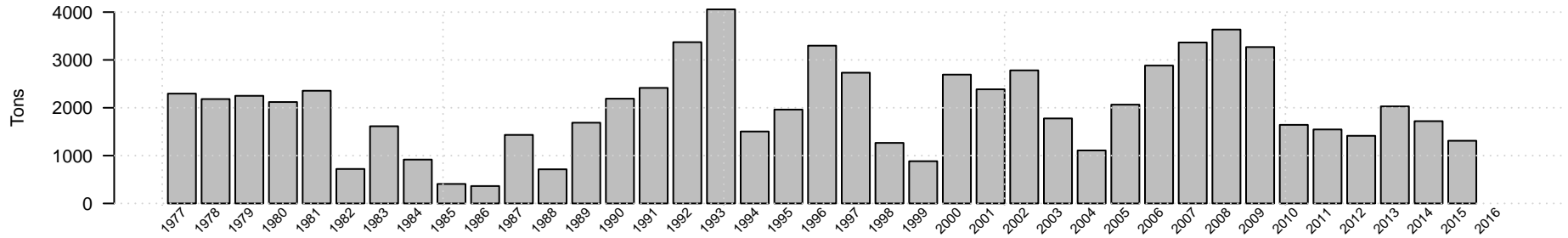
Gulf of Alaska catch of Northern rock sole
