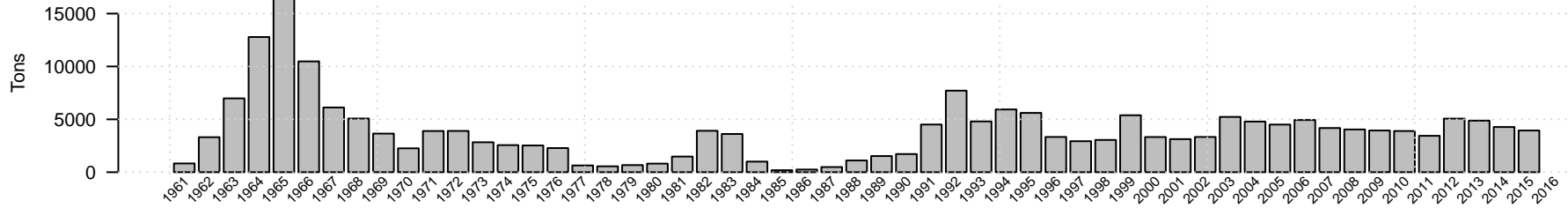
Gulf of Alaska age 2 plus biomass of Northern rockfish
