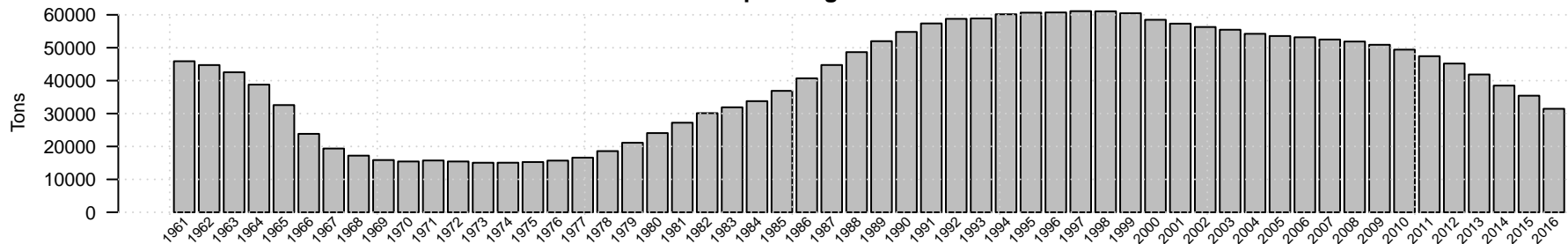
Gulf of Alaska spawning biomass of Northern rockfish
