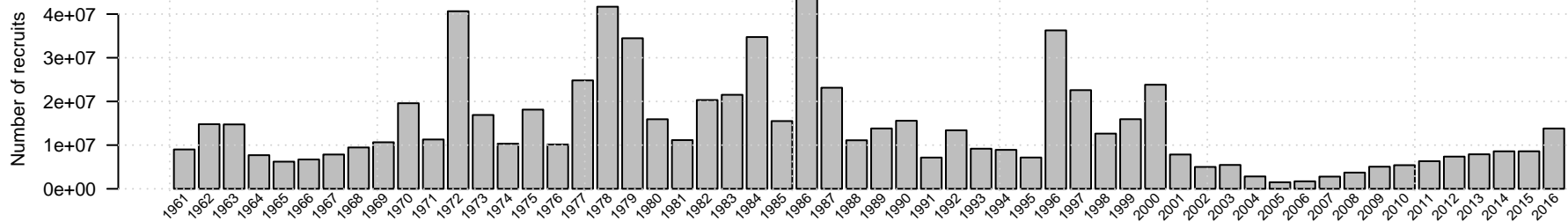
Gulf of Alaska age 2 recruitment of Northern rockfish
