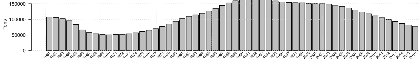
Gulf of Alaska age 2 plus biomass of Northern rockfish
