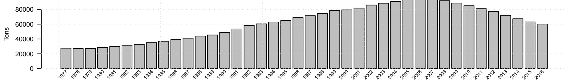
Gulf of Alaska age 4 plus biomass of Dusky rockfish
