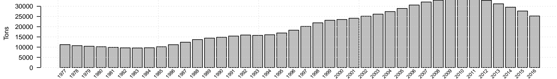
Gulf of Alaska spawning biomass of Dusky rockfish
