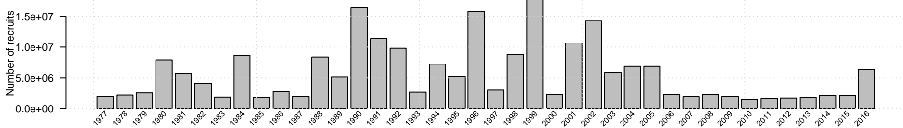
Gulf of Alaska age 4 recruitment of Dusky rockfish
