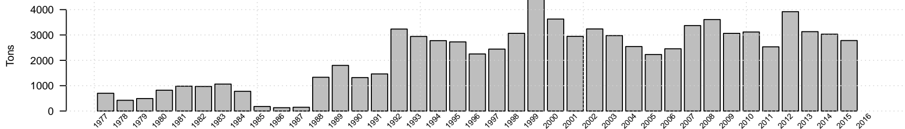
Gulf of Alaska catch of Dusky rockfish
