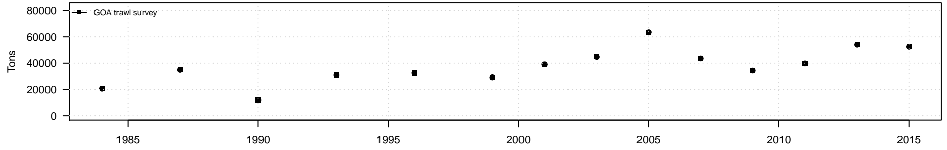
Gulf of Alaska survey biomass of Dusky rockfish
