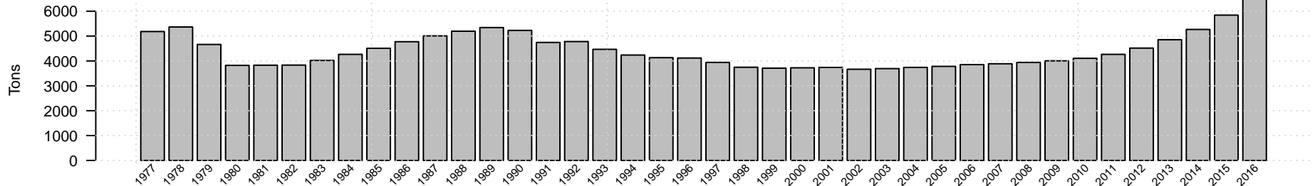
Bering Sea Aleutian Islands spawning biomass of Blackspotted rockfish
