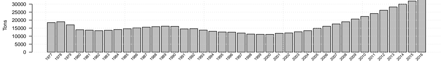
Bering Sea Aleutian Islands age 3 plus biomass of Blackspotted rockfish
