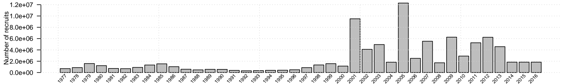
Bering Sea Aleutian Islands age 3 recruitment of Blackspotted rockfish
