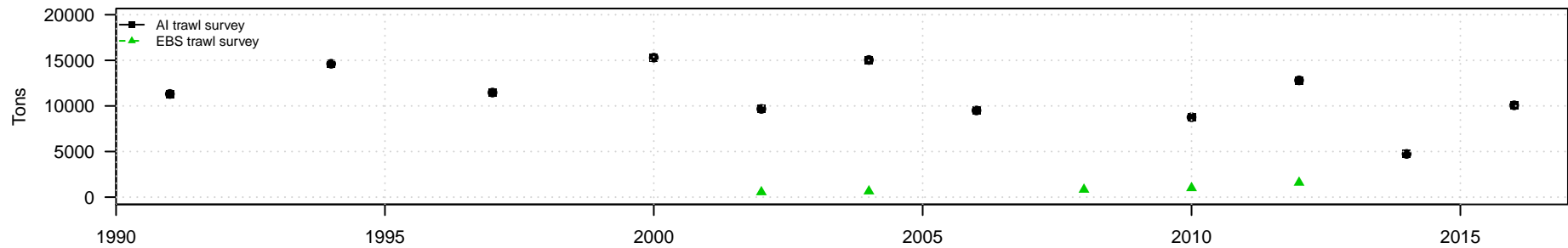
Bering Sea Aleutian Islands survey biomass of Blackspotted rockfish
