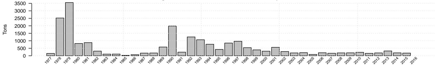
Bering Sea Aleutian Islands catch of Blackspotted rockfish
