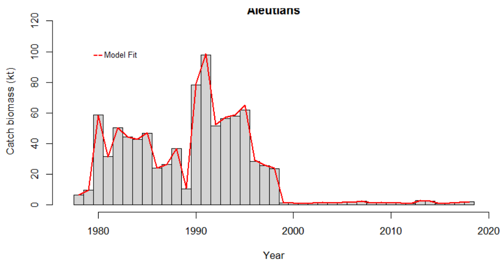
Figure 1A.17 Fits to total catch in 1,000s of tons for AI pollock over time 1978-2018.
