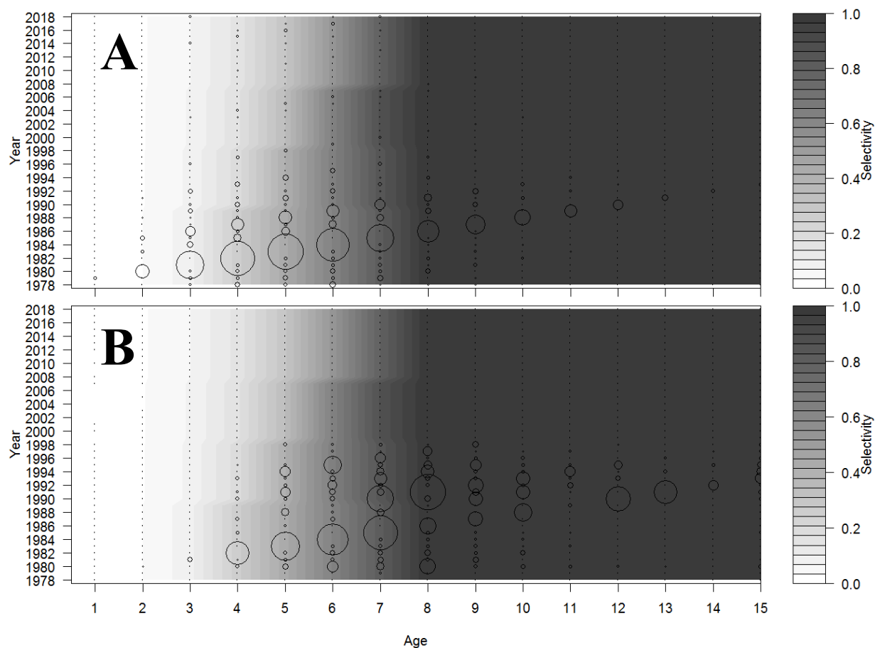
Figure 1A.19 Contour plots of fishery selectivity by age for AI pollock with bubble plots of (A) total biomass at age and (B) catch biomass at age for the Authors' preferred Model 1.0. Total biomass is scaled to 1/20 of the catch biomass bubbles.
