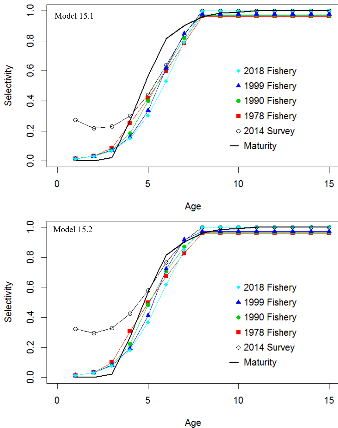
Figure 1A.14. Fishery and survey selectivity estimates with maturity at age for Aleutian Islands pollock models.
