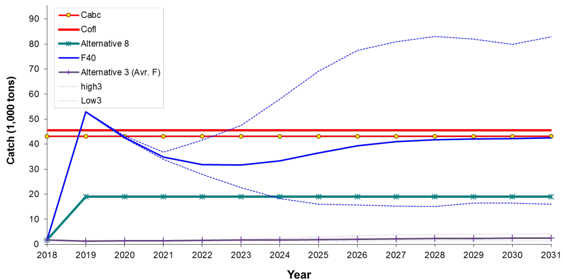
Figure 1A.24 Authors' preferred Model 15.1 projected catch for F_{40\%} , Alternative 3 (average F ), and Alternative 8 (19,000t) ABC scenarios.
