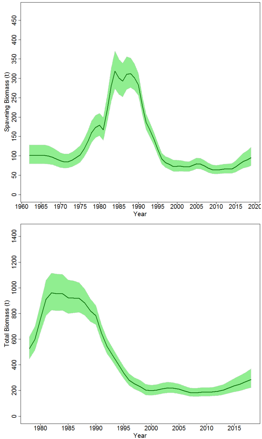
Figure 1A.16. Estimates of Aleutian Islands pollock spawning biomass (top) and age 1+ total biomass (bottom) in 1,000s of tons from the authors' preferred Model 15.1. Confidence intervals are two standard deviations.
