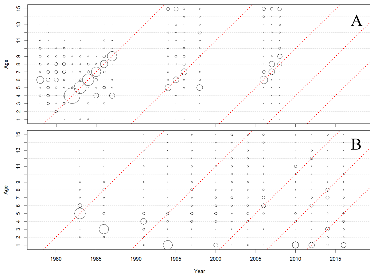
Figure 1A.4. Age distributions for 1978-2008 Aleutian Islands pollock fishery (A; top) and 1980 - 2016 Aleutian Islands Bottom Trawl surveys (B; bottom). The 1978, 1989, 2000, 2006, and 2011 year classes are indicated by the diagonal dashed lines.
