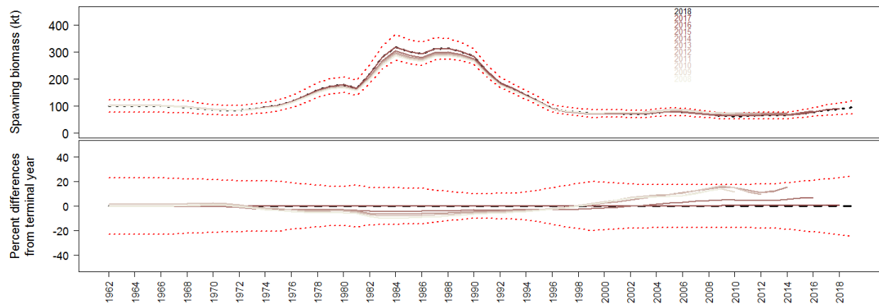
Figure 1A.23 Retrospective analysis for Authors' preferred Model 15.1 with data for the previous 10 years being systematically removed from the model. Black dashed line is the 2018 Model 15.1 estimate, the red dotted lines are the 95% confidence intervals calculated as \pm 1.96 \times \text{standard deviation} .
