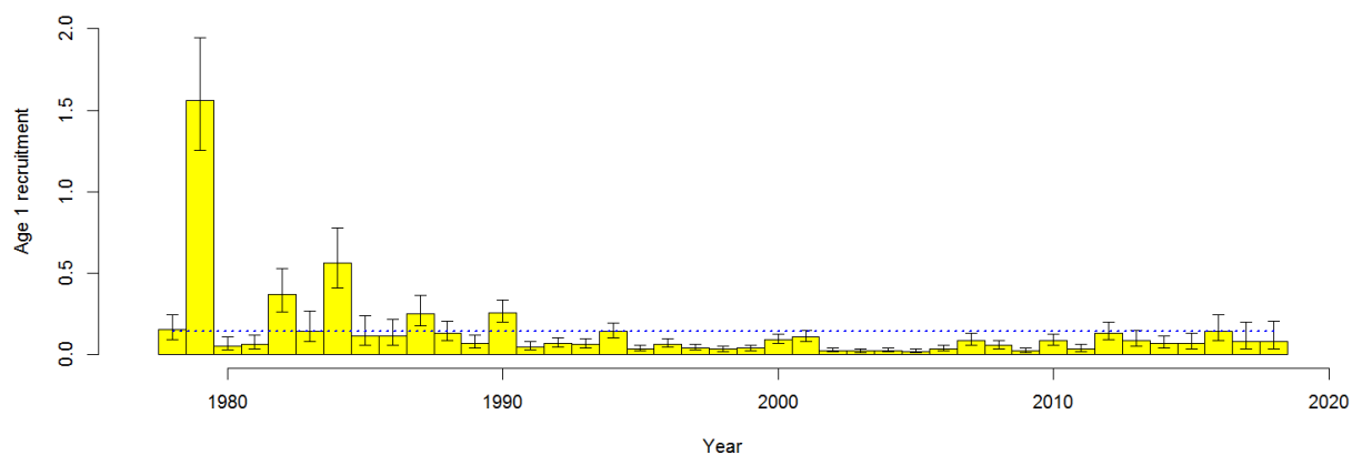
Figure 1A.20. Authors' preferred model estimates of Aleutian Islands pollock age 1 recruitment. The vertical bars represent the upper and lower 95% confidence bounds. The dotted line is the 1978-2015 mean age-1 recruitment.
