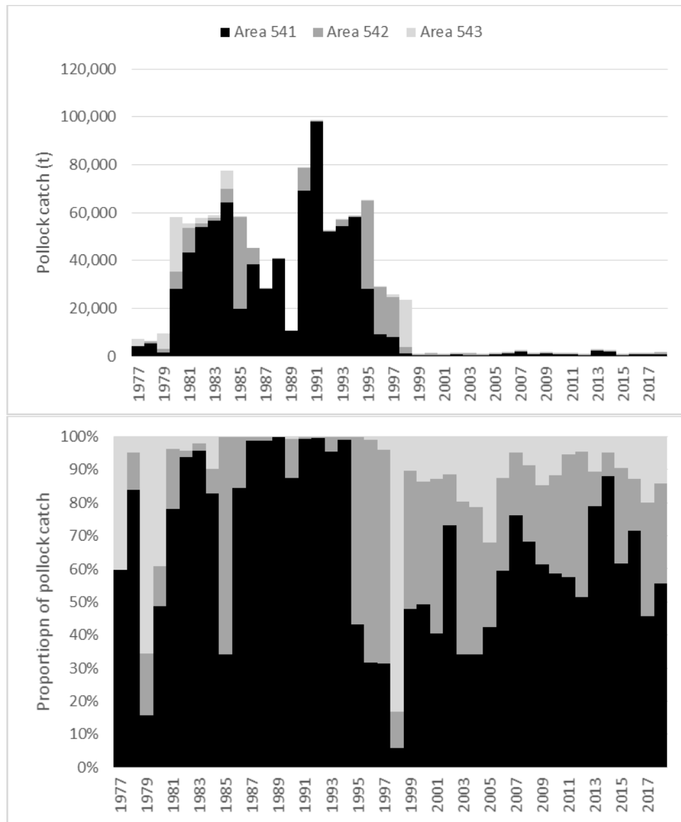
Figure 1A.3. Pollock catch by NMFS reporting area for 1977- 2018 by total catch (top) and percentage of catch by area (bottom).
