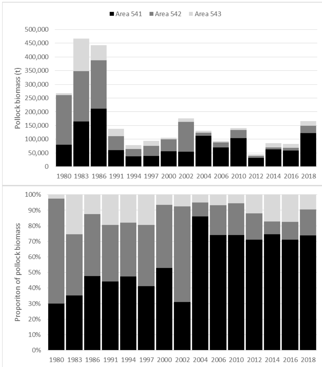
Figure 1A.1 Aleutian Islands bottom trawl survey pollock biomass (top) and proportion of biomass (bottom) for the three Aleutian Island management regions.
