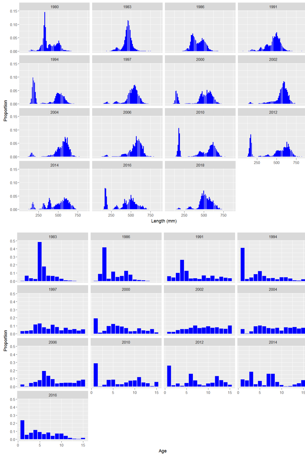
Figure 1A.6. Distribution by length (top) for 1980-2018 and age (bottom) for 1983-2016 for the Aleutian Islands bottom trawl surveys.
