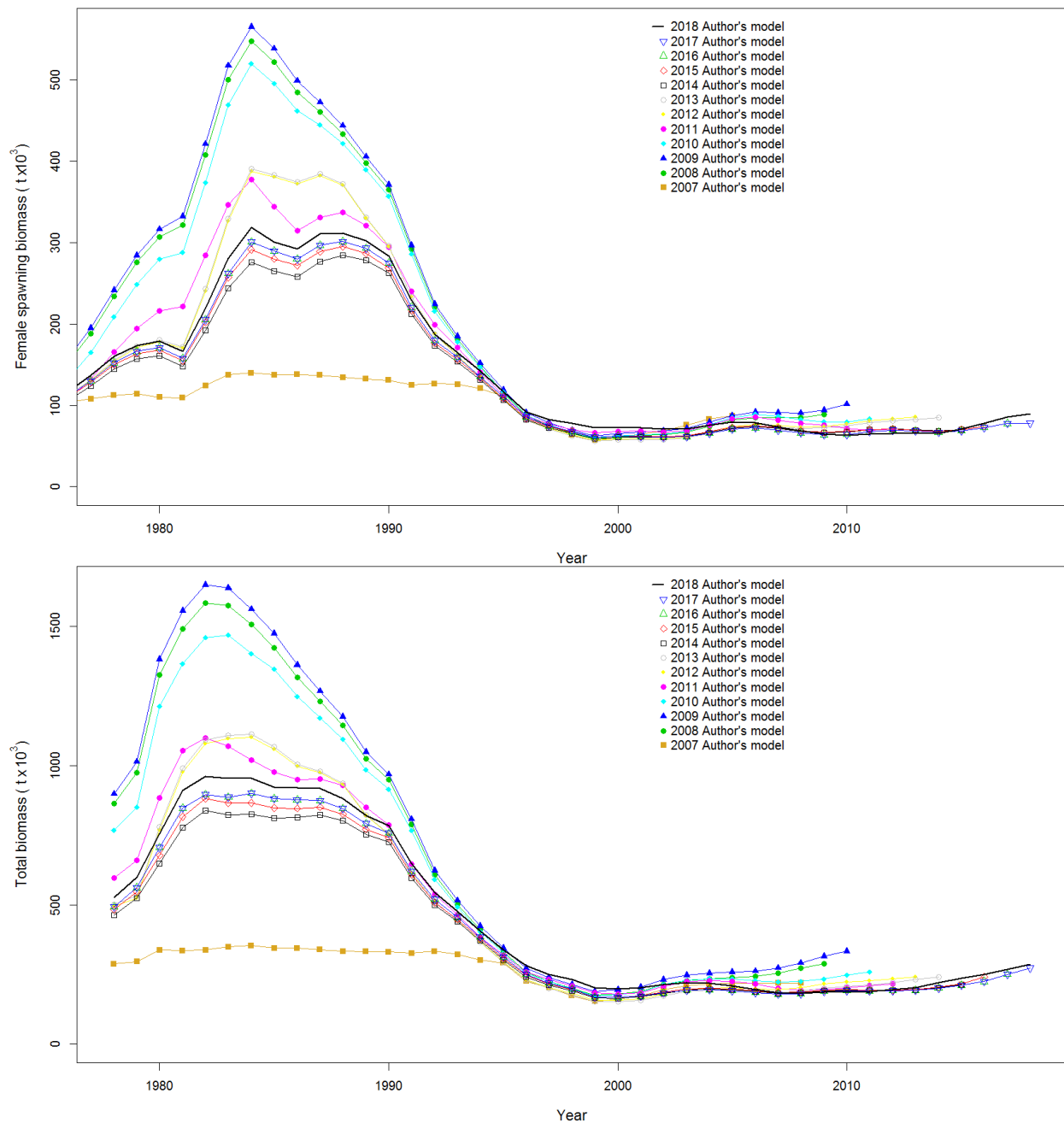
Figure 1A.15. Female spawning (top) and total (bottom) biomass trajectories for the 2018 Authors' preferred model compared with the 2007 through 2017 Authors' preferred models.
