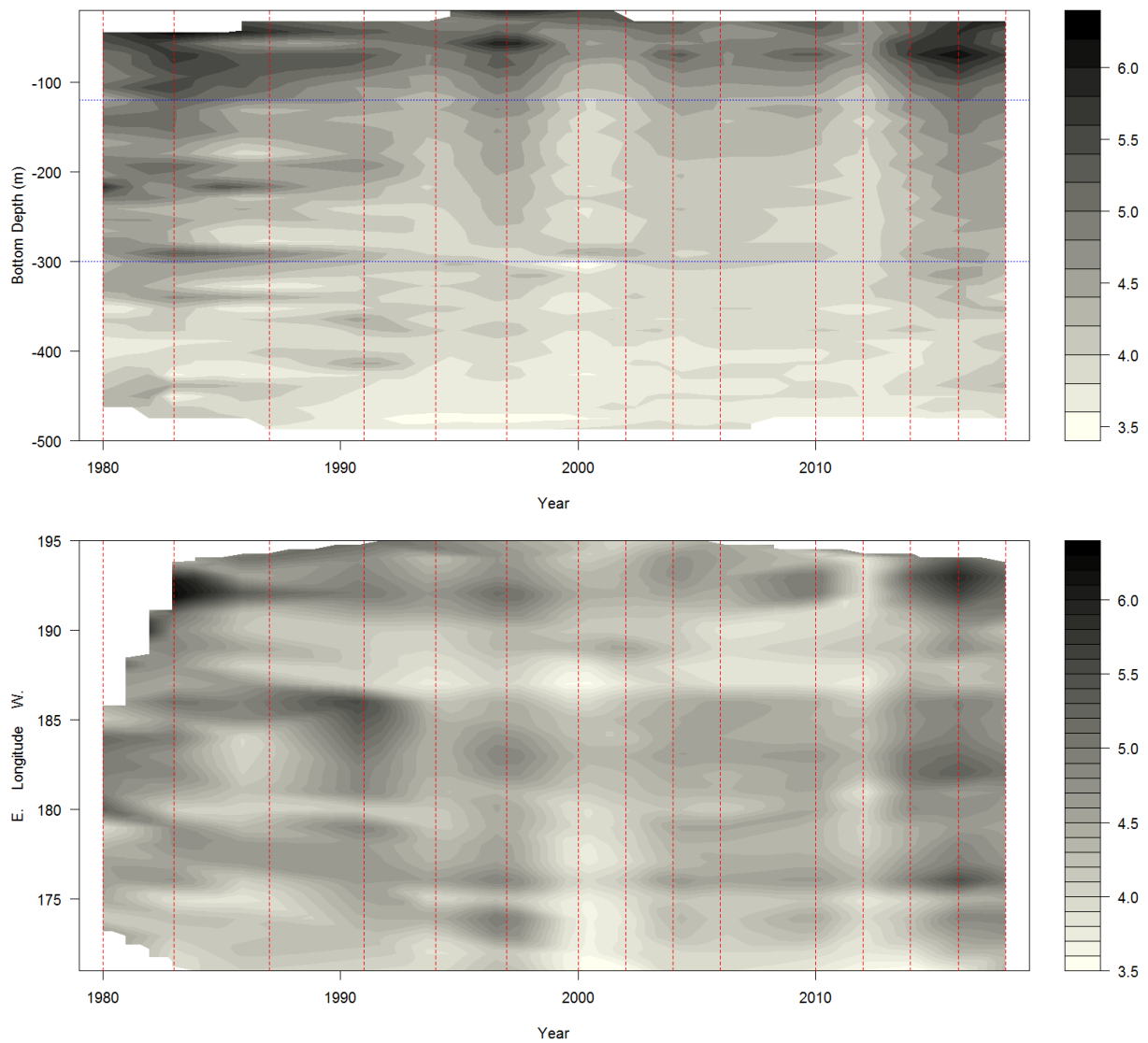
Figure 1A.33 Mean bottom temperatures by 10 m bottom depth (top) and by 1 degree longitude (bottom) by year. Red lines indicate years with survey data. Note the E longitudes ( >180 ) are further west in the Aleutian Islands. Blue lines are at -120 and -300, the area of highest densities for pollock in the AI.
