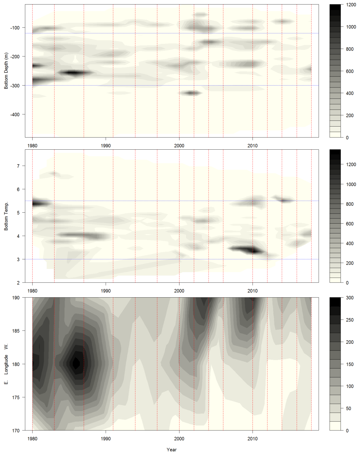
Figure 1A.34 Pollock CPUE \text{kg ha}^{-1} by 10 m bottom depth (top), 0.1 °C bottom temperature (middle), and 10° longitude (bottom). Note the E longitudes (<180) are further west in the Aleutian Islands.
