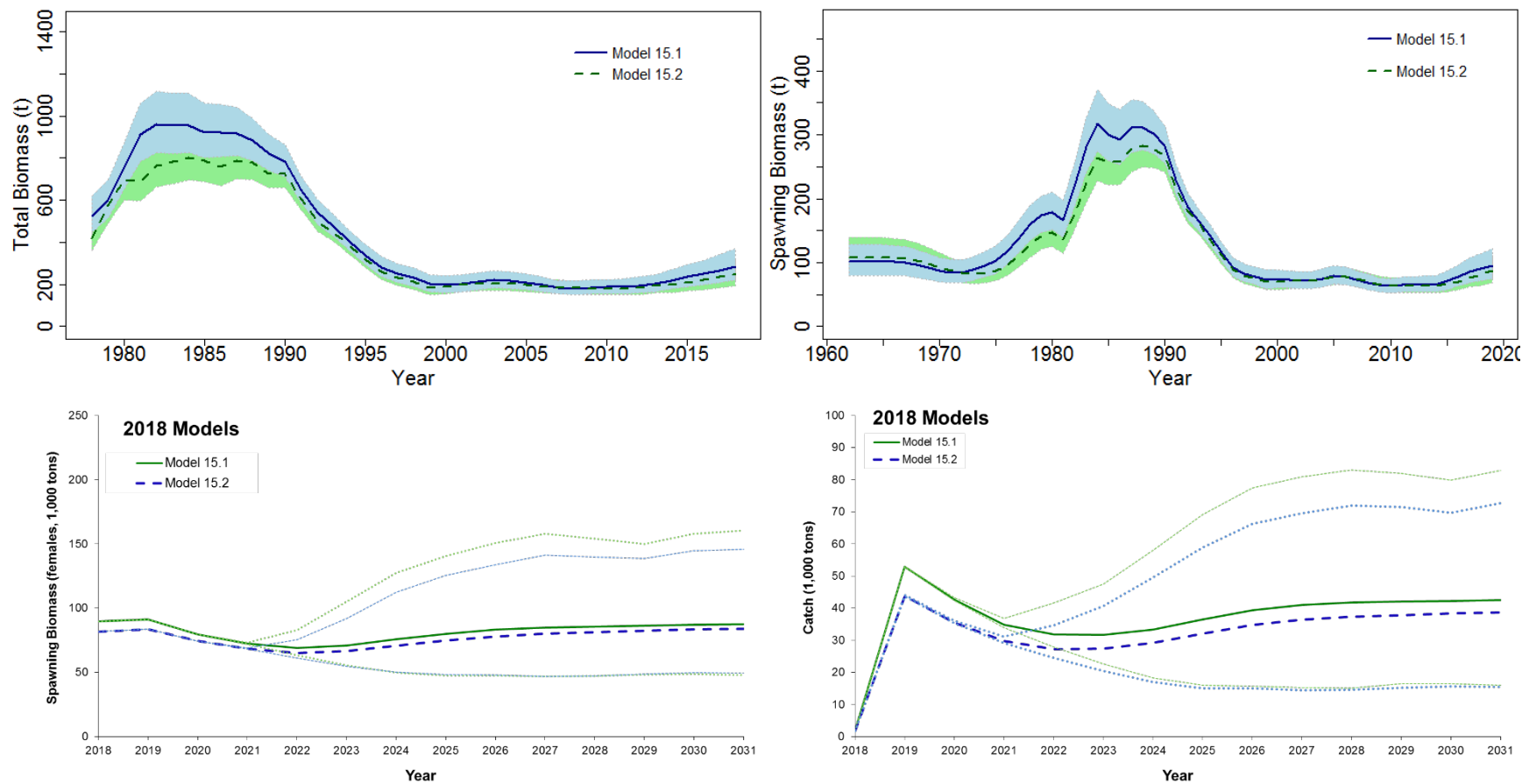
Figure 1A.8. Total biomass (top left), spawning biomass (top right), and spawning biomass projection (bottom left) and catch projection (bottom right) from Model 15.1. and Model 15.2.
