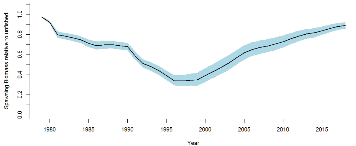
Figure 1A.22. Aleutian Islands pollock ratio of spawning biomass with fishing relative to spawning biomass without fishing for the authors' preferred model with 95% confidence interval.
