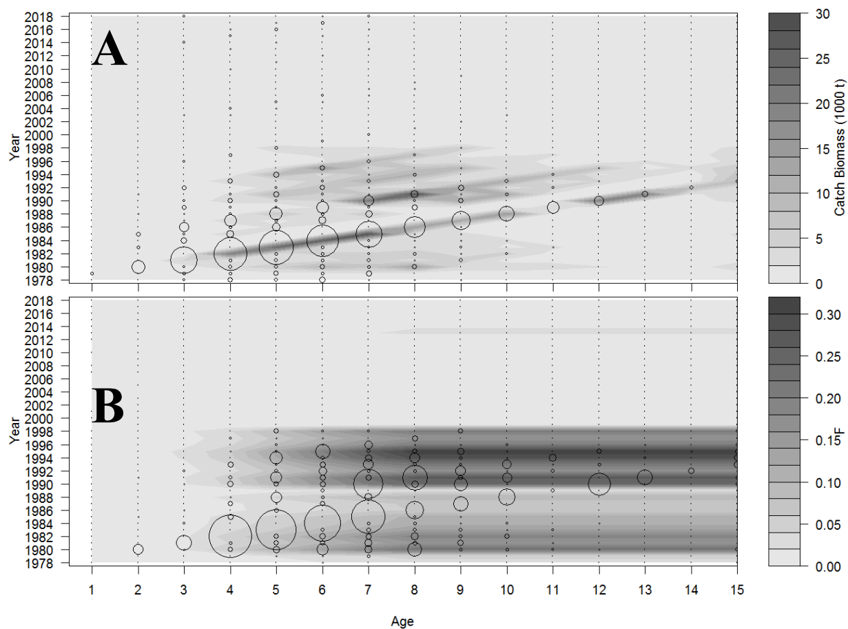
Figure 1A.18 AI pollock authors' preferred Model 15.1 (A-contour) catch biomass in 1,000s of tons and (A-bubbles) total biomass and (B-contour) fishing mortality rates and (B-bubbles) catch biomass by age. Total biomass is scaled to 1/20^{\text{th}} of the catch biomass in the bubble plots.
