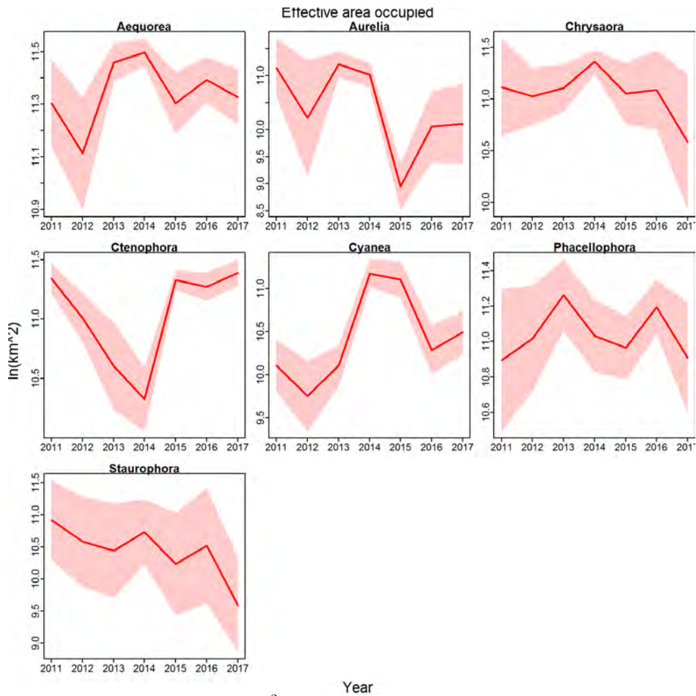
Figure 49: Effective area occupied (ln(km 2 )) indicating range expansion/contraction plus/minus 1 standard deviation for jellyfish in the eastern Gulf of Alaska during summer, 2011–2017.
