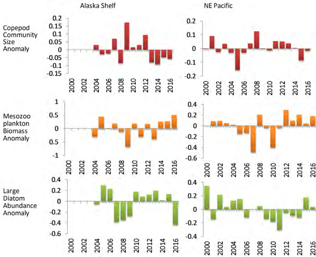
Figure 29: Annual anomalies of three indices of lower trophic levels (see text for description and derivation) for each region shown in (Figure 28). Note that sampling of this Alaskan Shelf region did not begin until 2004.
