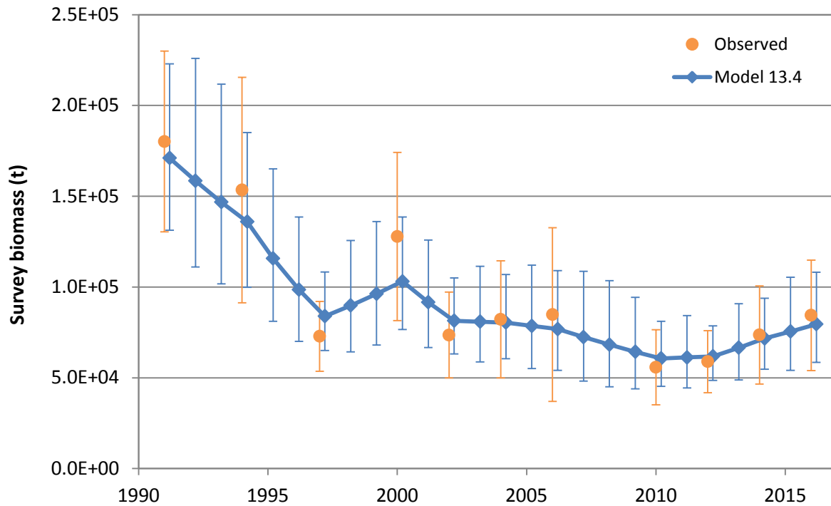
Figure 2A.2—Fit of Model 13.4 to survey biomass time series, with 95% confidence intervals for the observations and the estimates.
