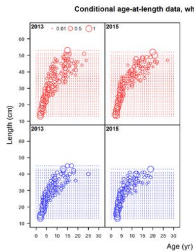
Figure 4.7. Survey conditional age-at-length data for northern rock sole.
