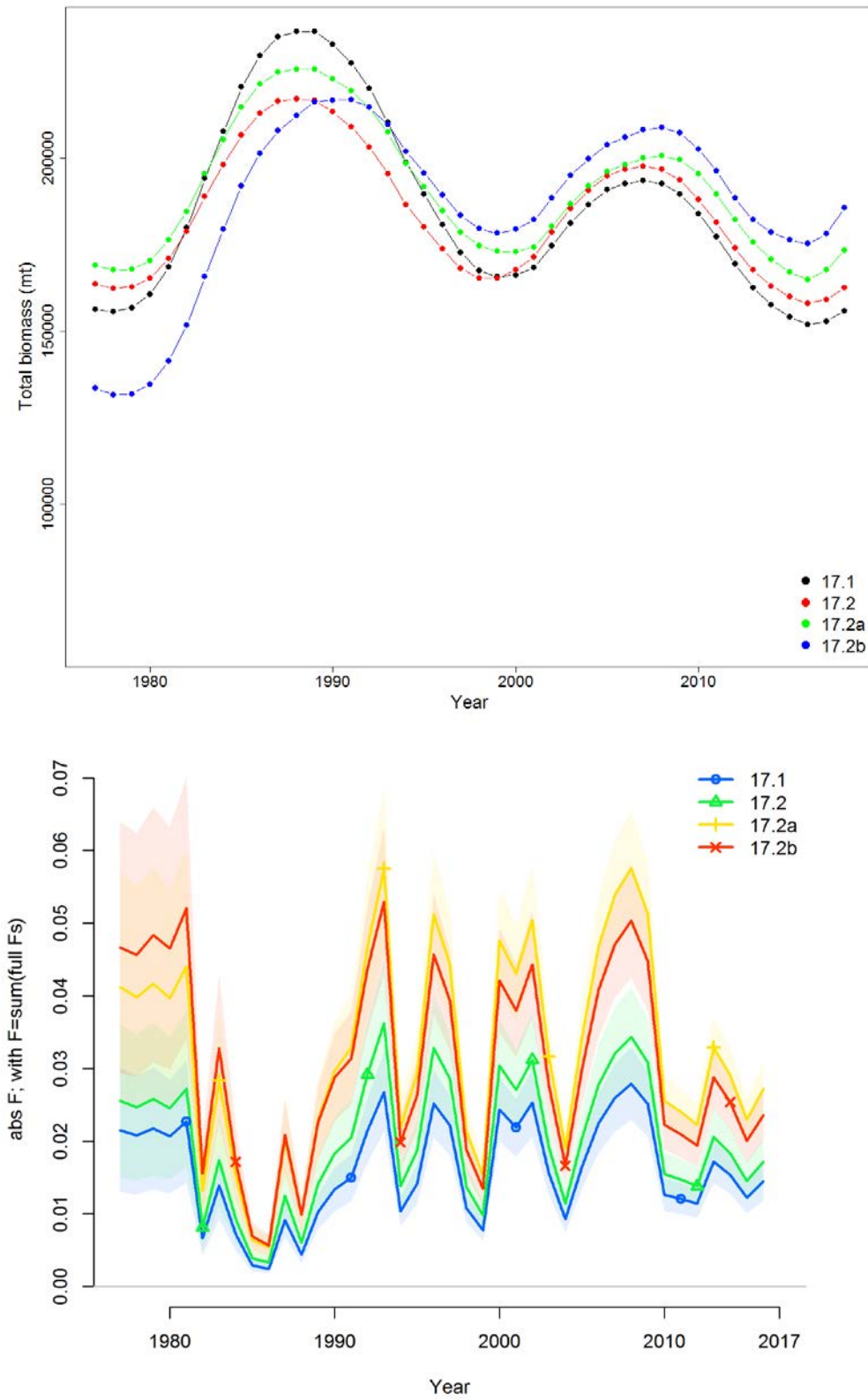
Figure 4.38. Southern rock sole total biomass and fishing mortality time-series.
