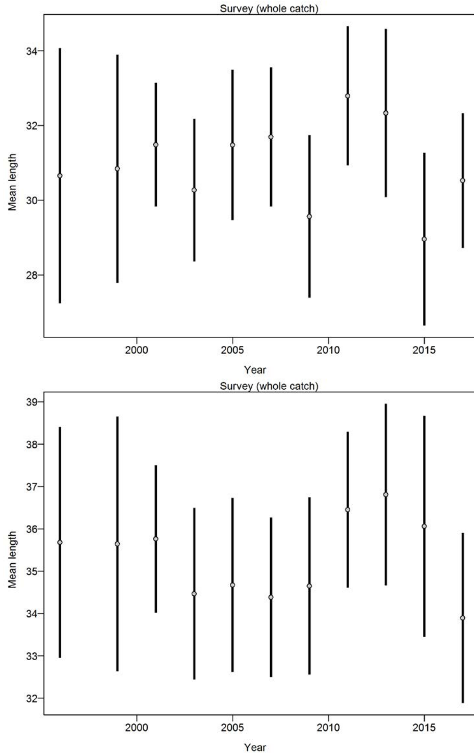
Figure 4.6 Northern rock sole mean length (cm) and the 95% confidence intervals based on the input sample size. Northern rock sole (top), southern rock sole (bottom).
