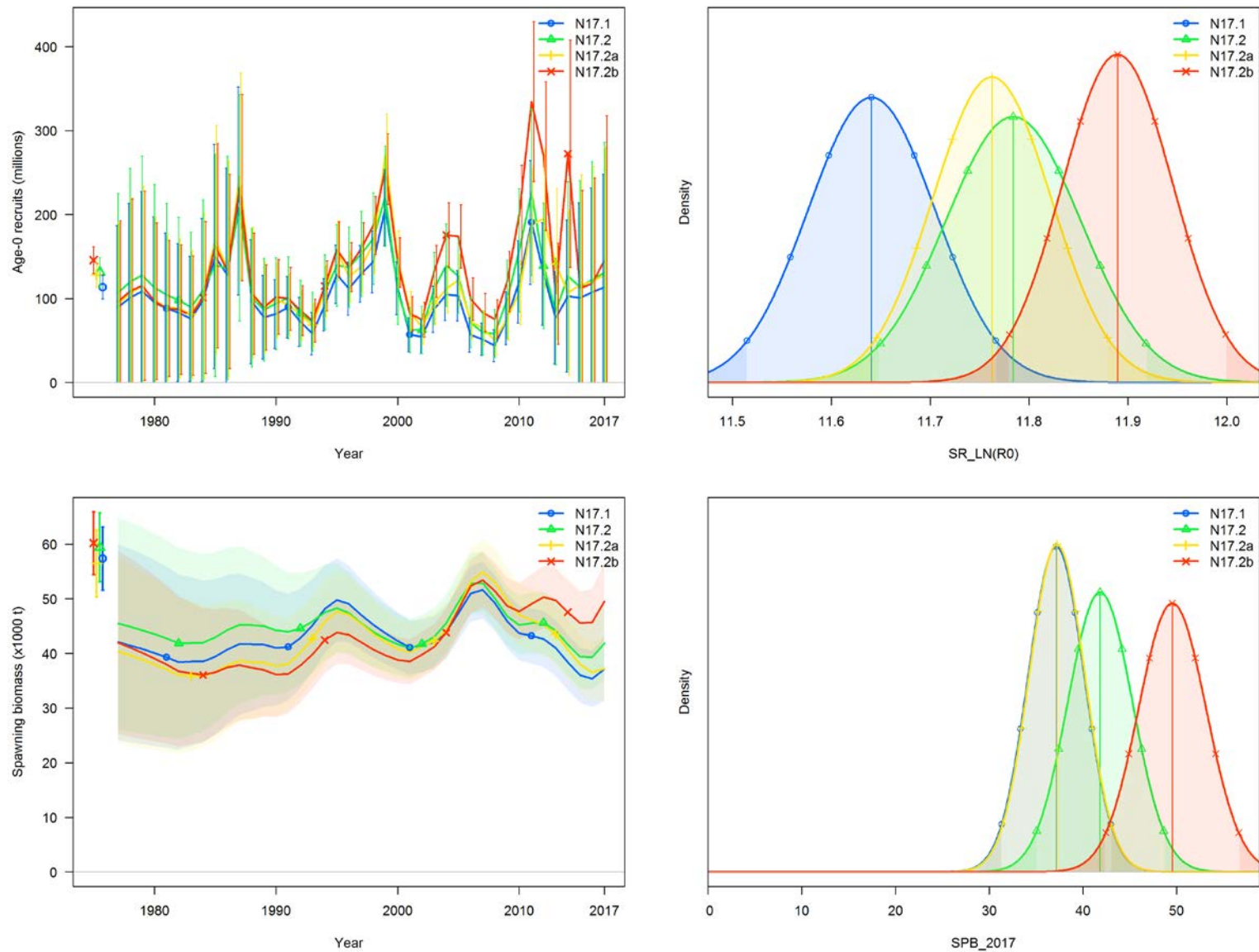
Figure 4.22. Northern rock sole age-0 recruits, \text{Ln}(R_0) density, spawning stock biomass with uncertainty, and spawning biomass density in 2017.
