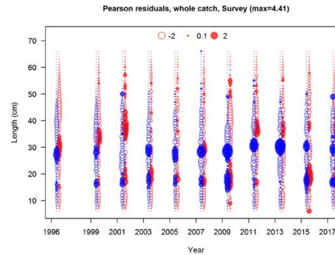
Figure 4.17. Pearson residuals (red - female, blue – male) for survey size composition data. Closed bubbles are positive residuals (observed > estimated).
