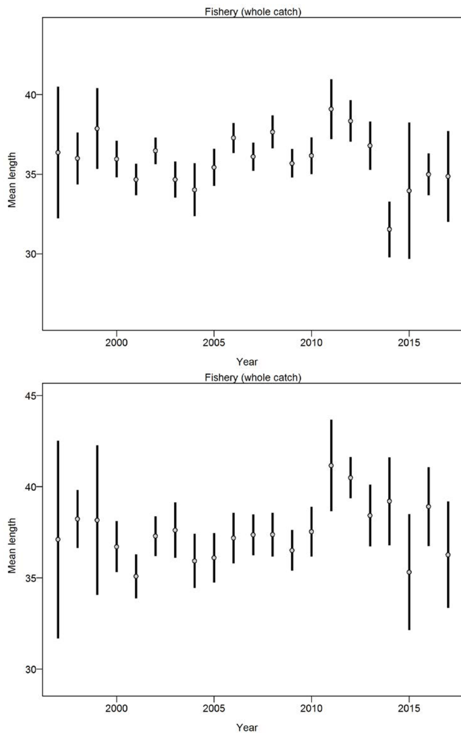
Figure 4.3 Mean length and the 95% confidence intervals based on the input sample size. Northern rock sole (top), southern rock sole (bottom).
