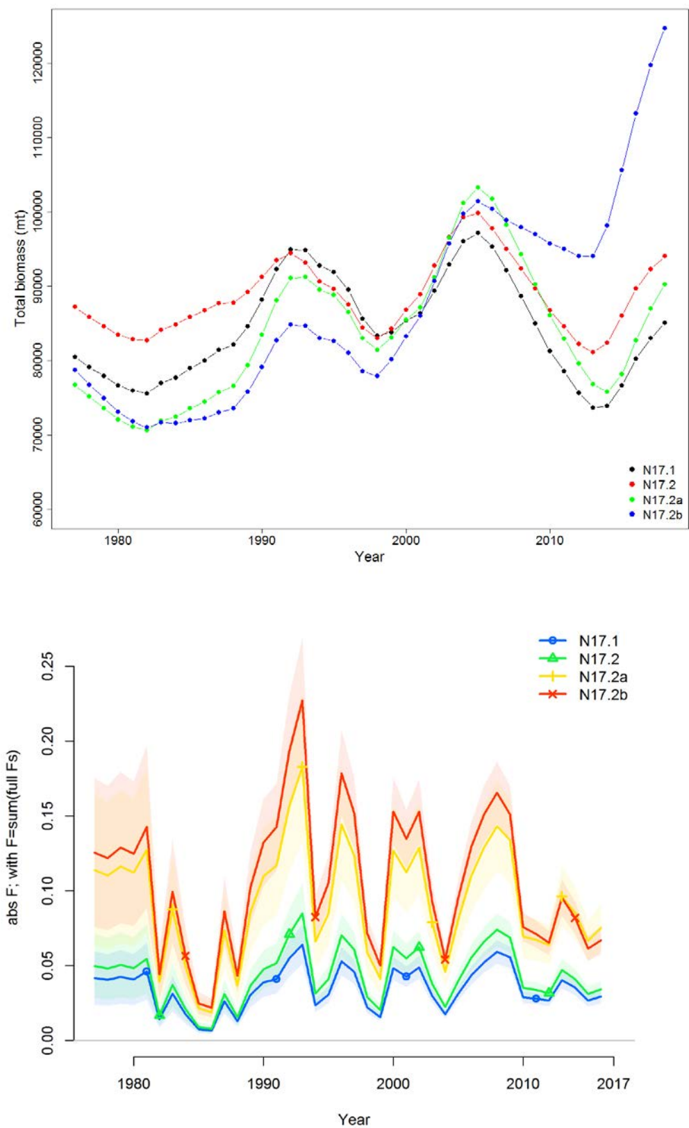
Figure 4.23. Northern rock sole total biomass (age0+) and fishing mortality estimates.
