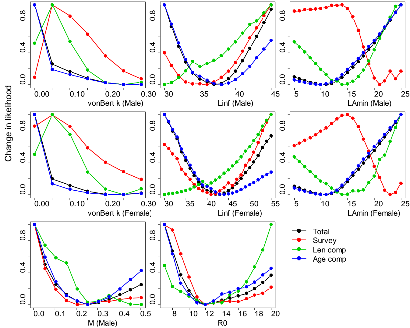
Figure 4.24. Likelihood profiles for the preferred northern rock sole assessment model, model 17.2. The change in the likelihood was scaled to 1 so that the pattern could be seen for all likelihood components. Likelihood profiles are shown for estimated model parameters, excluding the selectivity parameters.
