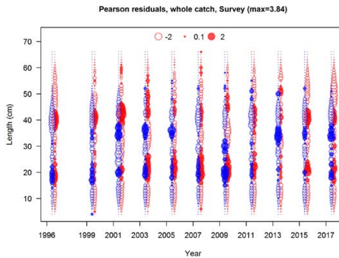
Figure 4.32. Pearson residuals (red - female, blue – male) for southern rock sole survey size composition data. Closed bubbles are positive residuals (observed > estimated). Scales differ by model. Model 15.1 was fit to the 2017 length composition data, hence the absence of residuals.
