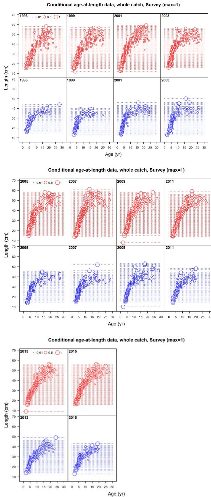
Figure 4.8. Survey conditional age-at-length data for southern rock sole.
