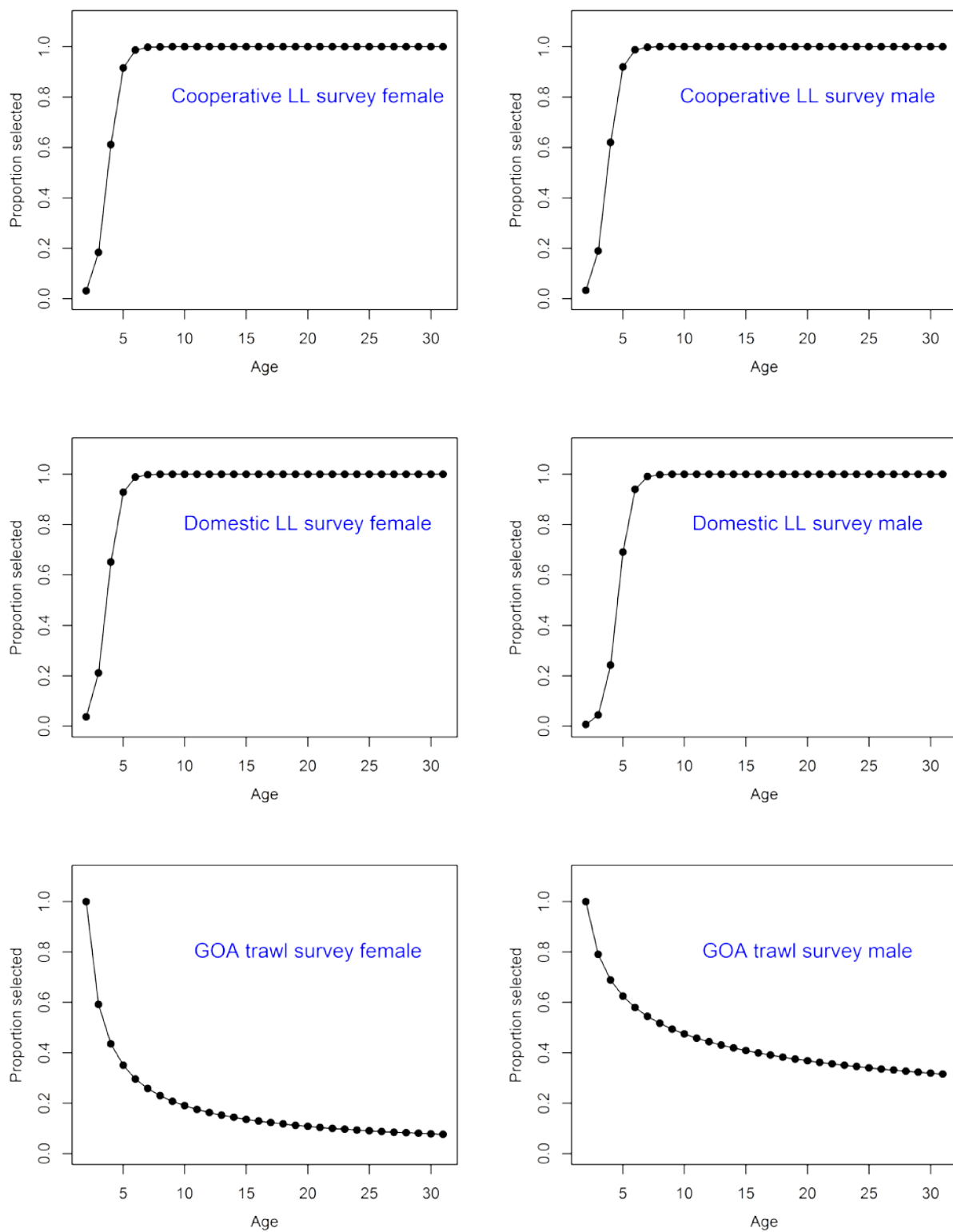
Figure 3.40 (cont.). Sablefish selectivities for surveys.
