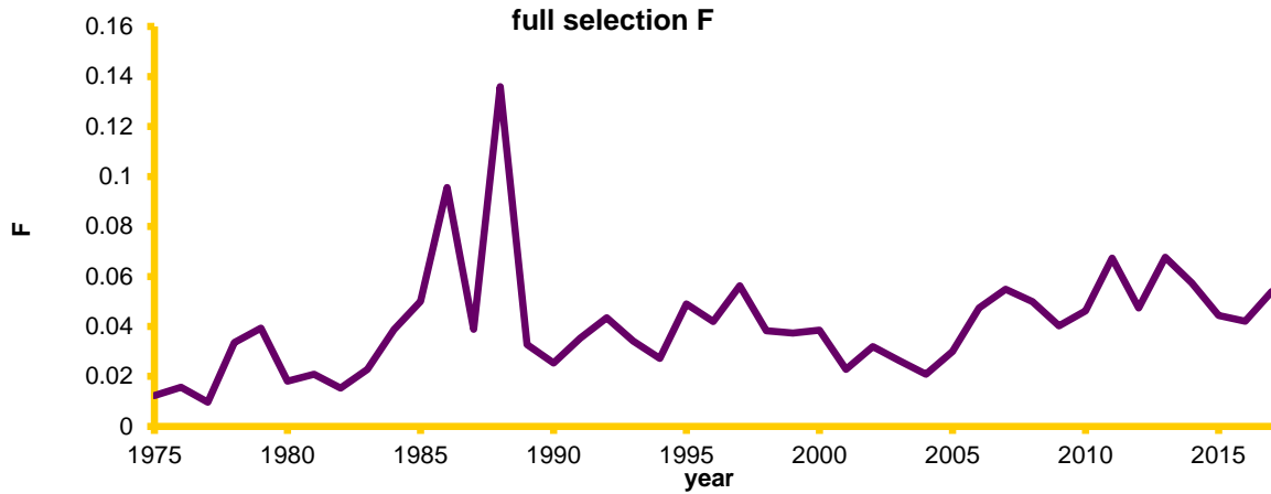
Figure 10.17--Estimated fully selected fishing mortality.
