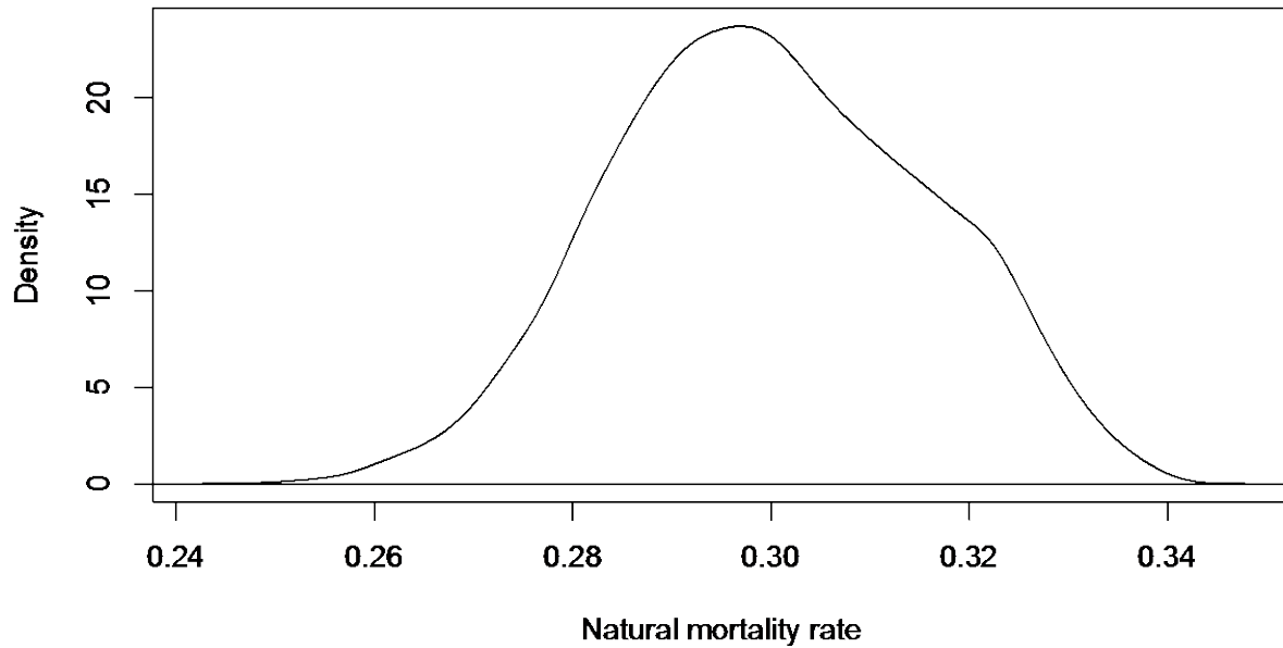
Figure 1B.5. Posterior marginal distribution of one million MCMC samples for the Bogoslof pollock age-structured model for natural mortality ( M ) under Model 1.1 configuration. The median and the mean were 0.299, and 0.301, respectively.
