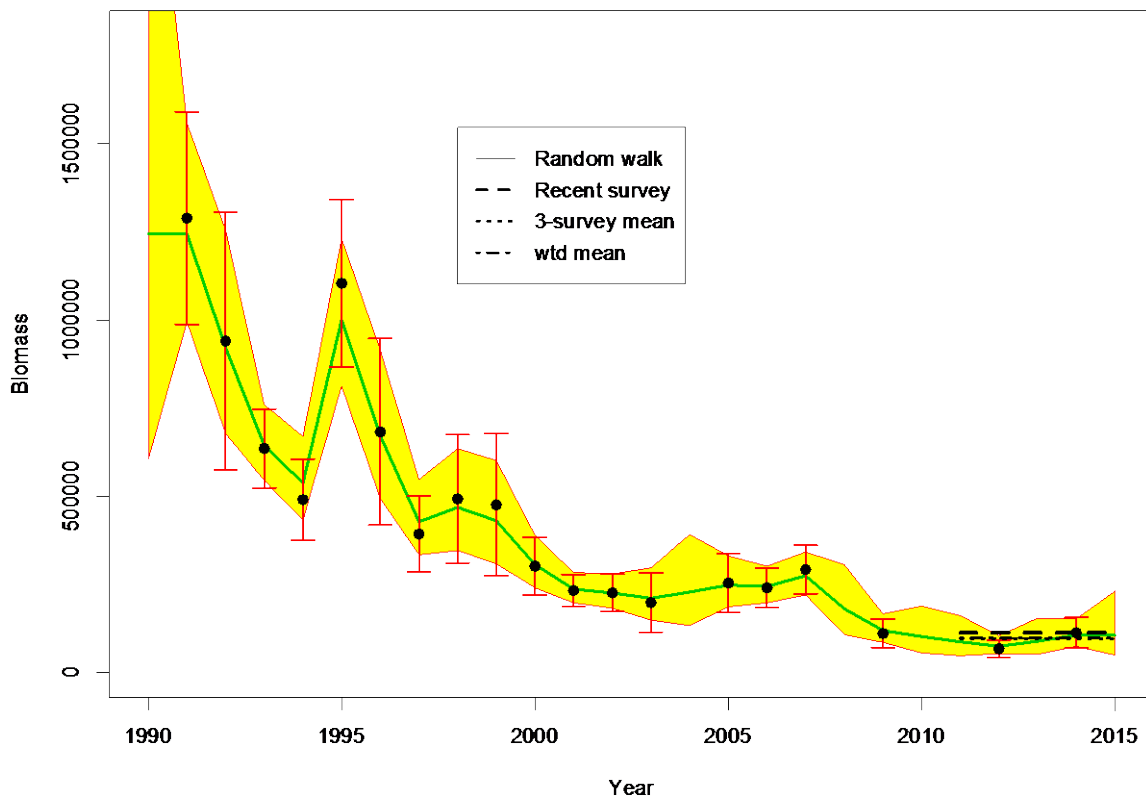
Figure 1B.6. Bogoslof Island pollock survey estimates fitted to a process error model for averaging recruitment. The shade represents the approximate 90% confidence interval from the model. Note that the lines described in the legend appear for the last few years and are difficult to distinguish given the scale.
