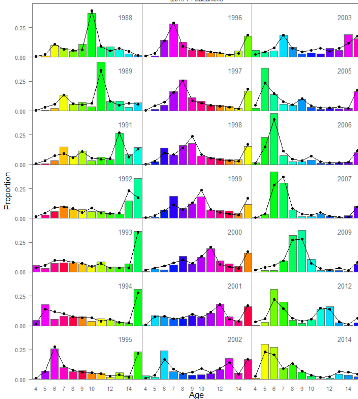
Figure 1B.2. Bogoslof pollock age-structured model fits to the survey age compositions when natural mortality ( M ) was freely estimated.
