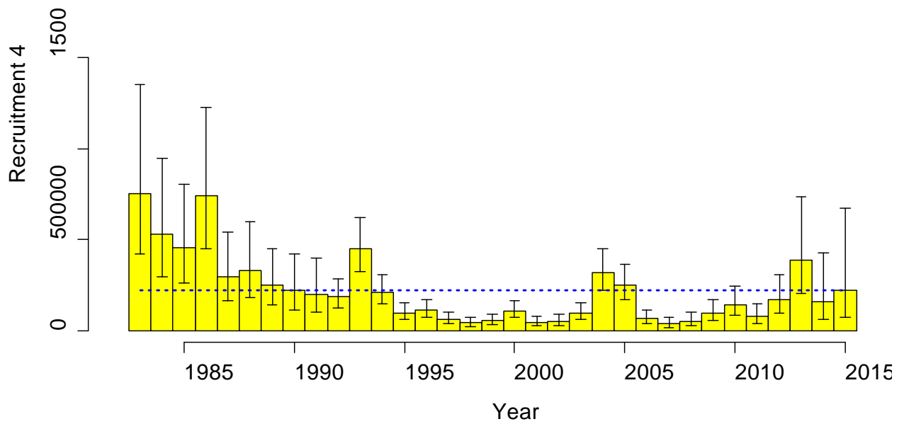
Figure 1B.4. Bogoslof pollock age-structured model results in recruitment (at age 4) in thousands.
