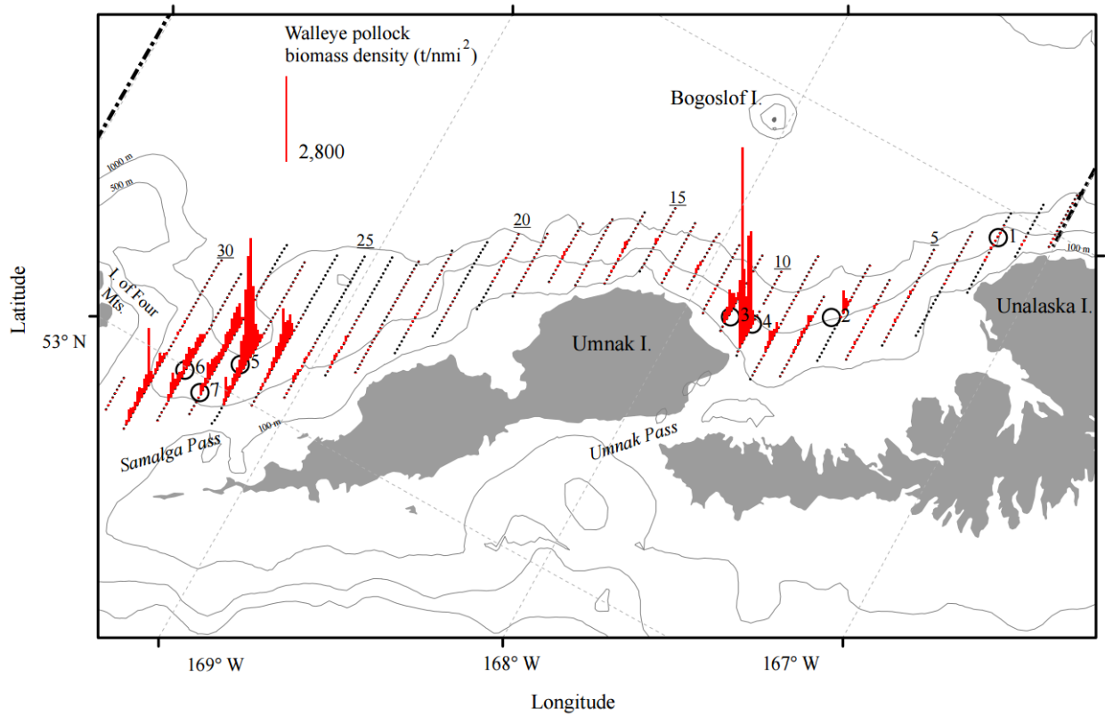
Figure 1B.1. Distribution of pollock biomass ( t/nmi^2 ) observed along transects during the winter 2014 acoustic-trawl survey. Transect numbers are underlined; trawl haul locations are indicated by circles.
