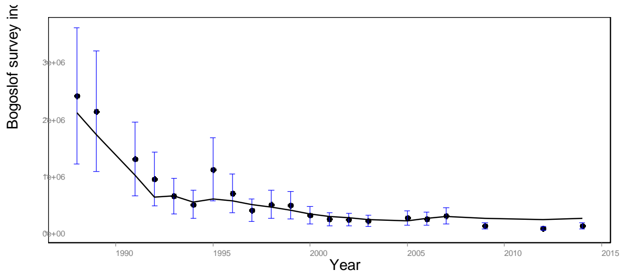
Figure 1B.3. The Bogoslof pollock age-structured model fit to the survey index data when natural mortality ( M ) was freely estimated.
