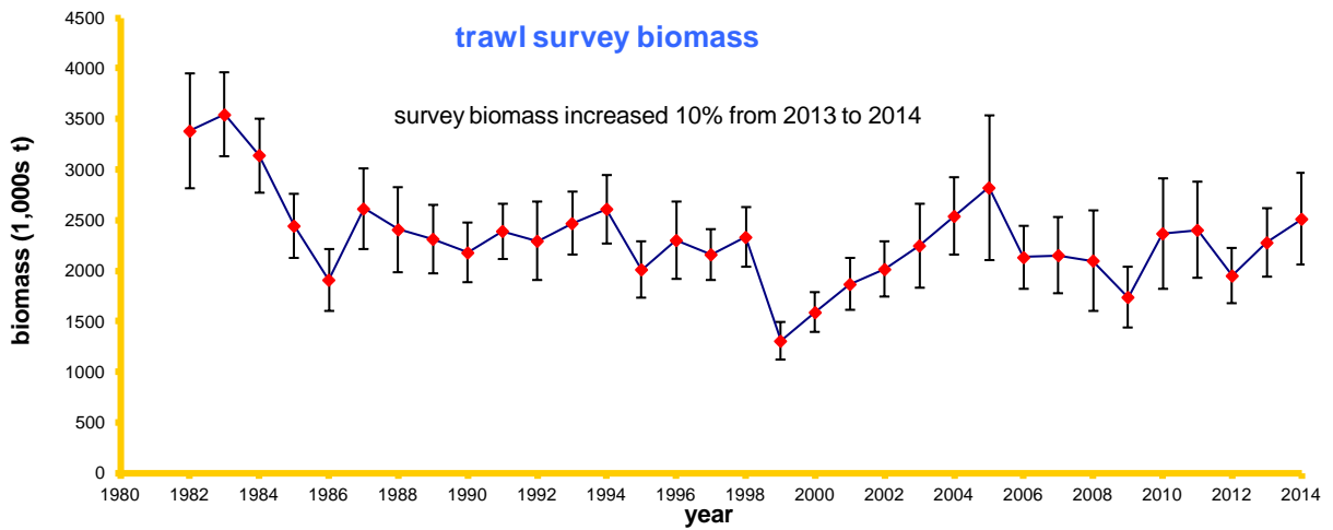
Figure 4.6.--Annual bottom trawl survey biomass point-estimates and 95% confidence intervals for yellowfin sole, 1982-2014.
