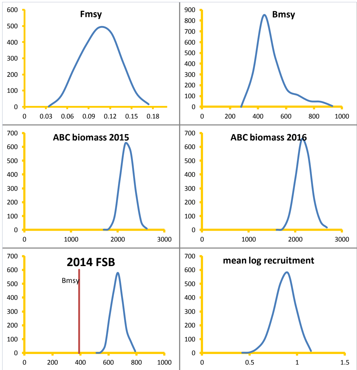
Figure 4.20.--Posterior distributions of some important parameters estimated by the preferred stock assessment model (from mcmc integration).
