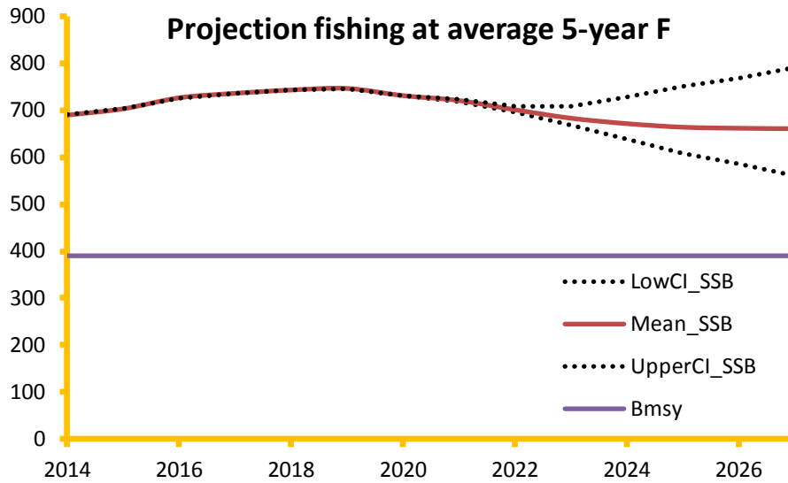
Figure 4.22.--Projection of yellowfin sole female spawning biomass (1,000s t) at the average full-selection F from the past 5 years (0.104) through 2027 with B_{40\%} and B_{msy} levels indicated.
