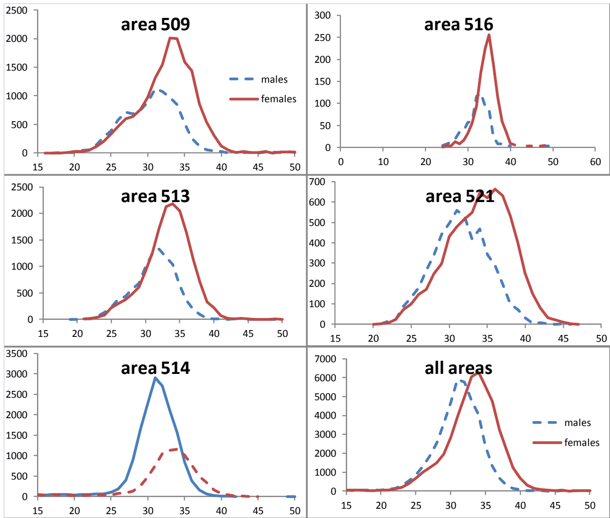
Figure 4.2--Size composition of the yellowfin sole catch in 2013 (through September), by subarea and total.
