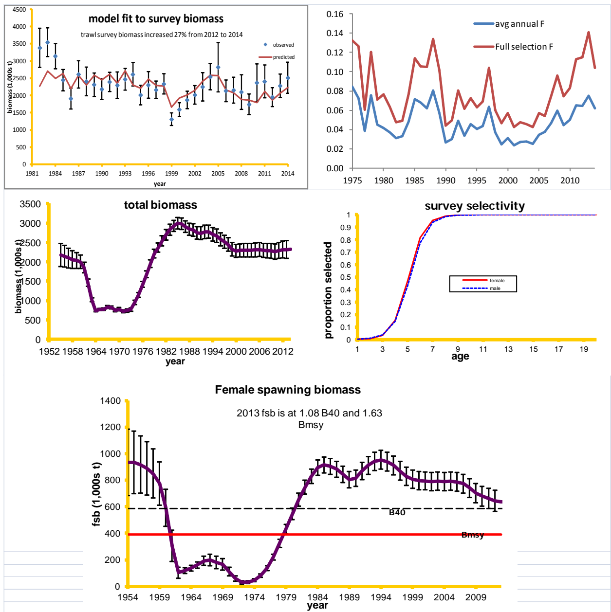
Figure 4.16. Model fit to the survey biomass estimates (top left panel), model estimate of the full selection fishing mortality rate throughout the time-series (top right panel), model estimate of total biomass (middle left panel), the model estimate of survey selectivity (middle right panel) and the estimate of female spawning biomass (bottom left panel).
