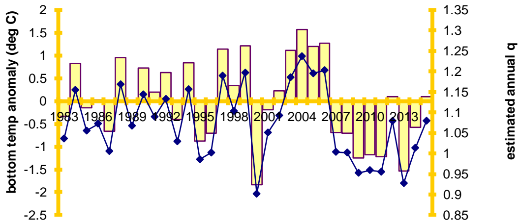
Figure 4.11.--Average bottom water temperature from stations less than or equal to 100 m in the Bering Sea trawl survey (bars) and the stock assessment model estimate of q for each year 1982-2014.
