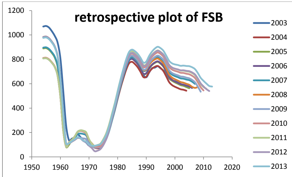
Figure 4.21—Retrospective plot of yellowfin sole female spawning biomass (1,000s t), 2003-2013, from the recommended assessment model.
