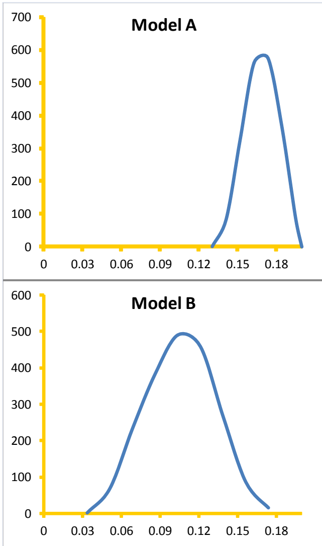
Figure 4.13--Posterior distributions of F_{msy} for the two models considered in the stock productivity analysis.
