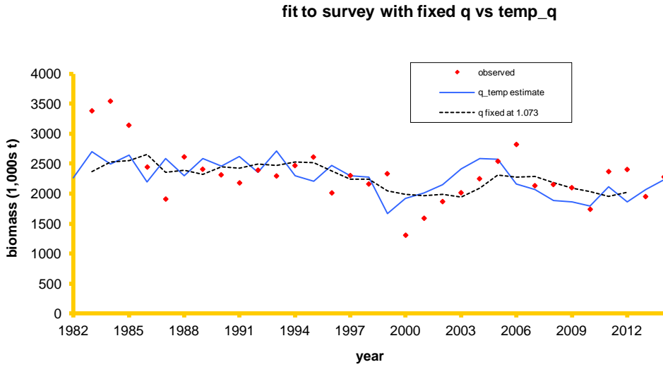
Figure 4.18.--Comparison of the fit to the survey biomass using a fixed q and the q-bottom temperature relationship.
