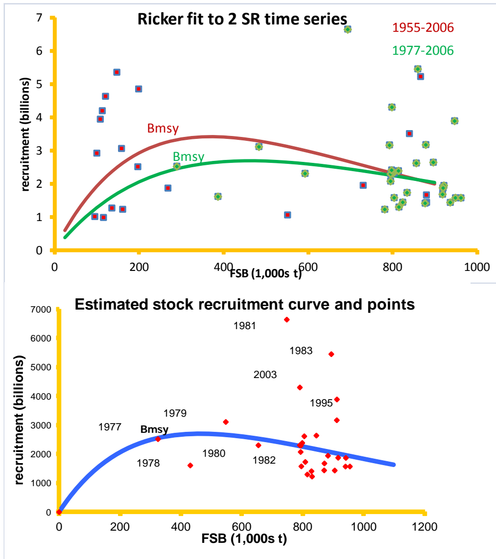
Figure 4.12--Fit of the Ricker (1958) stock recruitment model to two distinct stock recruitment time-series data sets (top panel), and the fit to the assessment preferred model (model B, lower panel).
