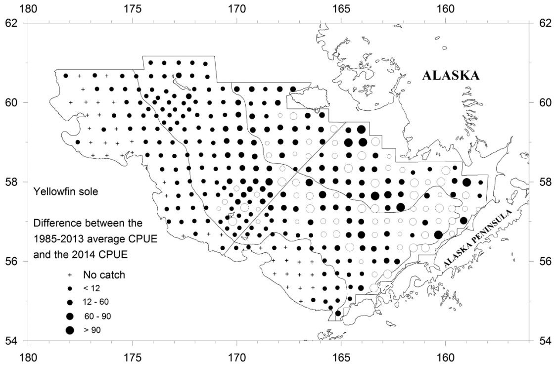
Figure 4.7.--Difference between the 1985-2013 average trawl survey CPUE for yellowfin sole and the 2014 survey CPUE. Open circles indicate that the magnitude of the catch was greater in 2014 than the long-term average, closed circles indicate the catch was greater in the long-term average than in 2014.
