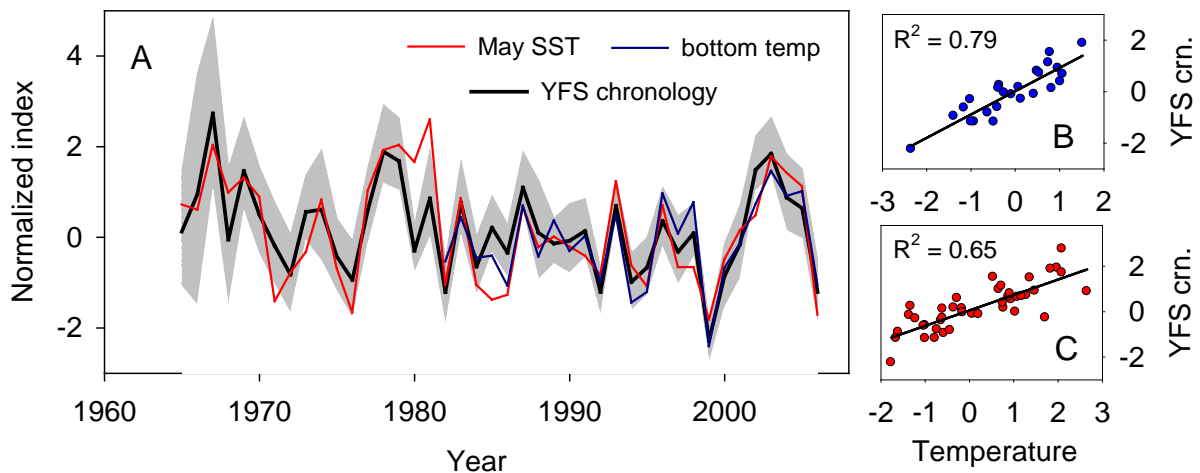
Figure 4.9--Master chronology for yellowfin sole and time series of mean summer bottom temperature and May sea surface temperature for the southeastern Bering Sea (Panel A). All data re normalized to a mean of 0 and standard deviation of 1. Correlations of chronologies with bottom temperature and sea surface temperature are shown in panels B and C, respectively. From Matta et al. 2010.
