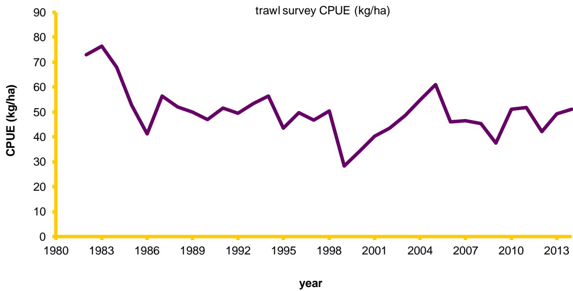
Figure 4.5.--Yellowfn sole CPUE (catch per unit effort in kg/ha) from the annual Bering Sea shelf trawl surveys, 1982-2014.
