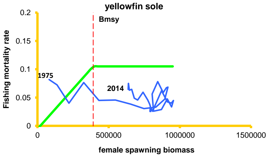
Figure 4.23.--Phase plane figure of the time-series of yellowfin sole female spawning biomass relative to the harvest control rule with 1975 and 2014 indicated.
