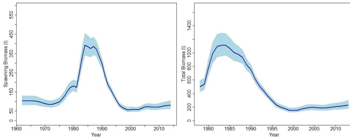
Figure 1A.18. Estimates of Aleutian Islands pollock spawning biomass (left) and age 2+ total biomass (right) in 1,000s of tons from the reference model. Confidence intervals are two standard deviations.
