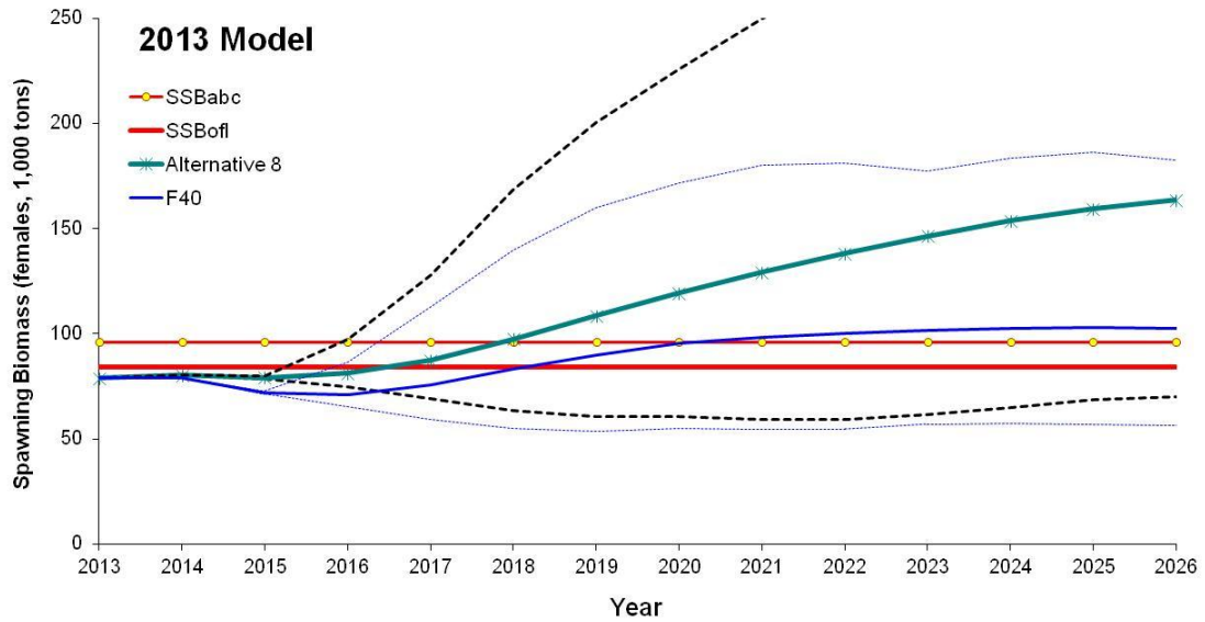
Figure 1A.26 Projected spawning biomass for F_{40\%} and Alternative 8 ABC scenarios.
