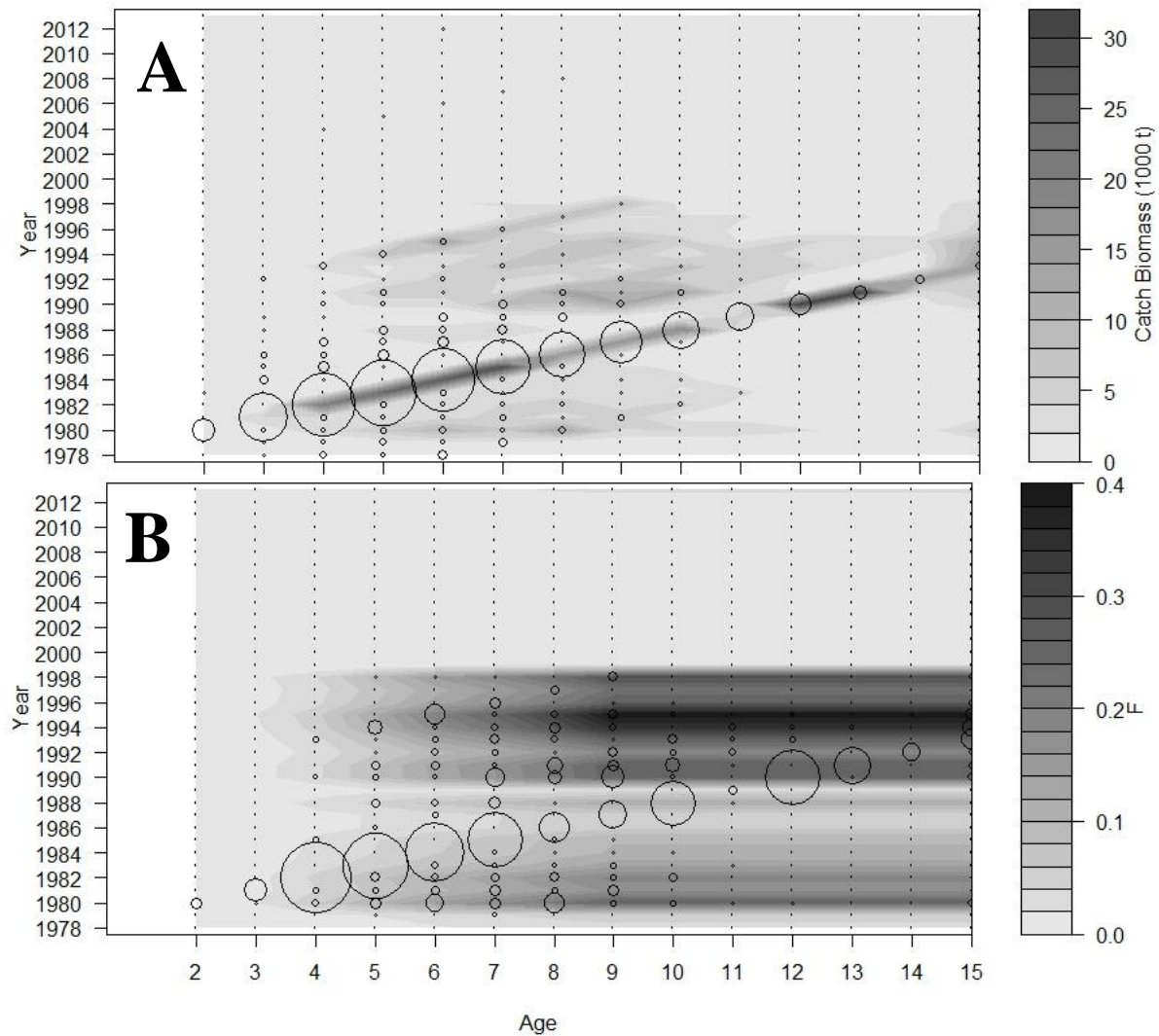
Figure 1A.20 AI pollock reference model (A-contour) catch biomass in 1,000s of tons and (A-bubbles) total biomass and (B-contour) fishing mortality rates and (B-bubbles) catch biomass by age. Total biomass is scaled to 1/20^{\text{th}} of the catch biomass in the bubble plots
