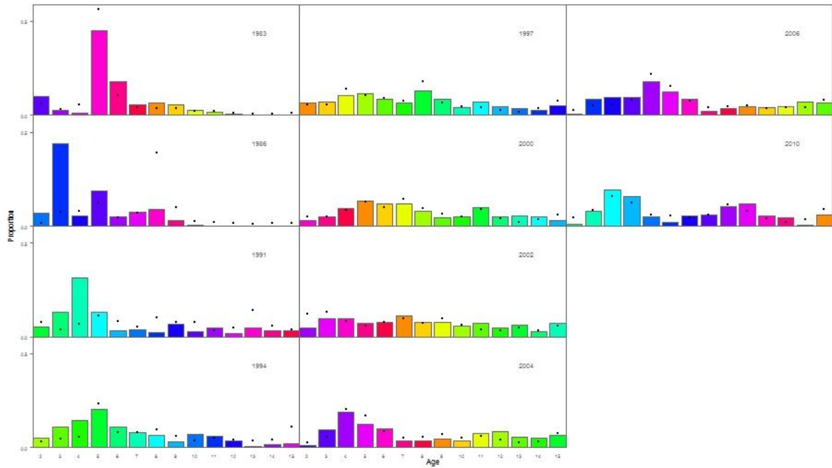
Figure 1A.12. Aleutian Islands pollock reference model fit to NMFS summer bottom trawl survey age composition data. The “•” symbol are the model predictions and columns are the observed proportions at age (with colors corresponding to cohorts).
