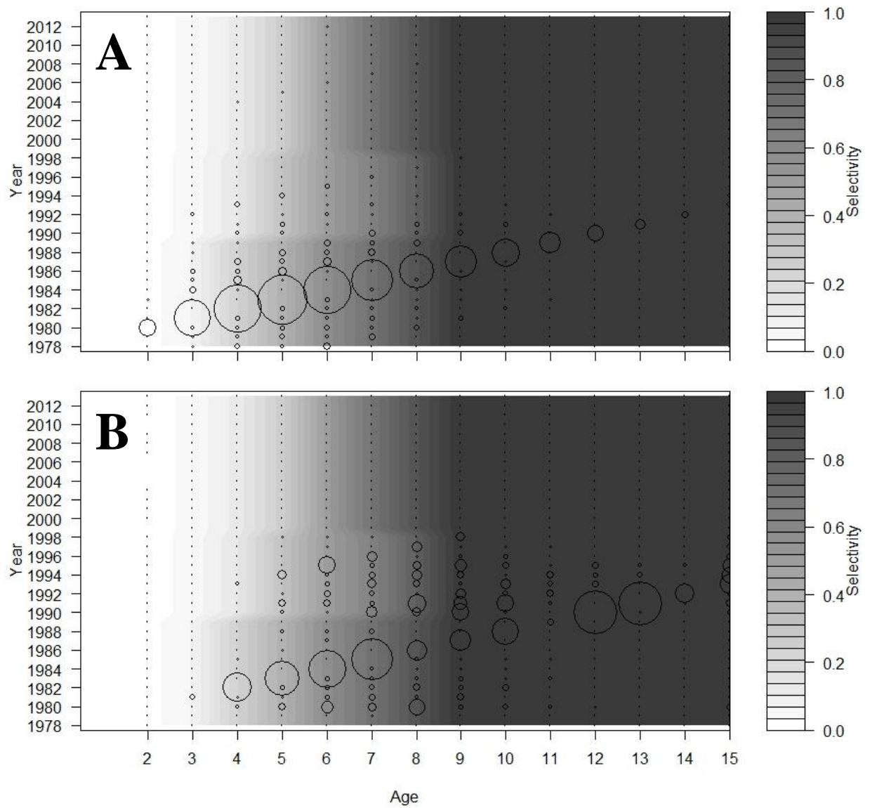
Figure 1A.21 Contour plots of fishery selectivity by age for AI pollock with bubble plots of (A) total biomass at age and (B) catch biomass at age. Total biomass is scaled to 1/20 of the catch biomass bubbles.
