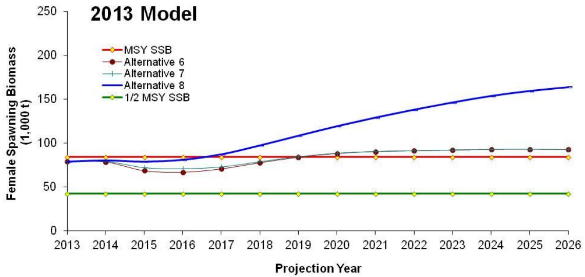
Figure 1A.27 Projected spawning biomass for MSY, \frac{1}{2} MSY, and Alternatives 6, 7, and 8 ABC scenarios from the reference model.
