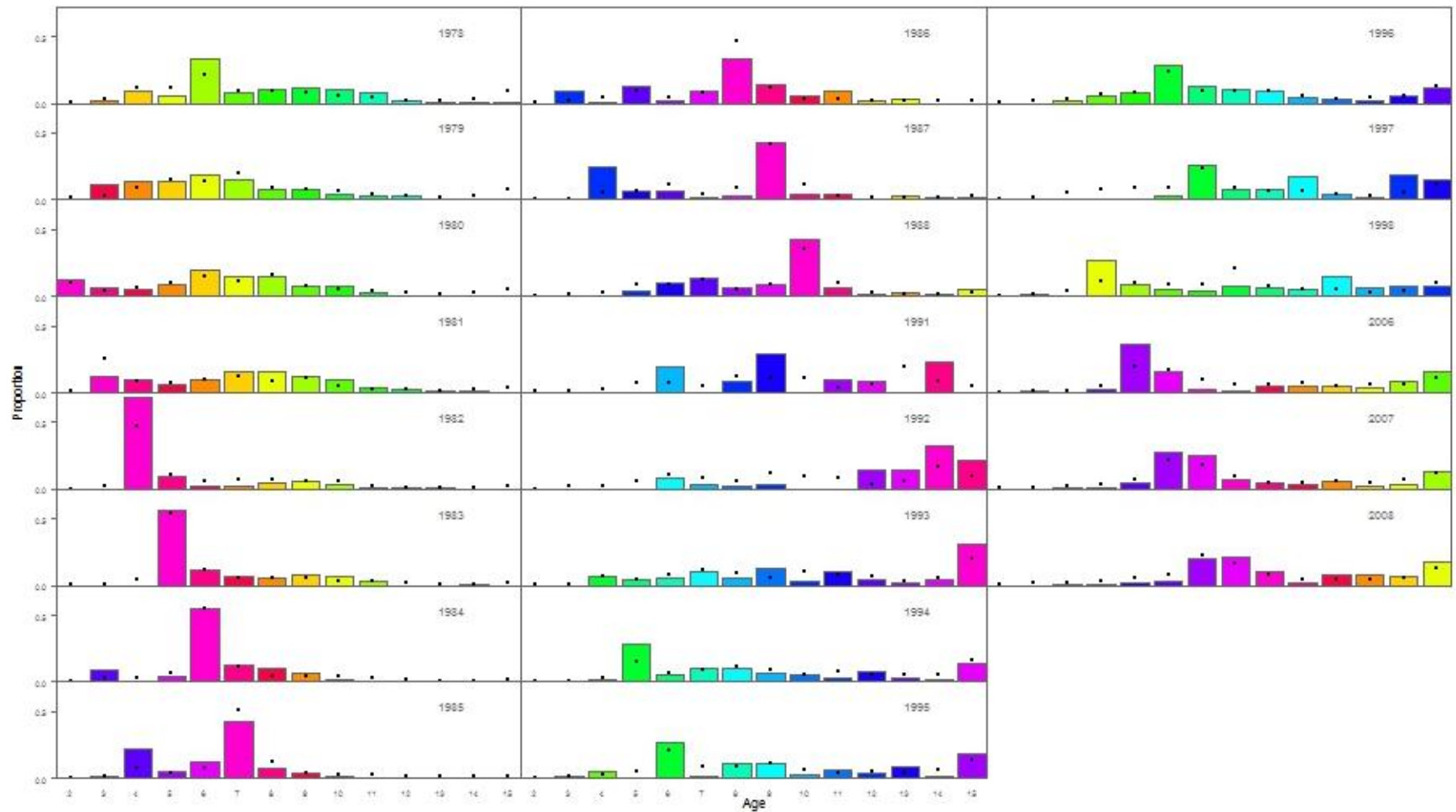
Figure 1A.13. Fit to fishery age composition data for Aleutian Islands pollock. The “•” symbol are the model predictions and columns are the observed proportions at age (with colors corresponding to cohorts).
