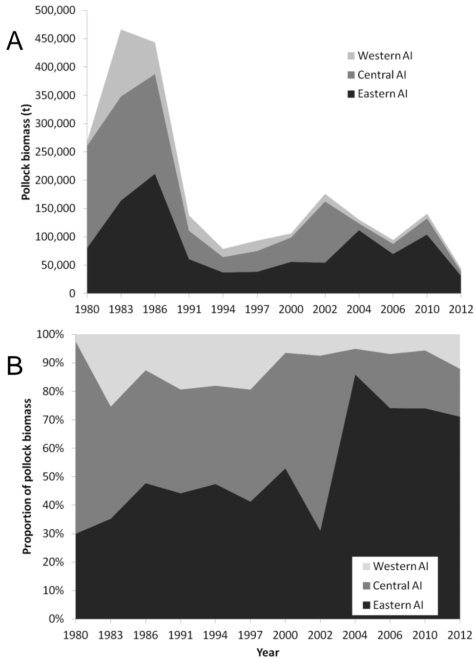
Figure 1A.1 Aleutian Islands bottom trawl survey pollock biomass (A; top) and proportion of biomass (B; bottom) for the three Aleutian Island management regions.
