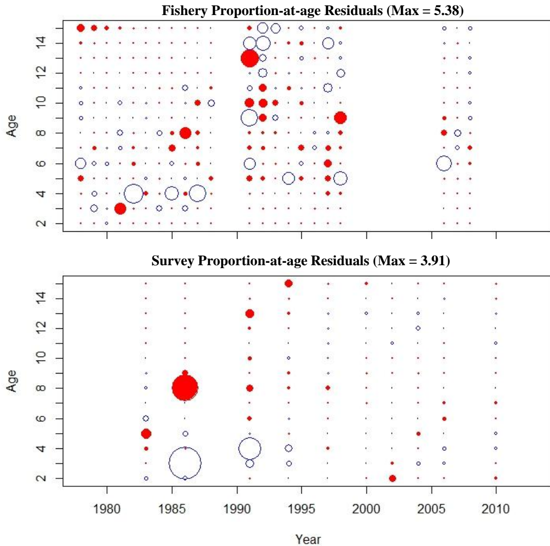
Figure 1A.15. Standardized residuals for fits to the fishery (top) and survey (bottom) proportion-at-age data for the AI pollock reference model.
