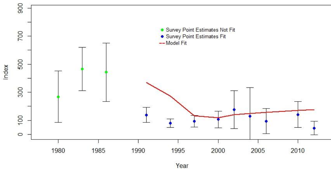
Figure 1A.11. Reference model fit (solid line) to NMFS summer bottom trawl survey (dots).
