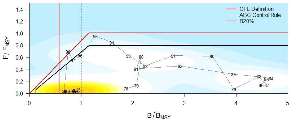
Figure 1A.22. Aleutian Islands pollock spawning biomass relative to B_{msy} and full-selection fishing mortality relative to F_{msy} (1978-2013). The ratio of fishing mortality to F_{msy} is calculated using the estimated selectivity pattern in that year. Color is scaled relative to density of points in the region from high orange to low blue.
