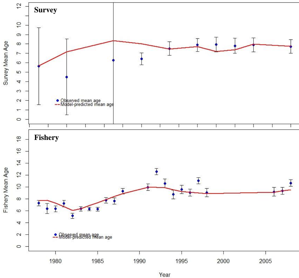
Figure 1A.14. Observed mean age and model derived mean age from the AIBTS (top) and fishery catch at age data (bottom) for the reference model. The confidence intervals are adjusted by the multinomial sample sizes used in reference model.
