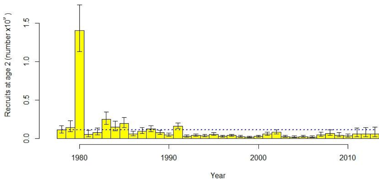
Figure 1A.24. Reference model estimates of Aleutian Islands pollock age 2 recruitment. The vertical bars represent the upper and lower 95% confidence bounds. The dotted line is the 1978-2010 mean age 2 recruitment.
