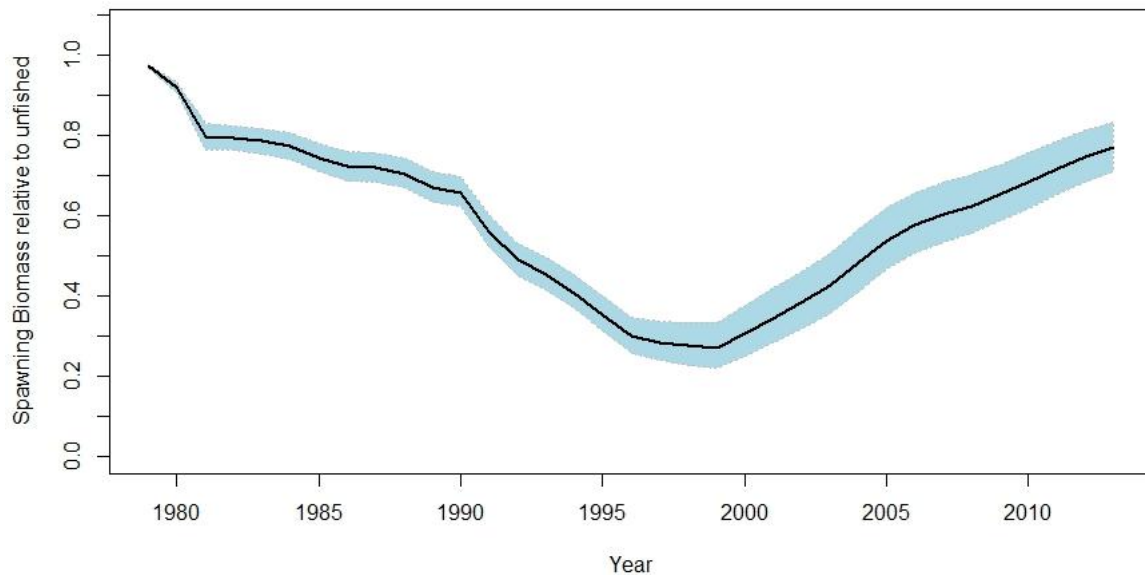
Figure 1A.23. Aleutian Islands pollock ratio of spawning biomass with fishing relative to spawning biomass without fishing for the reference model with 95% confidence interval (shaded).
