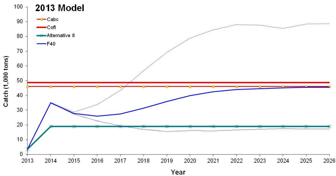
Figure 1A.25 Projected catch for F_{40\%} and Alternative 8 ABC scenarios.
