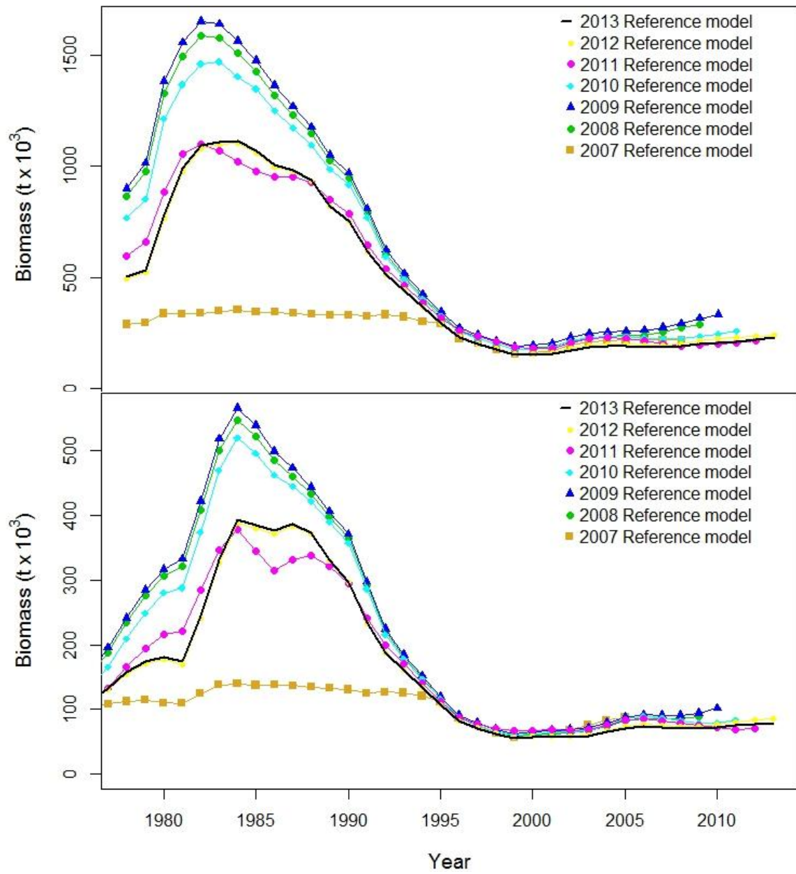
Figure 1A.17. Age 2+ (top) and spawning (bottom) biomass trajectories for the 2012 model compared with the 2007 through 2011 reference models.
