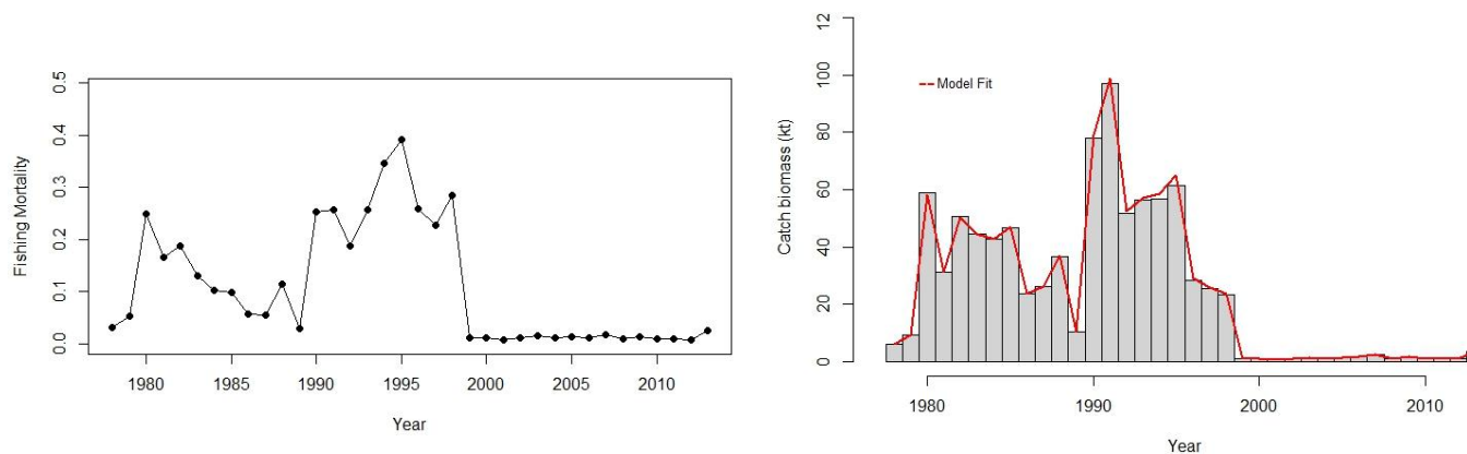
Figure 1A.19 Fishing mortality rates (left) and fits to total catch in 1,000s of tons (right) for AI pollock over time 1978-2012. Fishing mortality rates are based on the average over ages 2-15.
