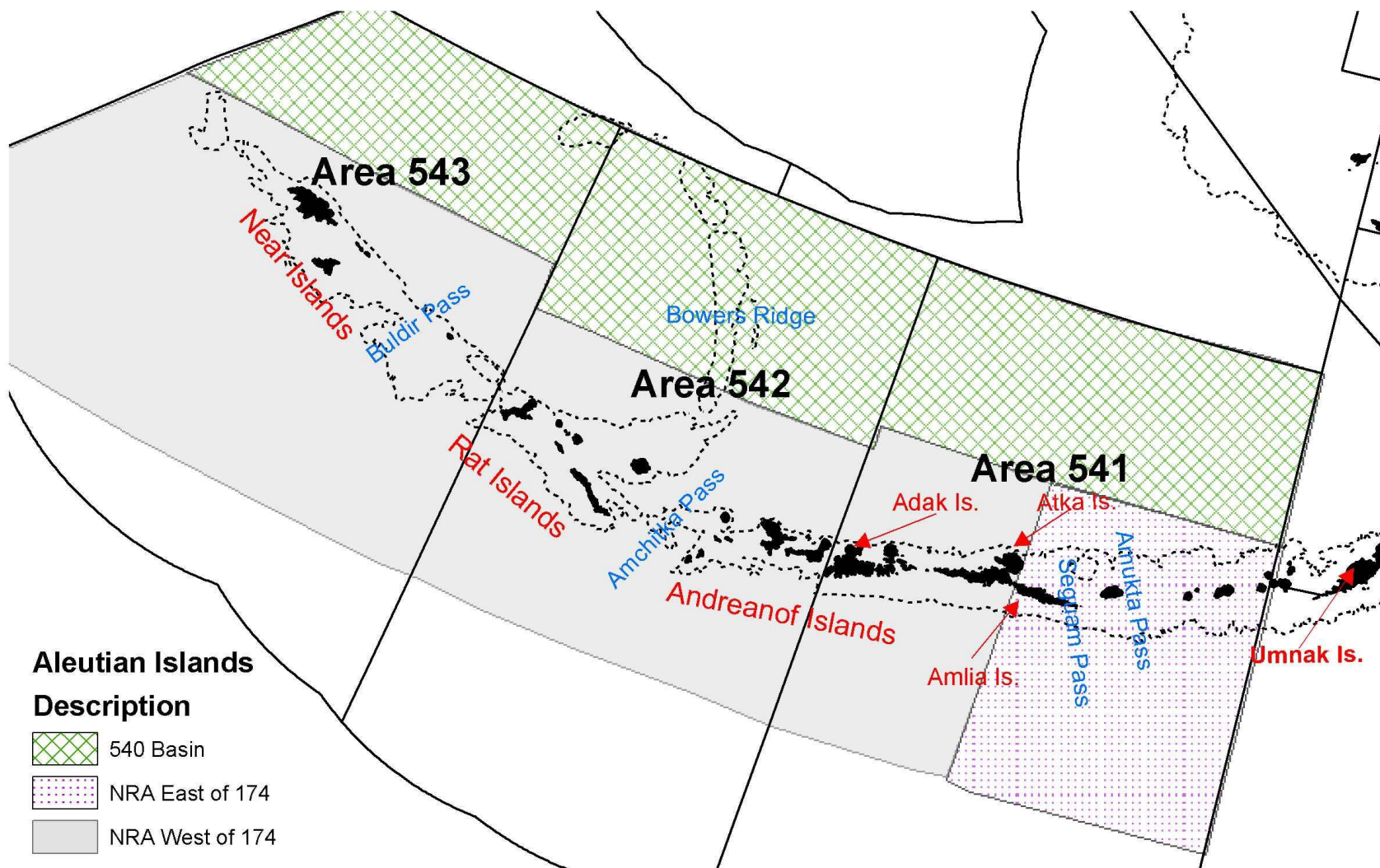
Figure 1A. 3. Regions defined for consideration of alternative data partitions for Aleutian Islands Region pollock. The abbreviation “NRA” represents the Near, Rat, and Andreanof Island group.
