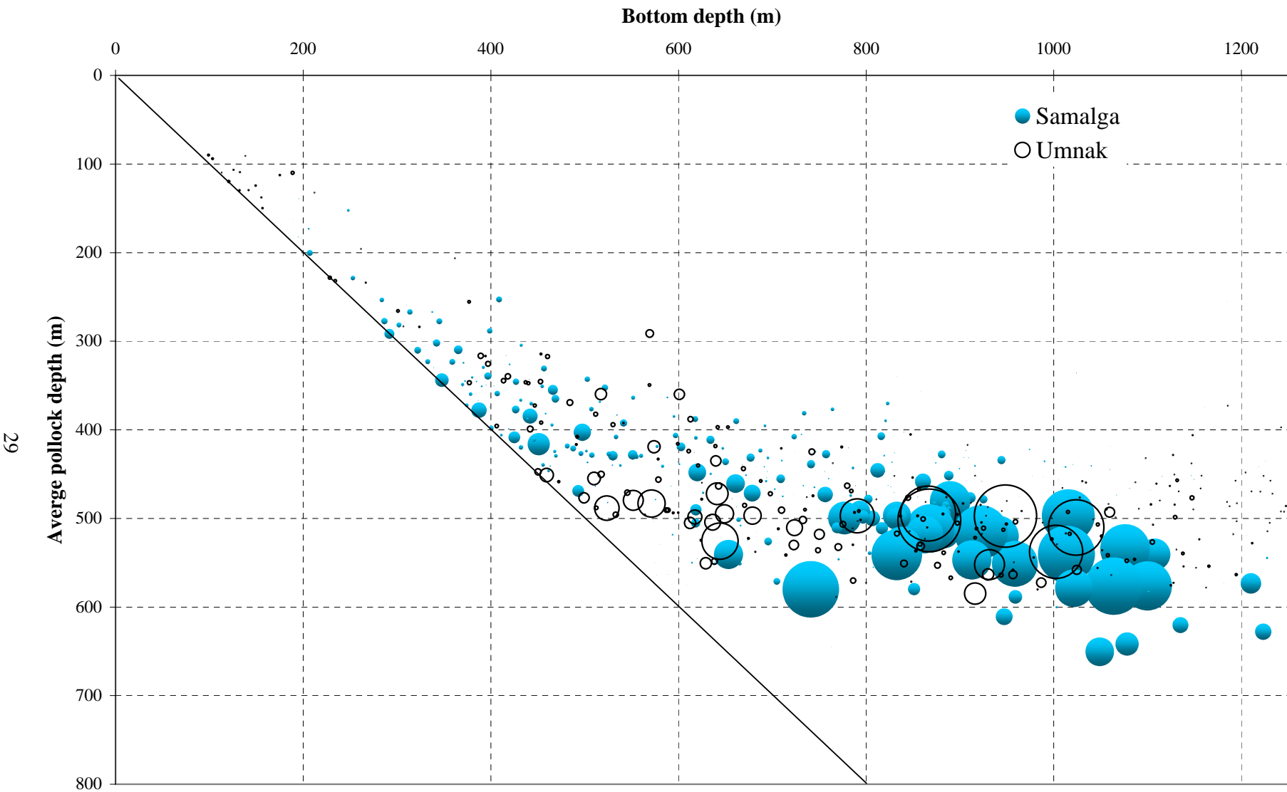
Figure 5.--Average pollock depth (weighted by biomass) versus bottom depth (m), per 0.5 nmi sailed distance for the Umnak and Samalga regions during the winter 2007 echo integration-trawl survey of walleye pollock in the Bogoslof Island area. Bubble size was scaled to the maximum biomass/0.5 nmi interval (Umnak region, 13,710 t). The diagonal line indicates where the average pollock depth equals bottom depth.
