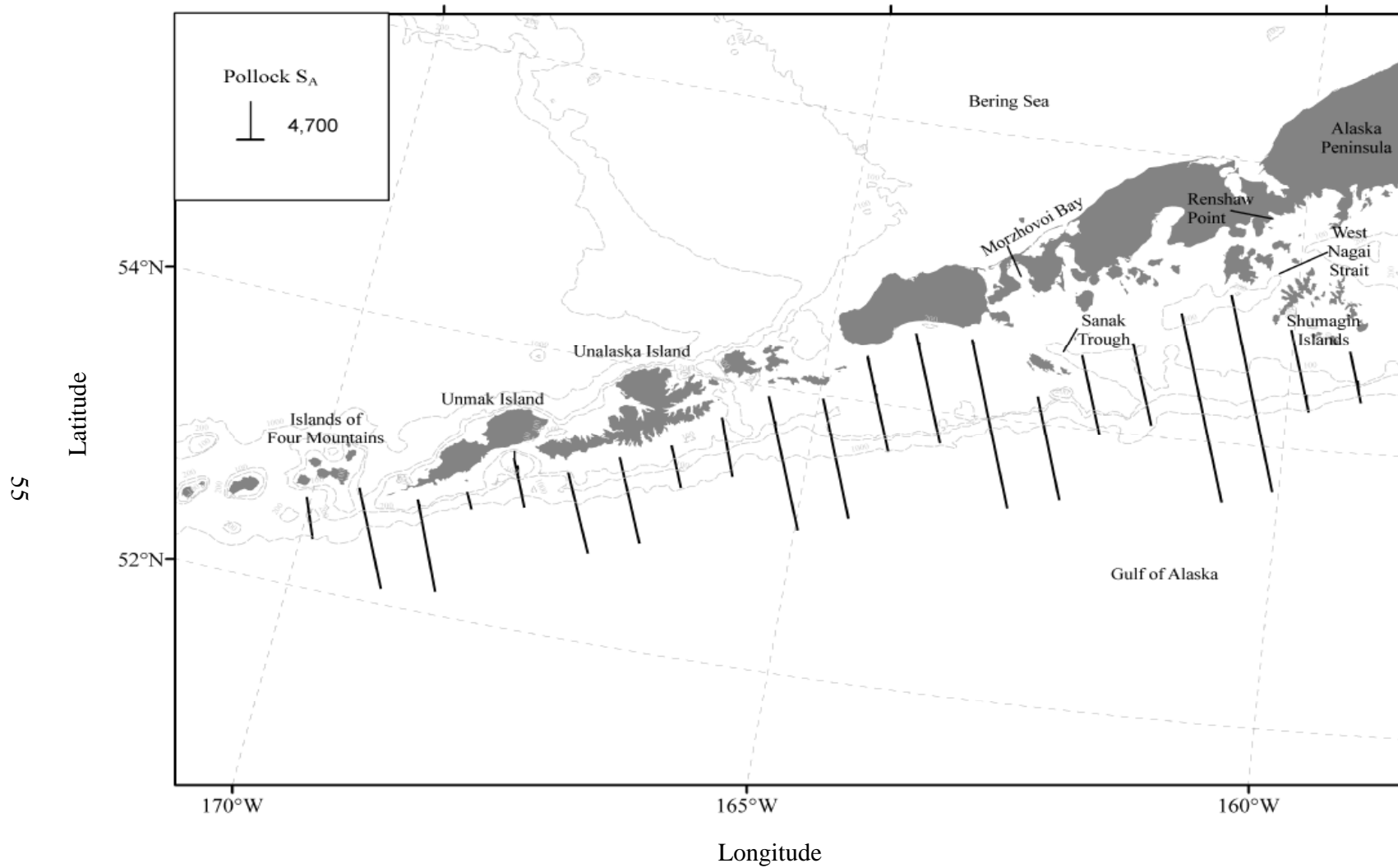
Figure 14.--Acoustic backscattering ( S_A ) attributed to pollock along transects from the summer 2005 echo integration-trawl survey of the Gulf of Alaska.
