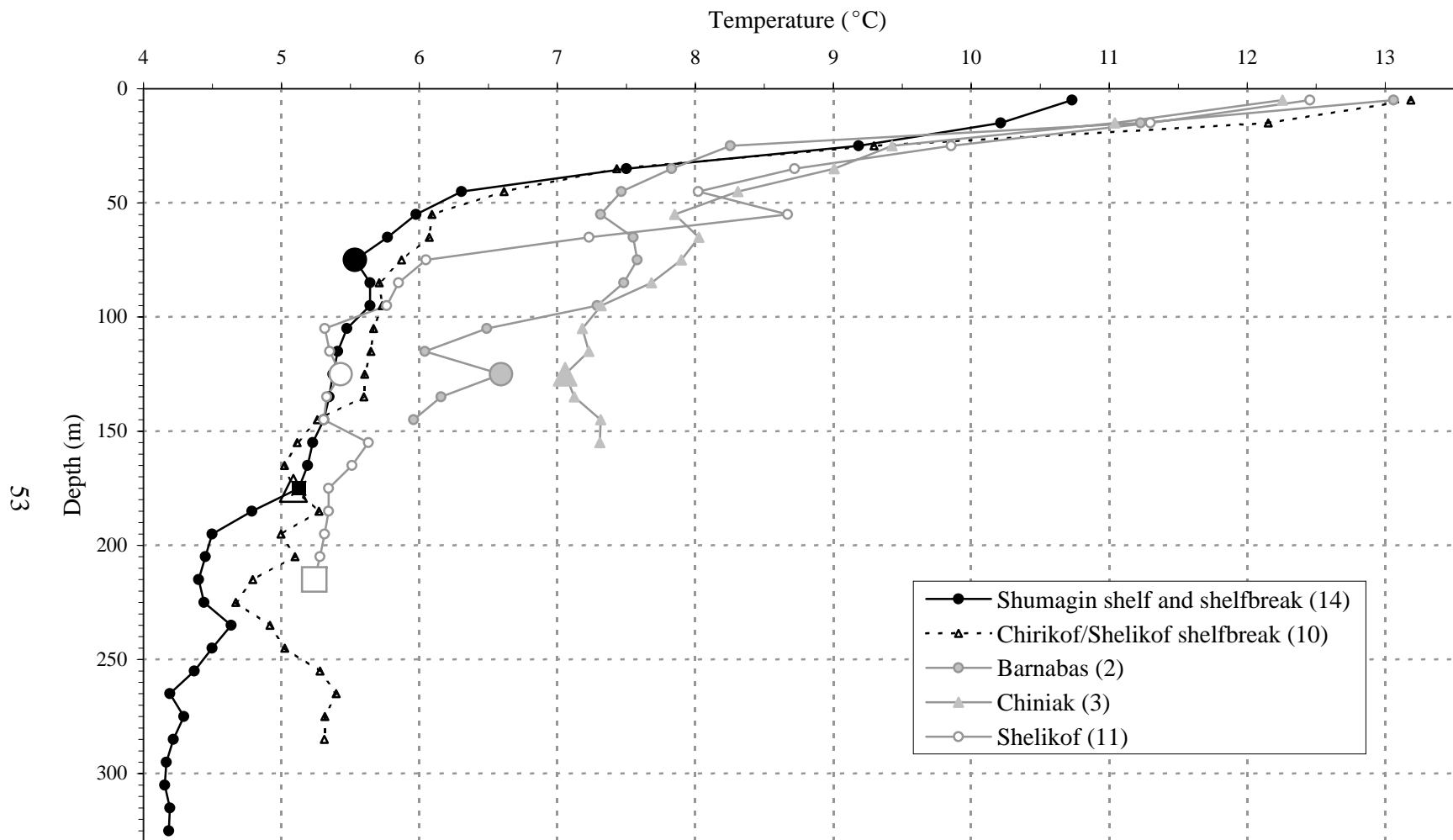
Figure 12.--Average temperature (°C) and number of samples taken by area surveyed during the summer 2005 echo integration-trawl survey of the Gulf of Alaska. The largest symbol for each profile represents the mean depth of pollock biomass in that area. Note: the Shumagin shelfbreak and Shelikof "near-bottom" depth means are represented by squares.
