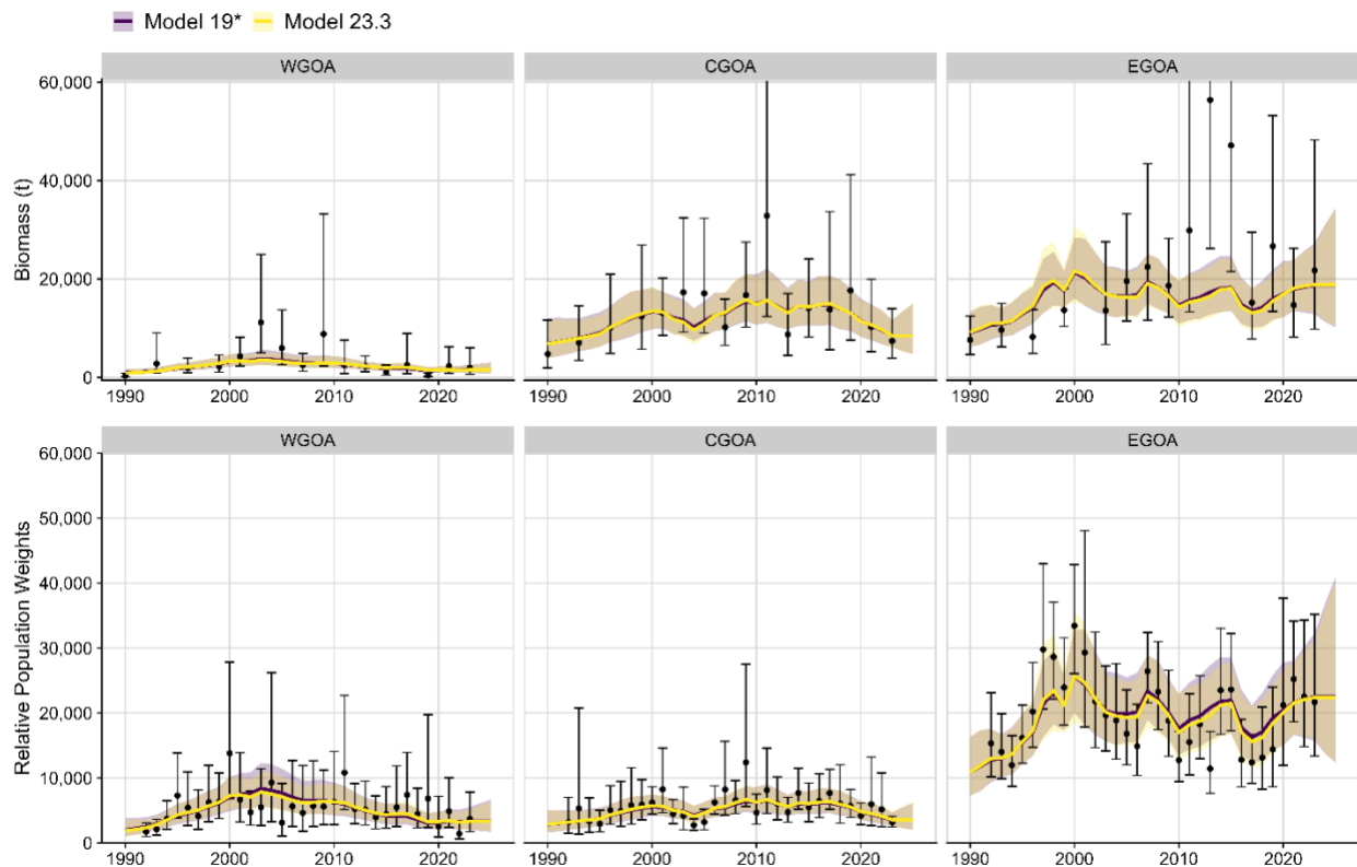
Figure 11-10.--Two-survey random effects (REMA) model fits to Gulf of Alaska (GOA) shortraker rockfish bottom trawl survey (BTS) biomass (top panels) and longline survey (LLS) relative population weights (bottom panels) by western, central, and eastern GOA (WGOA, CGOA, and EGOA) management area, where the points and error bars are the design-based survey estimates and the lines with shaded regions are the model predictions and 95% confidence intervals from the REMA model. Results are shown for Model 19* (LLS weight = 0.5) in purple and Model 23.3 (LLS weight = 1.0 with extra LLS observation error) in yellow.
