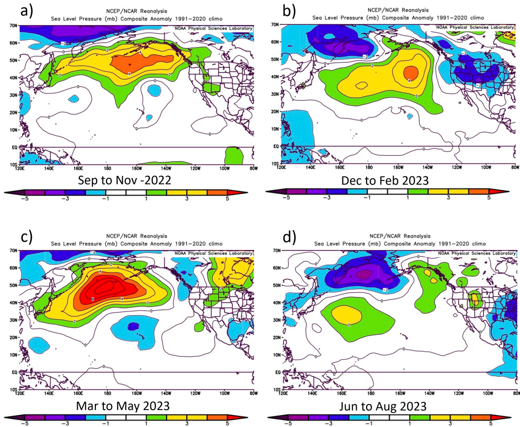
Figure 13: Left, right, top to bottom: SLP composite anomalies (hPa) 1991–2020 climo for a) autumn (September–November 2022), b) winter (December 2022–February 2023), c) spring (March–May 2023), d) summer (June–August 2023)
