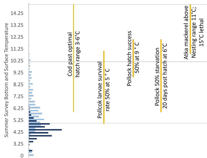
Figure 7: Bottom and surface temperature from biennial summer bottom trawl survey and key temperatures for commercial fish in the Aleutian Islands.
