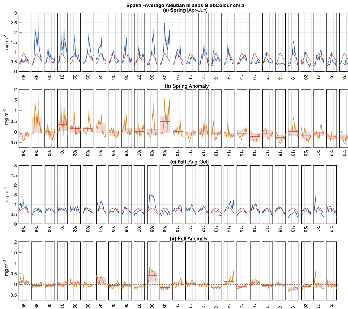
Figure 26: Time series of spatial-average Aleutian Islands chlorophyll a in GlobColour 8-day composites, for the months of (a)-(b) April to June, and (c)-(d) August to October. Panels (a) and (c) show the full time series, while (b) and (d) show anomalies from a composite seasonal cycle (red line in (a)/(c)). In (b) and (d), red line and shading respectively indicate the mean and interquartile range of anomalies in each year. Gray shading indicates (preliminary) 95% confidence bounds. Light gray lines delineate monthly boundaries.
