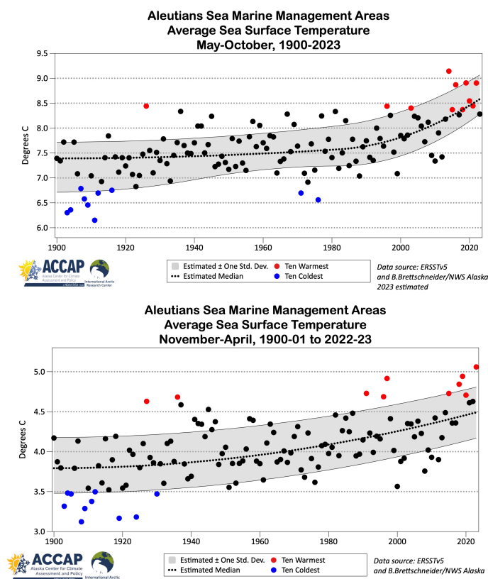
Figure 16: Sea surface temperatures for the Aleutian Islands from 1900–2023 for (a) summer (May–Oct) and (b) winter (Nov–Apr). Presented here are the quantiles representing \pm 1 standard deviation of a Gaussian distribution and for completeness the median calculated using constrained B-Spline regression.
