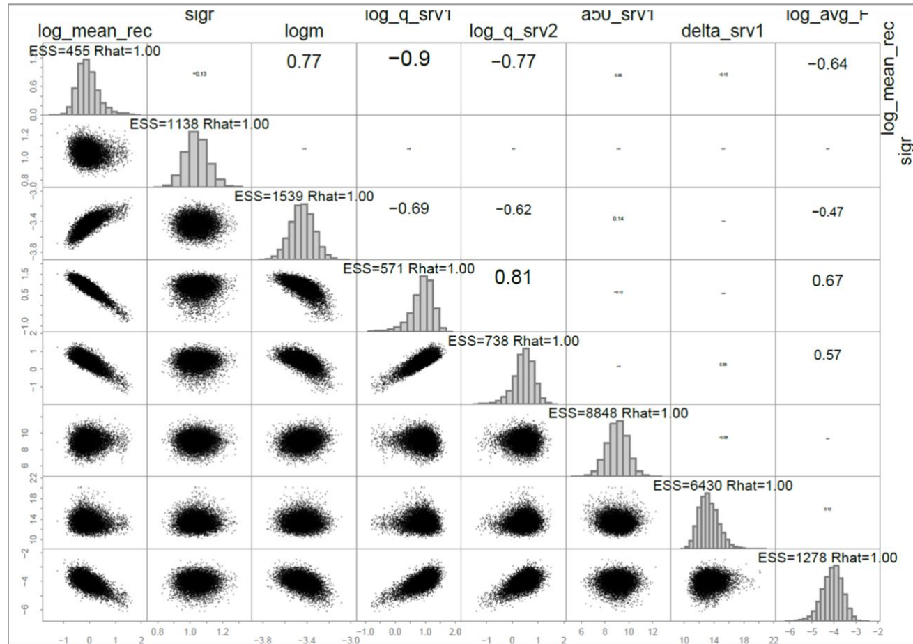
Figure 13-10. Convergence diagnostics and pairwise plots of the MCMC marginal posterior distributions for several key parameters. For brevity, only results for Model 15.4a, Model 23.1, Model 23.1a, and Model 23.1b are shown.
