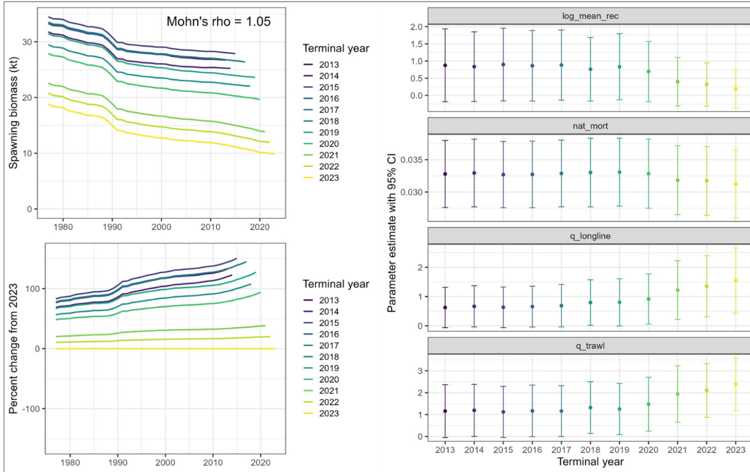
Figure 13-9. Retrospective analysis results for all candidate models, where Model 23.1b is the author-preferred model. For each model, we show the following: (1) retrospective peels of estimated female spawning biomass (top left); (2) percent change from the 2023 model (bottom left) are shown; and (3) parameter estimates with 95% confidence intervals (right) from ten retrospective peels for mean recruitment in log space ( \log\_mean\_rec ), natural mortality ( nat\_mort ), longline survey catchability ( q\_longline ), and bottom trawl survey catchability ( q\_trawl ).
