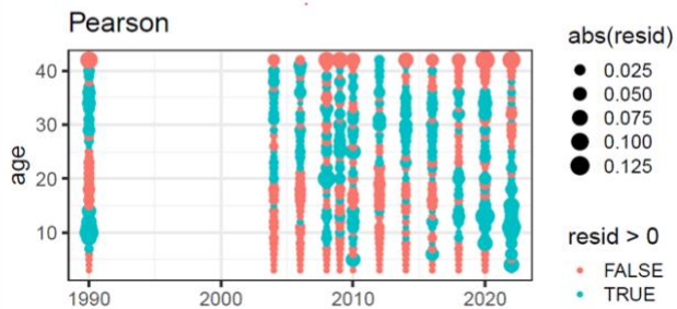
Figure 13-11. A comparison of one-step ahead (OSA) and Pearson residuals for fishery age composition data. The first age bin (age-3) was dropped for the OSA analysis. For brevity, only results for Model 15.4a and Model 23.1b are shown.
