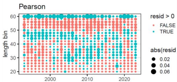
Figure 13-14. A comparison of one-step ahead (OSA) and Pearson residuals for longline survey length composition data in Model 15.4a and Model 23.1b. The first length bin (20 cm) was dropped for the OSA analysis.
