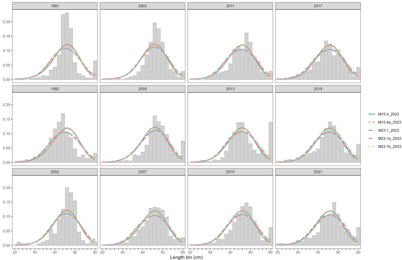
Figure 13-3. Fishery length composition data. Observed = grey bars, predicted from candidate assessment models = colored lines. M23.1b (green dotted lines) is the author-preferred model.
