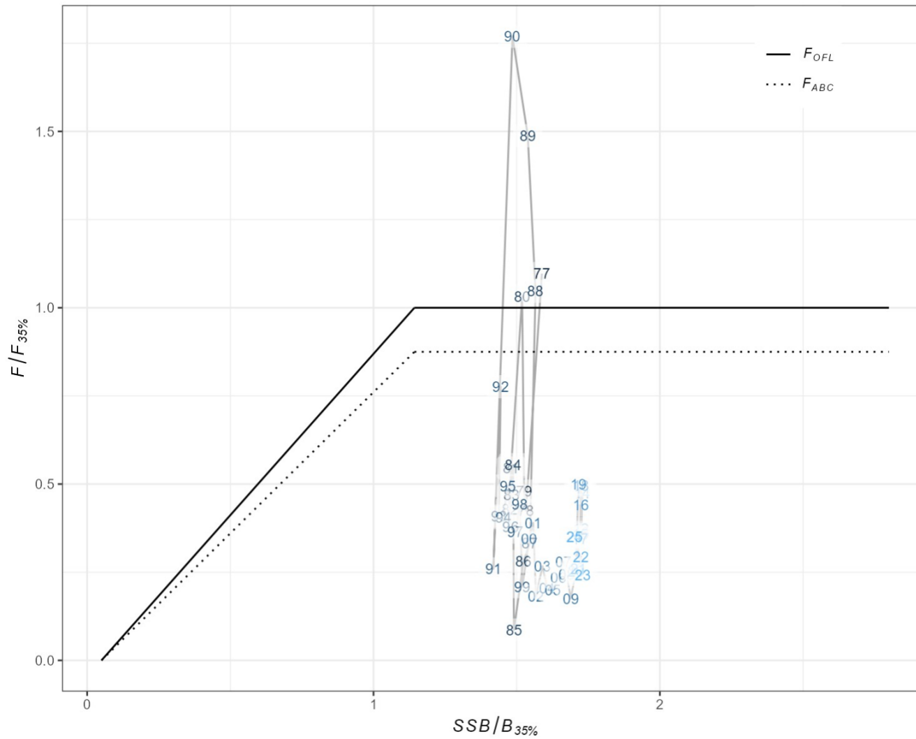
Figure 13-16. Time series of GOA RE/BS rockfish estimated spawning biomass relative to the target B_{35\%} level and fishing mortality relative to F_{OFL} for author-recommended model.
