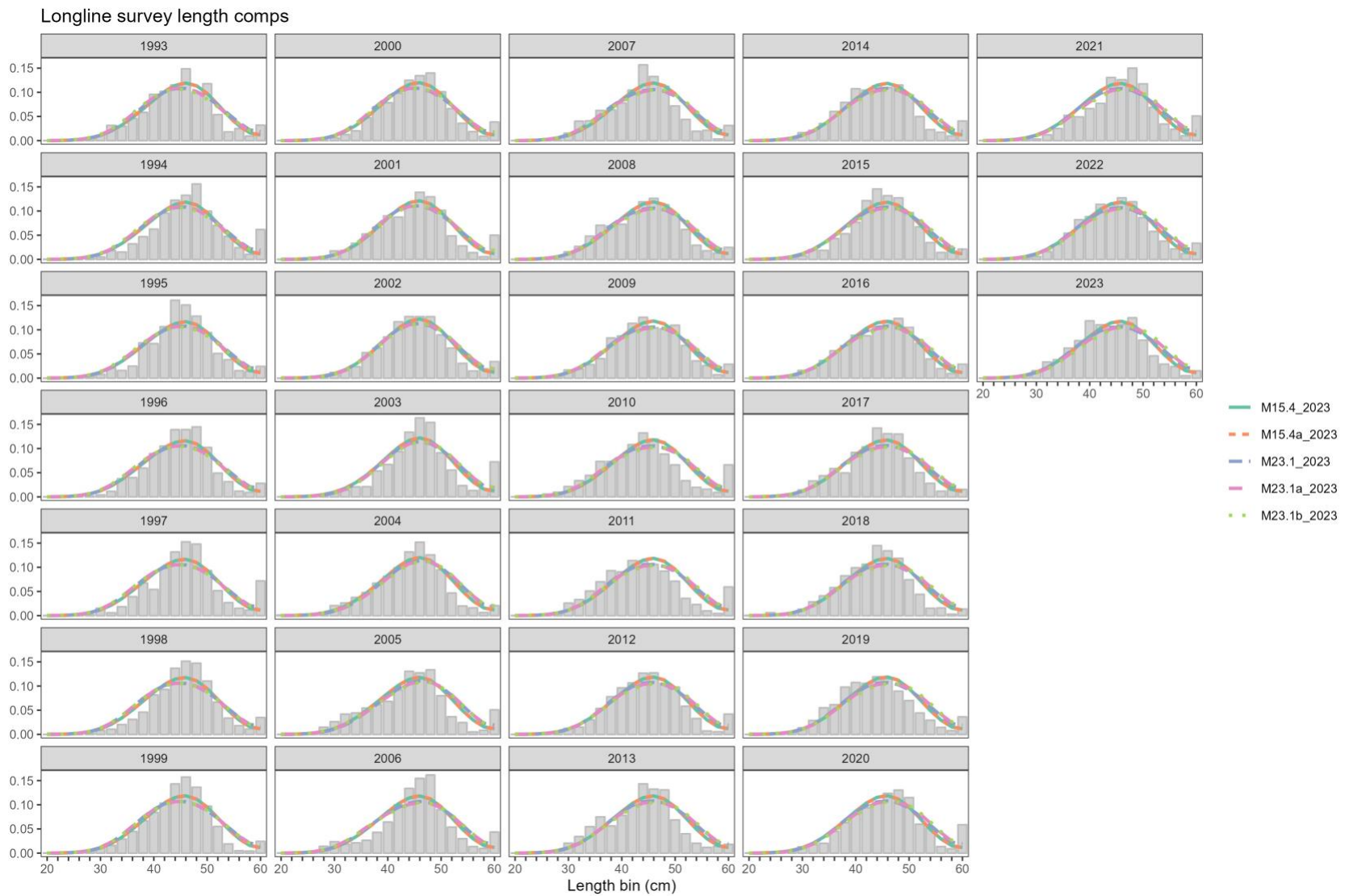
Figure 13-6. Longline survey length composition data. Observed = grey bars, predicted from candidate assessment models = colored lines. M23.1b (green dotted lines) is the author-preferred model.
