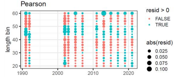
Figure 13-12. A comparison of one-step ahead (OSA) and Pearson residuals for fishery length composition data in Model 15.4a and Model 23.1b. The first length bin (20 cm) was dropped for the OSA analysis.
