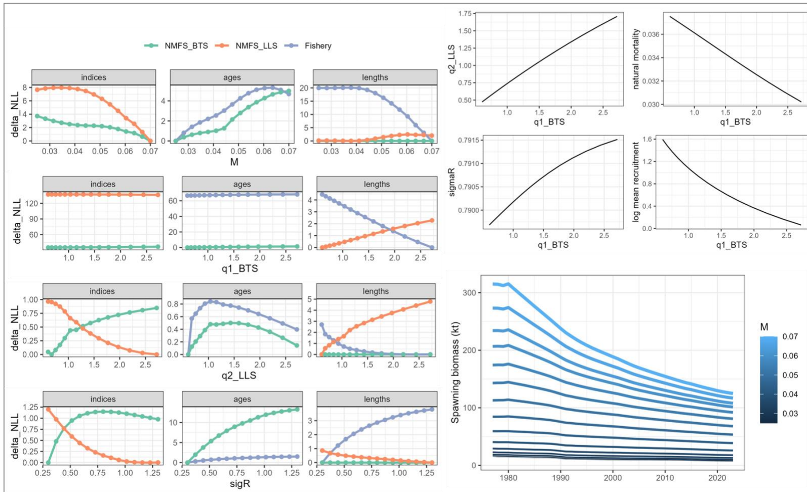
Figure 13-15. Left: Likelihood profiles over natural mortality ( M ), bottom trawl survey catchability ( q1\_BTS ), longline survey catchability ( q2\_LLS ), and recruitment variability ( \text{sigR} ), where the negative log likelihood is separated by data source (BTS=bottom trawl survey, LLS=longline survey, or fishery) and data type (indices, ages, and length). Top right: Parameter estimates of q2\_LLS , natural mortality, \text{sigmaR} , and log mean recruitment when profiling over q1\_BTS . Bottom right: Spawning biomass estimates for the scaling parameter that exhibited the strongest influence on biomass trajectory ( M for Model 15.4a, q1\_BTS for Model 23.1b).
