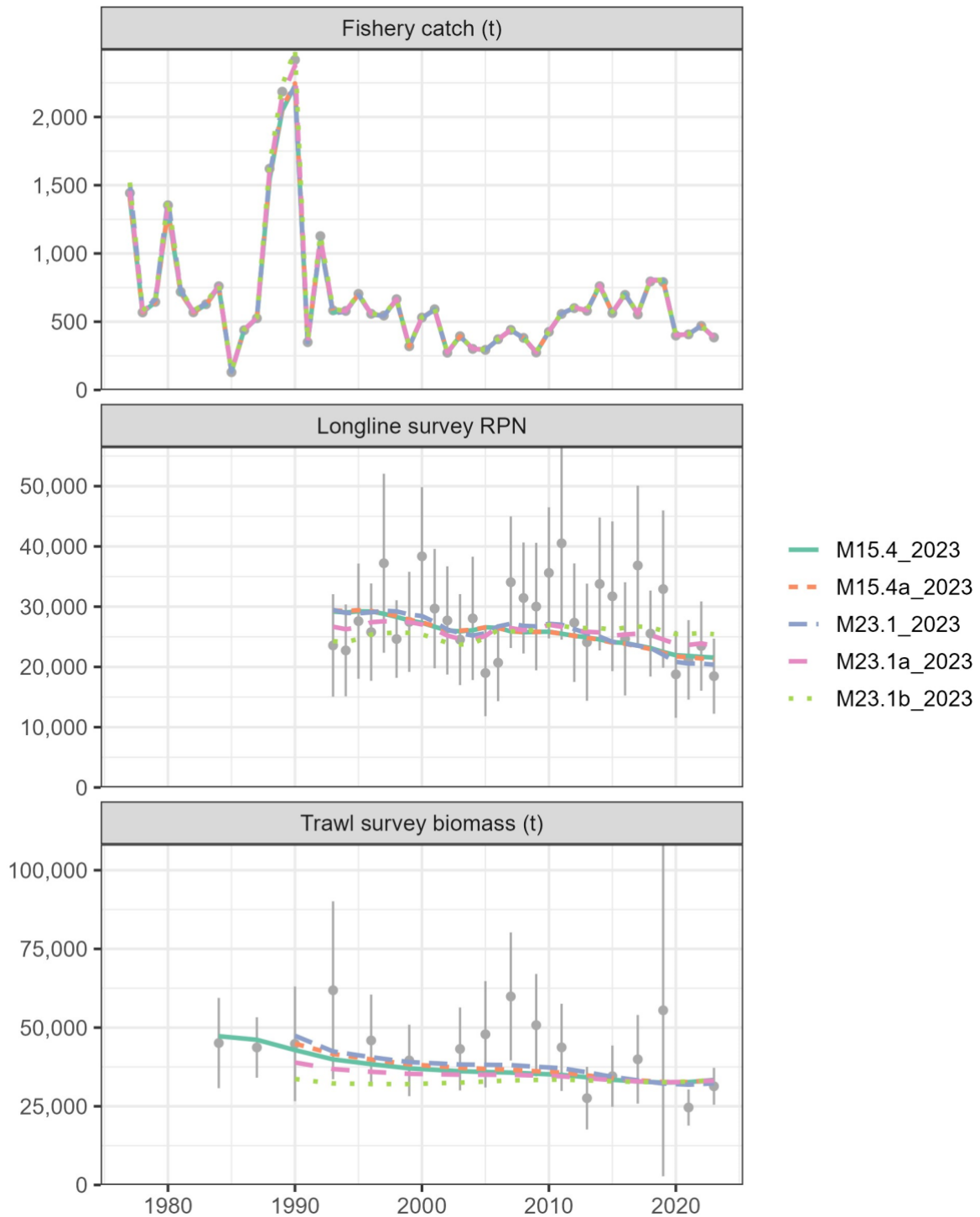
Figure 13-1. Candidate assessment model fits to commercial catch in tons (top), longline survey relative population numbers (RPN; middle), and trawl survey biomass in tons (bottom). Observed = grey points with 95% confidence intervals, predicted from candidate assessment models = colored lines. M23.1b (green dotted lines) is the author-preferred model.
