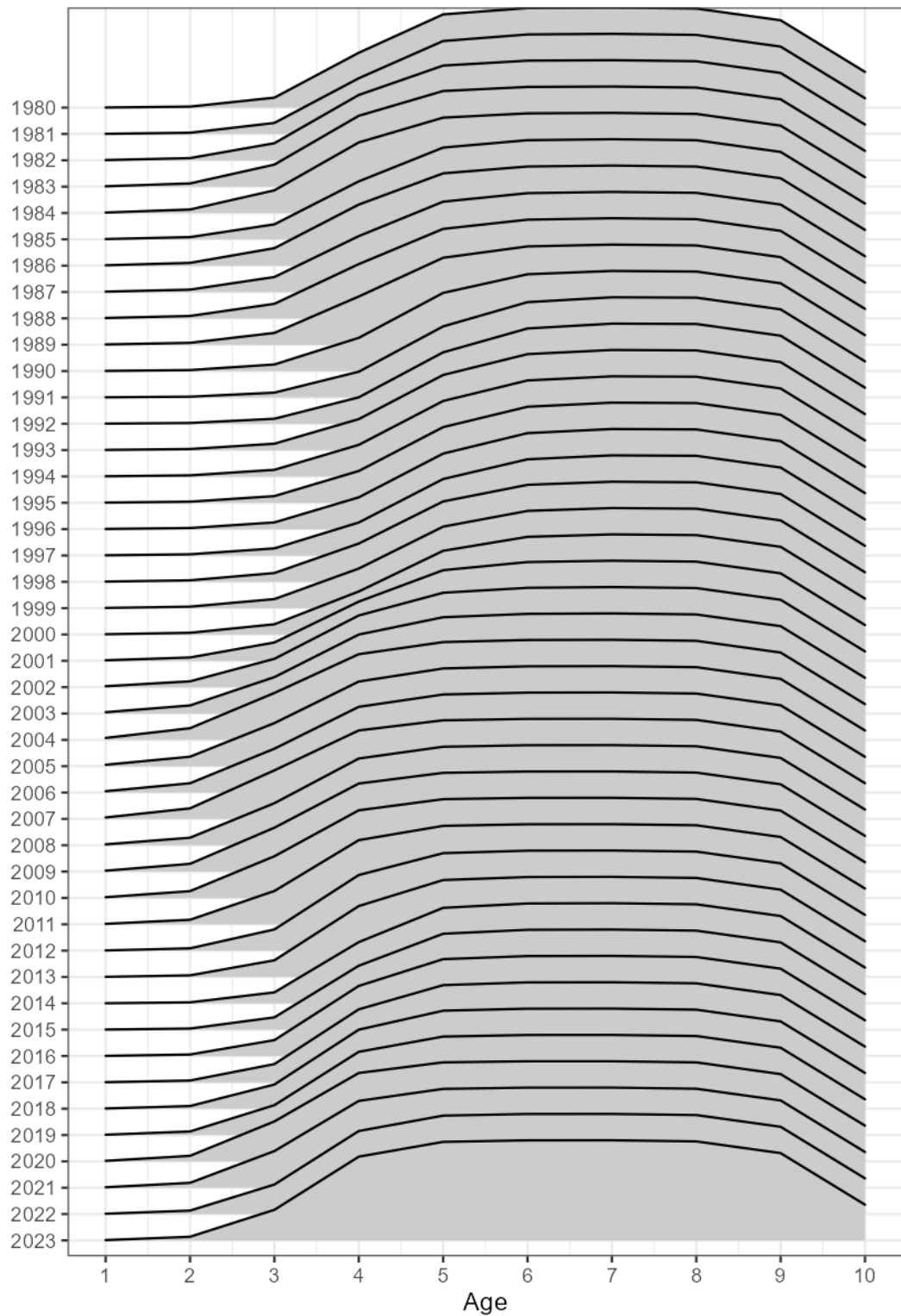
Figure 1.35. Estimates of time-varying double-logistic fishery selectivity for GOA pollock for the base model. The selectivity is scaled so the maximum in each year is 1.0.
