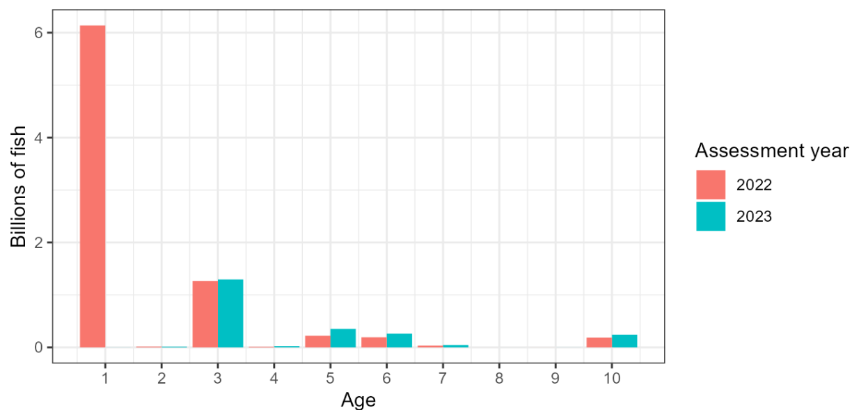
Figure 1.39. The estimated age composition in 2023 from the 2022 and 2023 assessments. The age-1 recruits have no information in the 2022 assessment and so are the average and hence not comparable
