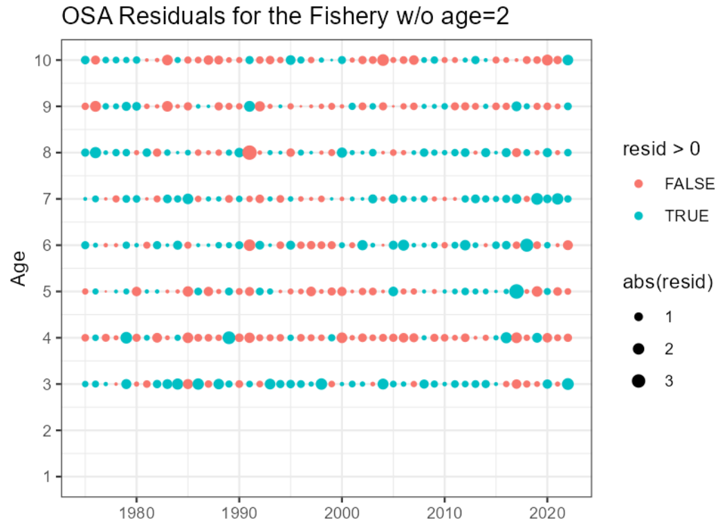
Figure 1.26. OSA residuals for fishery age compositions. Age 1 is combined with age 2 due to lack of data. OSA residuals will be distributed iid standard normal, within and among years, under a correctly specified model and assuming that the first bin fits perfectly. When the absolute residuals are larger than 3 or there are clear correlations or other patterns across ages/years, then the assumption is likely violated and interpreted as model misfit. See Trijoulet et al. (2023) for more information.
