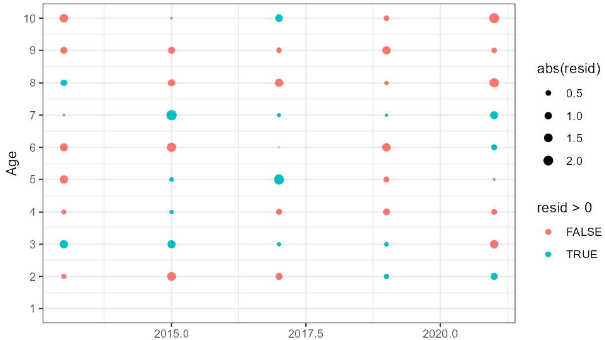
Figure 1.31. Observed and predicted summer acoustic trawl age composition for GOA pollock from the base model (top). Dashed blue lines are observations and solid red lines are model expectations. OSA residuals for the summer acoustic trawl survey (bottom). See caption for figure 1.26 for interpretation of these residuals.
