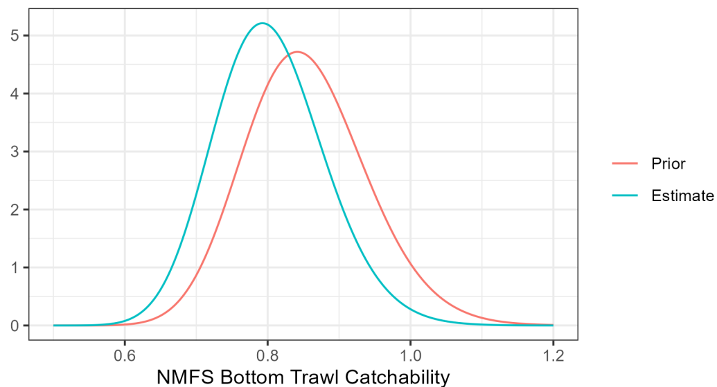
Figure 1.16. Prior on bottom trawl catchability used in the base model, and the estimate and uncertainty from the base model.
