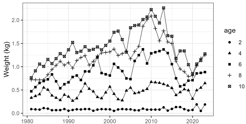
Figure 1.21. Estimated weight at age of GOA pollock (ages 2, 4, 6, 8, and 10) from Shelikof Strait acoustic surveys used in the assessment model. In 1999 and 2011, when the acoustic survey was not conducted, weights-at-age were interpolated from surveys in adjacent years.
