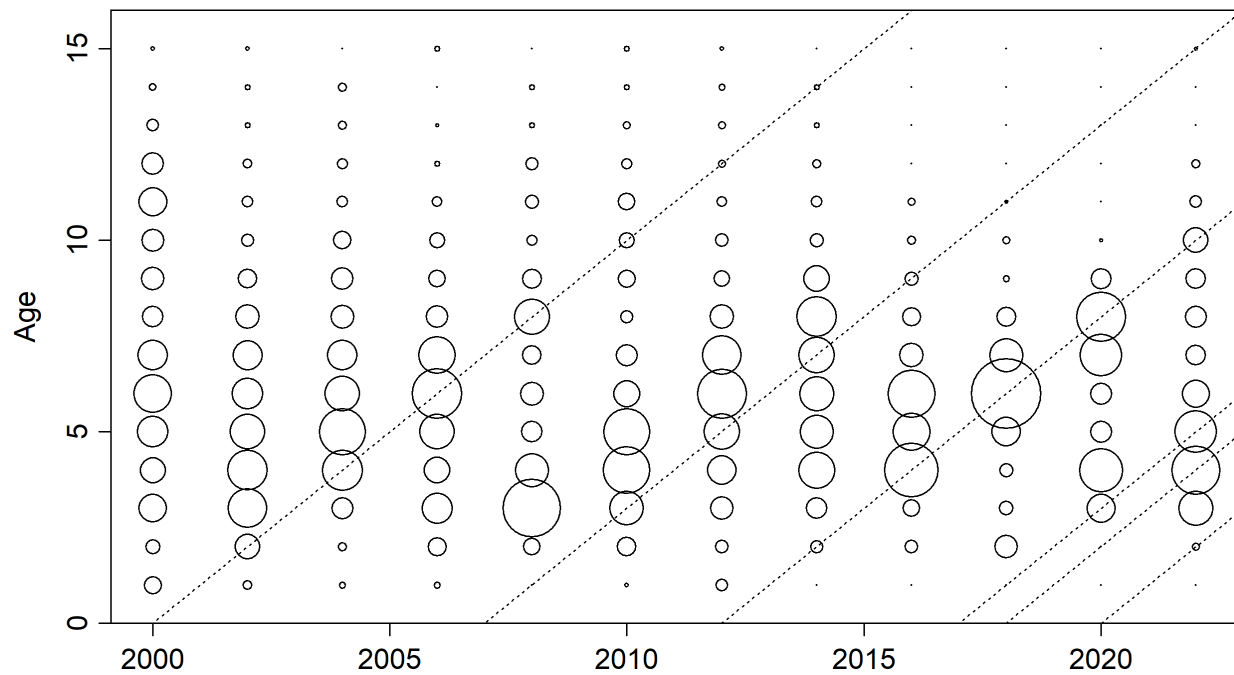
Figure 1.13. Estimated proportions at age in the ADF&G crab/groundfish survey (2000-2022). The area of the circle is proportional to the estimated abundance.
