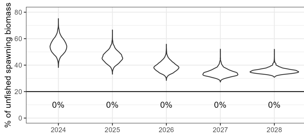
Figure 1.43. Uncertainty in spawning biomass in 2024-2028 based on a posterior samples from MCMC from the joint likelihood for the base model where catch is set to the maximum permissible FABC. Shown are the percentage below the horizontal line at 20% for each year.
