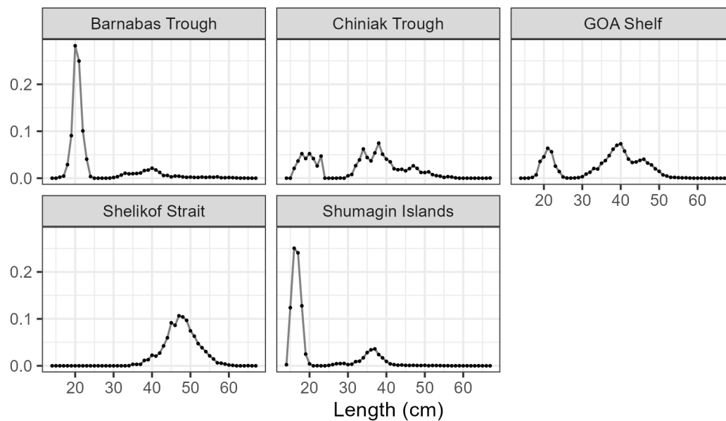
Figure 1.10. Length composition of pollock by survey area for the 2023 summer acoustic survey.
