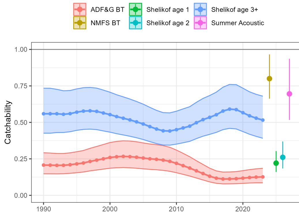
Figure 1.24. Time-varying catchability for the Shelikof Strait acoustic survey (Survey 1), the ADF&G crab/groundfish trawl survey (Survey 3), and constant catchability for the NMFS bottom trawl (Survey 2) and the age-1 and age-2 Shelikof indices (Surveys 4 and 5; representing selectivity), and for the summer NMFS acoustic survey (Survey 6), for model 19.1a. Ribbons and lines represent the 95% CI
