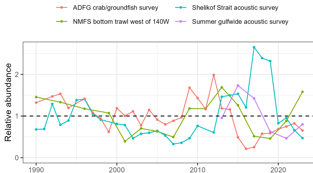
Figure 1.14. Relative trends in pollock biomass since 1990 for the Shelikof Strait acoustic survey, the NMFS bottom trawl survey, and the ADF&G crab/groundfish trawl survey. Each survey biomass estimate is standardized to the average since 1990. Shelikof Strait acoustic surveys prior to 2008 were re-scaled to be comparable to the surveys conducted from 2008 onwards by the R/V Oscar Dyson.
