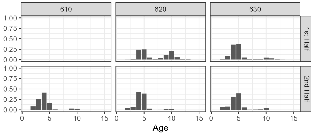
Figure 1.3. Distribution of pollock catch at age in the 2022 separated by season and area.
