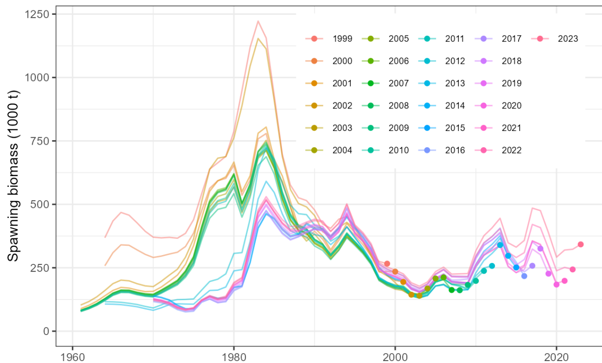
Figure 1.38. Estimated female spawning biomass for historical stock assessments conducted between 1999-2023. Lines represent the estimate in the assessment year and point is the terminal estimate in that year.
