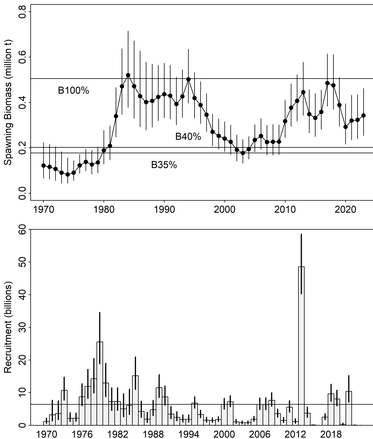
Figure 1.36. Estimated time series of GOA pollock spawning biomass (top) and age 1 recruitment (bottom) for the base model, with horizontal line at the average from 1978-2022. Vertical bars represent two standard deviations. The B35% and B40% lines represent the current estimate of these benchmarks.
