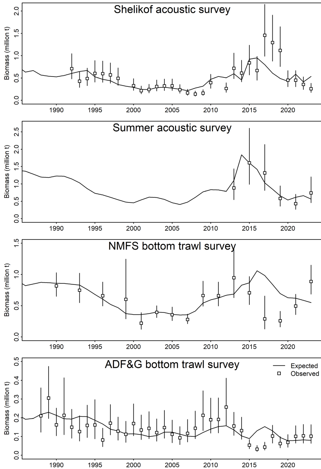
Figure 1.32. Model predicted (line) and observed survey biomass (points and 95% confidence intervals) for the four surveys. The winter Shelikof survey (top panel) is only for ages 3+.
