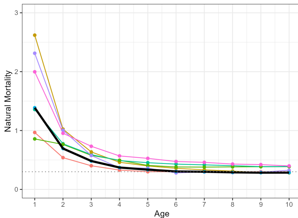
Figure 1.17. Alternative estimates of age-specific natural mortality. The scaled average was used in the stock assessment model. See table 1.14 for more information
