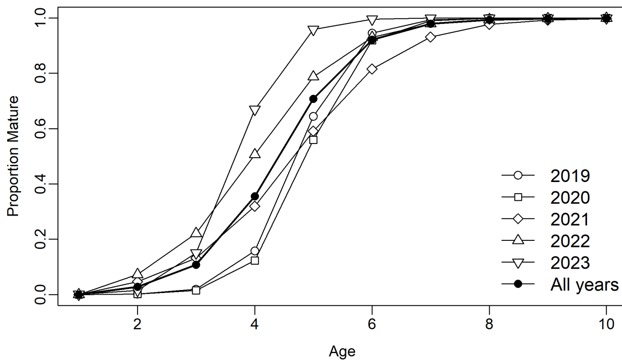
Figure 1.19. Estimates of the proportion mature at age from weighted visual maturity data collected during 2019-2023 winter acoustic surveys in the Gulf of Alaska and long-term average proportion mature at age (1983-2023). Maturity for age-1 fish is assumed to be zero.
