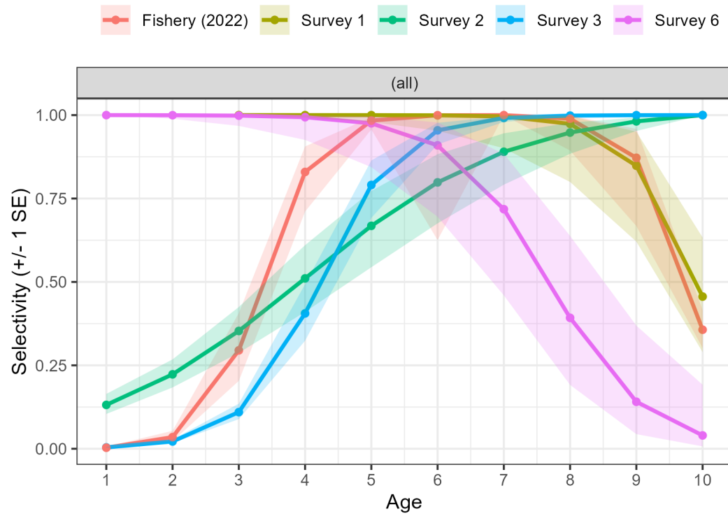
Figure 1.34. Estimated selectivity at age (lines) and uncertainty ( \pm 1 SE; ribbons) for the fishery and surveys. Uncertainty calculations are done in logit space then converted and hence are asymmetric.
