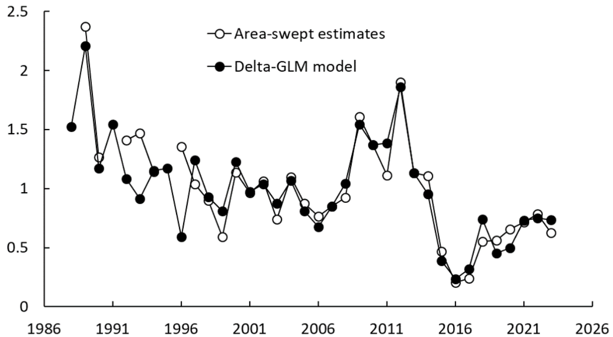
Figure 1.12. Comparison of ADF&G crab/groundfish trawl area-swept indices with year indices for a delta GLM model with a gamma error assumption for the positive observations. Both time series have been scaled by the mean for the time series.
