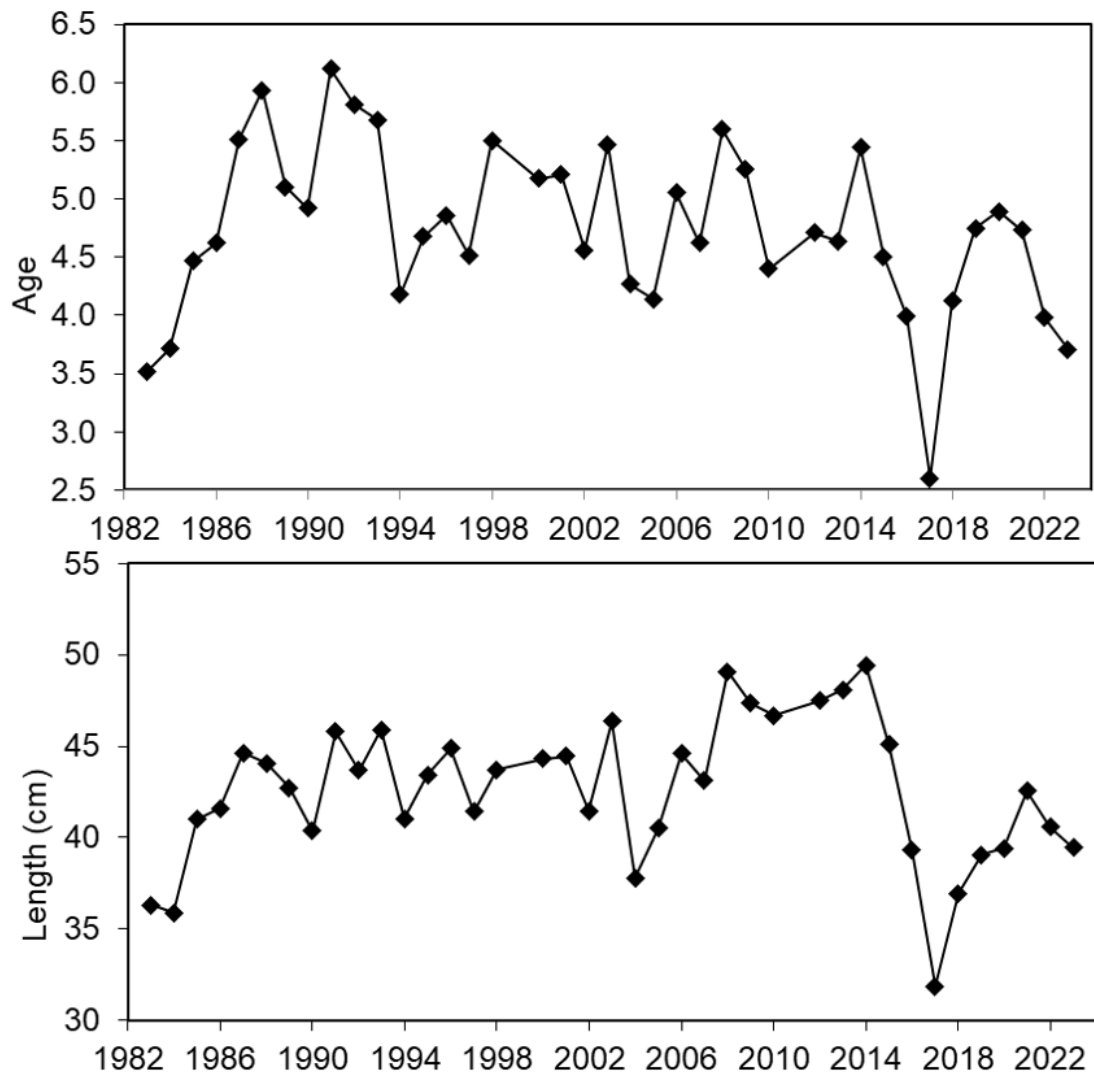
Figure 1.20. Age at 50% mature (top) and length at 50% mature (bottom) from annual logistic regressions for female pollock from winter acoustic survey data in the Gulf of Alaska. Estimates since 2003 are weighted by local abundance.
