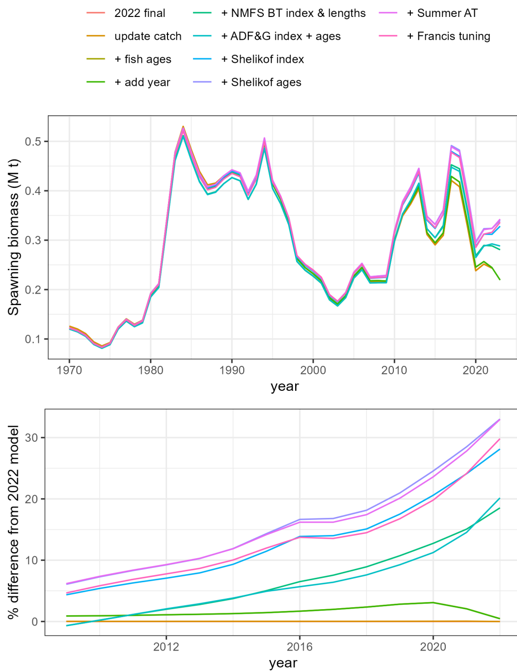
Figure 1.23. Changes in estimated spawning biomass as new data were added successively to last year's base model, ordered by row in the legend at the top. The lower panel shows recent years with an expanded scale to highlight differences.
