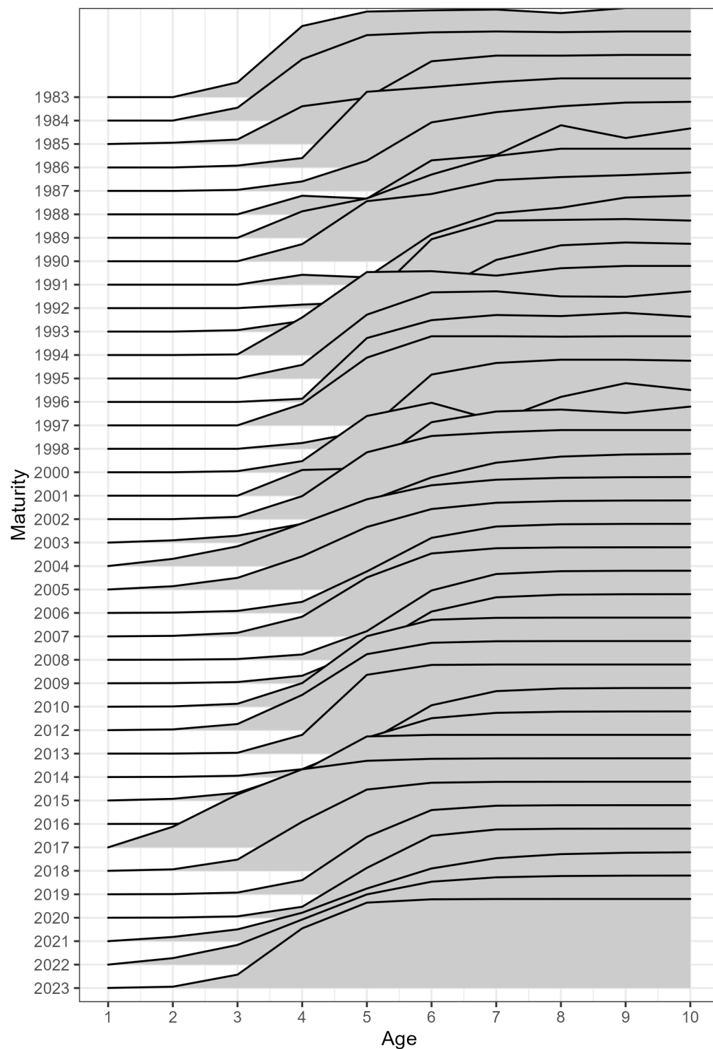
Figure 1.18. Estimates of the proportion mature at age from weighted visual maturity data collected on winter acoustic surveys in the Gulf of Alaska for all years. Maturity for age-1 fish is assumed to be zero.
