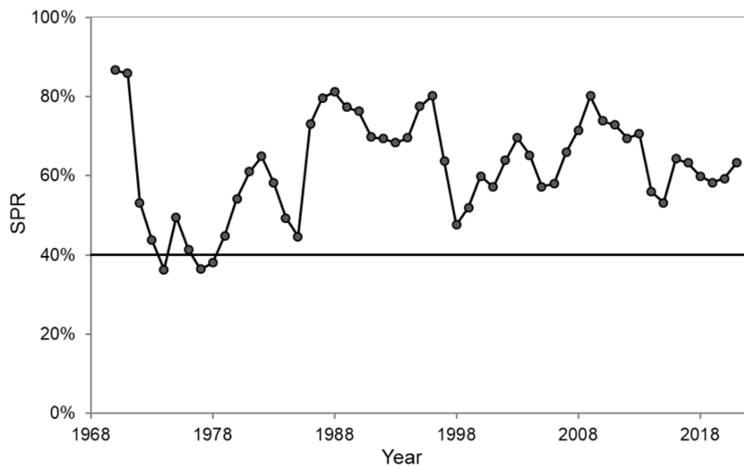
Figure 1.37. Annual fishing mortality as measured in percentage of unfished spawning biomass per recruit (top). GOA pollock spawning biomass relative to the unfished level and fishing mortality relative to F_{MSY} (bottom). The ratio of fishing mortality to F_{MSY} is calculated using the estimated selectivity pattern in that year. Estimates of B_{100\%} spawning biomass are based on current estimates of maturity at age, weight at age, and mean recruitment. Because these estimates change as new data become available, this figure can only be used in a general way to evaluate management performance relative to biomass and fishing mortality reference levels.
