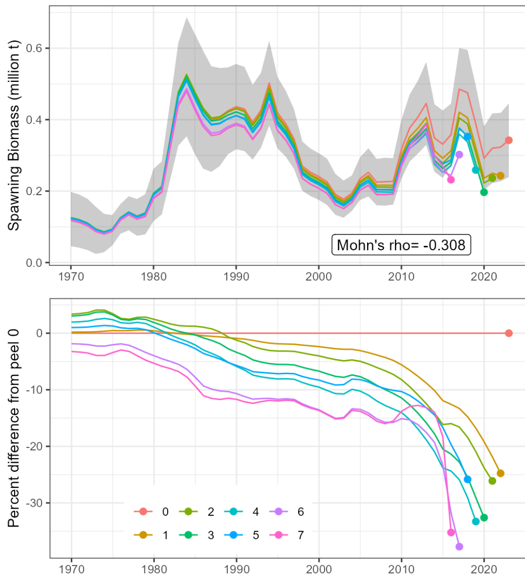
Figure 1.40. Retrospective plot of spawning biomass for models ending in years 2016-2022 for the 2023 base model. The revised Mohn's rho (Mohn 1999) for ending year spawning biomass is -0.308.
