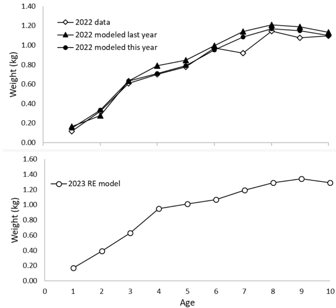
Figure 1.22. Comparison of fishery weight at age for 2022 with estimates from the random effects model last year and this year's assessment (top panel). Random effects model estimates for 2023 used in the assessment model and for yield projections (bottom panel).
