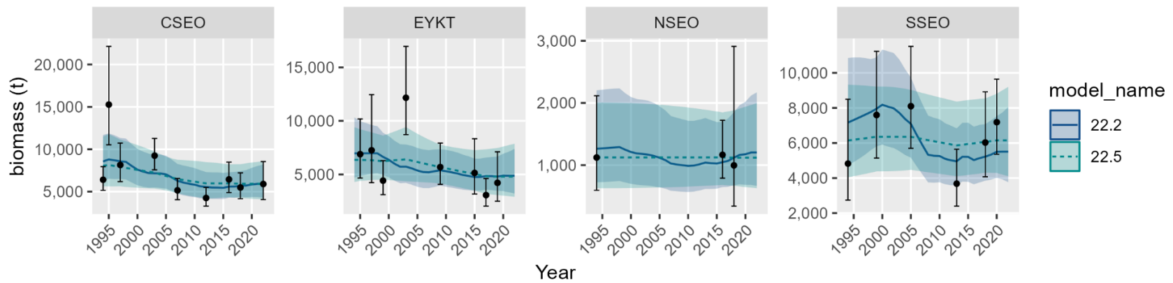
Figure 14.12.—Comparisons of biomass estimates from random effect models with (22.1 and 22.2) and without the inclusion of IPHC longline CPUE indices of abundance (22.4 and 22.5). Models 22.1 and 22.4 include no extra variance term for biomass estimates (A) while models 22.2 and 22.5 include an extra variance term for biomass estimates (B).
