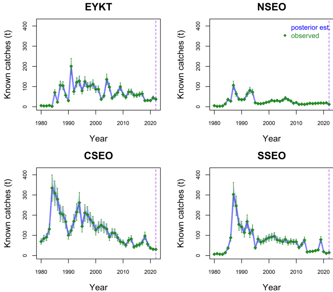
Figure 14.A7. Estimates of yelloweye rockfish known catches from the Stage-1 SS-SPM in the four management units in the Southeast Outside subdistrict (SEO) of the Gulf of Alaska (blue line with 50 and 95% credibility interval polygons) and the catch estimates from reported harvests (green diamonds with 95% confidence interval error bars).
