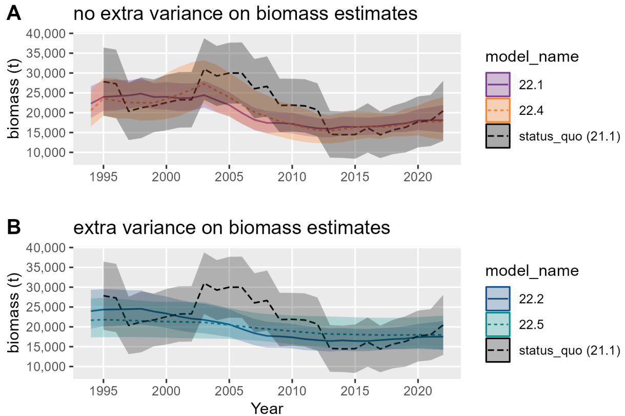
Figure 14.1.—Total Southeast Outside (SEO) yelloweye rockfish biomass (t) with 95% confidence intervals from the five alternative models, 1994–2022. Model 21.1 uses status-quo methods with revised values calculated directly from published density estimates, Model 22.1 uses the two-survey random effects (REMA) model, Model 22.2 is Model 22.1 but estimates additional observation error for the biomass data, Model 22.4 is the same as Model 22.1 but without the inclusion of IPHC longline survey CPUE, and Model 22.5 is the same as Model 22.2 but without the inclusion of IPHC longline survey CPUE. Models without extra variance on the biomass estimates (Model 22.1 and 22.4) are in panel A and models with extra variance (Model 22.2 and 22.5) are in panel B
