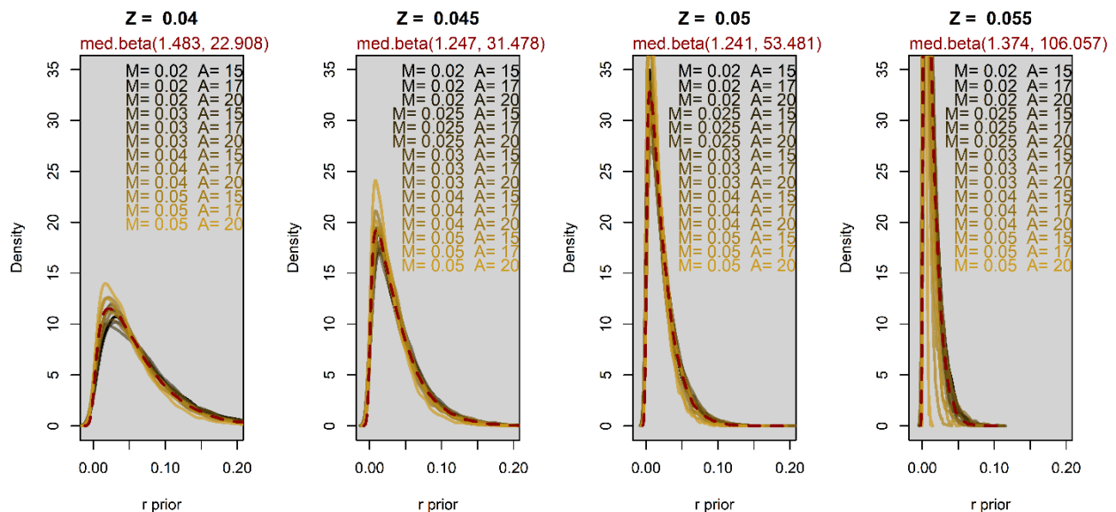
Figure 14.A14. Posterior estimates of R derived from Bayesian projections of a Leslie matrix for yelloweye rockfish using various values for daily mortality of larval fish in their first year of life, Z , annual mortality, M , and average age-of-maturity, A . Average distributions for each panel are represented by the dashed red lines with the beta parameters listed above the panel.
