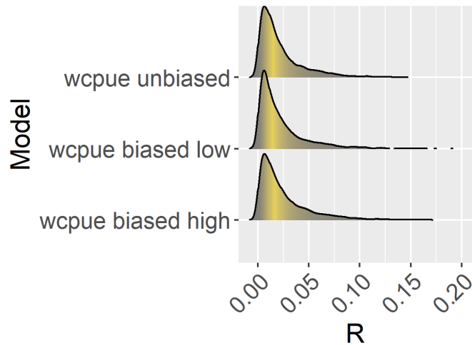
Figure 14.A13. Posterior estimates of R from three Stage-2 SS-SPMs modelled with different assumptions about how bycatch rates of yelloweye rockfish in the pre-IFQ halibut fishery differed relative to WCPUE estimates derived from the IPHC longline survey.
