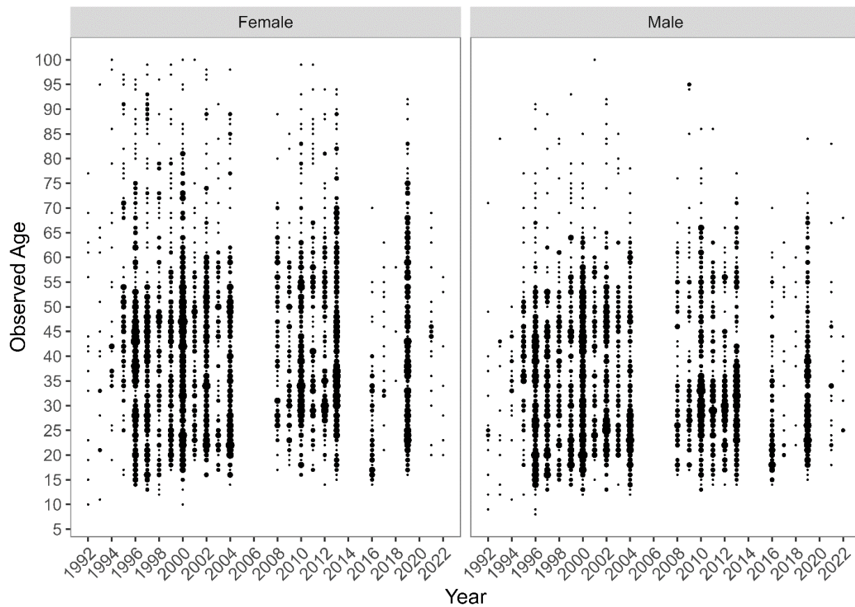
Figure 14.20.—Yelloweye rockfish age compositions sampled in the Southern Southeast Outside (SSEO) Section obtained from directed and incidental catch, 1992–2022. The directed commercial demersal shelf rockfish fishery was closed in 2006, 2007, 2020, 2021, and 2022, and fishery biological data from these years are from halibut incidental fisheries, when available.
