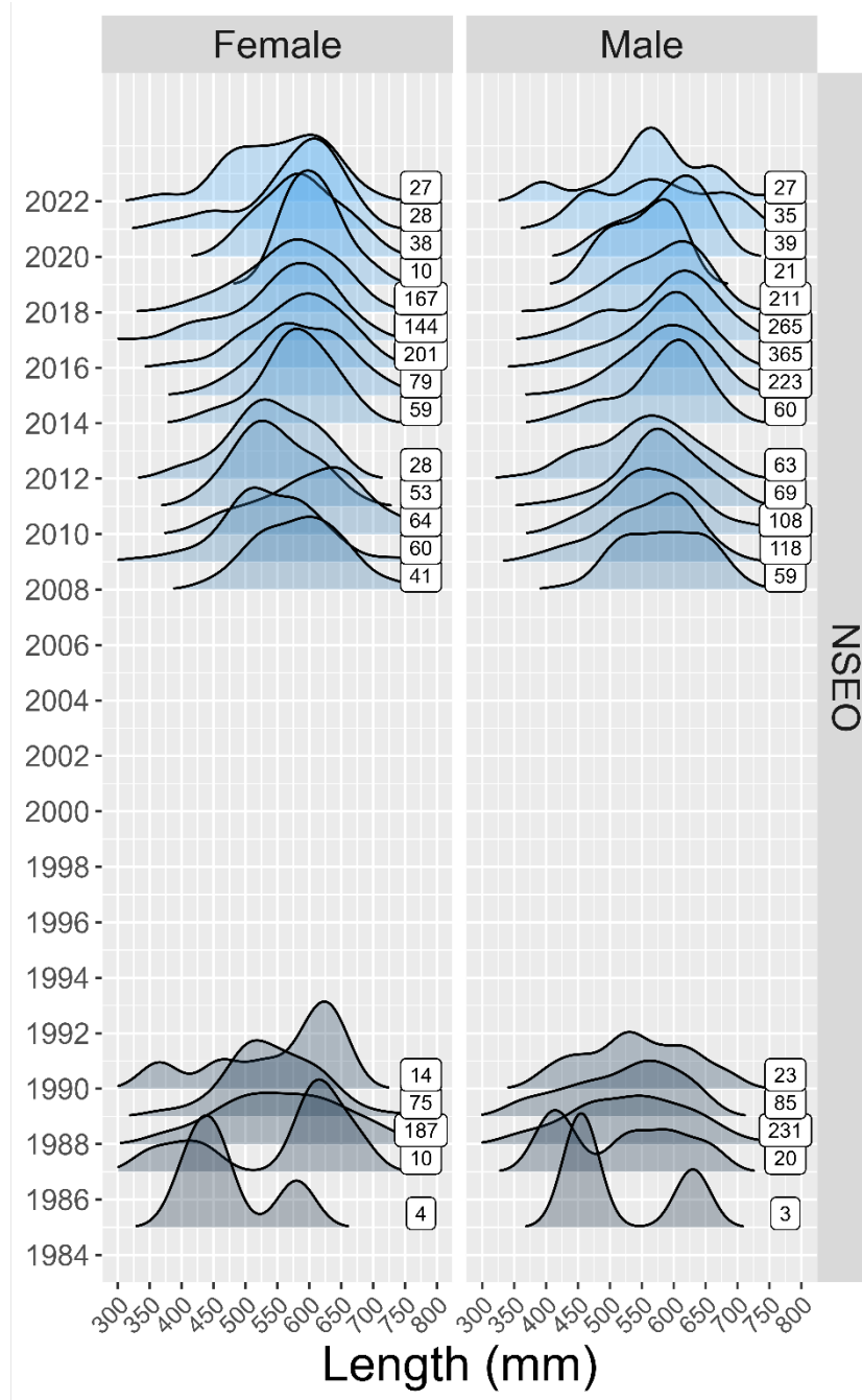
Figure 14.14.—Yelloweye rockfish length compositions sampled in the Northern Southeast Outside (NSEO) Section obtained from directed and incidental catch, 1985–2022. The directed commercial demersal shelf rockfish fishery in NSEO has been closed since 1994, and fishery biological data in recent years are from halibut incidental fisheries, when available. The number of samples in each year are presented next to the density plots.
