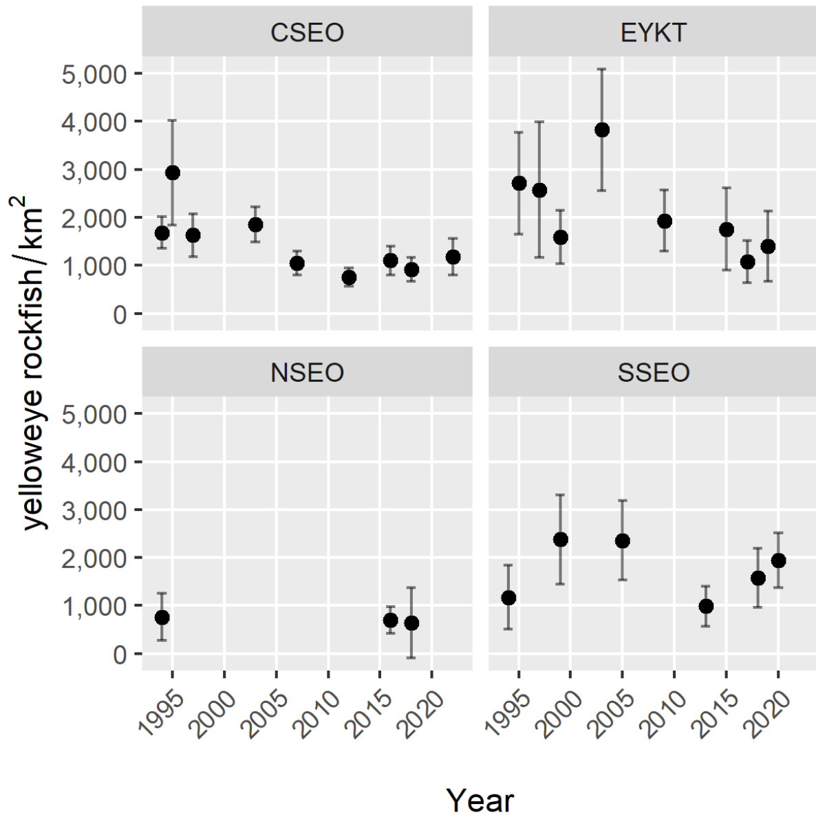
Figure 14.9.—Estimates of yelloweye rockfish density in four management areas in the Southeast Outside (SEO) Subdistrict of the Gulf of Alaska: East Yakutat (EYKT), Northern Southeast Outside (NSEO), Central Southeast Outside (CSEO), and Southern Southeast Outside (SSEO) Sections, 1994–2022 as derived from submersible and ROV surveys and distance sampling methods. Error bars represent 95% confidence intervals.
