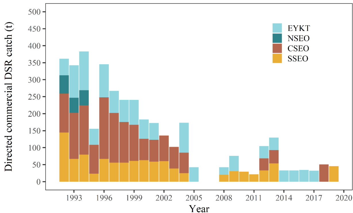
Figure 14.3.—Directed commercial demersal shelf rockfish (DSR) fishery catch (t) in the Southeast Outside (SEO) Subdistrict groundfish management areas: East Yakutat (EYKT), Northern Southeast Outside (NSEO), Central Southeast Outside (CSEO), and Southern Southeast Outside (SSEO) Sections, 1992–2019. The directed commercial fishery was closed in SEO in 2006 and 2007 and has been closed since 2020.
