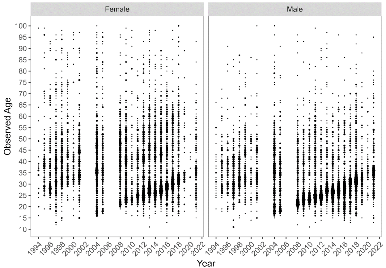
Figure 14.17.—Yelloweye rockfish age compositions sampled in the East Yakutat (EYKT) Section obtained from directed and incidental catch, 1994–2022. The directed commercial demersal shelf rockfish fishery was closed in 2006, 2007, 2020, 2021 and 2022, and fishery biological data from these years are from halibut incidental fisheries, when available.
