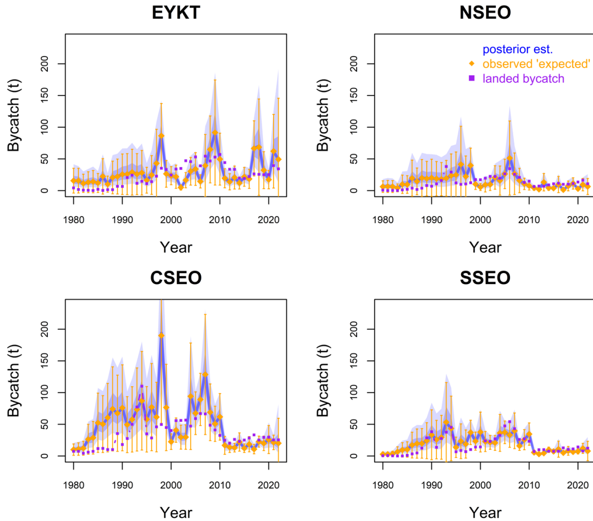
Figure 14.A6. Estimates of yelloweye rockfish bycatch in the halibut fishery from the Stage-1 SS-SPM in the four management units in the Southeast Outside subdistrict (SEO) of the Gulf of Alaska (blue line with 50 and 95% credibility interval polygons), the expected bycatch estimates from the IPHC longline survey (orange diamonds with 95% confidence interval error bars) and reported landings of yelloweye rockfish in the halibut fishery (purple squares). Note that error bars on the expected bycatch estimates are constructed parametrically where-as the SS-SPM applies log-normal error structure.
