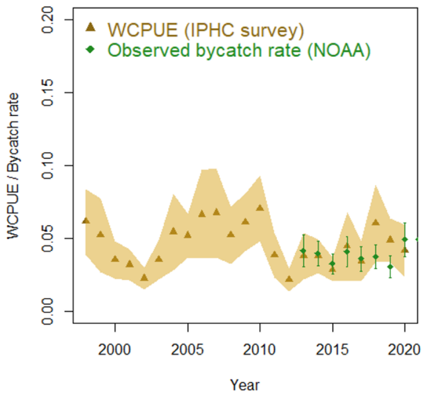
Figure 14.A2: Estimated bycatch rates (wcpue estimates) in the Southeast Outside subdistrict (SEO) of the Gulf of Alaska (brown triangles) and bycatch rates from the NOAA Catch Accounting System (CAS; green diamonds). Error polygons and error bars represent 95% confidence intervals.
