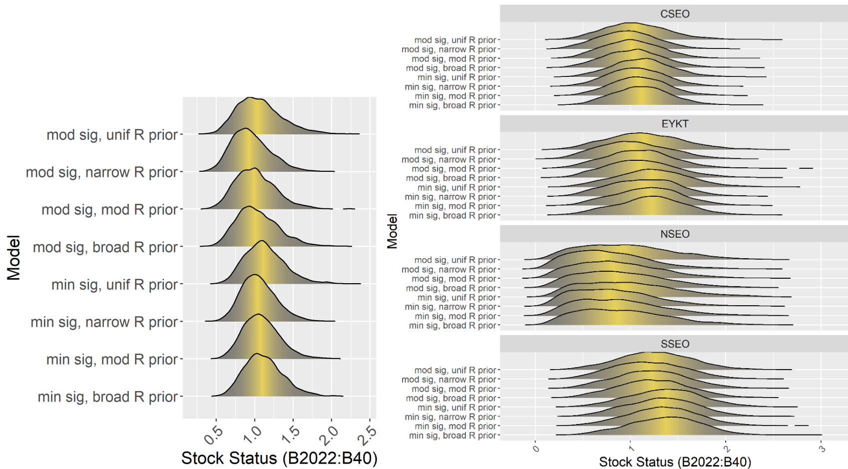
Figure 14.A25. Posterior distributions of stock status (The ratio of biomass in 2022 relative to B_{msy}/B_{40} ) for the Southeast Outside (SEO) district as a whole (left side) and for the management units (right side) produced by eight Stage-3 SS-SPMs modelled with moderate (mod sig) and minimal (min sig) process error, \sigma_{proc} , and four priors for R ranging from an uninformative beta distribution (unif R) through the broadest (broad R), moderate (mod R) and narrowest (narrow R) beta distributions derived from the projected Leslie matrices (Figure X23).
