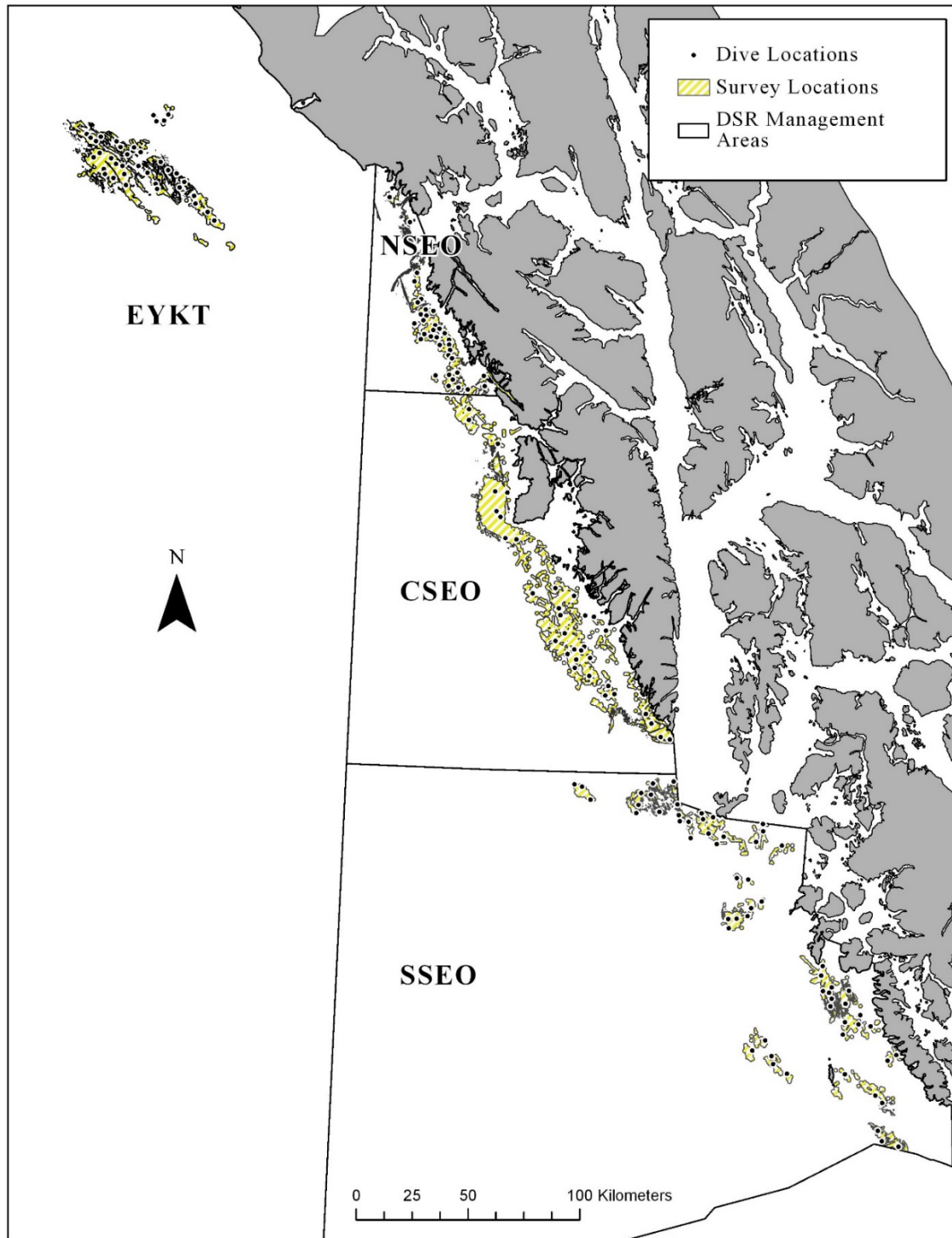
Figure 14.7.—The designated yelloweye rockfish habitat (DYRH; yellow hatching) and example dive locations (black circles) for remotely operated vehicle (ROV) surveys in the Southeast Outside Subdistrict (SEO) of the Gulf of Alaska.
