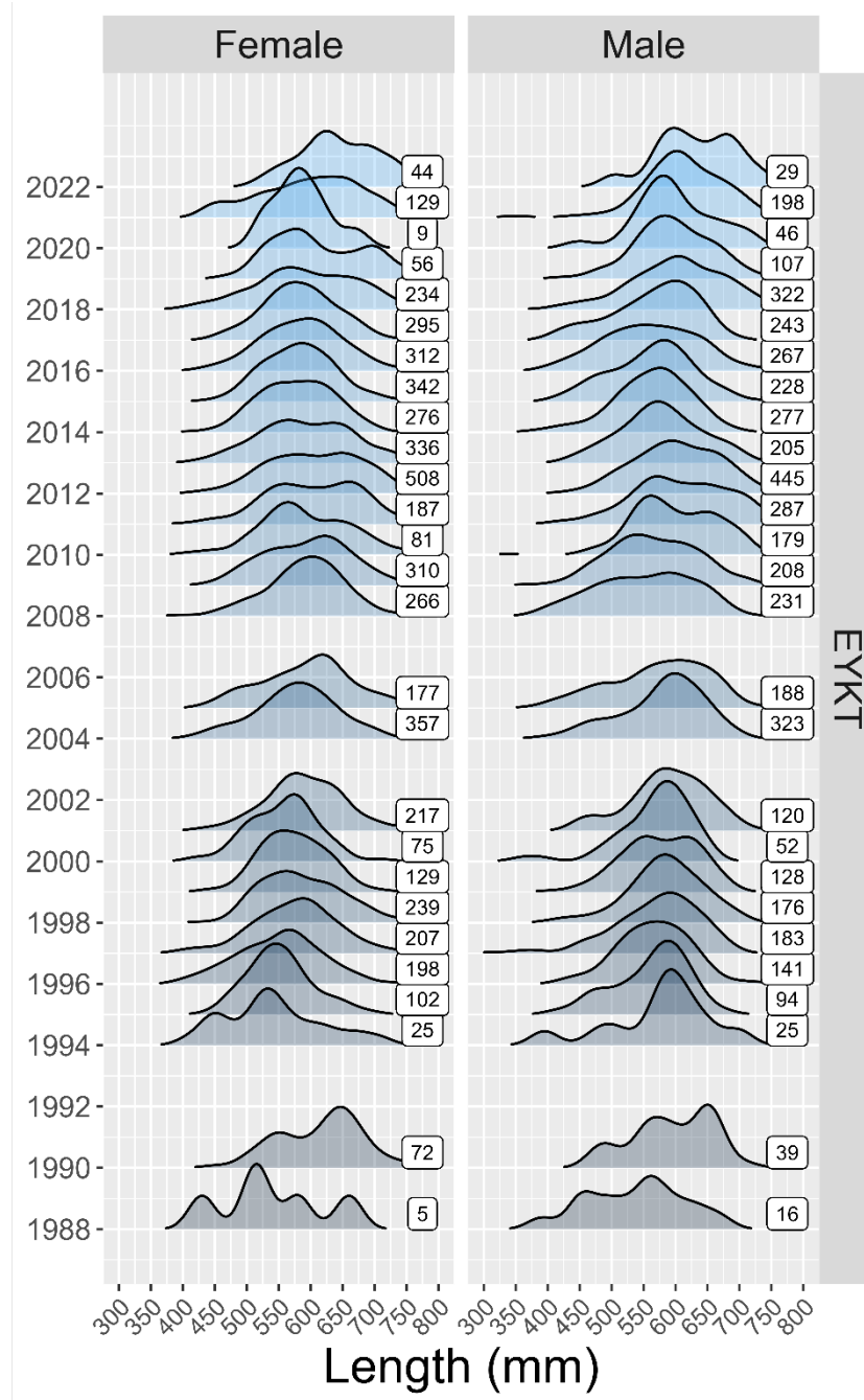
Figure 14.13.—Yelloweye rockfish length compositions sampled in the East Yakutat (EYKT) Section obtained from directed and incidental catch, 1988–2022. The directed commercial demersal shelf rockfish fishery was closed in 2006, 2007, 2020, 2021, and 2022, and fishery biological data from these years are from halibut incidental fisheries, when available. The number of samples in each year are presented next to the density plots.
