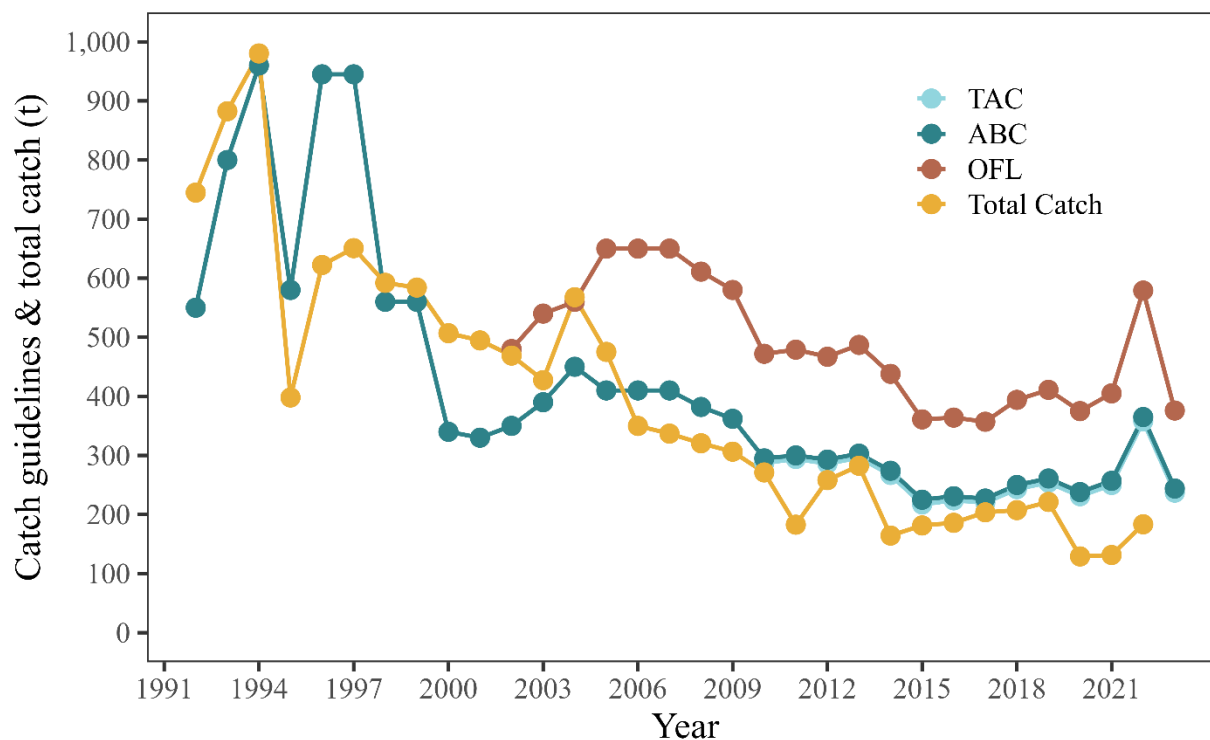
Figure 14.5.—Demersal shelf rockfish (DSR) catch guidelines: overfishing level (OFL), allowable biological catch (ABC), total allowable catch (TAC), and total catch for the Southeast Outside (SEO) Subdistrict, 1992–2023. The directed commercial fishery was closed in SEO in 2006 and 2007 and has been closed since 2020. The recreational fishery was closed to the retention of DSR in all Southeast Alaska management areas in 2020 and 2021; however, 2020 and 2021 recreational fishery catch include the estimated release mortality.
