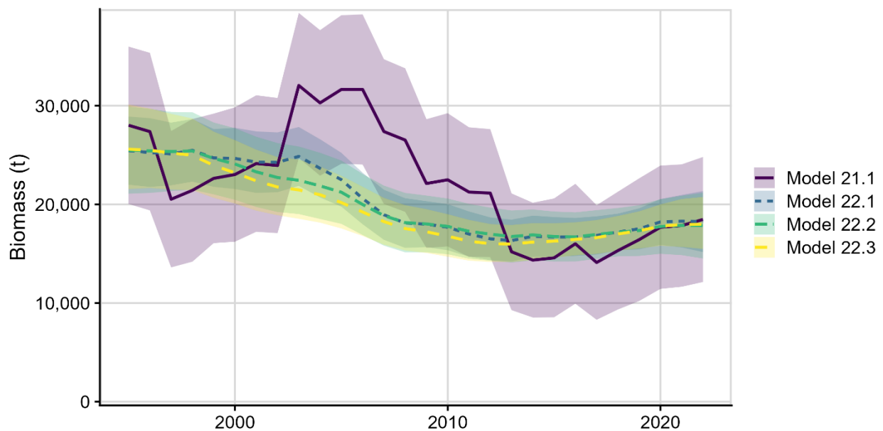
Figure 14.A17. Total Southeast Outside (SEO) yelloweye rockfish biomass (t) with 90% confidence intervals from the four alternative models, 1995-2022. Model 21.1 uses status-quo methods with revised values calculated directly from published density estimates, Model 22.1 uses the two-survey random effects (REMA) model, Model 22.2 is Model 22.1 but estimates additional observation error for the biomass data, and Model 22.3 uses the Bayesian state-space surplus production model (SS-SPM; Appendix A).
