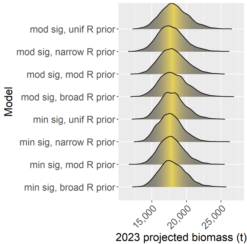
Figure 14.A18. Posterior distributions of projected biomass for 2023 produced by eight Stage-3 SS-SPMs modelled with moderate (mod sig) and minimal (min sig) process error, \sigma_{proc} , and four priors for R ranging from an uninformative beta distribution (unif R) through the broadest (broad R), moderate (mod R) and narrowest (narrow R) beta distributions derived from the projected Leslie matrices (Figure X23).
