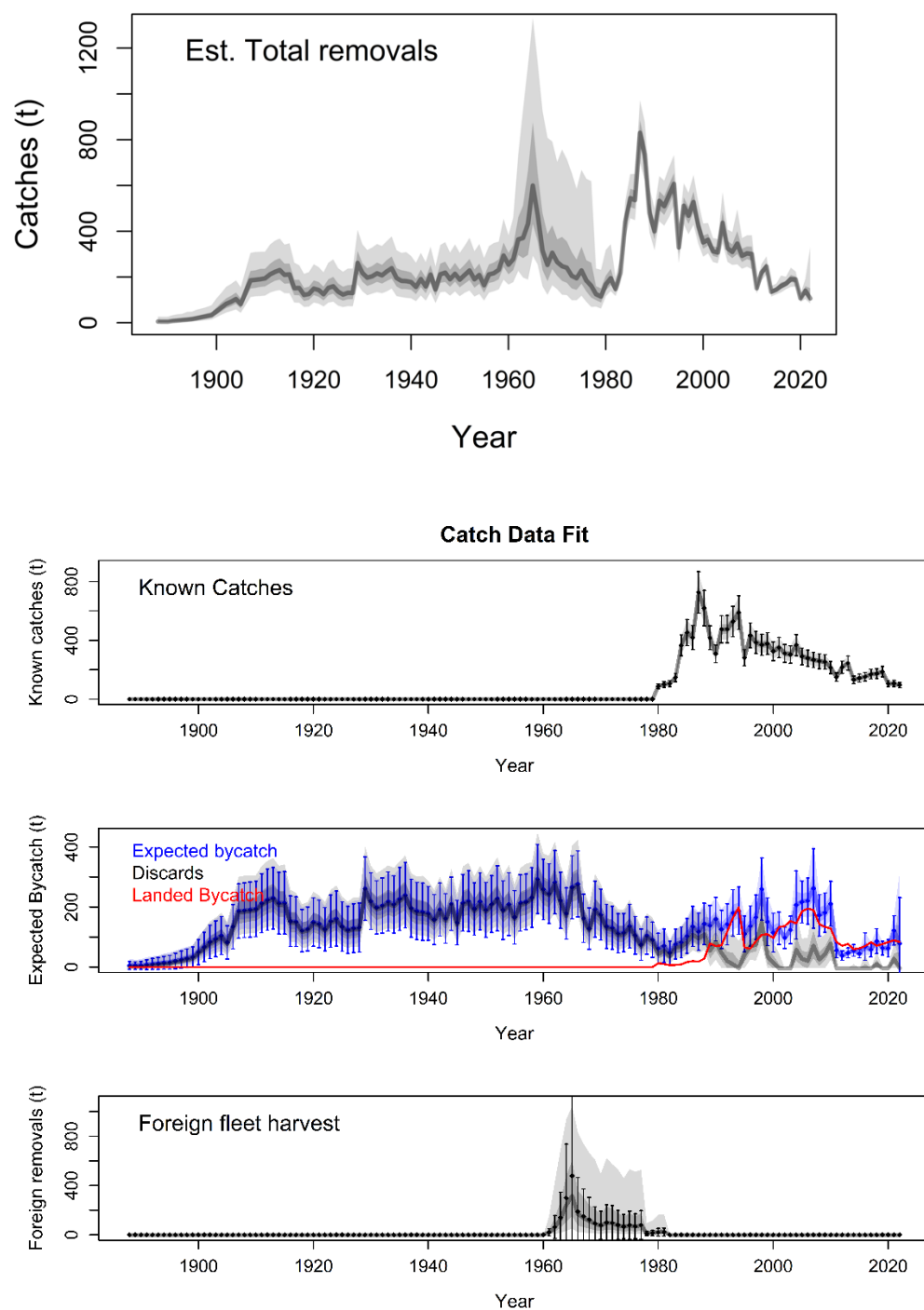
Figure 14.A11. Posterior estimates of total removals of yelloweye rockfish in the Southeast Outside subdistrict (SEO) of the Gulf of Alaska from the Stage-2 SS-SPM with 50 and 95% credibility interval polygons (top plot) and the fit of known catches, expected bycatch and foreign fleet removals to data sources with 95% confidence interval error bars. Error bars from the data are plotted as normally distributed whereas posterior estimates from the SS-SPM are modelled as log-normal.
