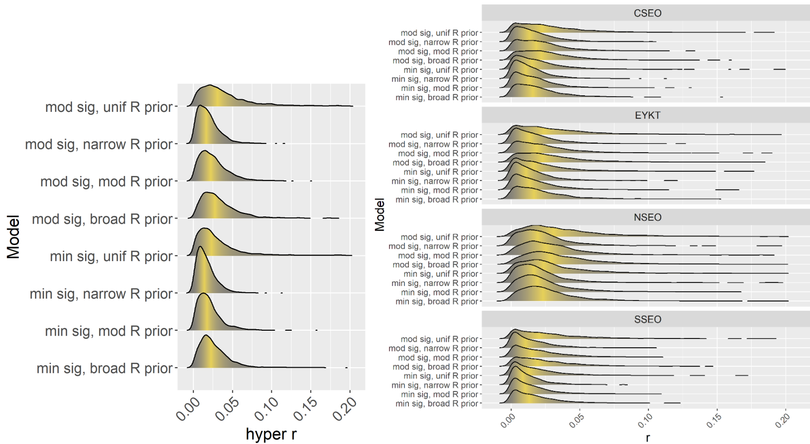
Figure 14.A19. Posterior distributions of R (left side) and r_s (right side) produced by eight Stage-3 SS-SPMs modelled with moderate (mod sig) and minimal (min sig) process error, \sigma_{proc} , and four priors for R ranging from an uninformative beta distribution (unif R) through the broadest (broad R), moderate (mod R) and narrowest (narrow R) beta distributions derived from the projected Leslie matrices (Figure X23).
