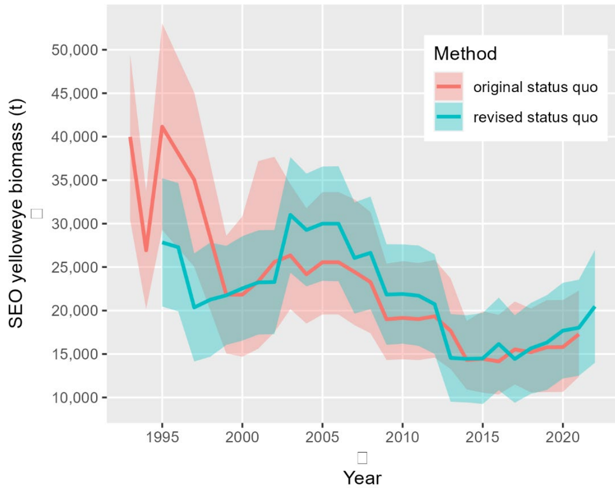
Figure 14.10.—Estimated biomass of yelloweye rockfish in the Southeast Outside district of the Gulf of Alaska (SEO) as determined by the status-quo methods using historically published estimates and revised values calculated directly from published density estimates.
