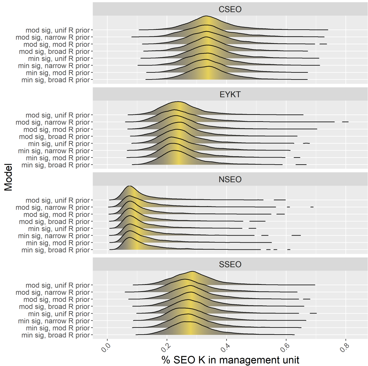
Figure 14.A21. Posterior distributions of \pi_i , the estimated proportion of K composed of the K_s estimates, produced by eight Stage-3 SS-SPMs modelled with moderate (mod sig) and minimal (min sig) process error, \sigma_{proc} , and four priors for R ranging from uninformative beta distribution (unif R) through the broadest (broad R), moderate (mod R) and narrowest (narrow R) beta distributions derived from the projected Leslie matrices (Figure X23).
