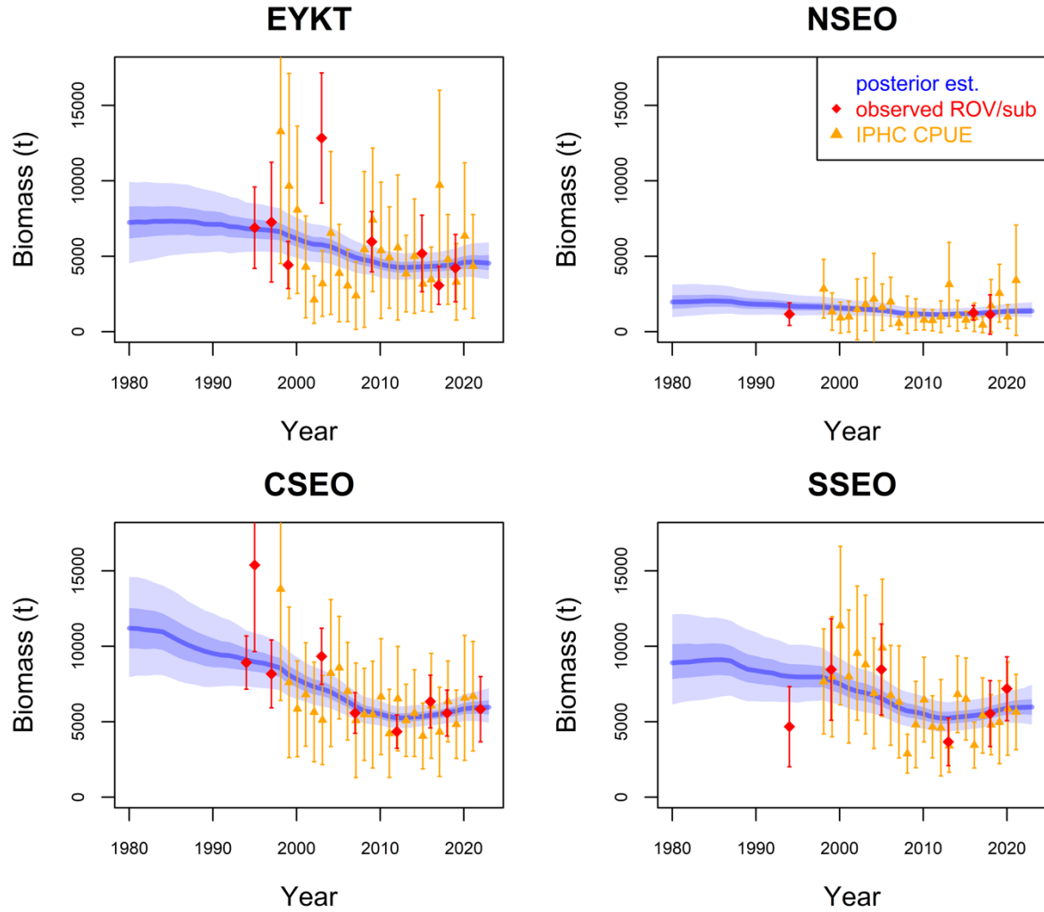
Figure 14.A15. Estimates of yelloweye rockfish biomass from the Stage-3 SS-SPM in the four management areas of the Southeast Outside subdistrict (SEO) of the Gulf of Alaska (blue line with 50 and 95% credibility interval polygons), the biomass estimates from submersible and ROV surveys (red diamonds with 95% confidence interval error bars) and IPHC CPUE indices scaled with the mean estimate of q_s from the SS-SPM (orange triangles with 95% confidence interval error bars). These results are from the minimal process error model with an uninformative prior on R .
