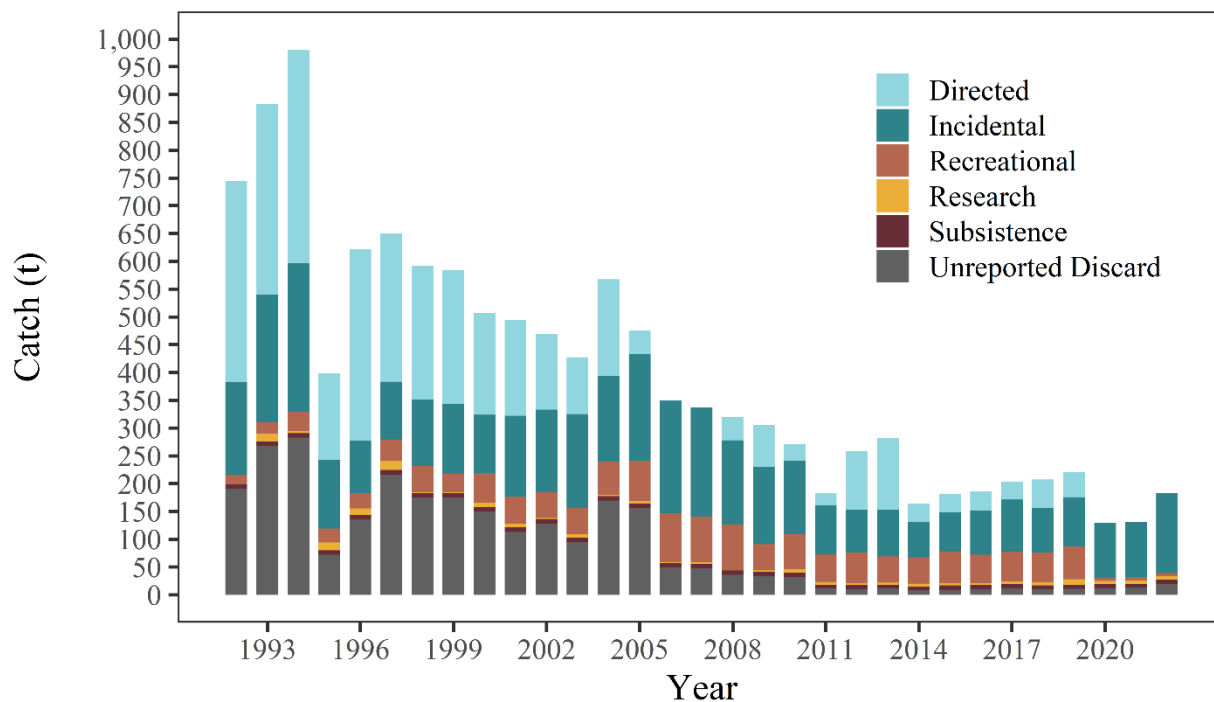
Figure 14.6.—Demersal shelf rockfish (DSR) catch (t) by fishery type: commercial (directed, incidental, and estimated unreported discards from the halibut longline fishery), recreational, research, and subsistence for the Southeast Outside (SEO) Subdistrict, 1992–2022. The directed commercial fishery was closed in SEO in 2006 and 2007 and has been closed since 2020. The recreational fishery was closed to the retention of DSR in all Southeast Alaska management areas in 2020 and 2021; however, 2020 and 2021 recreational fishery catch include the estimated release mortality.
