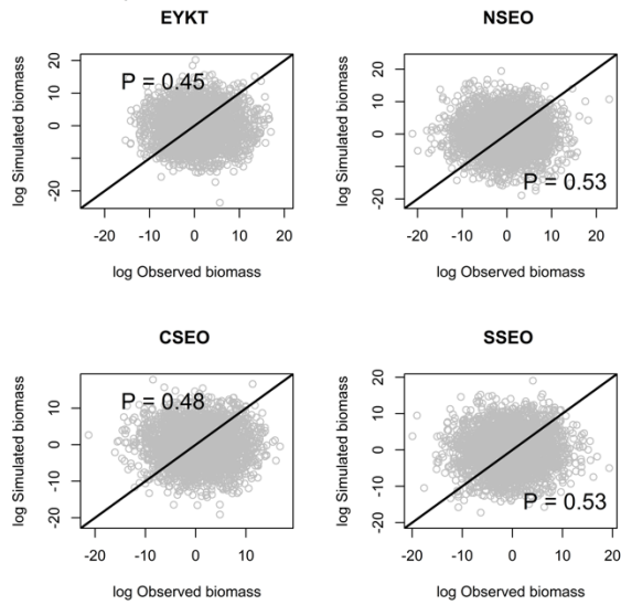
Figure 14.A4 Posterior-predictive checks of Stage-1 SS-SPM observed and simulated biomass for the submersible and ROV biomass estimates (left side) and for the IPHC CPUE index (right side) in the four management areas of the Southeast Outside (SEO) district.
