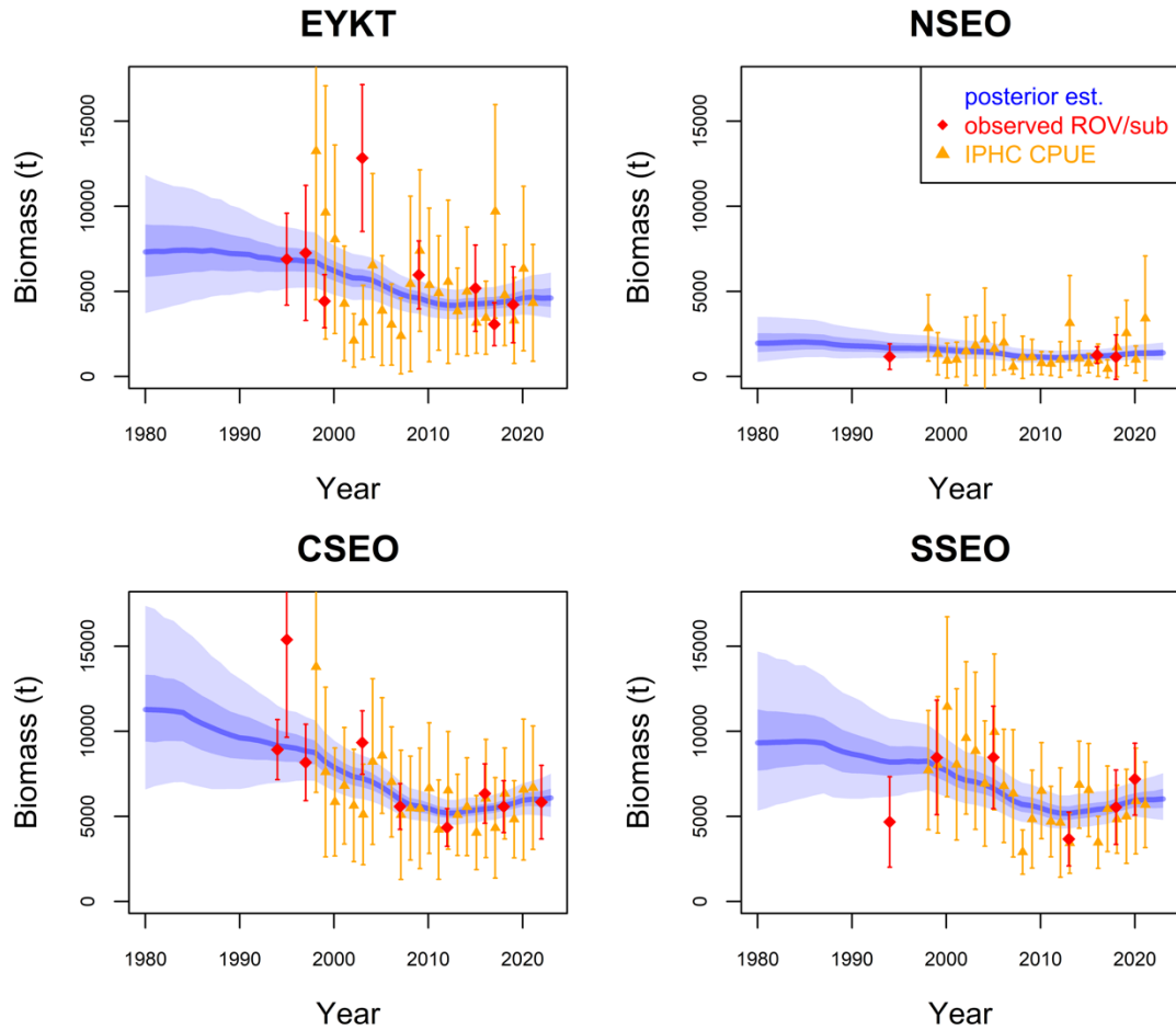
Figure 14.A5. Estimates of yelloweye rockfish biomass from the Stage-1 SS-SPM in the four management areas in the Southeast Outside subdistrict (SEO) of the Gulf of Alaska (blue line with 50 and 95% credibility interval polygons), the biomass estimates from submersible and ROV surveys (red diamonds with 95% confidence interval error bars) and IPHC CPUE indices scaled with the mean estimate of q_s from the SS-SPM (orange triangles with 95% confidence interval error bars).
