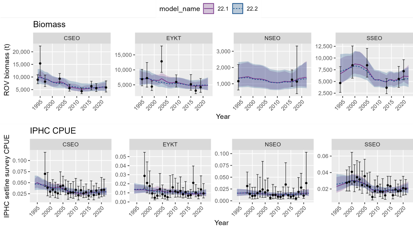
Figure 14.11.—Two-survey random effects (REMA) model fits to the ADF&G submersible and ROV survey biomass (t; top) and IPHC longline survey CPUE (bottom). Model 22.1 and Model 22.2 share the same structure (single process error, area-specific scaling parameter), but Model 22.2 estimates additional observation error for the biomass data.
