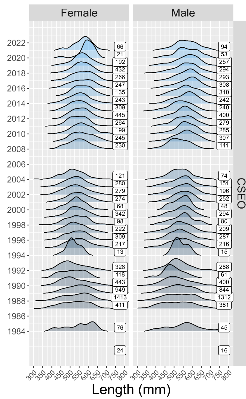
Figure 14.15.—Yelloweye rockfish length compositions sampled in the Central Southeast Outside (CSEO) Section obtained from directed and incidental catch, 1981–2022. The directed commercial demersal shelf rockfish fishery was closed in 2006, 2007, 2020, 2021, and 2022, and fishery biological data from these years are from halibut incidental fisheries, when available. The number of samples in each year are presented next to the density plots.
