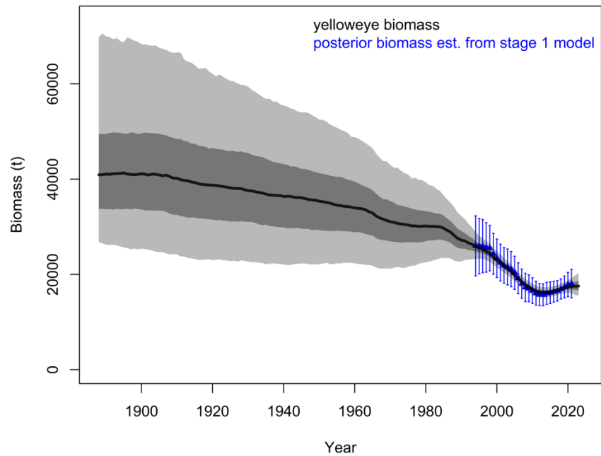
Figure 14.A10. Estimates of yelloweye rockfish biomass in the Southeast Outside subdistrict (SEO) of the Gulf of Alaska from the Stage-2 SS-SPM (black line with 50 and 95% credibility interval polygons) and the estimates of biomass from Stage-1 SS-SPM (blue dots with 95% credibility interval error bars), 1888-2022.
