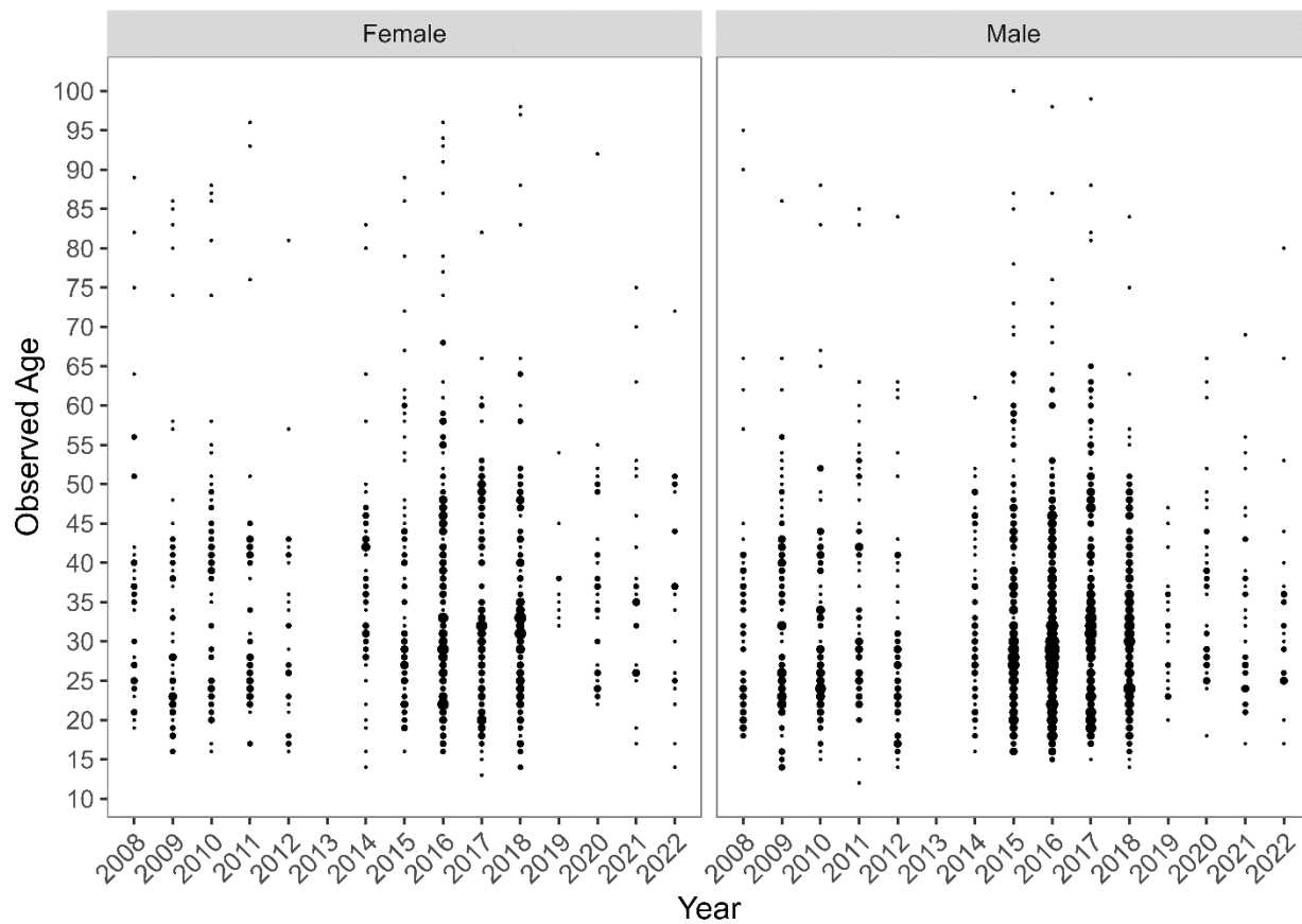
Figure 14.18.—Yelloweye rockfish age compositions sampled in the Northern Southeast Outside (NSEO) Section obtained from directed and incidental catch, 2008–2022. The directed commercial demersal shelf rockfish fishery in NSEO has been closed since 1994, and fishery biological data in recent years are from halibut incidental fisheries, when available.
