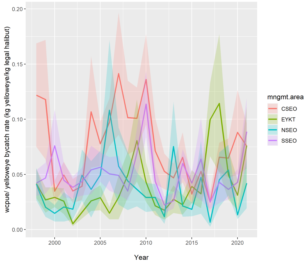
Figure 14.A1: Estimated bycatch rates (WCPUE estimates) derived from the IPHC longline survey data in the four management areas of the Southeast Outside subdistrict (SEO) of the Gulf of Alaska 1998-2021. Error polygons represent 95% confidence intervals.
