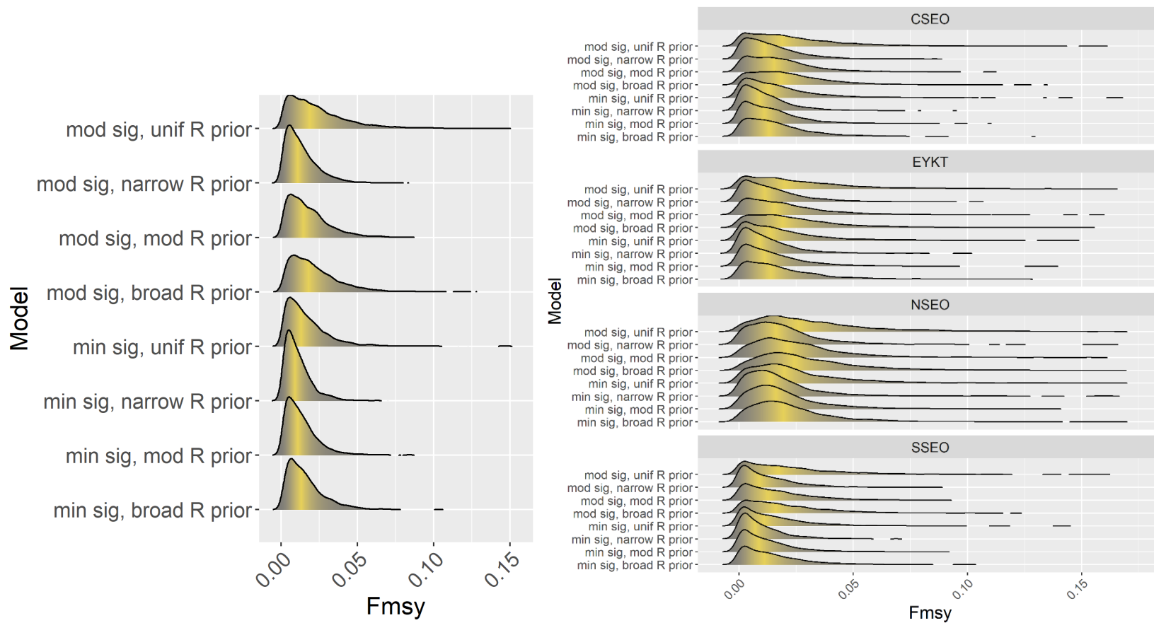
Figure 14.A24. Posterior distributions of F_{MSY} for the Southeast Outside (SEO) district as a whole (left side) and for the management units (right side) produced by eight Stage-3 SS-SPMs modelled with moderate (mod sig) and minimal (min sig) process error, \sigma_{proc} , and four priors for R ranging from an uninformative beta distribution (unif R) through the broadest (broad R), moderate (mod R) and narrowest (narrow R) beta distributions derived from the projected Leslie matrices (Figure X23).
