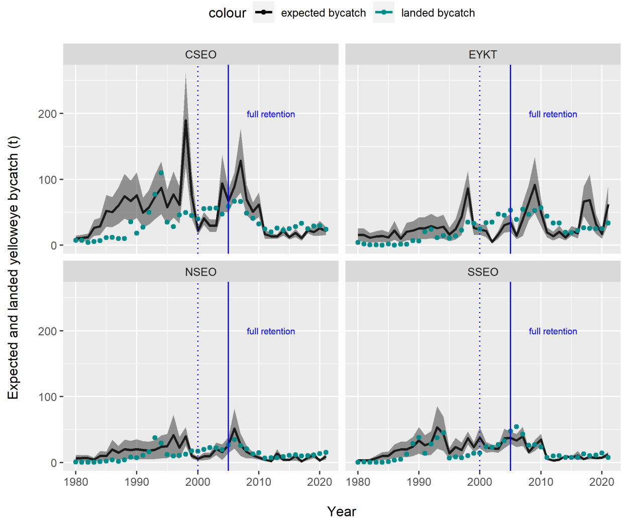
Figure 14.A3: Estimates of expected bycatch of yelloweye rockfish in the halibut fishery derived from halibut harvests and bycatch rates calculated from the IPHC longline survey (black lines and grey error polygons) and landed yelloweye rockfish bycatch in the halibut fishery as recorded on fish tickets (blue dots) in each of four management areas in the Southeast Outside subdistrict (SEO). Error polygons represent 95% confidence intervals. Vertical blue lines highlight the transition to full retention rules for bycatch that was phased in between 2000 and 2005.
