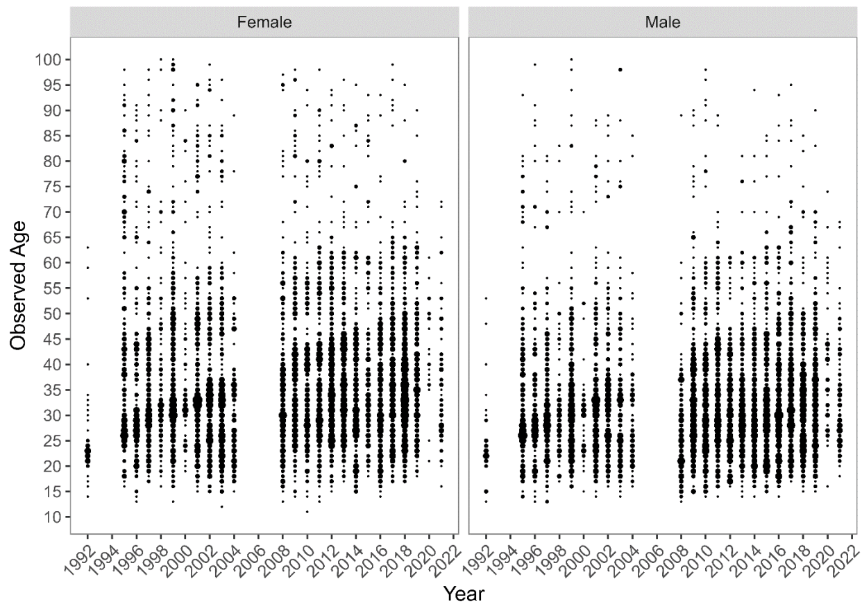
Figure 14.19.—Yelloweye rockfish age compositions sampled in the Central Southeast Outside (CSEO) Section obtained from directed and incidental catch, 1992–2022. The directed commercial demersal shelf rockfish fishery was closed in 2006, 2007, 2020, 2021, and 2022, and fishery biological data from these years are from halibut incidental fisheries, when available.
