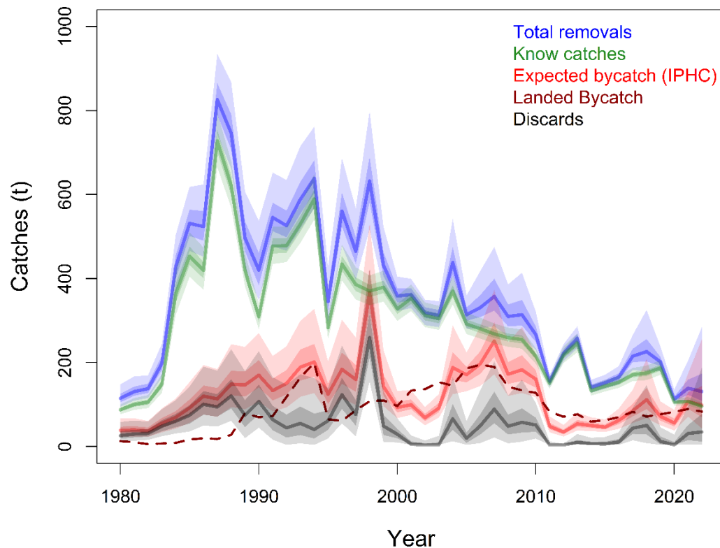
Figure 14.A9. Posterior estimates of total yelloweye rockfish catch (blue lines with 50 and 95% confidence interval polygons), total known catches (green), estimated bycatch in the halibut fishery (red), recorded landings of yelloweye rockfish in the halibut fishery (red dashed line) and estimated discards of yelloweye rockfish in the halibut fishery (dark grey) from Stage-1 SS-SPMs. Estimates of discards are derived by subtracting recorded landings from estimated bycatch. Total catch (in blue) is derived as the sum of the total known catches (in green) and the estimated discards. Error polygons represent 50 and 95% credibility intervals.
