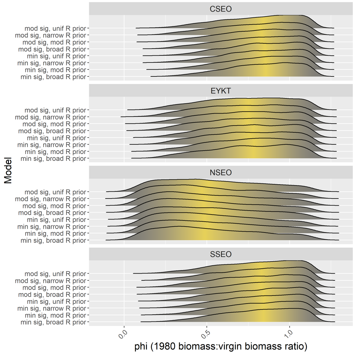
Figure 14.A22. Posterior distributions of \phi , the estimated proportion of K_s comprising biomass in 1980, produced by eight Stage-3 SS-SPMs modelled with moderate (mod sig) and minimal (min sig) process error, \sigma_{proc} , and four priors for R ranging from an uninformative beta distribution (unif R) through the broadest (broad R), moderate (mod R) and narrowest (narrow R) beta distributions derived from the projected Leslie matrices (Figure X23).
