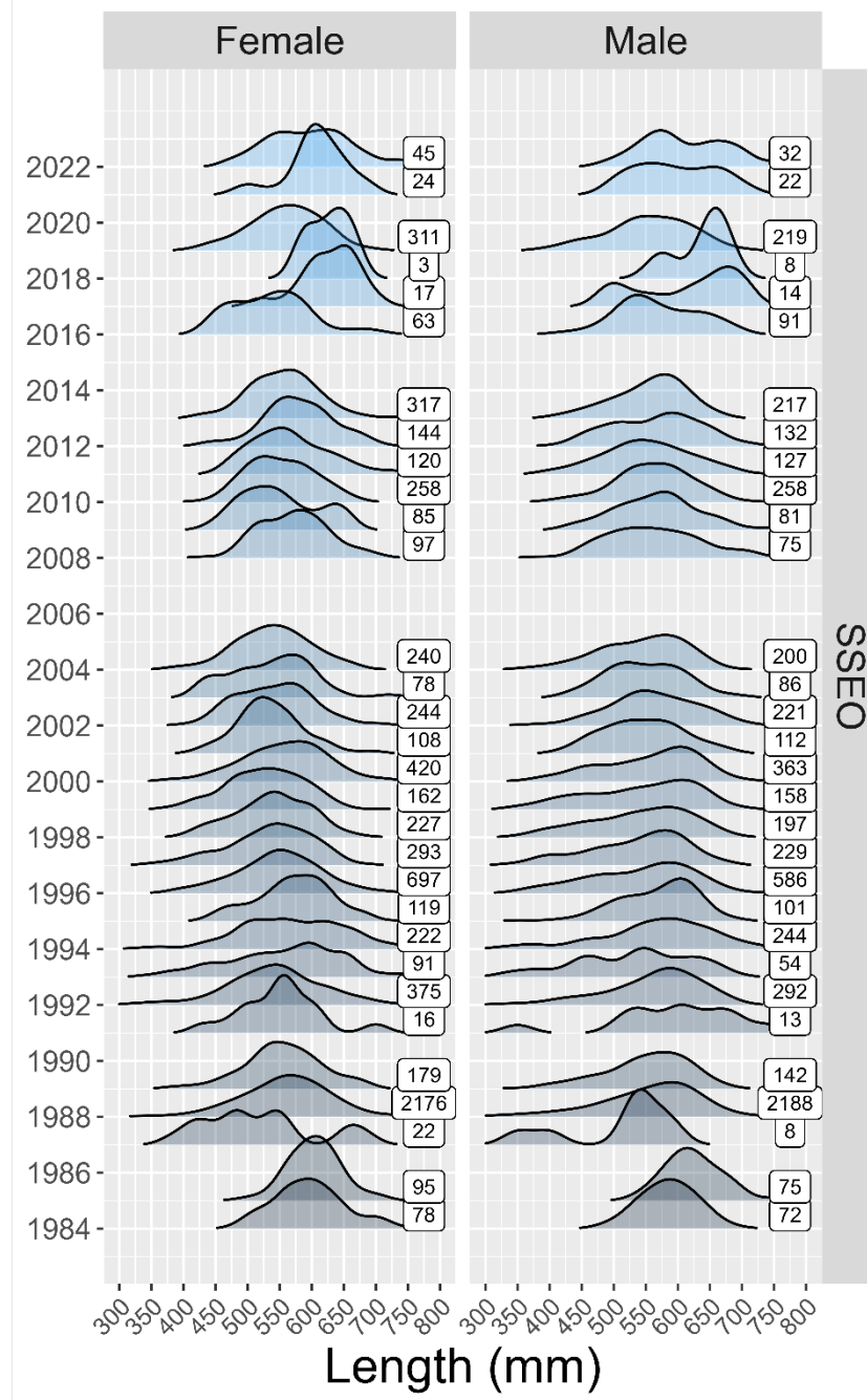
Figure 14.16.—Yelloweye rockfish length compositions sampled in the Southern Southeast Outside (SSEO) Section obtained from directed and incidental catch, 1984–2022. The directed commercial demersal shelf rockfish fishery was closed in 2006, 2007, 2020, 2021 and 2022, and fishery biological data from these years are from halibut incidental fisheries, when available. The number of samples in each year are presented next to the density plots.
