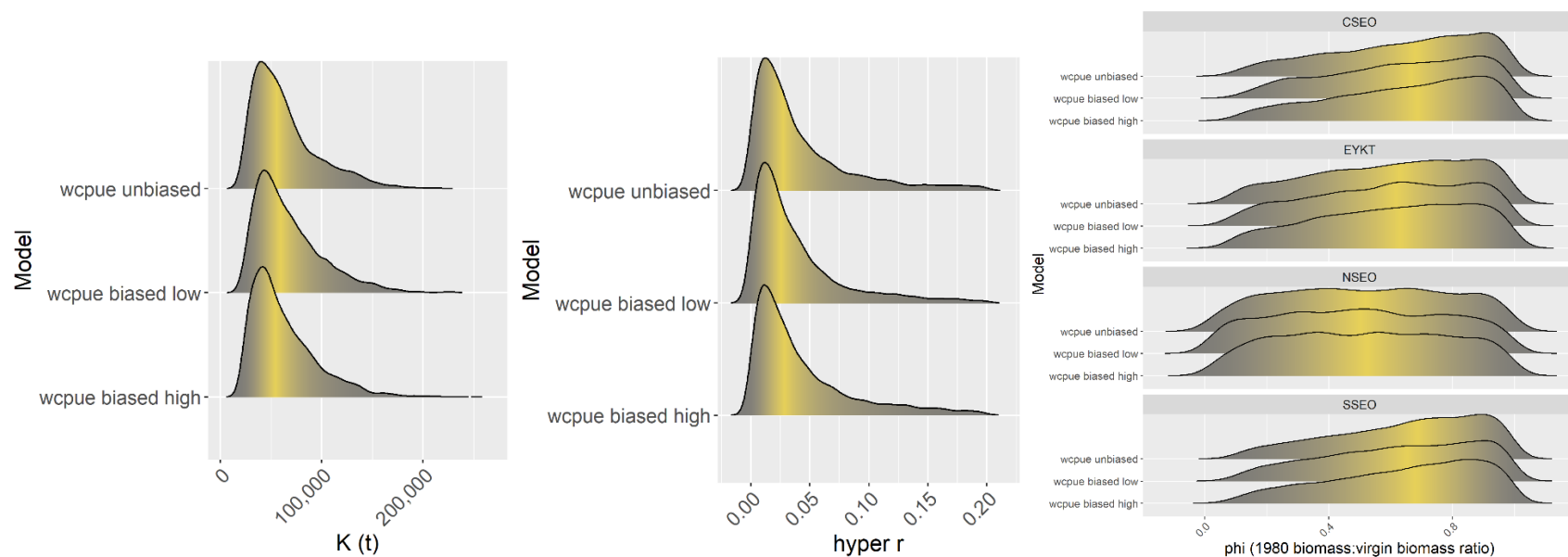
Figure 14.A8. Posterior distributions of Stage-1 SS-SPM estimates of K , R , and \phi_s , in the model variations that treated bycatch rates (WCPUE) calculated from IPHC longline survey data to be either unbiased, biased low by 30% and biased high by 30% relative to the “true” bycatch in the pre-IFQ halibut fishery.
