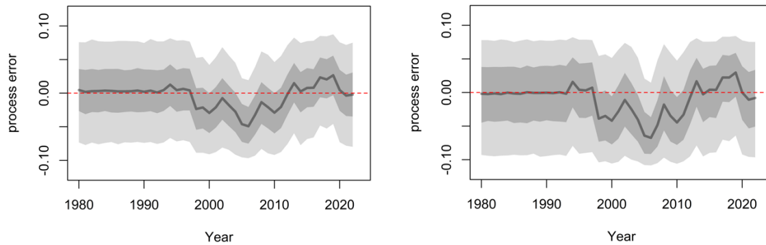
Figure 14.A16. Posterior estimates of process error for Stage-3 models from the minimal process error model ( \max \sigma_{proc} = 0.08 ) on the left and the moderate process error model ( \max \sigma_{proc} = 0.22 ) on the right.
