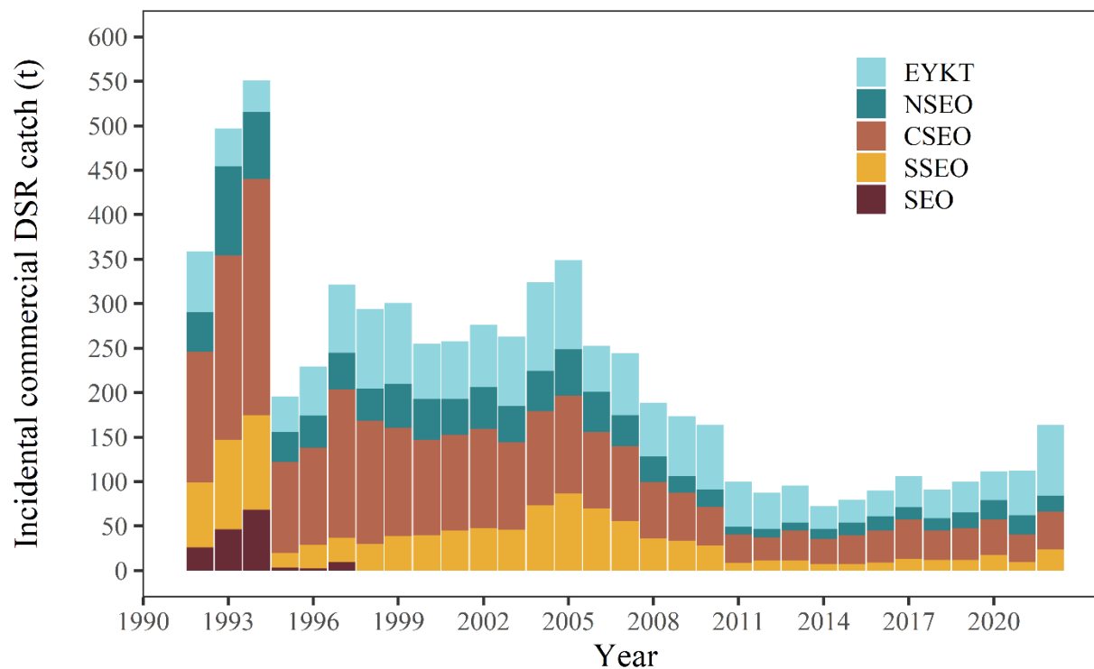
Figure 14.4.—Incidental commercial fishery catch (t) of demersal shelf rockfish (DSR) in the halibut, sablefish, lingcod, Pacific cod, miscellaneous finfish, and salmon fisheries for Southeast Outside (SEO) Subdistrict groundfish management areas: East Yakutat (EYKT), Northern Southeast Outside (NSEO), Central Southeast Outside (CSEO), and Southern Southeast Outside (SSEO) Sections, 1992–2022. Harvest in the SEO area could not be assigned to a management area due to fish ticket data limitations.
