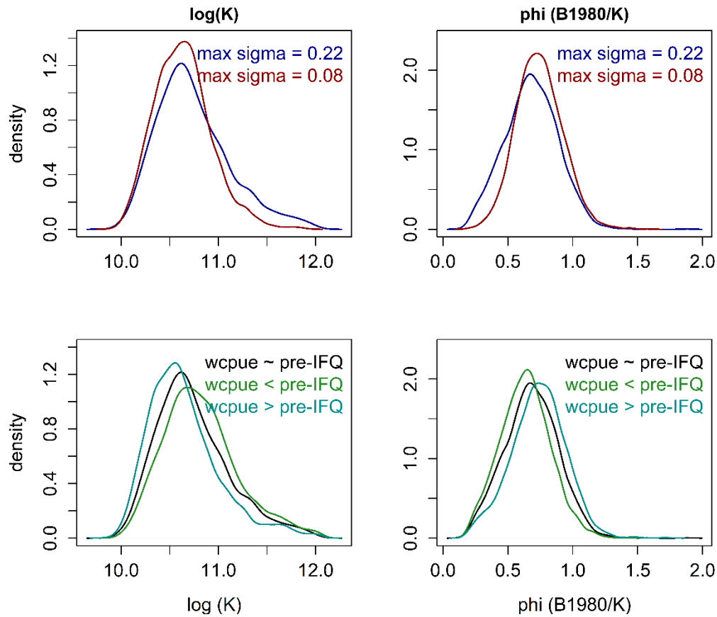
Figure 14.A12. Posterior distributions of \log(K) and the ratio of 1980 biomass to K ( \phi ) from Phase-2 SS-SPMs modelled under moderate and minimal process error (top row) and variable assumptions about how bycatch rates of yelloweye rockfish in the pre-IFQ halibut fishery differed relative to WCPUE estimates derived from the IPHC longline survey (bottom row). These distributions were used to model priors on K and \phi for Stage-3 models.
