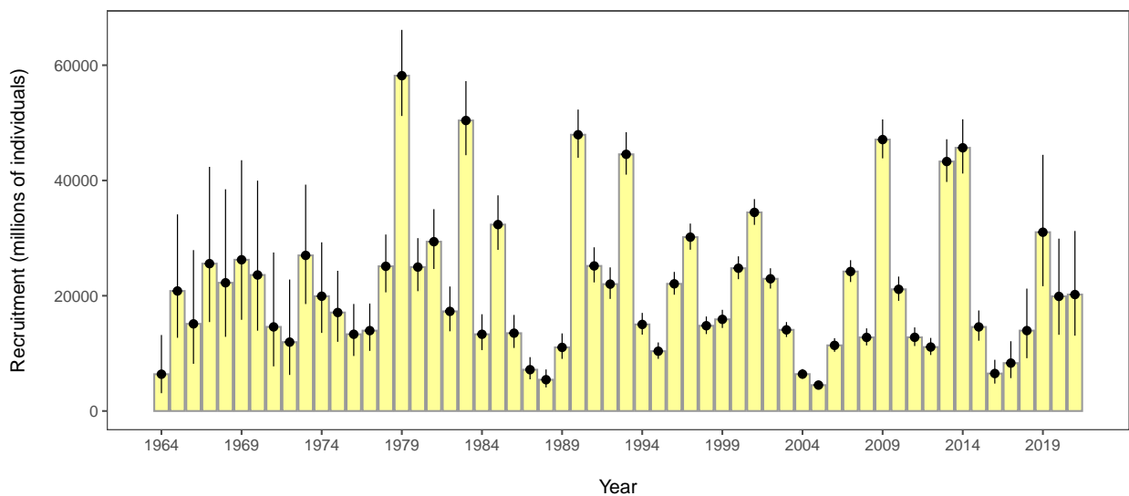
Figure 1-55. Recruitment estimates (age-1 recruits) for EBS pollock for all years since 1964 (1963–2020 year classes) for Model 20.0c. Error bars reflect 90% credible intervals based on model estimates of uncertainty.
