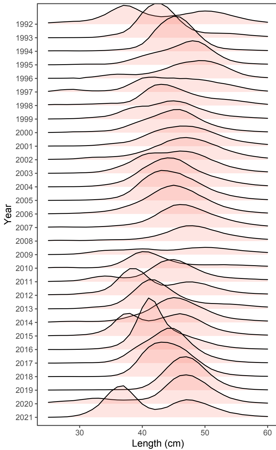
Figure 1-13. Fishery catch-at-length (cm) by the pollock fishery, 1992-2021.
