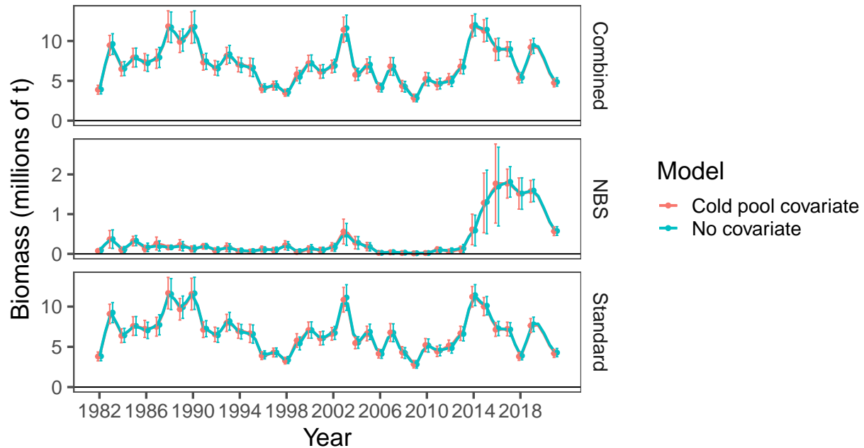
Figure 1-62. Pollock index values for the standard survey region, the NBS, and combined based on the VAST application to density-dependent corrected CPUE values from the BTS data, 1982–2019, 2021. The different lines are smoothed trends for with and without including the cold-pool extent as a covariate.
