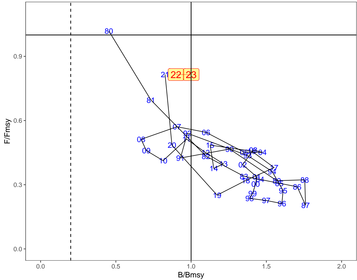
Figure 1-53. Estimated spawning biomass relative to annually estimated F_{MSY} values and fishing mortality rates for EBS pollock. Two projection years are shaded in yellow
