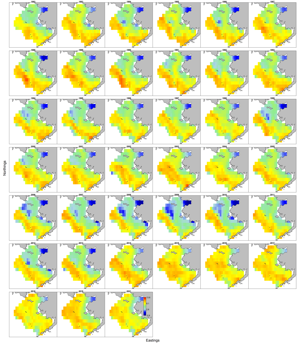
Figure 1-61. Pollock log density maps of the BTS data using the VAST model approach, 1982-2019,2021.
