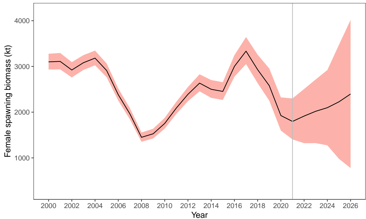
Figure 1-54. The estimated EBS pollock spawning stock biomass for model 20.0 with projections equal to the estimated fishing mortality from 2021.
