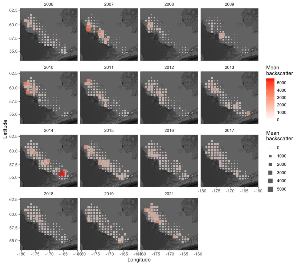
Figure 1-22. Maps of acoustic vessel-of-opportunity (AVO) index data 2006-2021. Grid cell size and shading is proportional to pollock backscatter.
