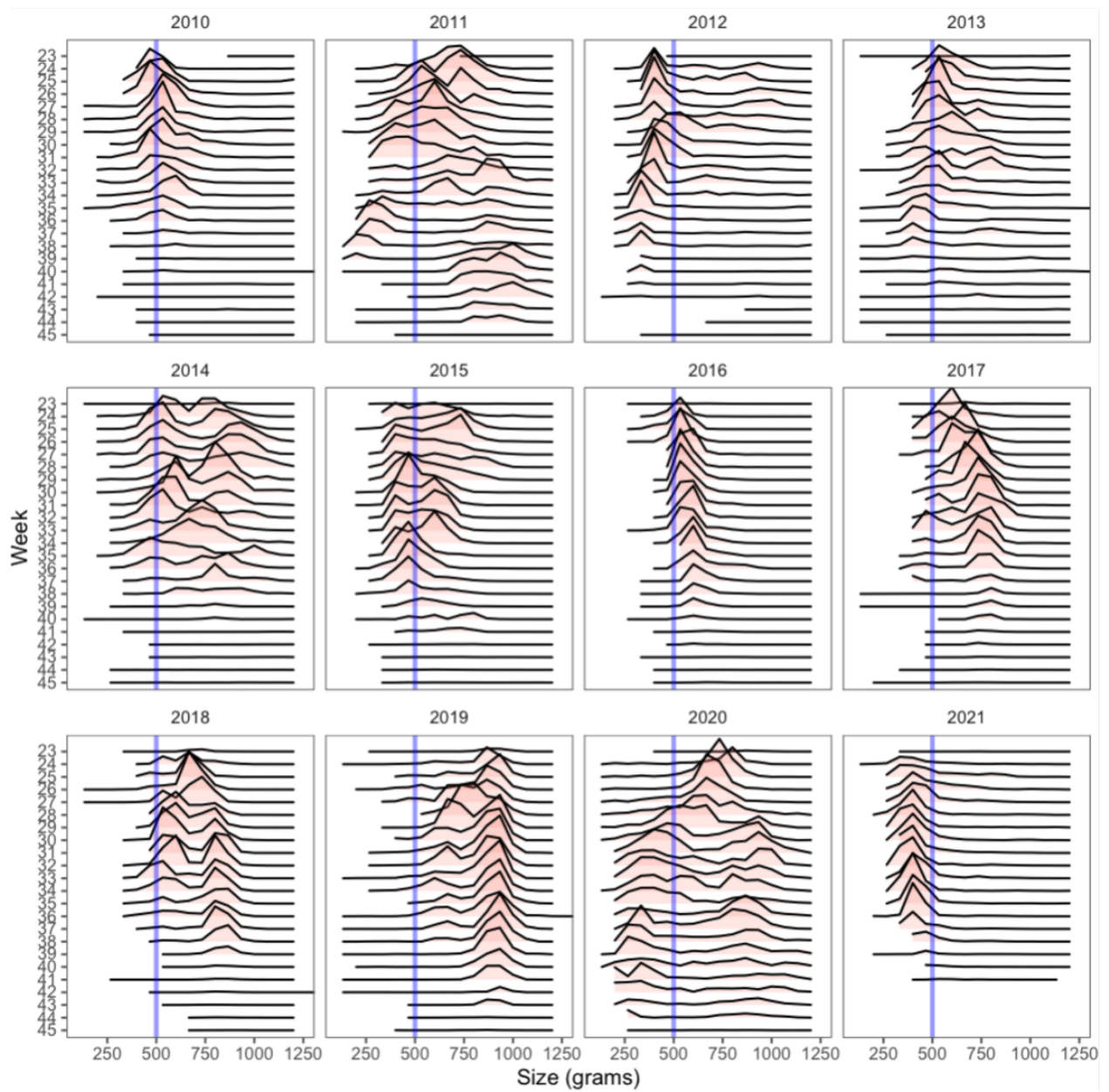
Figure 1-12. Pollock fishery data showing the frequency of mean pollock weight within a tow (in 50 g increments) by recent years and weeks of the B-season.
