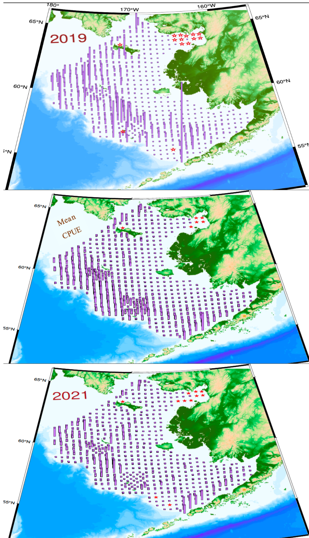
Figure 1-19. Bottom trawl survey pollock catch in kg per hectare for 2019 and 2021 (top and bottom) compared to the average station density (middle). Height of vertical lines are proportional to station-specific pollock densities by weight (kg per hectare) with constant scales for all years (red stars indicate tows where pollock were absent from the catch).
