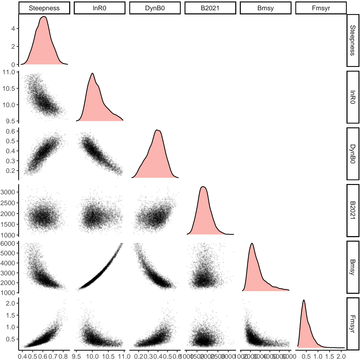
Figure 1-42. Pairwise plot of selected EBS pollock parameters and output from 3 million MCMC iterations thinned such that 5 thousand draws were saved as an approximation to the multivariate posterior distribution. Note that the figures on the diagonal represent the marginal posterior distributions. Key: lnR0 is the parameter that scales the stock-recruit relationship, B_Bmsy is estimated B_{2021}/B_{MSY} , DynB0 is the ratio of spawning biomass estimated for in 2021 over the value estimated that would occur if there had been no fishing, B2021 is the spawning biomass in 2021, and B_Bmean is B_{2021}/\bar{B} .
