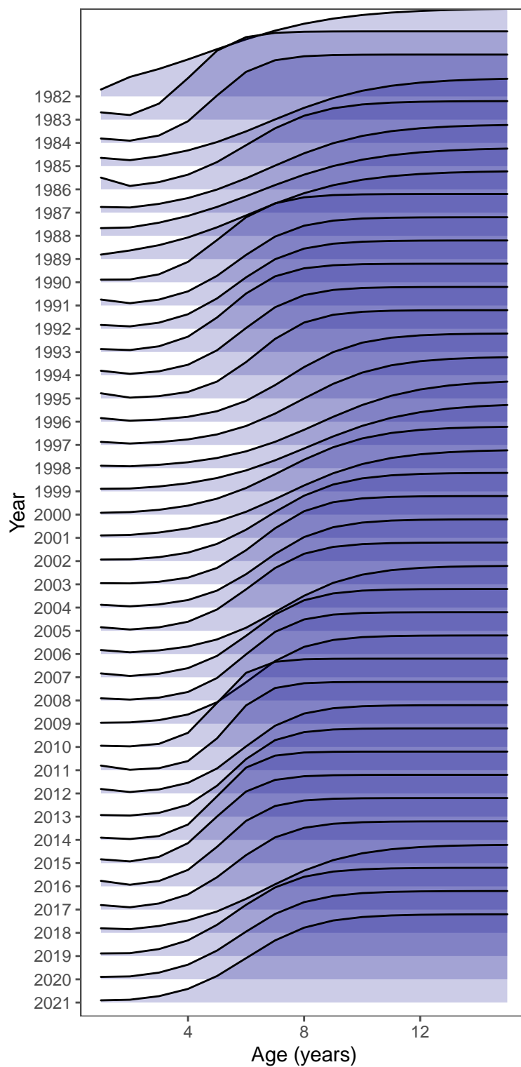
Figure 1-39. Model estimates of bottom-trawl survey selectivity, 1982–2021.
