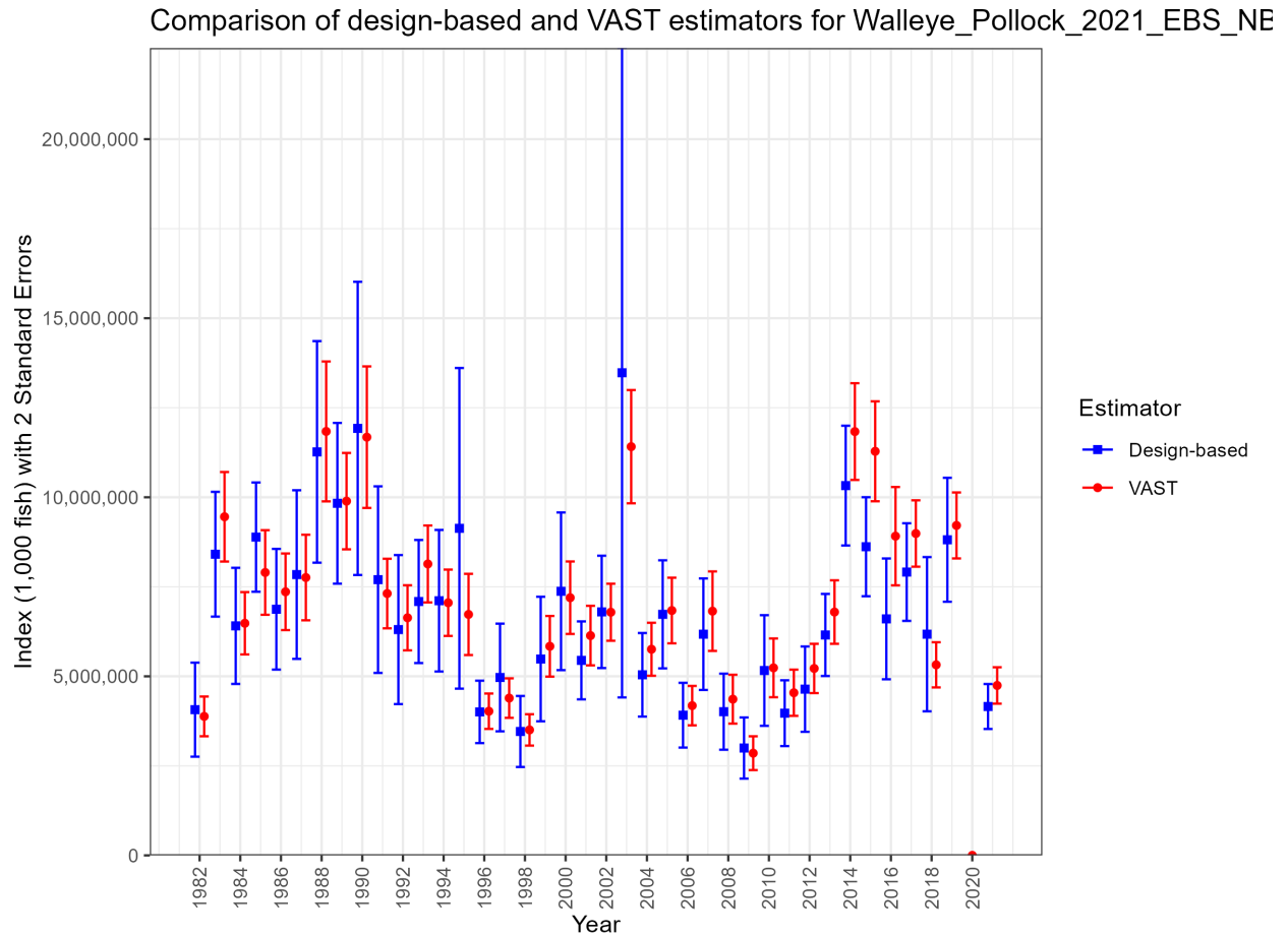
Figure 1-16. Bottom-trawl survey biomass estimates with error bars representing 95% credible interval (for design-based and VAST model-based methods) for EBS pollock.
