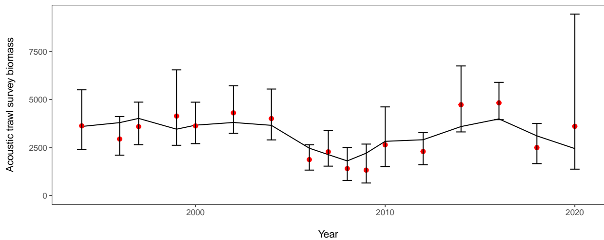
Figure 1-35. EBS pollock model fit to the ATS biomass index, 1994–2020.
