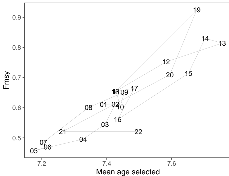
Figure 1-49. Comparison of F_{MSY} and mean selected age. The horizontal axis is a way to summarize if selectivity is tend towards younger or older fish. Labels indicate the year that demographic parameters (weight-at-age, selectivity) were used to compute F_{MSY} .
