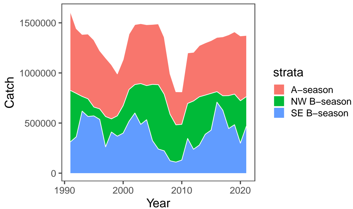
Figure 1-2. Pollock catch estimates (t) from the Eastern Bering Sea by season and region. The A-season is defined as from Jan-May and B-season from June-October.
