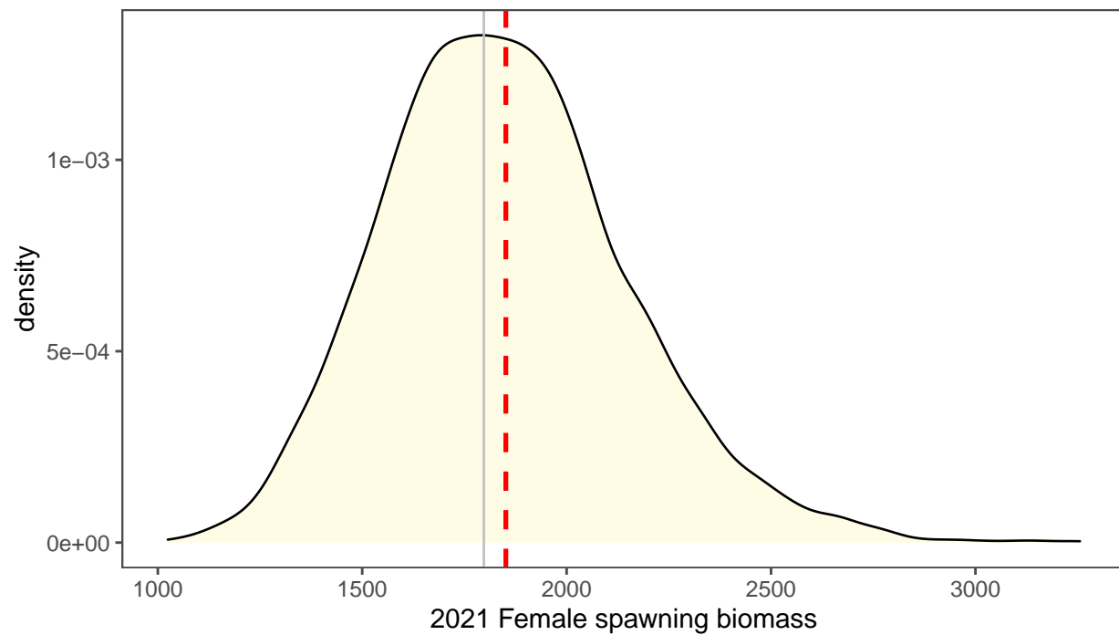
Figure 1-43. Integrated marginal posterior density (based on MCMC results) for the 2021 EBS pollock female spawning biomass compared to the point estimate (dashed red line).
