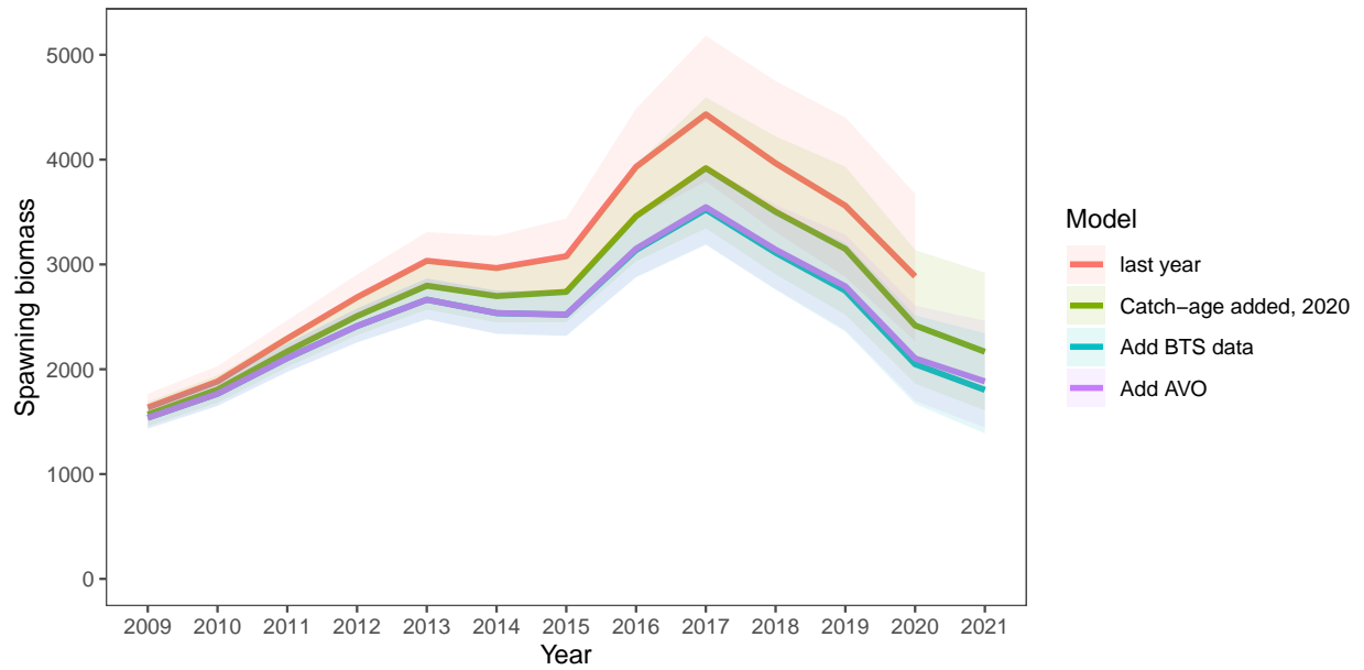
Figure 1-30. Model runs comparing last year's assessment with the impact of sequentially adding new data (first 2021 catch and 2020 fishery catch-at-age, then the 2021 bottom trawl survey data point, and finally the AVO data based on acoustic backscatter).
