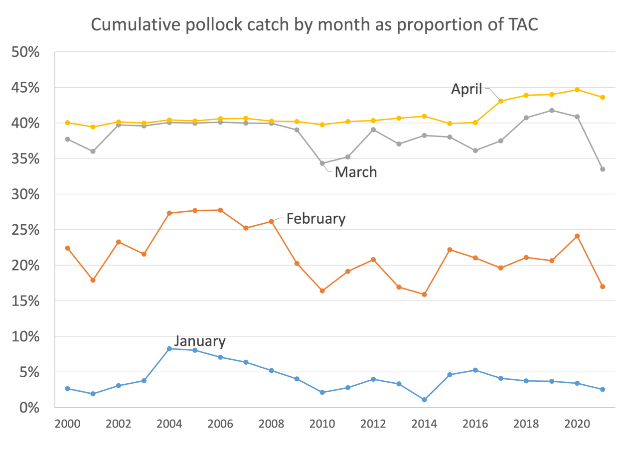
Figure 1-7. Proportion of the annual EBS pollock TAC by month during the A-season, 2000–2021. The higher value observed since 2017 was due to Amendment 110 of the FMP to allow greater flexibility to avoid Chinook salmon.
