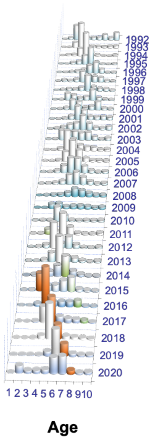
Figure 1-14. EBS pollock fishery estimated catch-at-age data (in number) for 1992–2020. Age 10 represents pollock age 10 and older. The 2012 year-class is shaded in orange.
