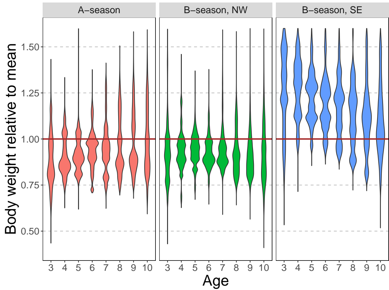
Figure 1-28. Fishery average weight-at-age anomaly (relative to mean) across strata and combined for all ages (3–10), and available years (1991–2020). Vertical shape reflects uncertainty in the data (wider shapes being more precise), colors are consistent with cohorts.
