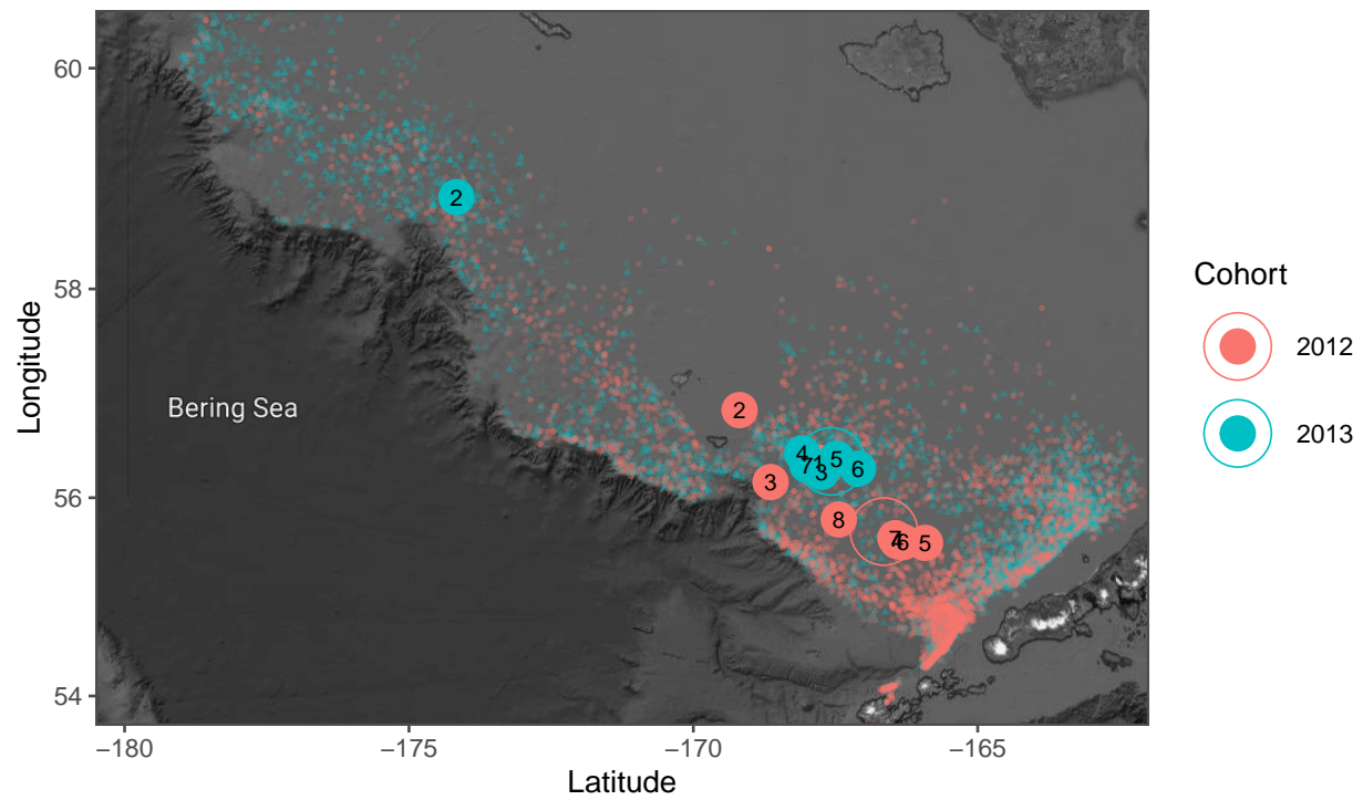
Figure 1-15. Pollock age sample locales (small dots) for two recent cohorts representing the 2012 and 2013 year-classes (from data through 2020). The large dots represent simple mean latitude and longitude of the samples.
