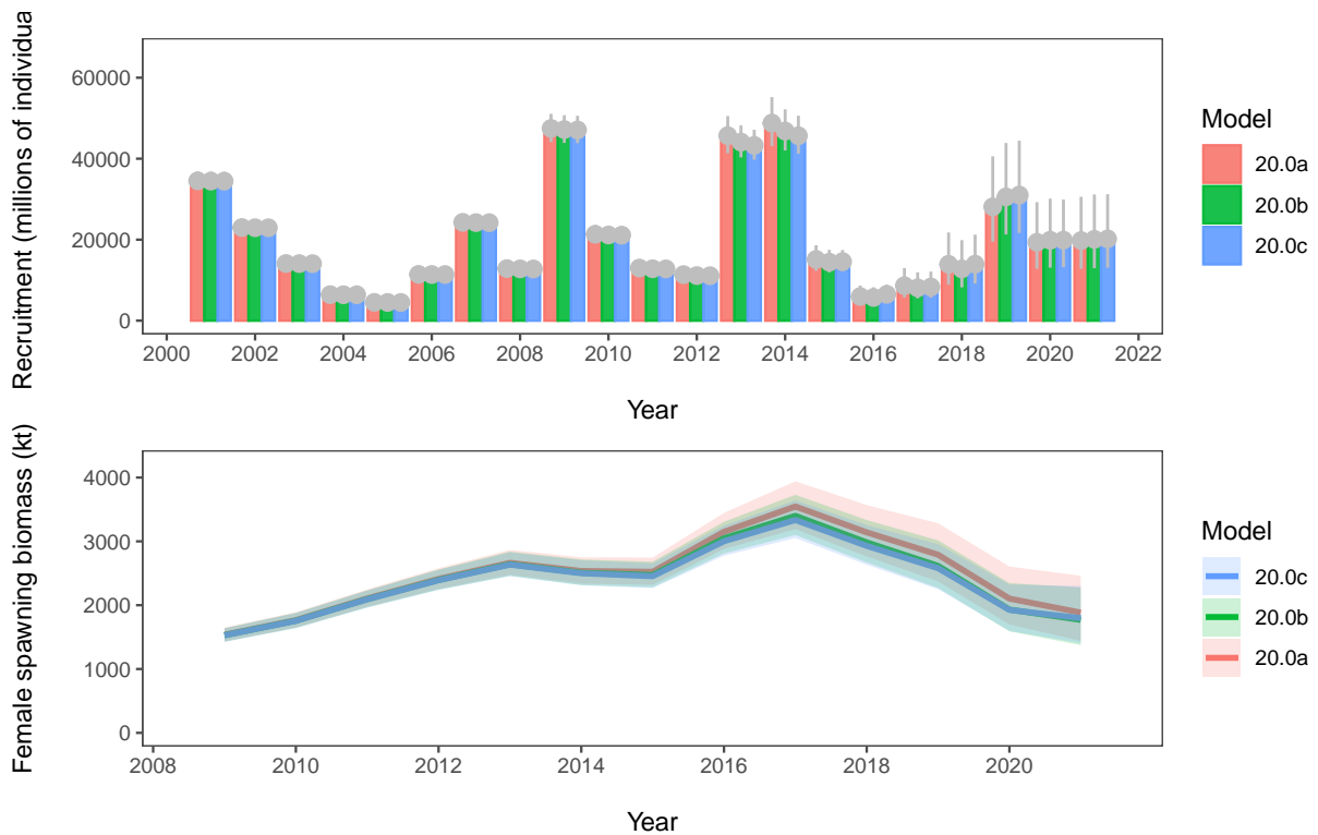
Figure 1-31. Model results showing the impact of adding in preliminary fishery length and age composition data from 2021.
