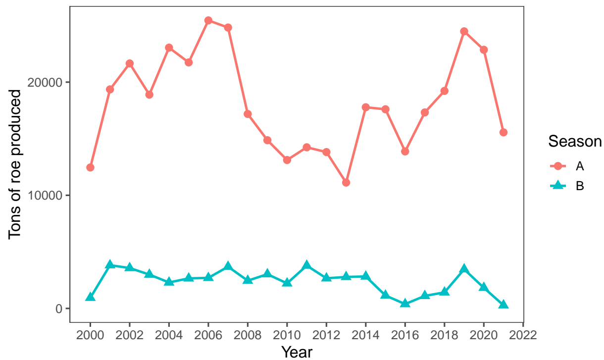
Figure 1-8. EBS pollock roe production in A and B seasons , 2000-2021.
