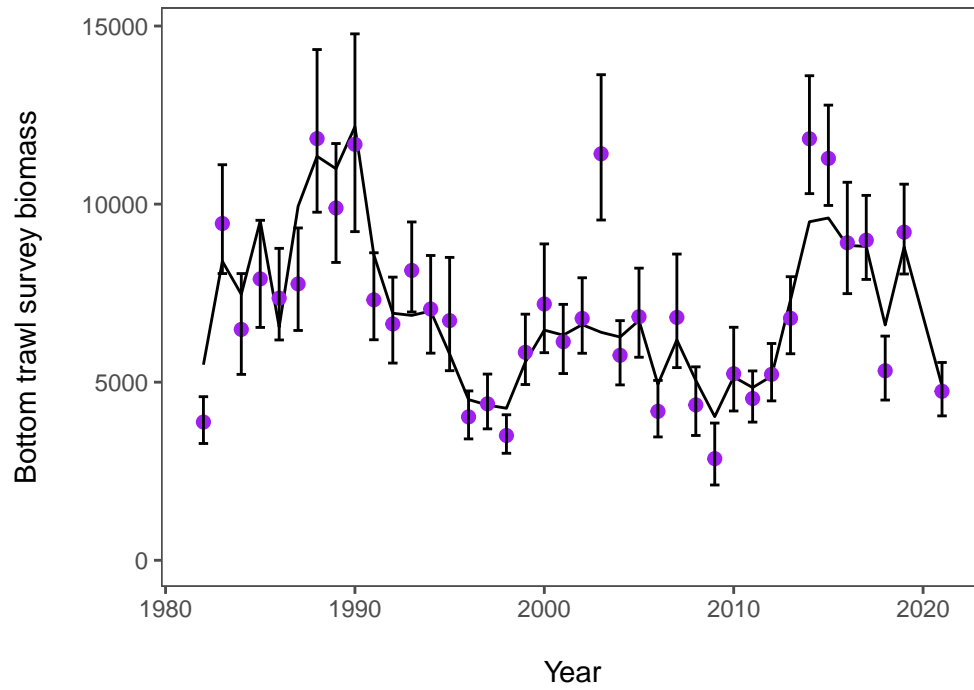
Figure 1-34. EBS pollock model fit to the BTS survey data (density dependence corrected estimates), 1982–2019, 2021. Units are relative biomass.
