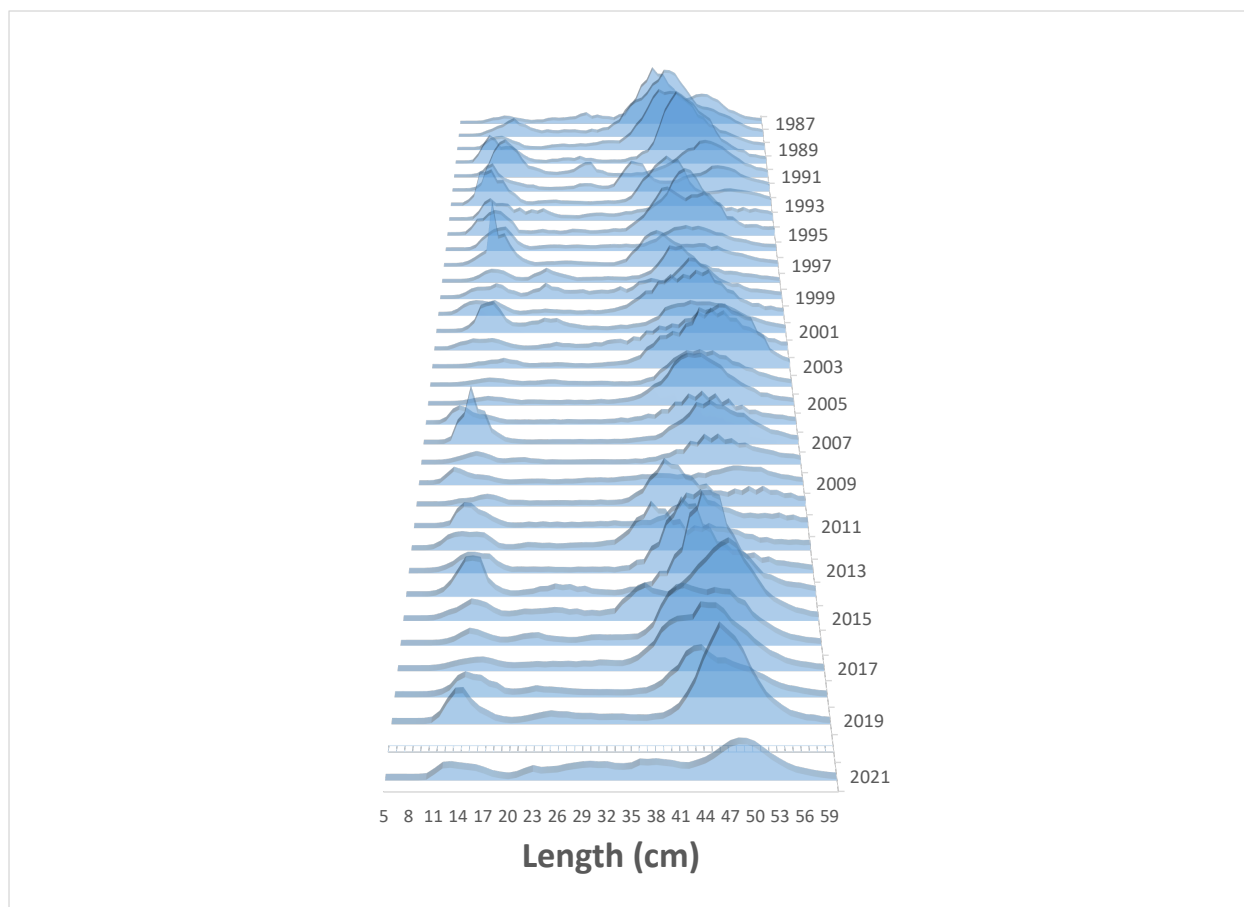
Figure 1-21. Pollock abundance levels by size and year as estimated directly from the NMFS bottom-trawl surveys (1990–2019, 2021).
