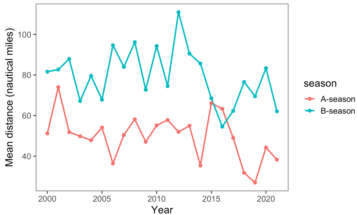
Figure 1-10. Estimated mean daily distance between operations, 2000-2021.
