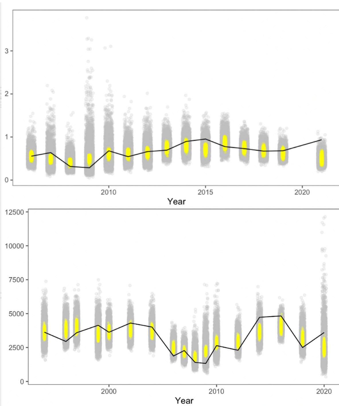
Figure 1-45. Plot of the model prediction (solid line), the distribution of the expected value (yellow dots) and the posterior predictive distribution (grey points).
