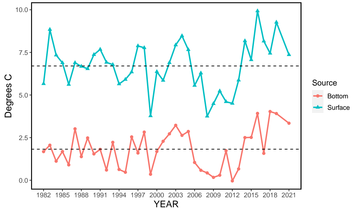
Figure 1-17. Bottom and surface temperatures for the Bering Sea from the NMFS summer bottom-trawl surveys (1982–2019, 2021). Dashed lines represent mean values.
