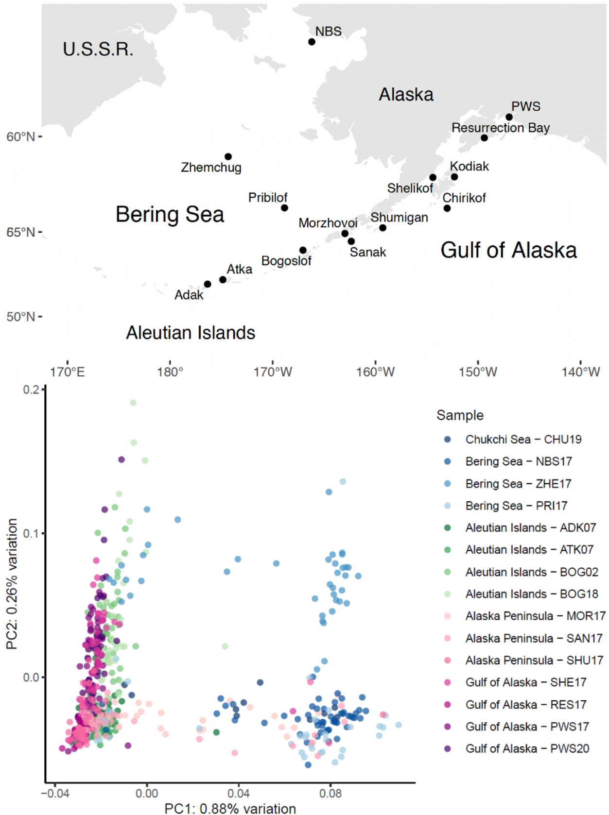
Figure 1-1. Principal Component Analysis of walleye pollock genetics. The color of each point indicates the sampling location and region shown in the map at top (Chukchi samples are further north).
