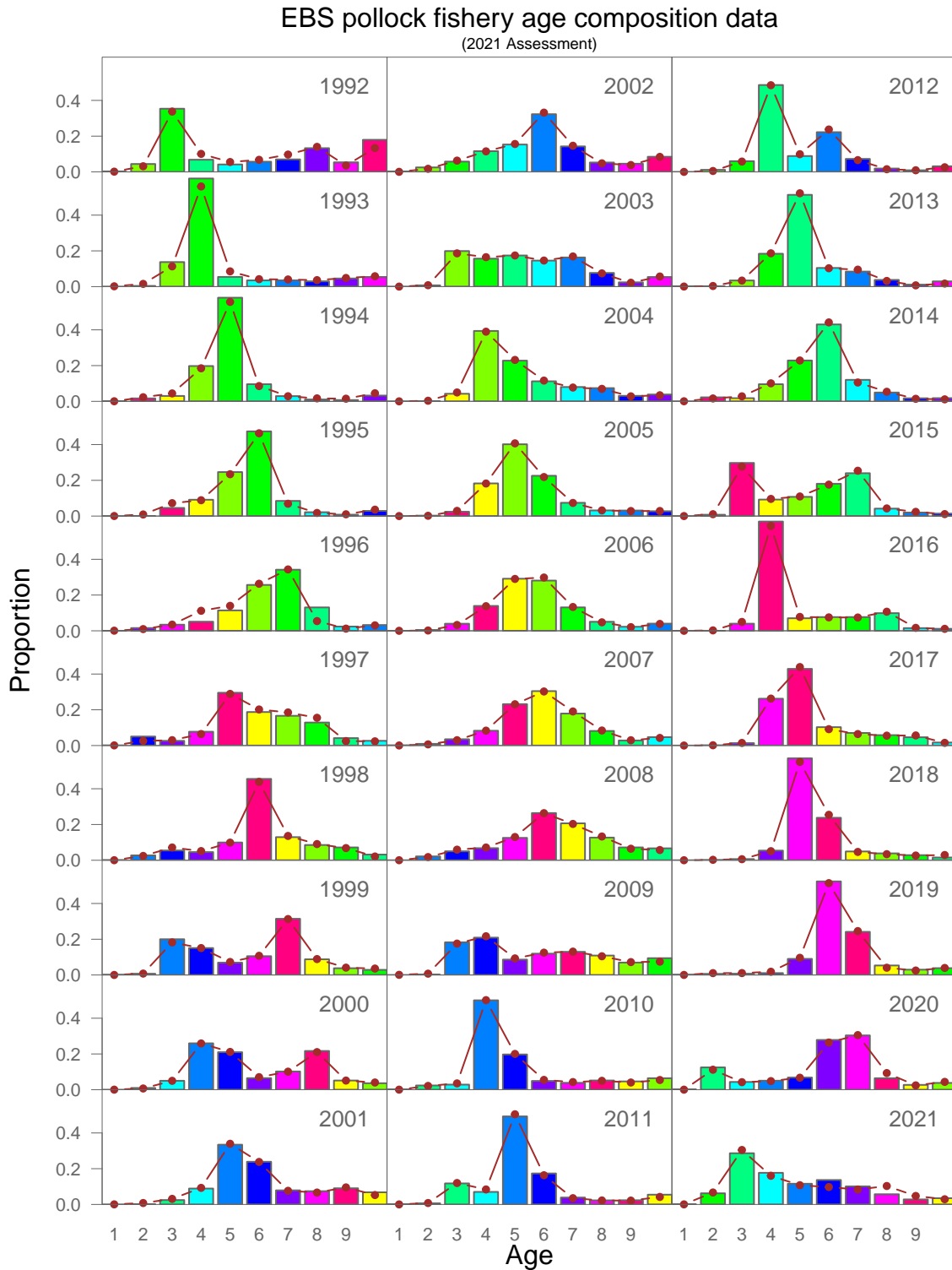
Figure 1-38. Model fit (dots) to the EBS pollock fishery proportion-at-age data (columns; 1992–2021). The 2020 data are new to this year’s assessment as are the preliminary 2021 data. Colors coincide with cohorts progressing through time.
