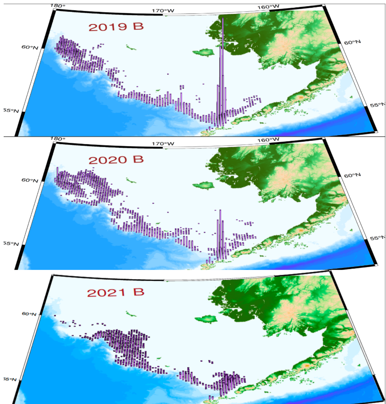
Figure 1-9. EBS pollock catch distribution during B-season, 2019–2021. Column height is proportional to total catch. Note that directed fishery for pollock generally is finished prior to October; the labels are indicative full-year catches.
