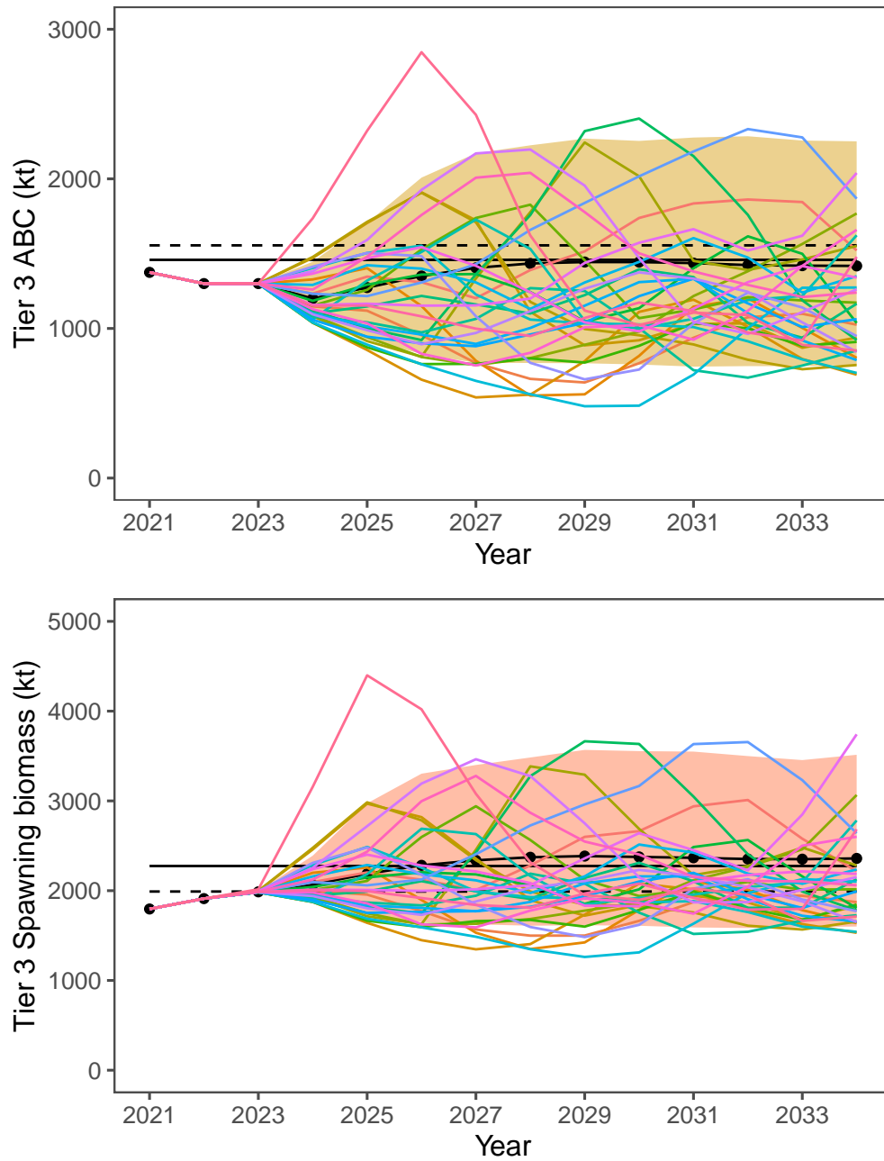
Figure 1-59. Projected EBS Tier 3 pollock yield (top) and female spawning biomass (bottom) relative to the long-term expected values under F_{35\%} and F_{40\%} (horizontal lines). B_{40\%} is computed from average recruitment from 1978–2017. Future harvest rates follow the guidelines specified under Tier 3 Scenario 1.
