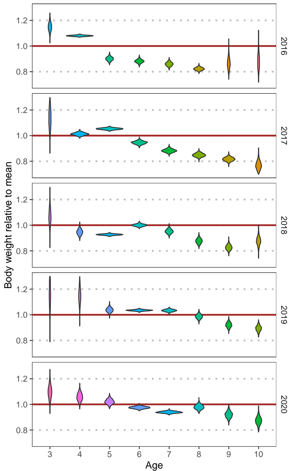
Figure 1-26. Recent fishery average weight-at-age anomaly (relative to mean) by strata for ages 3–10, 2016–2020. Vertical shape reflects uncertainty in the data (wider shapes being more precise), colors are consistent with cohorts.
