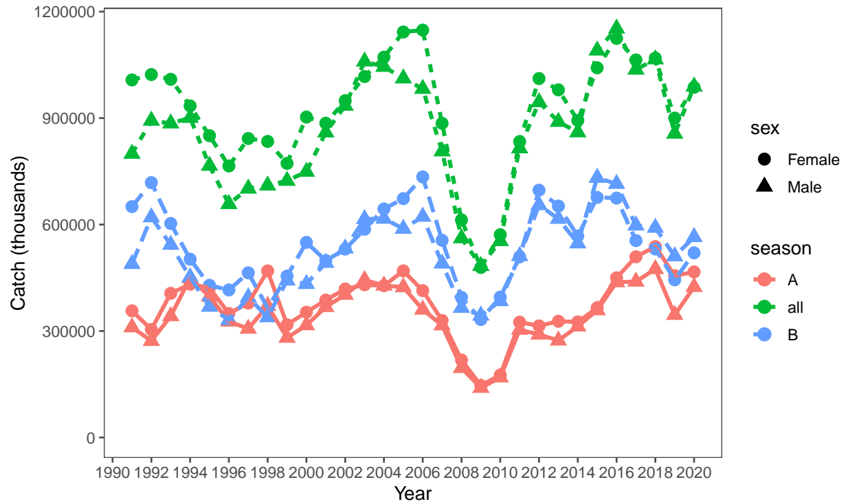
Figure 1-4. Estimate of EBS pollock catch numbers by sex for the A season (January-May) and B seasons (June-October) and total.
