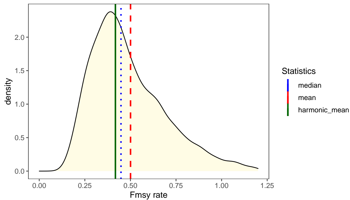
Figure 1-44. Integrated marginal posterior density (based on MCMC results) for the F_{MSY} for EBS pollock and different central tendency values..
