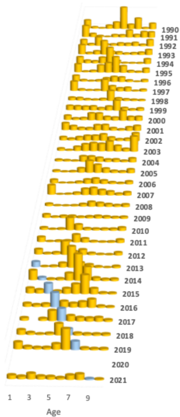
Figure 1-20. Pollock abundance levels by age and year as estimated directly from the NMFS bottom-trawl surveys (1990–2019,2021). The 2012 year-class is shaded differently.
