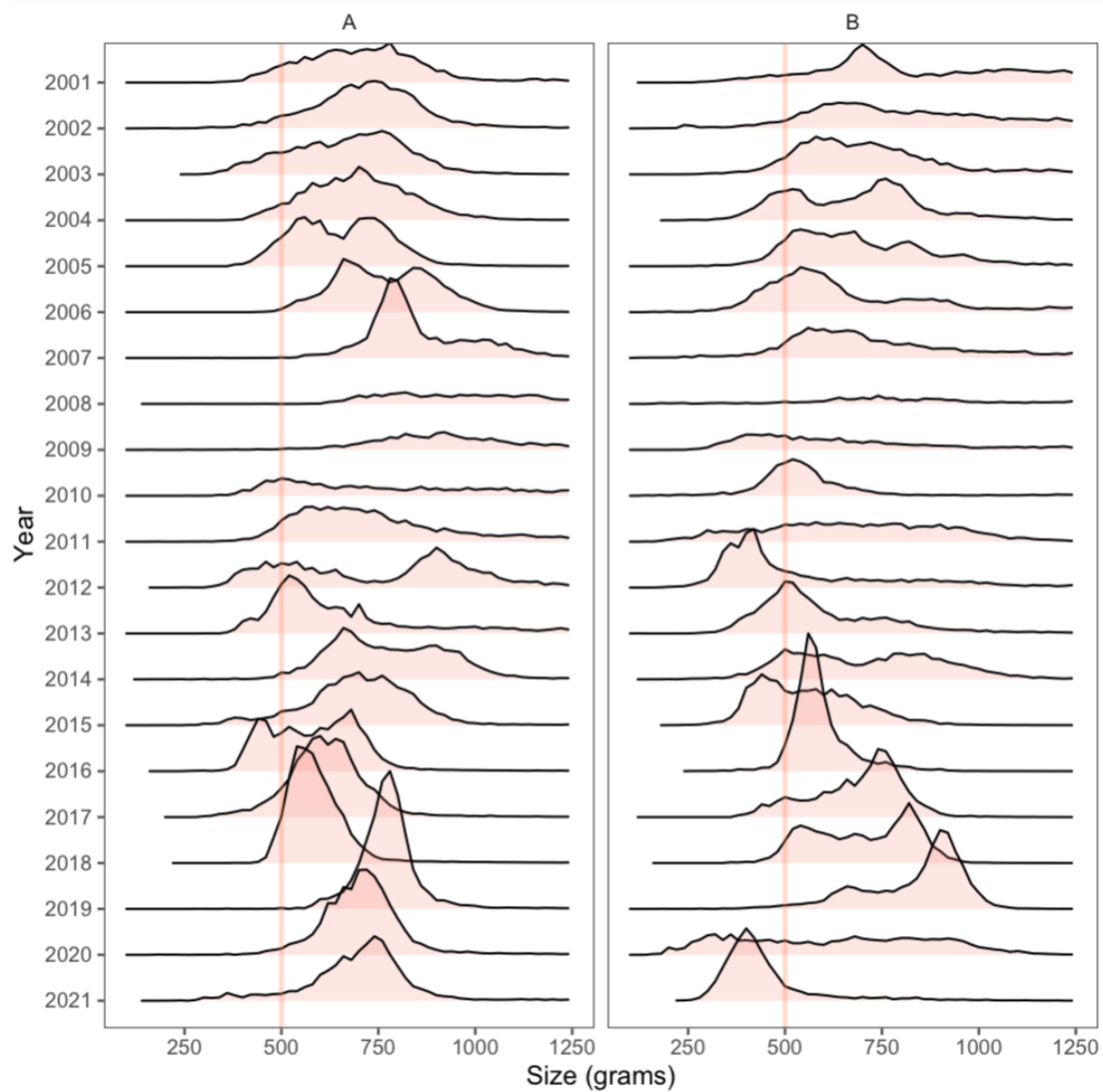
Figure 1-11. Pollock fishery data showing the frequency of mean pollock weight within a tow (in 50 g increments) by year and season.
