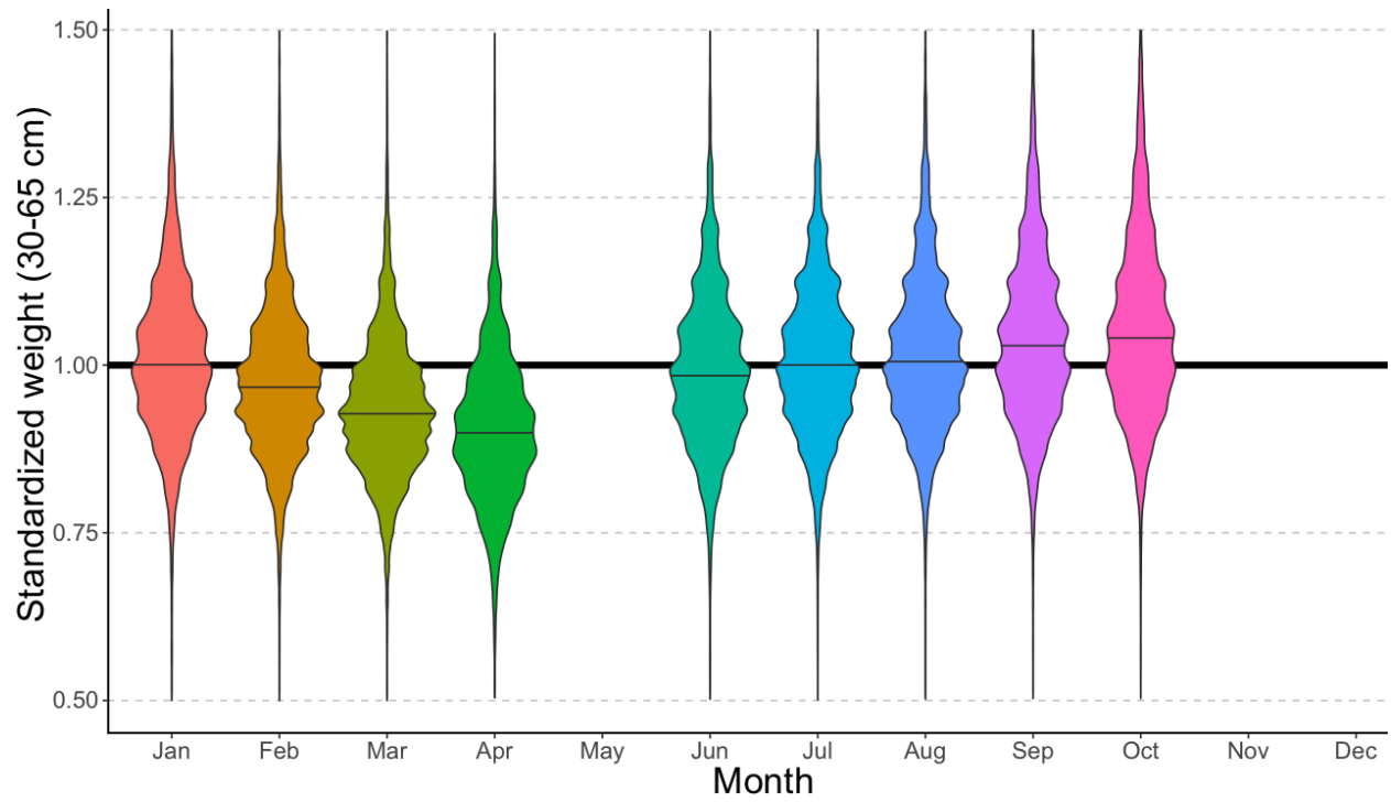
Figure 1-23. EBS pollock fishery body mass (given length) anomaly (standardized by overall mean body mass at each length) by month based on some over 700 thousand fish measurements from 1991–2021.
