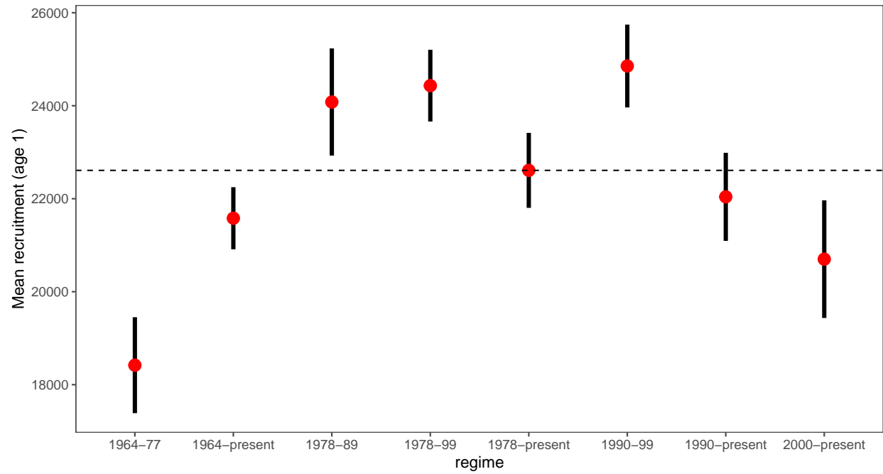
Figure 1-58. Mean recruitment estimates (age-1) for EBS pollock for different periods with error bars representing 95% credible intervals.
