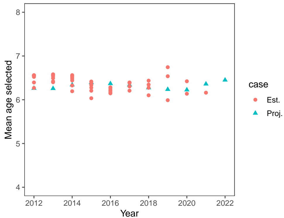
Figure 1-48. Retrospective pattern for the mean selected age (ages 1-8) based on estimated EBS pollock fishery selectivity compared to the projected selectivity from the year prior.
