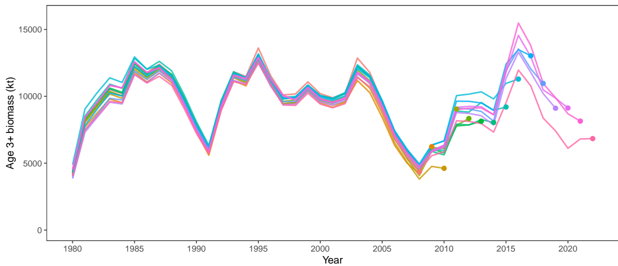
Figure 1-52. Comparison of the current assessment results with past assessments of begin-year EBS age-3+ pollock biomass.
