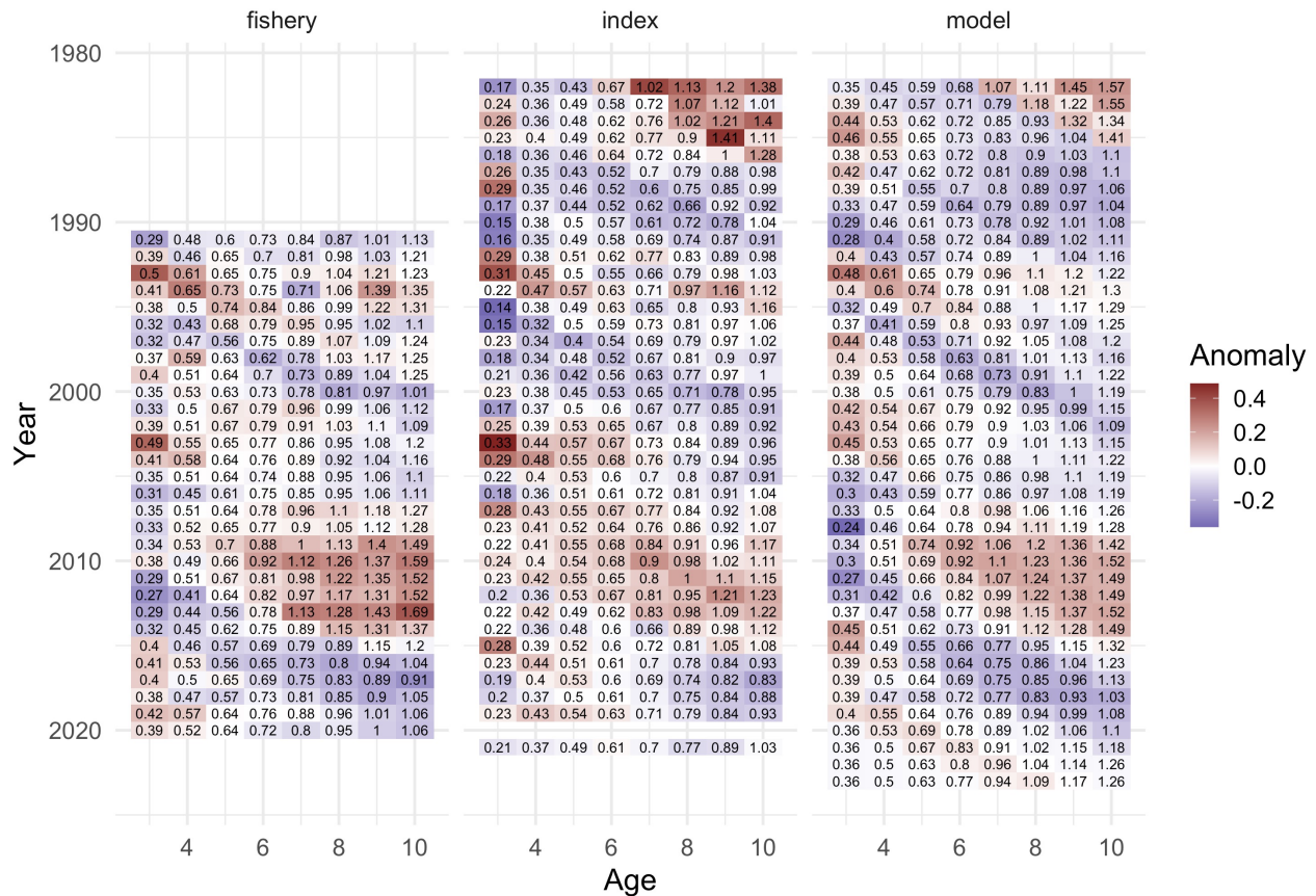
Figure 1-27. Data input and model predictions for the weight-at-age random-effects model fit separately to obtain variance estimates for cohort and year effect contributions to changes in incremental growth from one age to the next. Shadings reflect the anomaly from the mean while the numbers are the weight-at-age in kg.
