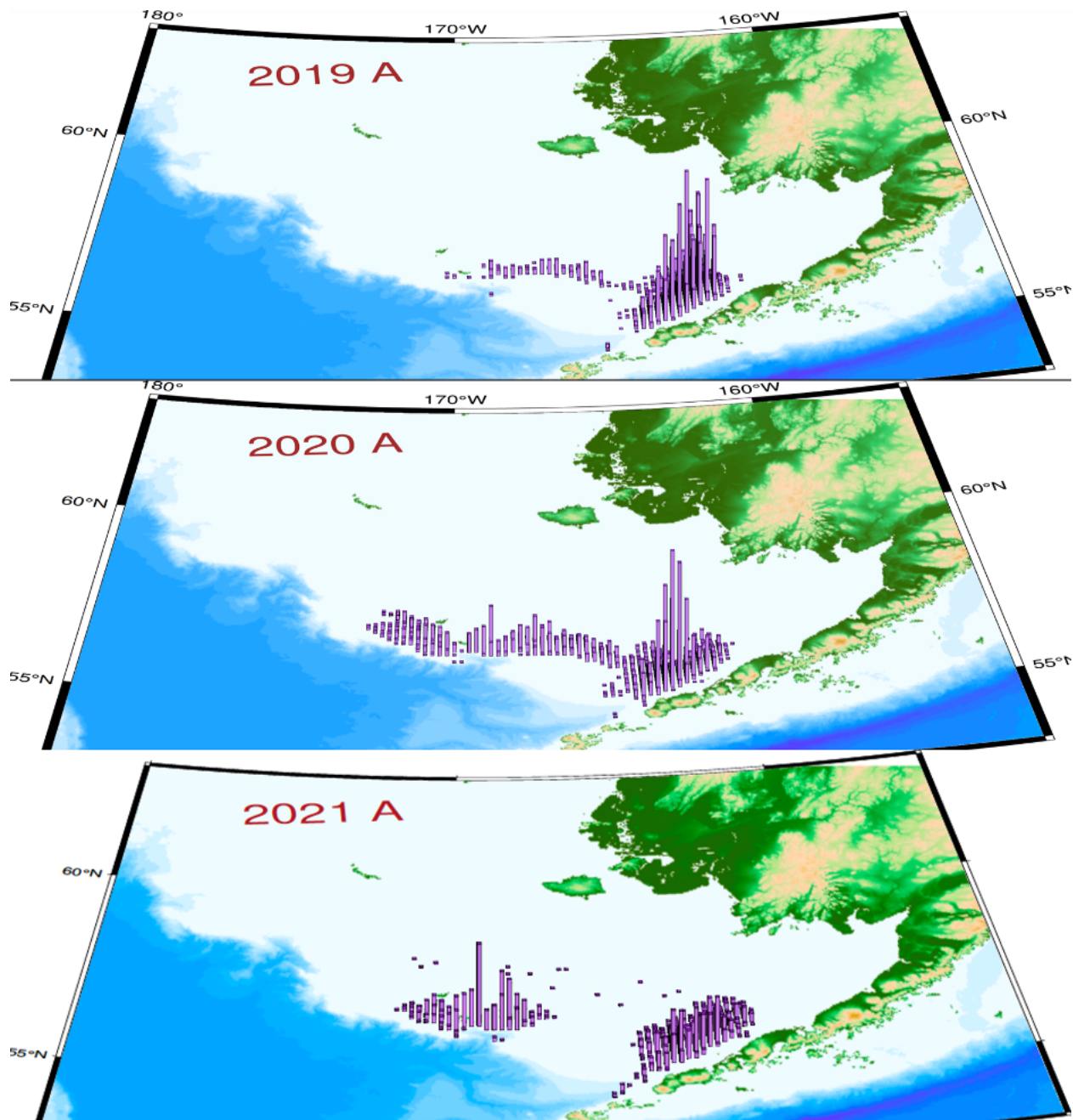
Figure 1-5. EBS pollock catch distribution during A-season, 2019–2021. Column height is proportional to total catch.
