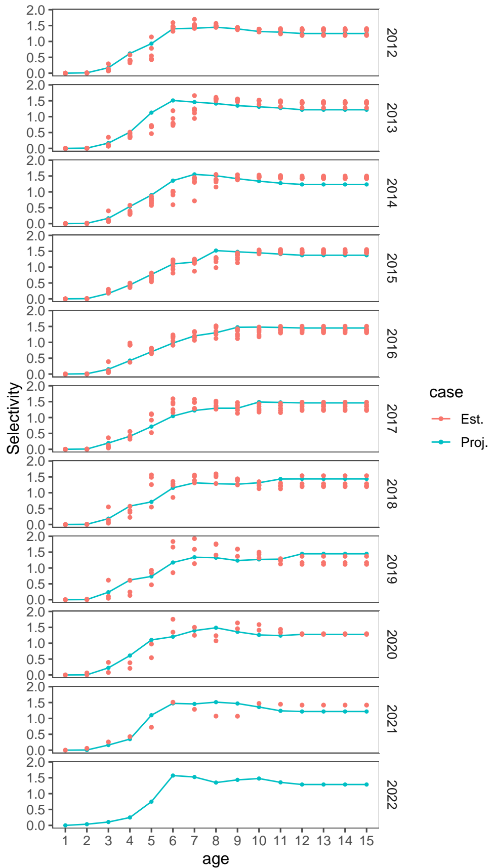
Figure 1-47. Retrospective pattern for estimated EBS pollock fishery selectivity (dots) compared to the projected selectivity from the year prior (solid line).
