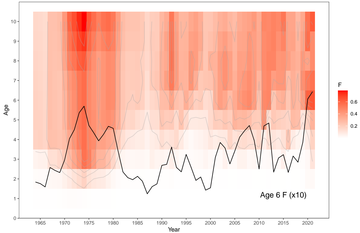
Figure 1-51. Estimated instantaneous age-specific fishing mortality rates for EBS pollock.
