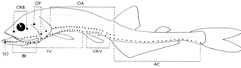
Figure 8. Generalized photophore patterns for gonostomatids (Fahay, 1983). For photophore definitions, see Table 16.
